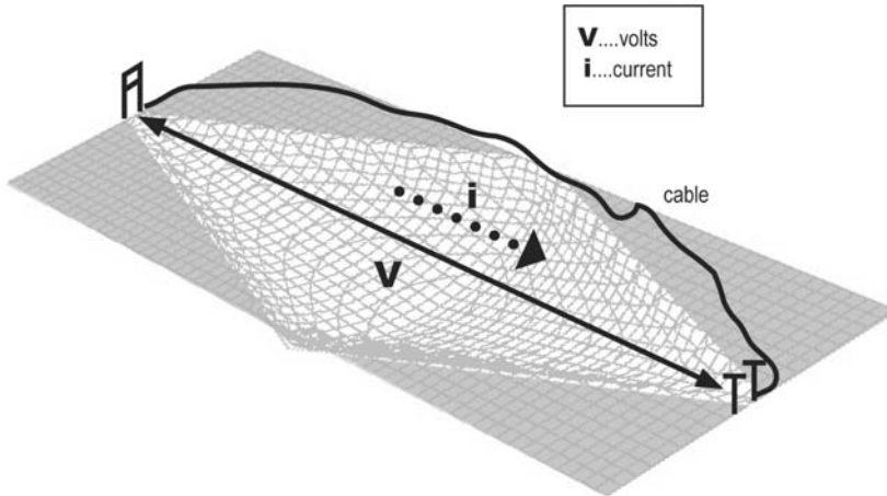
Figure 3.2 The twin probe arrangement actually uses four probes. It measures the voltage between two and the current through the other two. The current spreads out while it travels through the ground.
