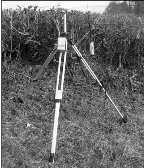
Figure 3.19 A GPS total station: (a) the roving unit, (b) the ground station.
