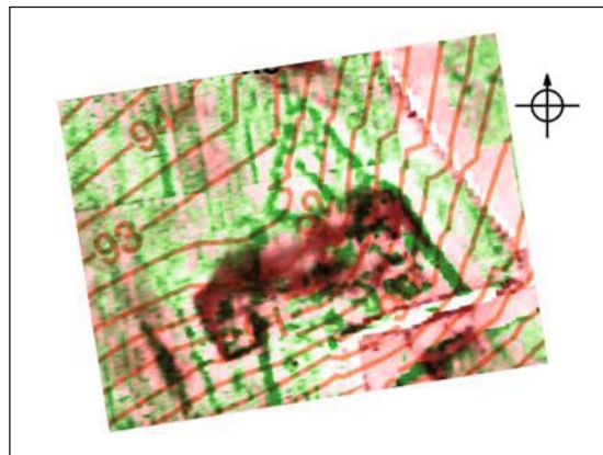
Plate 9 An overlay of a res plot of a Roman villa (red) on a mag plot of a ditched enclosure (green). The building lies right over some ditches. Contours are also overlaid.
