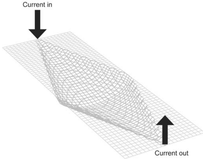
Figure 2.3 Electrical current may enter the ground at one point and leave at another, but between those points it spreads out. It does not travel in a line, as it does in a wire.
