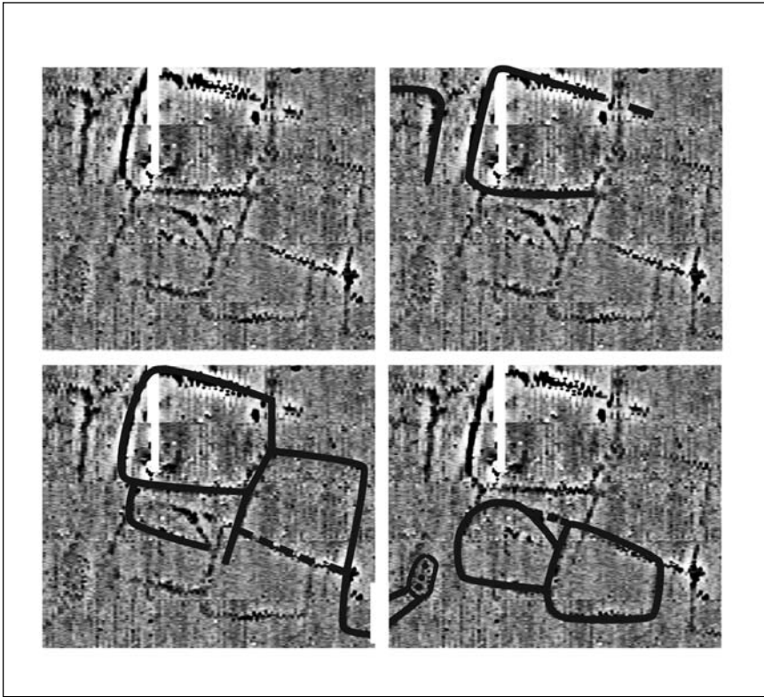
Figure 4.11 Features found by mag in a field, and a possible interpretation of these as separate phases of activity: original plot is top left, then three successive phases of activity. This interpretation need not be correct. Only excavation could reveal the true chronology.
