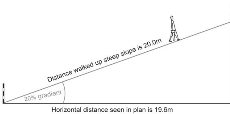
Figure 3.25 Steep slopes can cause surveying problems. The distance you actually walk up the slope is more than the 'level' distance. Which do you use in the survey?
