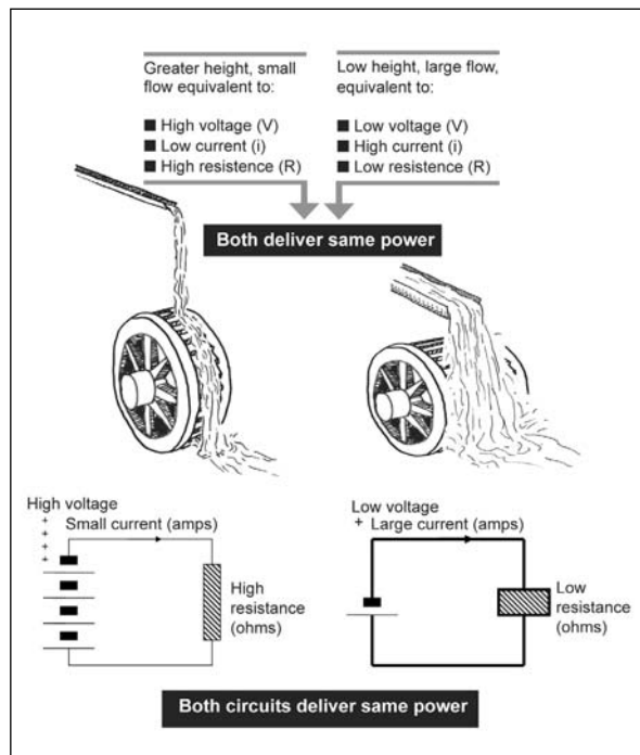
Figure 2.1 Electrical voltage is like water height, and current like water flow. In each case, the 'height' times the 'flow' gives the power delivered, and the 'height' divided by the 'flow' gives the resistance.
