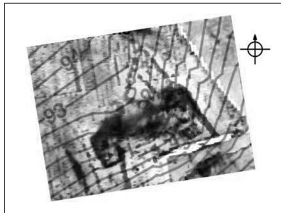
Figure 4.7 An overlay of a res plot of a Roman villa (red) on a mag plot of a ditched enclosure (green). The building lies right over some ditches. Contours are also overlaid. See also Plate 9.
