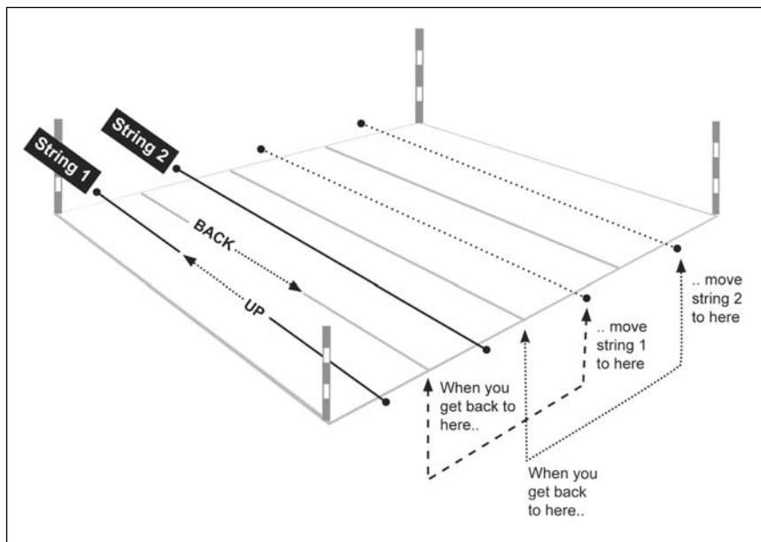
Figure 5.9 Laying out walking ropes, and walking the grid, based on the arrangement in Figure 5.8 (c).
