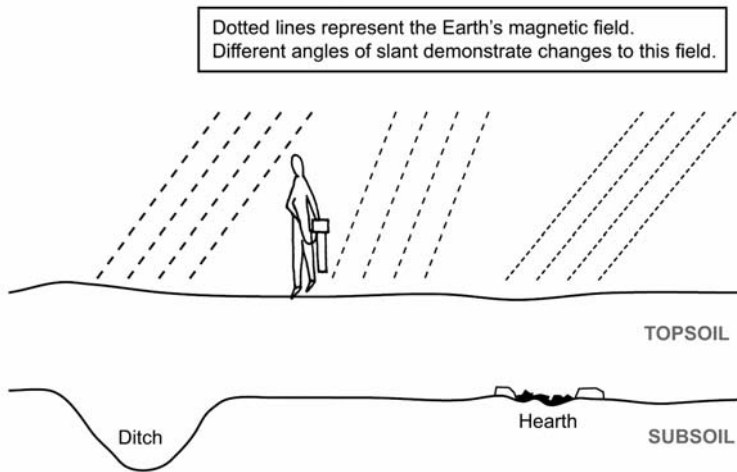
Figure 2.6 The presence of magnetic material in a now-filled ditch will cause a small disturbance to the Earth's magnetic field. Burning will also cause materials to disturb the magnetic field.
