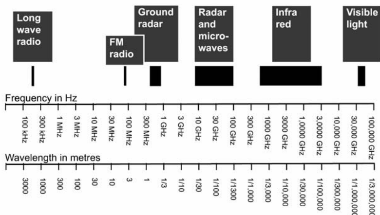
Figure 2.7 Light is only a small part of the spectrum of electromagnetic waves, which includes radio, microwave and infra red. By spectrum, I mean the range of wavelengths.
