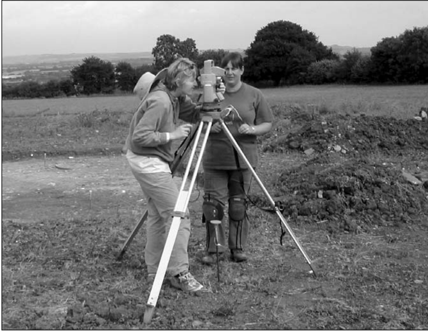
Figure 3.22 Electronic theodolite. The operator uses a telescope to point at a target. The laser above the telescope fires a beam to the target and detects the return. The electronics under the telescope calculates distance, angle, vertical angle and position of the target and logs the data.
