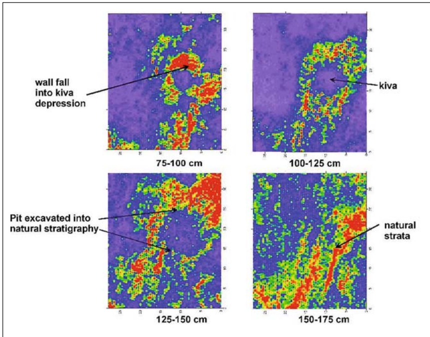
Plate 6 A set of time slices obtained by radar. Each slice represents a different depth under the surface, so you can see at what depth the archaeology is concentrated. Here it is mainly in slices 100–125 and 125–150 cm.
