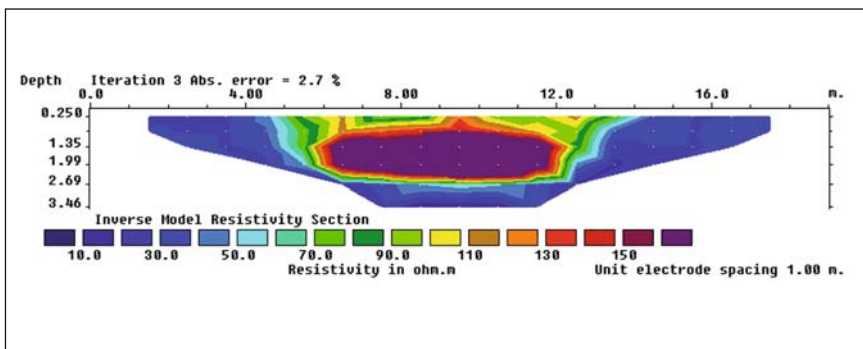
Plate 2 Vertical section obtained by depth profiling. The section gets narrower as less readings can be taken along the line at larger spacings. Blue is low resistance. The red shows a section through a buried building.
