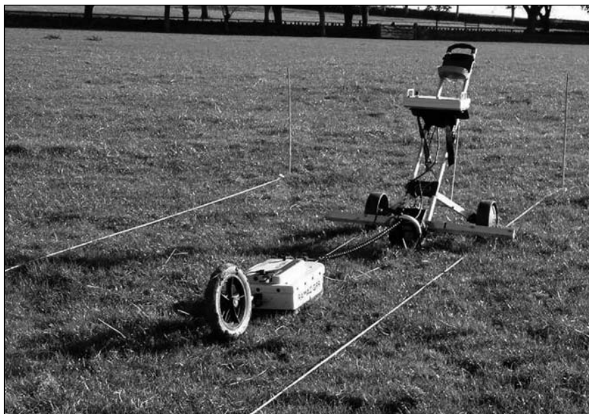
Figure 3.17 A typical radar set ready for use. The controls are on the buggy, with the antenna towed behind, and the wheel behind that measures distance.
