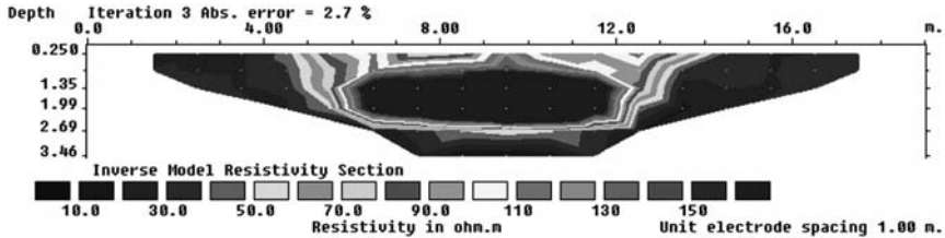
Figure 3.6 Vertical section obtained by depth profiling. The section gets narrower as less readings can be taken along the line at larger spacings. The outer area is low resistance. The inner area shows a section through a buried building. See also Plate 2.
