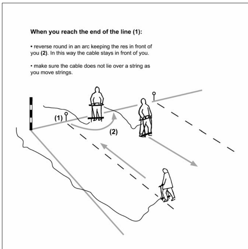
Figure 5.12 At the end of a line, reverse in an arc, keeping the res in front of you. This avoids tangling with the cable.
