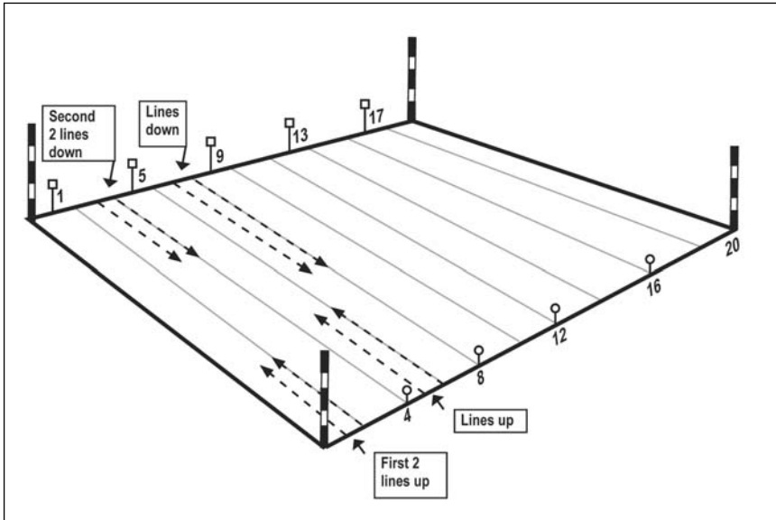
Figure 5.15 For using a double mag, 1m spacing, put flags at the top at 1m, 5m, 9m, 13m, 17m and pegs at the bottom, 4m, 8m, 12m, 16m, (20m).
