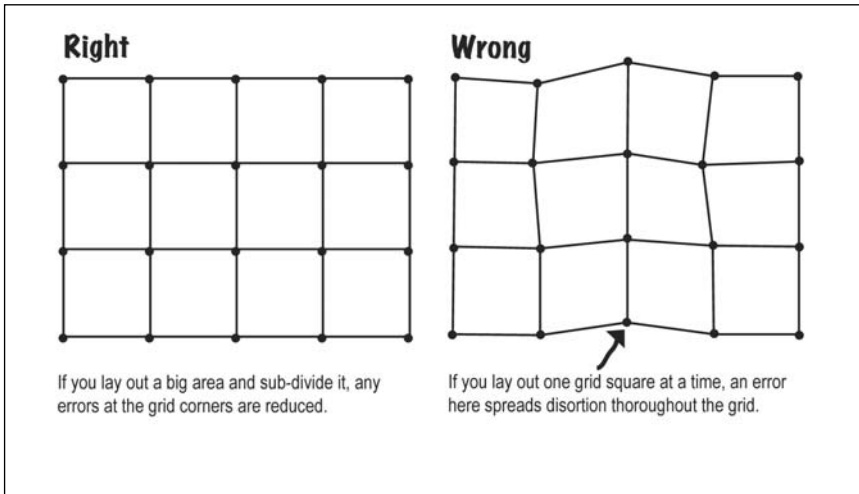
Figure 5.6 The grid gets distorted by one wrong measurement, and will get more distorted as it is expanded. The larger the area you can set up in one block, the less likelihood of an error growing.
