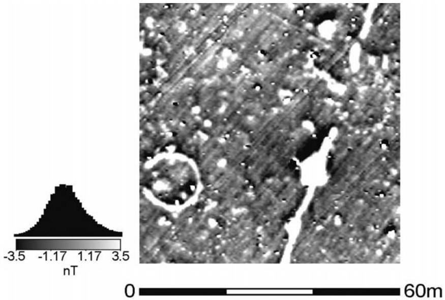
Figure 3.8 Computer output from a caesium magnetometer looks similar to that from a fluxgate device, but it can detect tinier anomalies.
