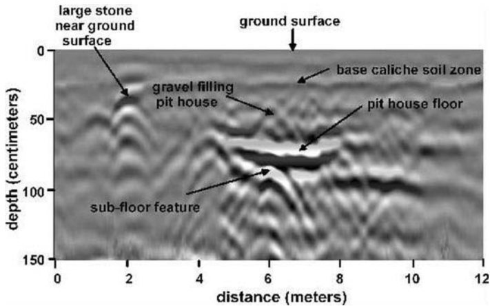
Figure 3.15 A typical radar screen, but which has been annotated by the user. Items appear as an upside down 'U', as the radar sees them first at a slant, and then closest as it passes directly overhead.
