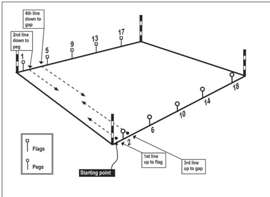
Figure 5.14 For mag without strings, put flags at the top, lines 1, 5, 9, 13, 17 and pegs at the bottom, lines 2, 6, 10, 14, 18.
