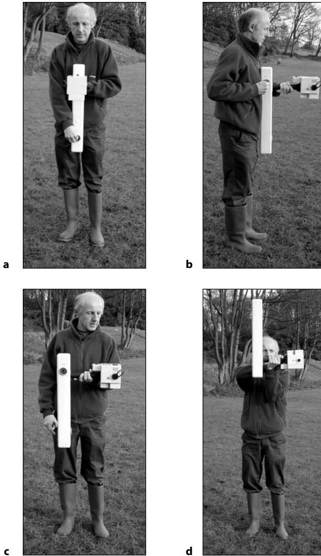
Figure 3.12 Calibrating the FM256. This involves holding the head first north (a), then south and adjusting to the average of the two readings; then measuring east (b) and then west and averaging, and then measuring upright (c) and upside down (d) and averaging.
