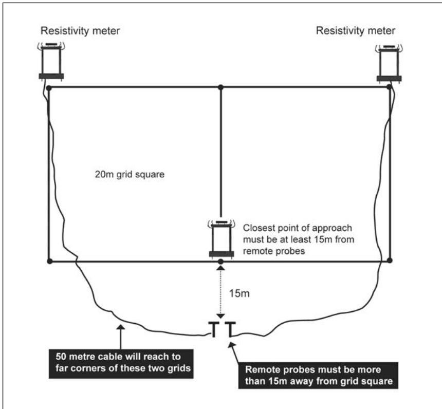
Figure 5.11 Setting the remote probes position to do two squares without needing to move them.
