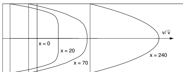
FIGURE 1.36. Velocity profiles in steady laminar flow at the entrance to a tube, showing the development of the parabolic velocity profile. The velocity is given as v/\bar{v} . At the entrance v/\bar{v} = 1 . When the Poiseuille flow is fully developed, v/\bar{v} is 2 at the center of the tube. These curves are calculated from a graph by Cebeci and Bradshaw (1977) for laminar flow in a tube of radius 2 mm and a pressure gradient of 20 \text{ torr m}^{-1} , carrying a fluid with a viscosity of 3 \times 10^{-3} \text{ N s m}^{-2} and a density of 10^3 \text{ kg m}^{-3} . The scales are different along the axis and radius of the tube; the tube radius is 2 mm and the entrance region is 240 mm long.
