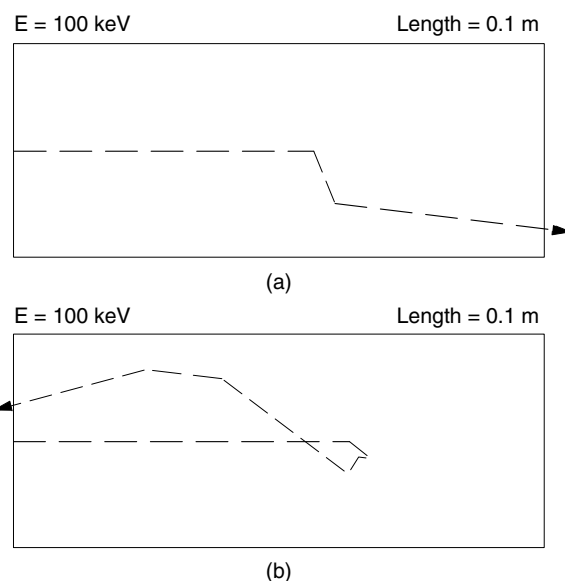
FIGURE 15.34. Secondary photons also interact in this simulation. One 100-keV photon enters from the left in each panel. (a) The primary photon undergoes a Compton scattering. The Compton-scattered photon also undergoes a Compton scattering. The third photon escapes from the water. (b) The primary photon is Compton scattered. Each Compton-scattered photon undergoes another Compton scattering, until the sixth scattered photon leaves through the upstream surface of the water, traveling nearly in the direction from which the incident photon came.
