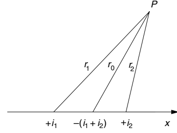
FIGURE 7.5. The axon of Fig. 7.4 is stretched along the x axis. There are current sources at x = -x_1 and x = x_2 , and a current sink at the origin. The distances from each source or sink to the observation point are shown.
