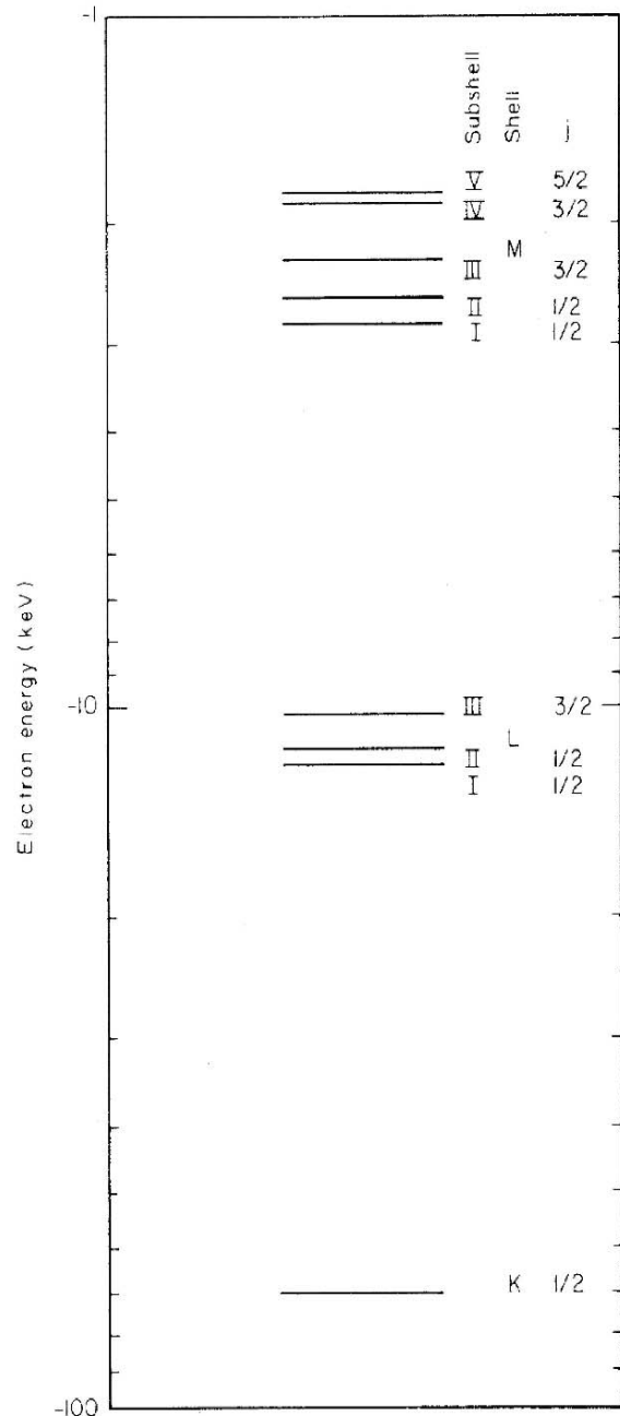
FIGURE 15.1. Energy levels for electrons in tungsten.
