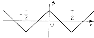
FIGURE 11.22. Plot of \phi_{11}(\tau) for the square wave.
