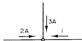
FIGURE 6.22. Conservation of charge means that current i is -5 A.
