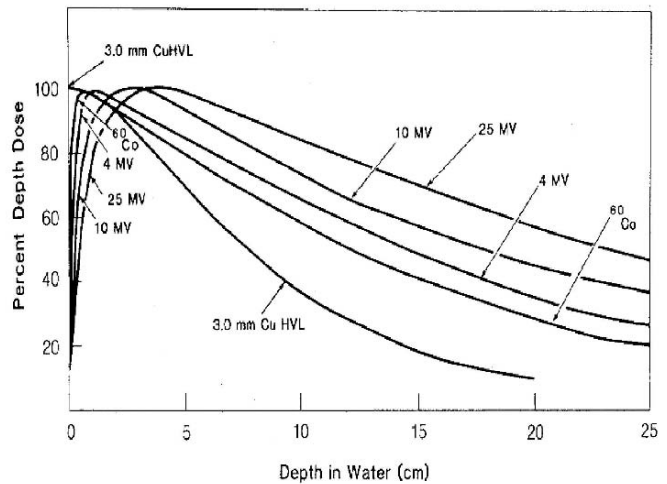
FIGURE 16.45. The dose vs depth for x-ray beams of different quality (energy) on the central axis of the beam. The source—surface distance (SSD) is 100 cm and the field size is 10 cm \times 10 cm. The curve “3.0 mm Cu HVL” is for a photon beam that is reduced to half intensity by a copper filter 3.0 mm thick. The labels 4, 10 and 25 MV refer to the energy of the electron beam striking the target. From F. M. Khan (2003). The Physics of Radiation Therapy , 3rd. ed. Philadelphia, Lippincott Williams & Wilkins, p.163. ©2003 Lippincott Williams and Wilkins.
