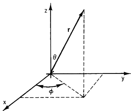
FIGURE L.1. Spherical coordinates.
