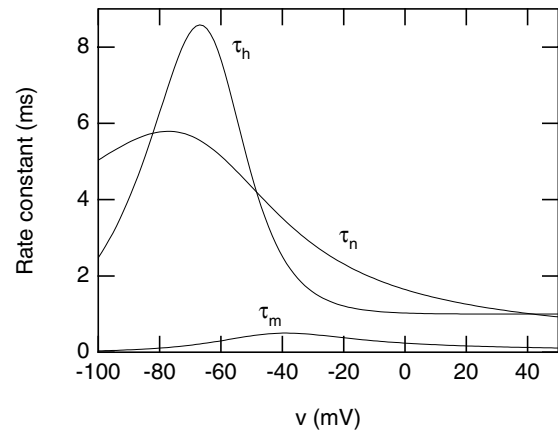
FIGURE 6.37. Plots of the sodium and potassium conductance parameters versus the transmembrane potential.
