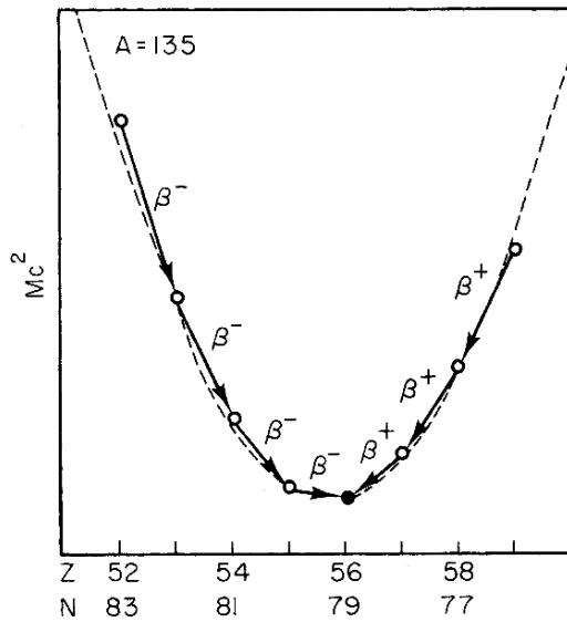
FIGURE 17.6. Energy of nuclei as a function of Z for an odd value of A ( A = 135 ). The only stable nucleus is ^{135}_{56}\text{Ba} ; nuclei of lower Z undergo \beta^- emission; those of higher Z undergo \beta^+ emission or electron capture.
