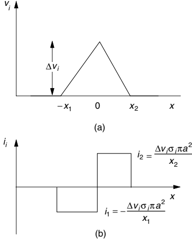
FIGURE 7.4. The action potential is approximated by a triangular wave form. In this piecewise-linear approximation the depolarization and repolarization are both linear. (a) The interior potential. (b) The interior current.
