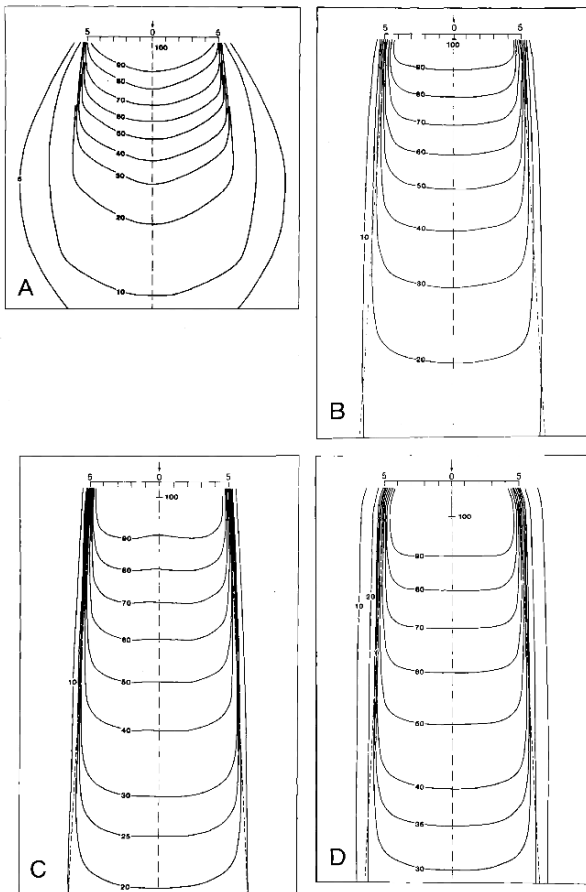
FIGURE 16.46. Isodose distributions for radiation under different conditions, all collimated to 10 cm \times 10 cm. (A) Radiation from an x-ray tube with 200 kVp, 0.5 m from the surface. (B) Photons from the radioactive isotope ^{60}\text{Co} , 0.8 m from the surface. (C) 4-MV photons, 1 m from the surface. (D) 10-MV photons, 1 m from the surface. From F. M. Khan, The Physics of Radiation Therapy , 3rd. ed. p. 204. Philadelphia, Lippincott Williams & Wilkins. ©2003 Lippincott Williams & Wilkins.
