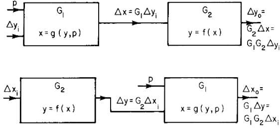
FIGURE 10.6. The open loop gain is calculated by opening the loop at any point. (a) Loop opened in y . (b) Loop opened in x .
