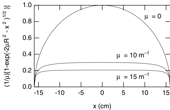
FIGURE 17.25. Plot of the projection including attenuation, Eq. 17.64, for \mu = 0 , \mu = 10 \text{ m}^{-1} (corresponding to 511-keV annihilation radiation) and \mu = 15 \text{ m}^{-1} (corresponding to the photons from ^{99m}\text{Tc} ). The radius of the circle is 16 cm.
