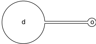
FIGURE 8.28. A superconducting loop shaped as shown becomes a flux transporter. Because the total flux in the loop is constant, a change of flux in the detecting loop d is accompanied by an equal and opposite flux change in the output loop o . The diameter of the output loop is matched to the size of the SQUID. Sensitivity is increased because the detecting loop has a larger area.
