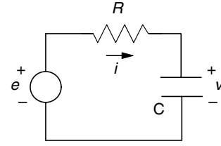
FIGURE 11.44. The circuit for analyzing the noise produced by a resistance R connected to capacitance C . The circuit assumes that the noise is generated in a voltage source e(t) in series with the resistance. The voltage across the capacitance is v .
