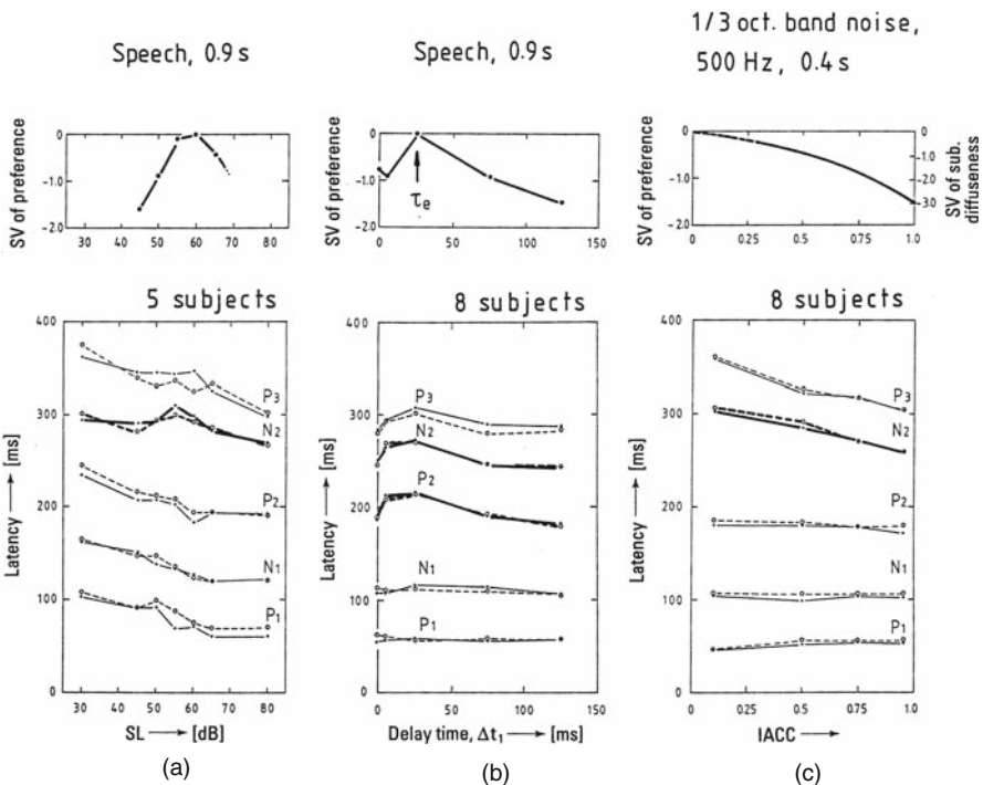
Fig. 4.14 Relationships between averaged latencies of SVR and subjective preference for three factors of the sound field. (—): Left hemisphere. (---): Right hemisphere. (a) As a function of the SL. (b) As a function of the delay time of reflection, \Delta t_1 . (c) As a function of the IACC
