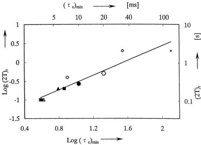
Fig. 5.4 Relationship between the temporal integration window (2T)_r and the minimum value of the effective duration (\tau_e)_{\min} of the running ACF. Different symbols signify experimental results using different sound sources
