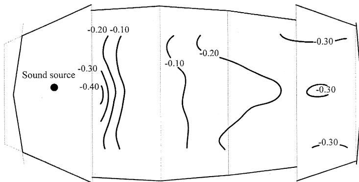
Fig. 8.9 Contour lines of equal \bar{S}_1 listening level preference values calculated for the geometry shown in Fig. 8.8
