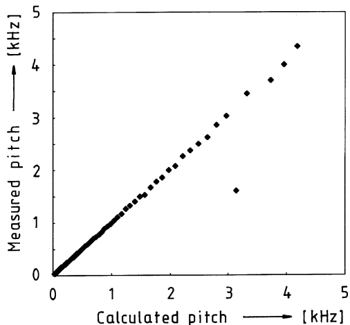
Fig. 8.2 Relationship between calculated and measured pitches obtained by the value of \tau_1 extracted from the ACF of source signals from a “tuned” piano
