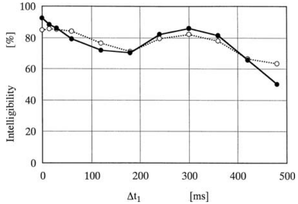
Fig. 9.5 Mean values of calculated and tested intelligibilities for all syllables used
