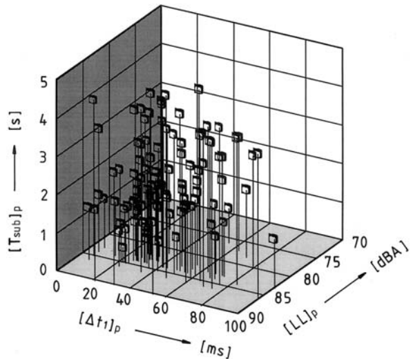
Fig. 8.23 Three-dimensional illustration of preferred factors, [LL]_p , [\Delta t_1]_p , and [T_{sub}]_p of the sound field for each individual subject. Preferred condition for the factor of IACC is excluded, because no fundamental individual differences could be observed. Preferred conditions are distributed in a certain range of each factor, such that subjects could not be grouped into any natural classes
