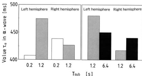
Fig. 4.18 Averaged effective durations \tau_e of EEG alpha rhythms in response to a change of later reverberation time T_{sub} for two pairs of reverberation conditions (0.2 and 1.2 s) and (1.2 and 6.4 s). The preferred condition for late reverberation time is 1.2 s. Data from 10 subjects
