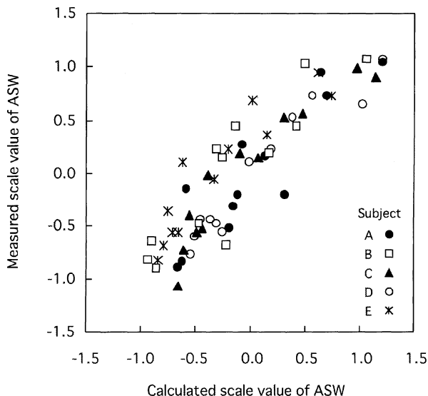
Fig. 7.10 Relationship between the measured individual scale values of apparent source width (ASW) and the scale values of ASW calculated by Equation (7.5) for each individual. Correlation coefficient r = 0.90 ( p < 0.01 ). Different symbols indicate data obtained by different individual subjects
