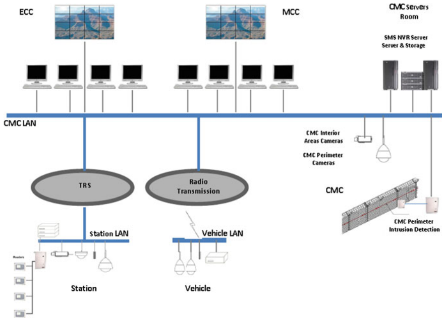
Fig. 4 ISS architecture
