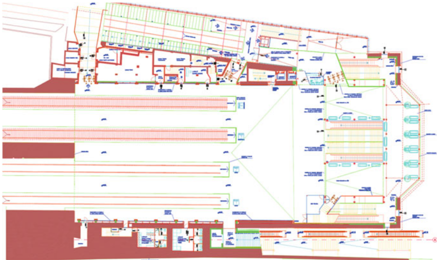
Fig. 4 Montesanto railway station layout after restyling
