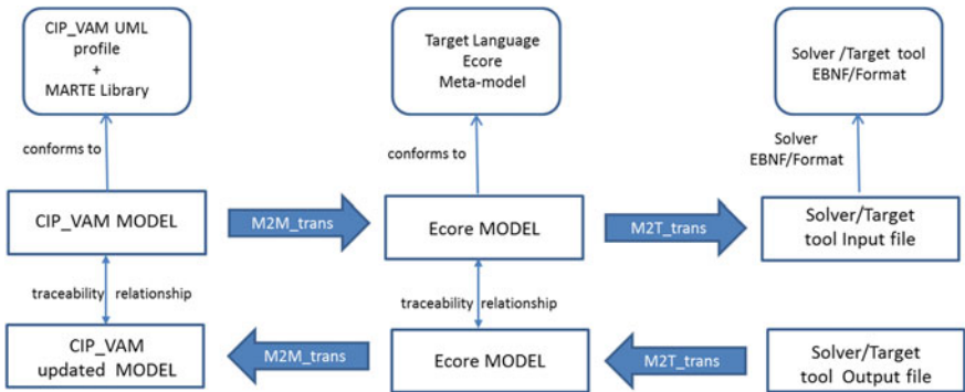
Fig. 5 Forward and backward transformations
