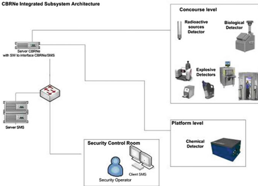
Fig. 4 CBRNE general architecture
