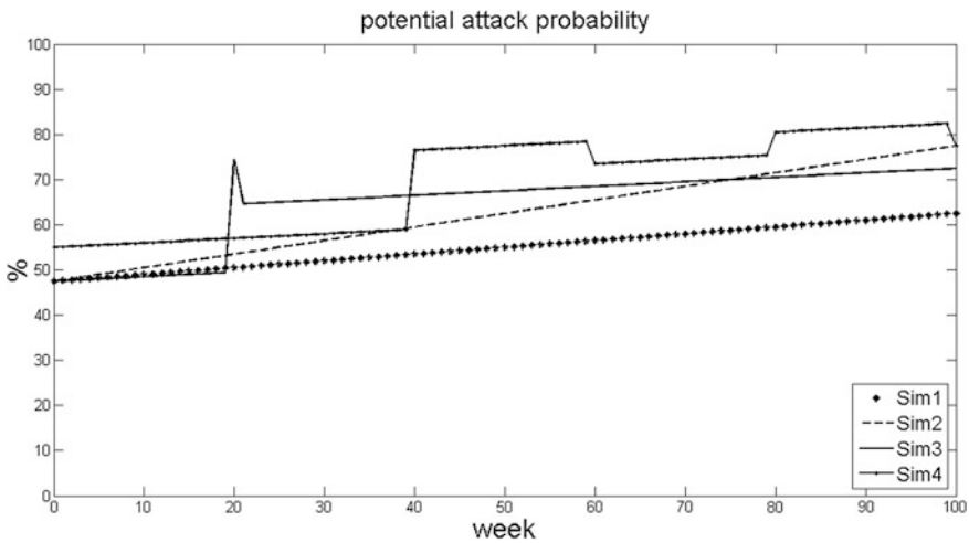
Fig. 9 Potential attack probability—results for the first simulation set for a medium size station. It changes accordingly to the asset vulnerability, asset attractiveness and the motivation for committing crime
