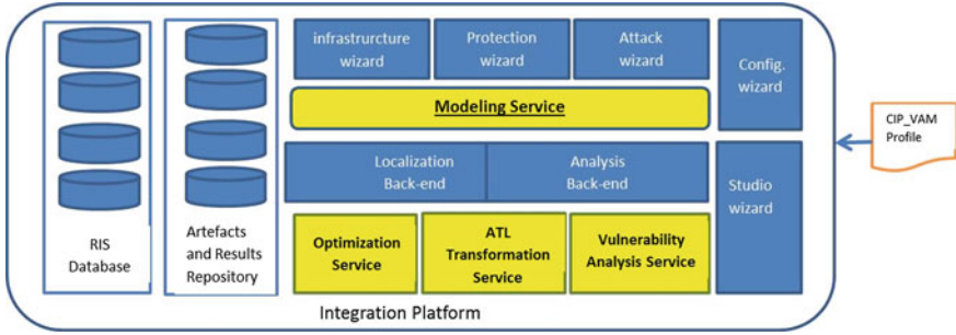
Fig. 4 METRIP tool chain
