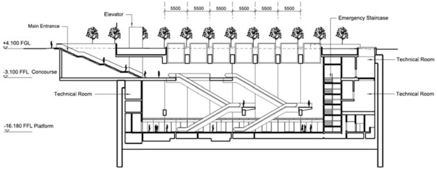
Fig. 2 Cross station of a typical station
