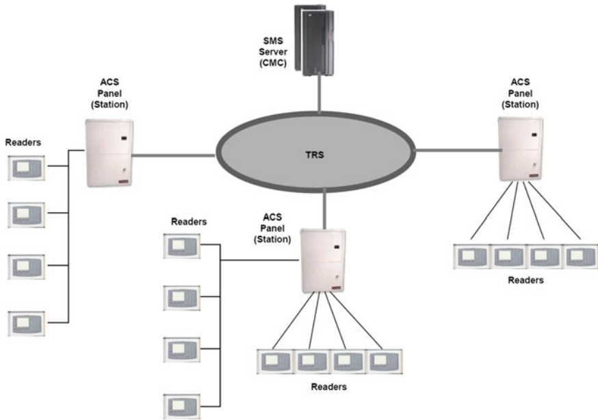
Fig. 6 System architecture
