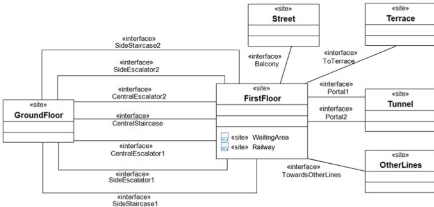
Fig. 14 Class diagram of the station
