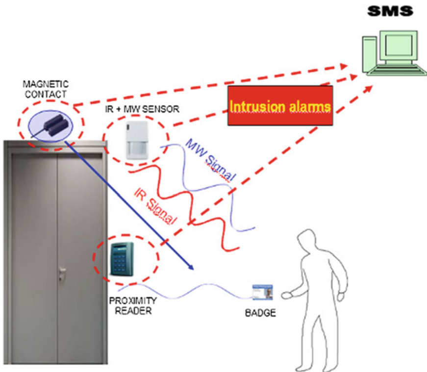
Fig. 2 Example of operation of an access control system
