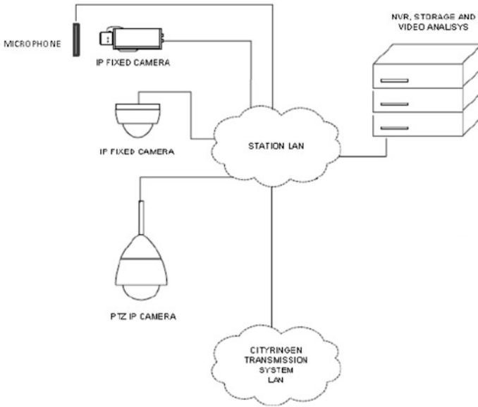
Fig. 7 System architecture—station
