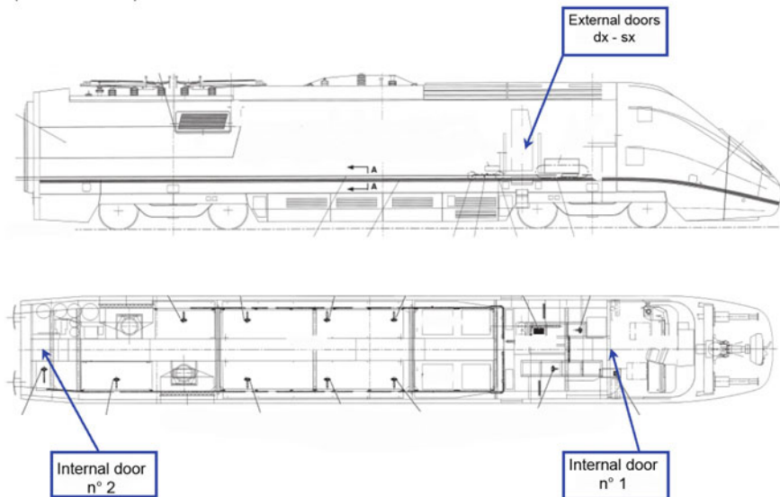
Fig. 8 Train Entrances
