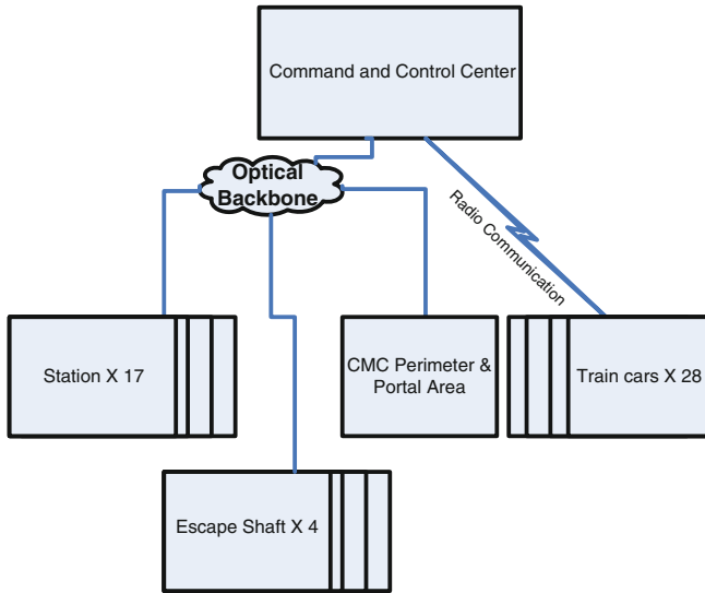
Fig. 5 CCTV system architecture
