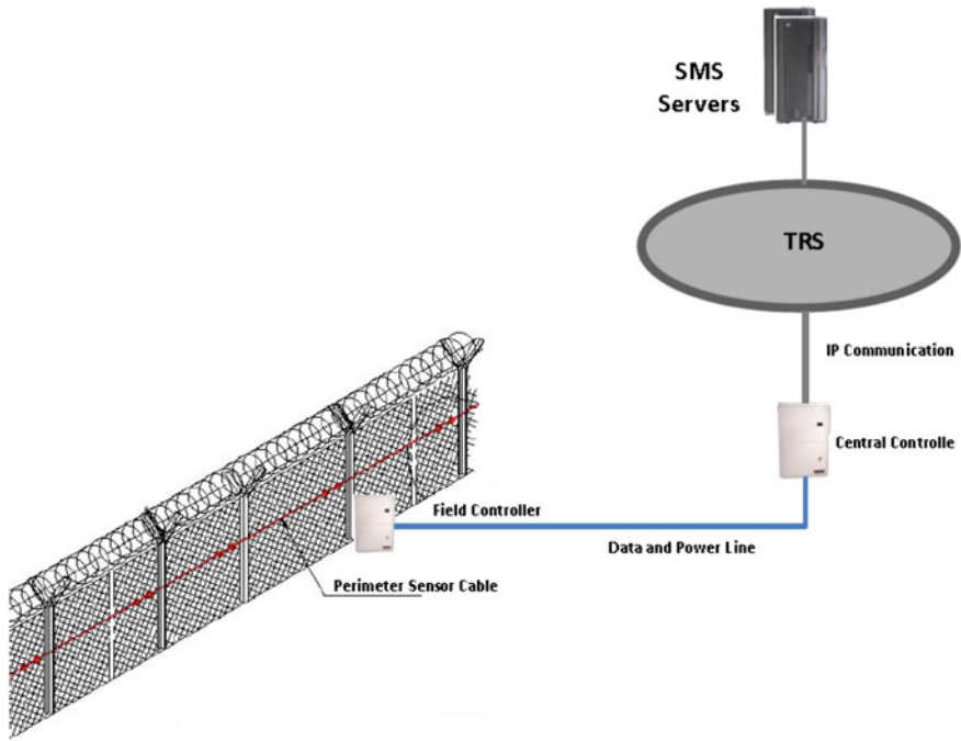
Fig. 8 Perimeter intrusion detection
