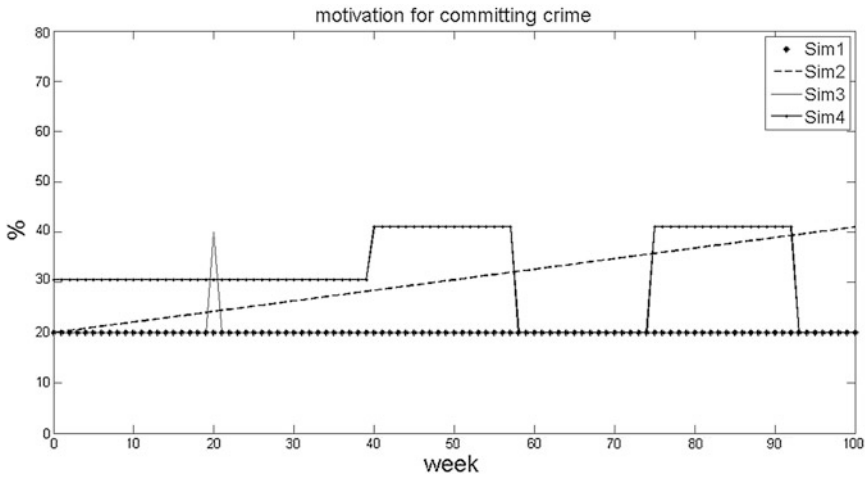
Fig. 7 Motivation for committing crime—results for the first simulation set for a medium size station. In Sim1 we assumed constant attacker’s triggers and motivation is settled at 20 %. Changing the trigger factors, we simulated an increasing trend (Sim2) and very quick changes in the attackers’ motivation (Sim3 and Sim4)
