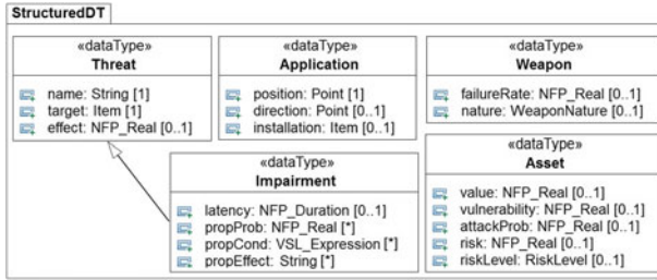
Fig. 9 StructuredDT package
