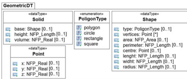
Fig. 8 GeometricDT package
