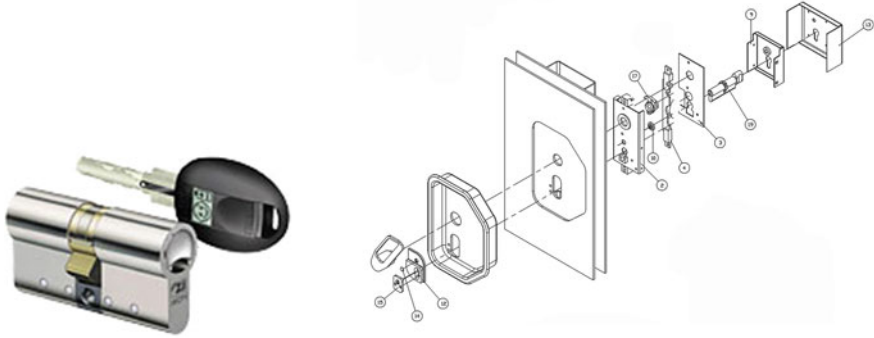
Fig. 7 Mechatronic key
