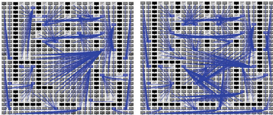
Fig. 17 MCM solutions using 31 and 39 cameras (8 + 12 orientations)
