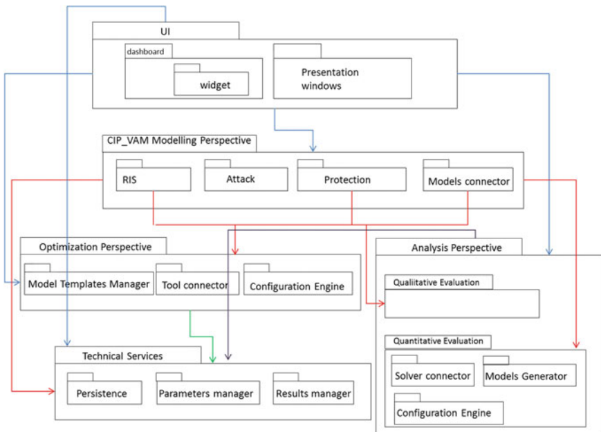
Fig. 2 Tool-chain logical architecture
