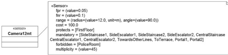
Fig. 19 12-meters camera
