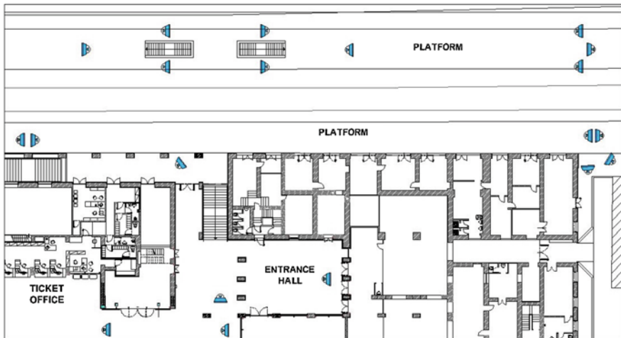
Fig. 5 Example of a station CCTV system draft
