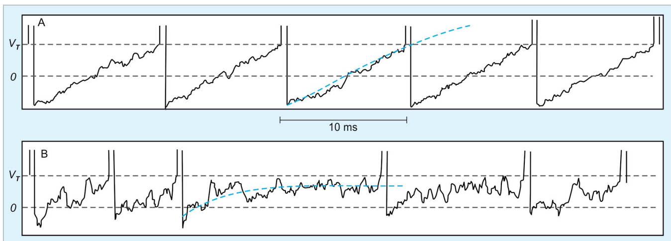
Fig. 4.13: Mathematical modeling of differences in afferent discharge regularity. Time- but not voltage-dependent potassium conductance leads to afterhyperpolarization in afferent terminals. This stochastic model demonstrates that two factors, the post spike voltage trajectory (dotted line in B) and synaptic noise, are relevant in determining discharge regularity. Horizontal dashed lines are the resting potential ( 0 ) and critical firing level ( V_T ).
