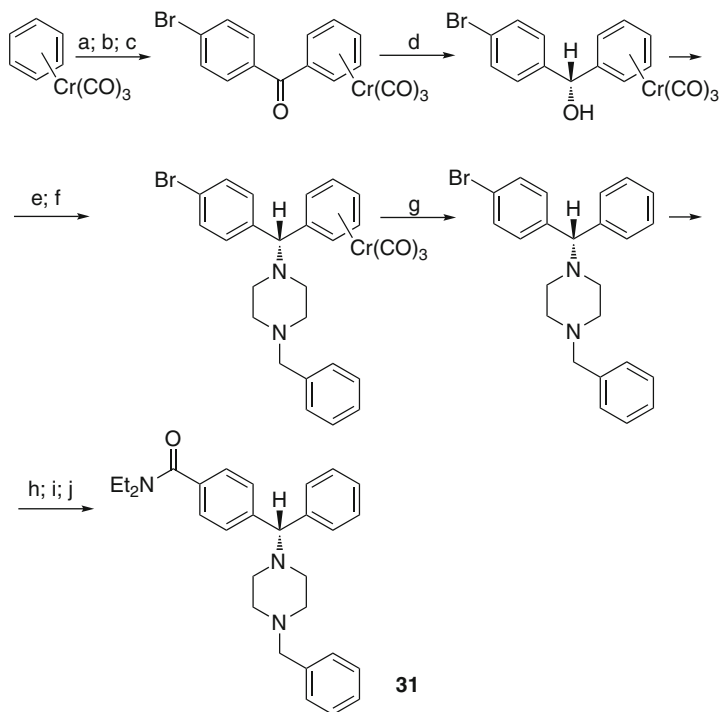
Scheme 2 Reagents. (a) n -BuLi, TMEDA, THF, -78 °C; (b) CuBr·Me 2 S, THF, -78 °C; (c) p -BrC 6 H 5 COCl (74%); (d) , catecholborane, toluene, -78 °C to -40 °C (91%); (e) HBF 4 ·OEt 2 , CH 2 Cl 2 , -60 °C; (f) N -Benzylpiperazine, CH 2 Cl 2 (75%); (g) (NH 4 ) 2 Ce(NO 3 ) 6 , MeOH (95%); (h) n -BuLi, CO 2 , THF, -78 °C; (i) SOCl 2 , CH 2 Cl 2 ; (j) Et 2 NH, CH 2 Cl 2 (34% overall) [44]
