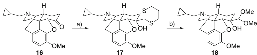
Scheme 4 Acetal exchange reaction of the 14-H compound 16 . Reagents and conditions: (a) n -BuLi, 1,3-dithiane, DME, -70\text{ }^{\circ}\text{C} , 49%; (b) \text{CuCl}_2\cdot 2\text{H}_2\text{O} , CuO, \text{CH}(\text{OMe})_3 , MeOH, 50\text{ }^{\circ}\text{C} , 63%
