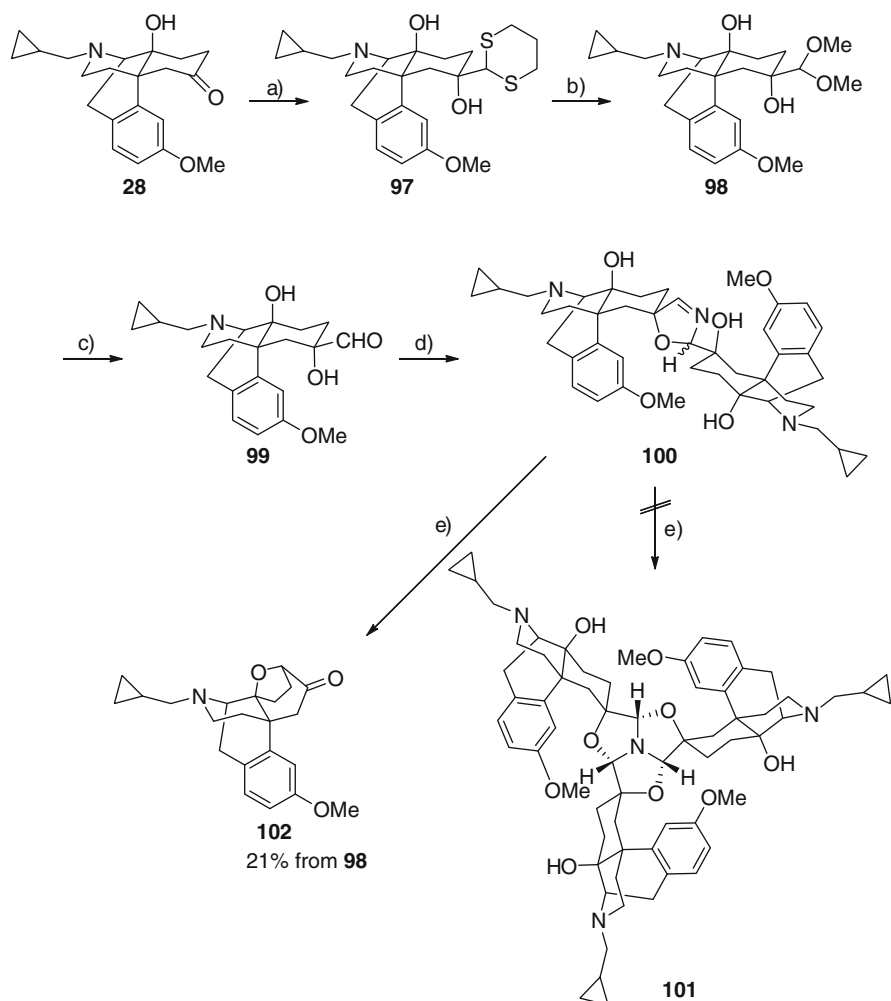
Scheme 32 Synthesis of oxabicyclo[3.2.1]octane derivative 102 . Reagents and conditions: (a) n -BuLi, 1,3-dithiane, DME, -70^{\circ}\text{C} , 69%; (b) \text{CuCl}_2 \cdot 2\text{H}_2\text{O} , CSA, \text{CH}(\text{OMe})_3 , MeOH, 50^{\circ}\text{C} , 37%; (c) 2 M HCl, reflux; (d) \text{NH}_4\text{Cl} , AcONa, MeOH, reflux.; (e) CSA, \text{CHCl}_3 , reflux
