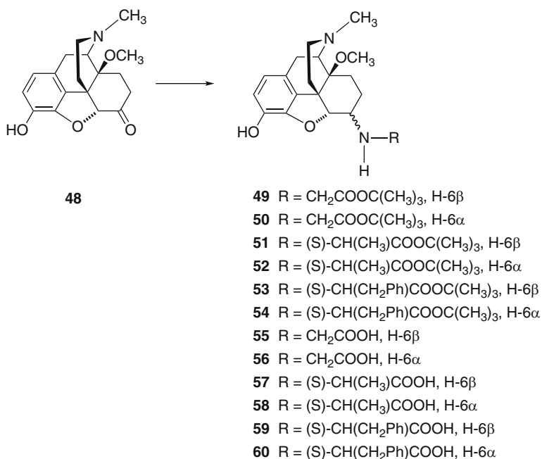
Scheme 12
