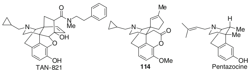
Fig. 23 Structures of TAN-821, rearrangement product 114 , and pentazocine
