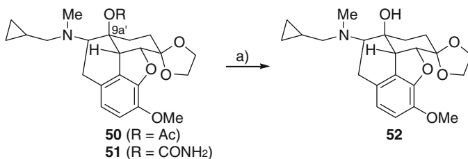
Scheme 22 Hydrolysis of 9a'-acetate 50 and 9a'-carbamate 51 . Reagents and conditions: (a) \text{K}_2\text{CO}_3 , \text{MeOH}/\text{H}_2\text{O} , 80^\circ\text{C} , quant. from 50 , 69% from 51
