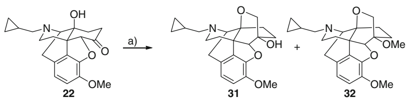
Scheme 12 Reaction of naltrexone methyl ether ( 22 ) with unstable sulfur ylide to afford 31 and 32 . Reagents and conditions: (a) trimethylsulfonium iodide, NaH, THF-DMSO, 0 °C, 31 : 62%, 32 : 26%
