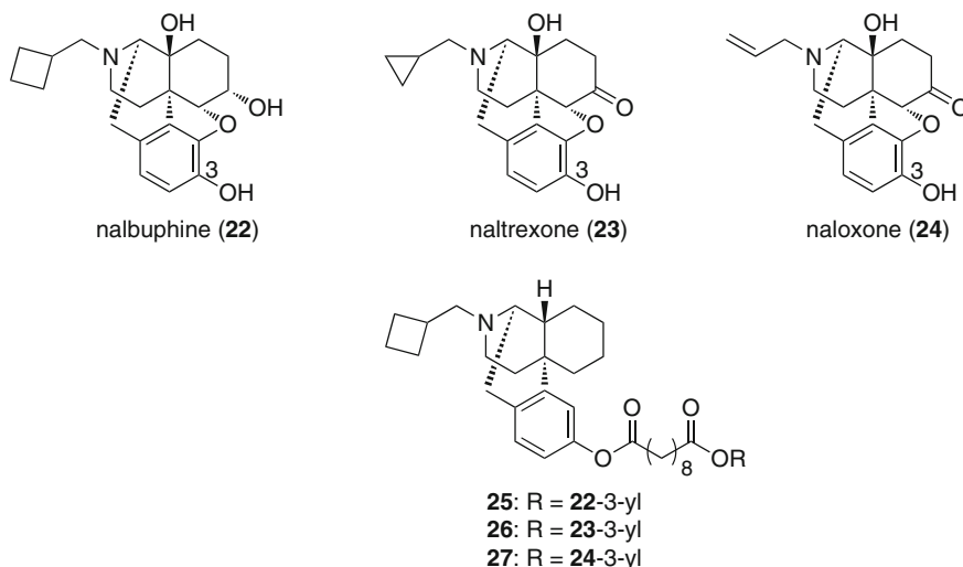
Fig. 7 Structures of nalbuphine ( 22 ), naltrexone ( 23 ), naloxone ( 24 ), and twin drugs 25–27
