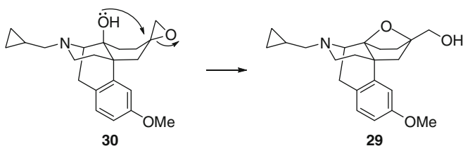
Scheme 10 Intramolecular cyclization reaction of epoxide 30 to produce 29
