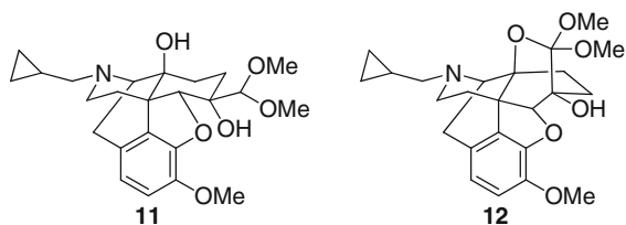
Fig. 5 Structures of acetal 11 and ortho ester 12
