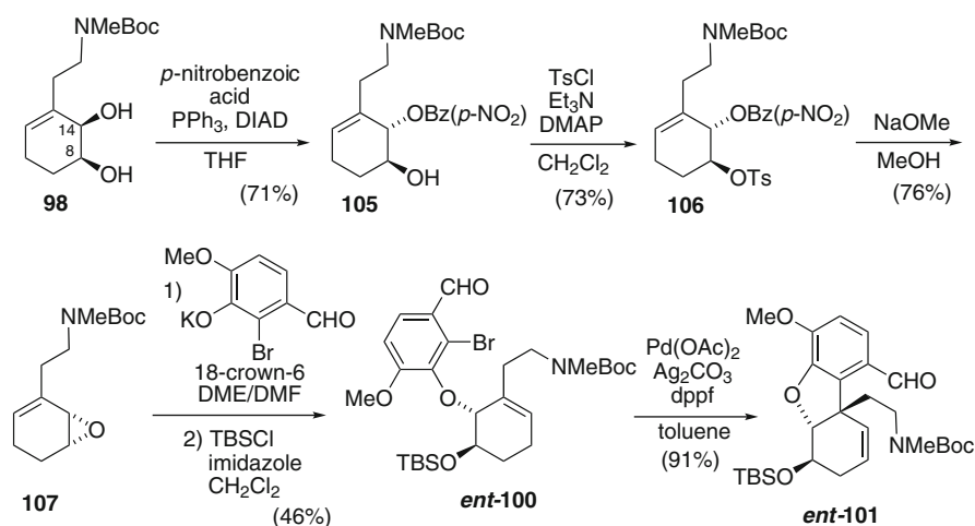
Scheme 21 Preparation of A–C–E ring of (–)-codeine
