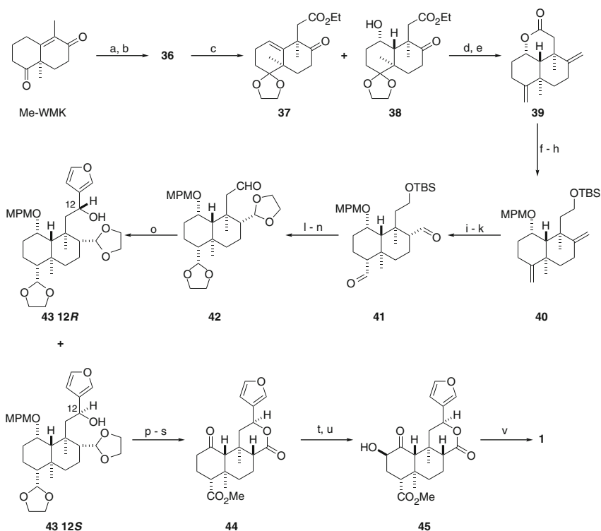
Scheme 4 (a) (\text{CH}_2)_2(\text{OTMS})_2 , \text{Me}_3\text{SiOTf} , 15 Kbar, 40^\circ\text{C} ; (b) \text{KOH} , \text{MeOH}/\text{H}_2\text{O} , \text{O}_2 , 65^\circ\text{C} ; (c) \text{Li}/\text{NH}_3 , \text{THF} , -78^\circ\text{C} , alkyl iodide; (d) 3\text{M HCl} aqueous \text{EtOH} ; (e) \text{NaHMDS} , \text{Ph}_3\text{PCH}_2\text{Br} , \text{THF} ; (f) \text{LAH} , \text{Et}_2\text{O} , 0^\circ\text{C} ; (g) \text{TBSCl} , \text{DMAP} , \text{Et}_3\text{N} , \text{CH}_2\text{Cl}_2 (h) \text{NaH} , \text{MPMCl} , \text{DMF} ; (i) \text{BH}_3 , \text{THF} , 3\text{M NaOH} , \text{H}_2\text{O}_2 ; (j) \text{PDC} , \text{NaOAc} , \text{MS-4 \AA} , \text{CH}_2\text{Cl}_2 ; (k) \text{NaOMe} , \text{MeOH} ; (l) ethylene glycol, \text{PTSA} , 40^\circ\text{C} ; (m) \text{TBAF} , \text{THF} ; (n) \text{PDC} , \text{NaOAc} , \text{MS-4 \AA} , \text{CH}_2\text{Cl}_2 ; (o) 3-bromofuran, t\text{-BuLi} , \text{THF} , -78^\circ\text{C} ; (p) \text{PTSA} , acetone, \text{H}_2\text{O} , reflux; (q) \text{DDQ} , \text{H}_2\text{O} , \text{CH}_2\text{Cl}_2 , 0^\circ\text{C} ; (r) \text{PDC} , 2-methyl-2-butene, \text{DMF} ; (s) \text{DCC} , \text{DMAP} , \text{MeOH} , \text{CH}_2\text{Cl}_2 ; (t) \text{NaHMDS} , \text{TESCl} , \text{THF} ; (u) m\text{-CPBA} , \text{NaHCO}_3 , toluene, \text{H}_2\text{O} , 0^\circ\text{C} , \text{AcOH} ; (v) \text{PPh}_3 , \text{DIAD} , \text{AcOH} , \text{CH}_2\text{Cl}_2
