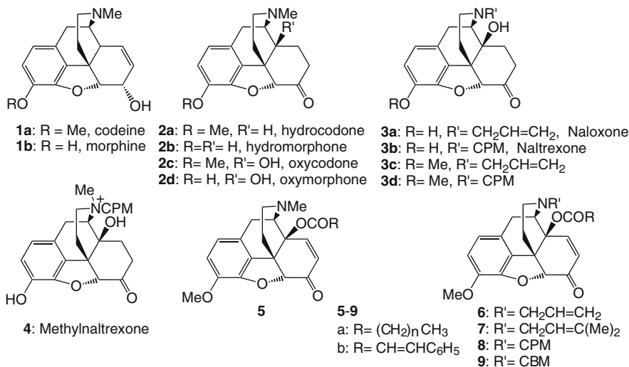
Fig. 1 Oxymorphinans and oxymorphinones
