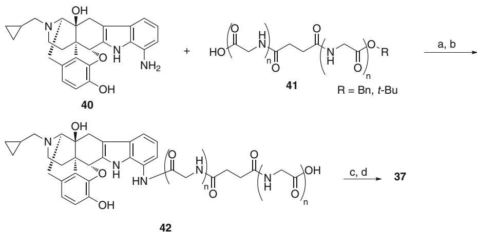
Scheme 4 Synthesis of compounds 37 . Reagents and conditions: (a) DCC, HOBt; (b) 1 M HCl, AcOH, or H 2 (80 psi), Pd/C; (c) 35 , DCC, HOBt; (d) H 2 (85 psi), Pd/C
