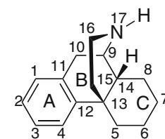
(-)-Morphinan
