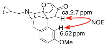
Scheme 32 Synthesis of oxabicyclo[3.2.1]octane derivative 102 . Reagents and conditions: (a) n -BuLi, 1,3-dithiane, DME, -70^{\circ}\text{C} , 69%; (b) \text{CuCl}_2 \cdot 2\text{H}_2\text{O} , CSA, \text{CH}(\text{OMe})_3 , MeOH, 50^{\circ}\text{C} , 37%; (c) 2 M HCl, reflux; (d) \text{NH}_4\text{Cl} , AcONa, MeOH, reflux.; (e) CSA, \text{CHCl}_3 , reflux
