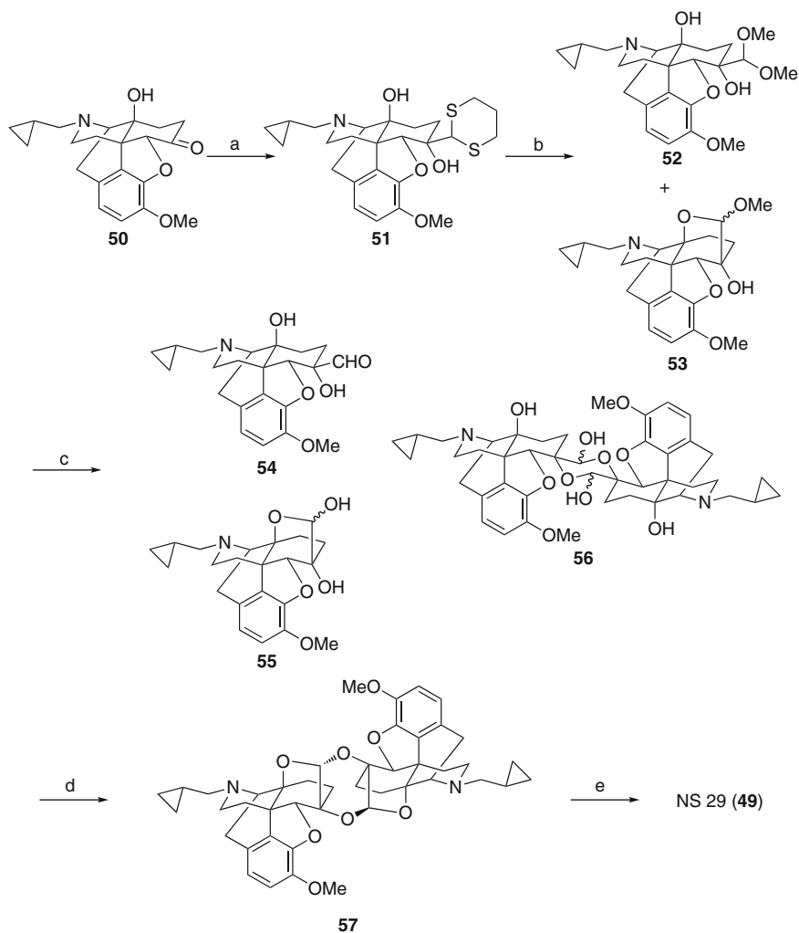
Scheme 5 Synthesis of NS 29 ( 49 ). Reagents and conditions: (a) 1,3-dithian, n -BuLi, THF, -70\text{ }^\circ\text{C} to -60 \sim -40\text{ }^\circ\text{C} , 85%; (b) \text{CH}(\text{OMe})_3 , \text{CuCl}_2/\text{CSA} , MeOH, 50\text{ }^\circ\text{C} , 52 : 65%, 53 : 18%; (c) 1 M HCl, reflux; (d) CSA, toluene, reflux, 23%; (e) t -BuOK, n -PrSH, DMF, 150\text{ }^\circ\text{C} , 82%
