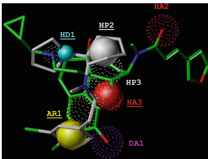
Fig. 23 Superimposition of U-50488H (arylac etamide) on TRK-820 (morphinan) and their 3D-pharmacophores. TRK-820 is shown in green , and U-50488H is shown in white . The 3D-pharmacophores of TRK-820 and U-50488H are represented by dotted and solid spheres , respectively. Matched spheres are indicated by underlined labels
