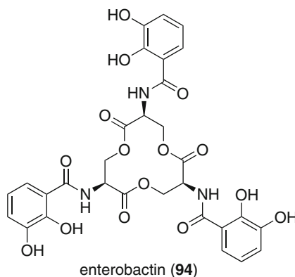
Fig. 18 Structures of valinomycin ( 93 ) and enterobactin ( 94 )
