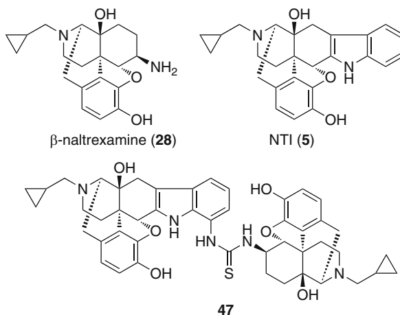
Fig. 12 Structures of β-naltrexamine ( 28 ), NTI ( 5 ), and twin drug 47
