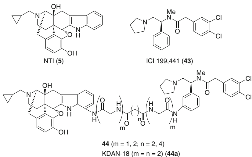
Fig. 10 Structures of NTI ( 5 ), ICI 199,441 ( 43 ), and KDAN twin drugs 44
