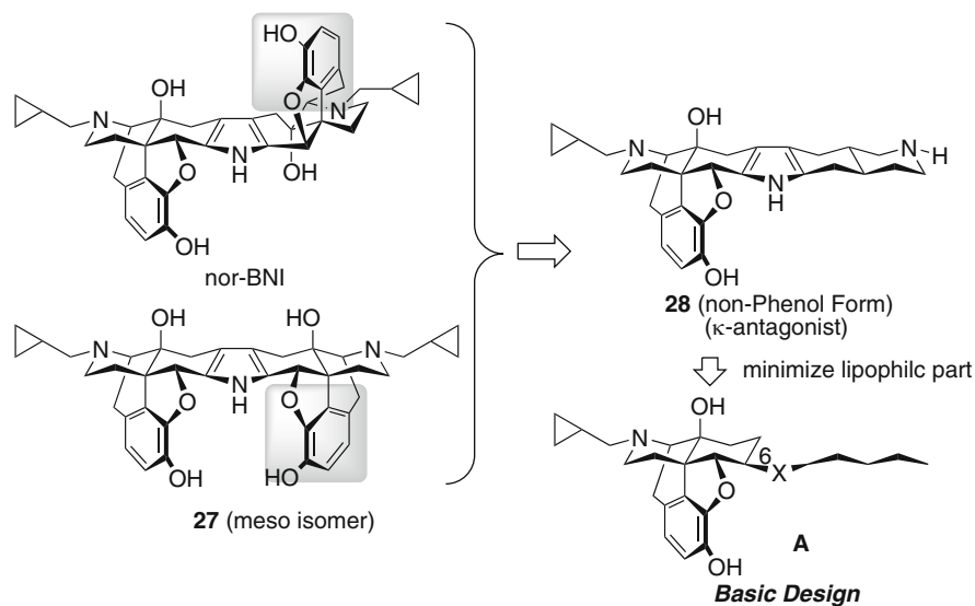
Fig. 14 Basic design of a new chemical class opioid \kappa agonist. Reprinted from [28] with permission from Elsevier. Copyright (2008)
