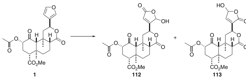
Scheme 18 Photooxidation in the presence of light
