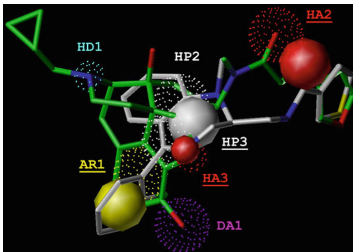
Fig. 26 Superimposition of tiftuadom (benzodiazepine) on TRK-820 (morphinan) and their 3D-pharmacophores. TRK-820 is shown in green , and tiftuadom is shown in white . The 3D-pharmacophores of TRK-820 and tiftuadom are represented by dotted and solid spheres , respectively. Matched spheres are indicated by underlined labels
