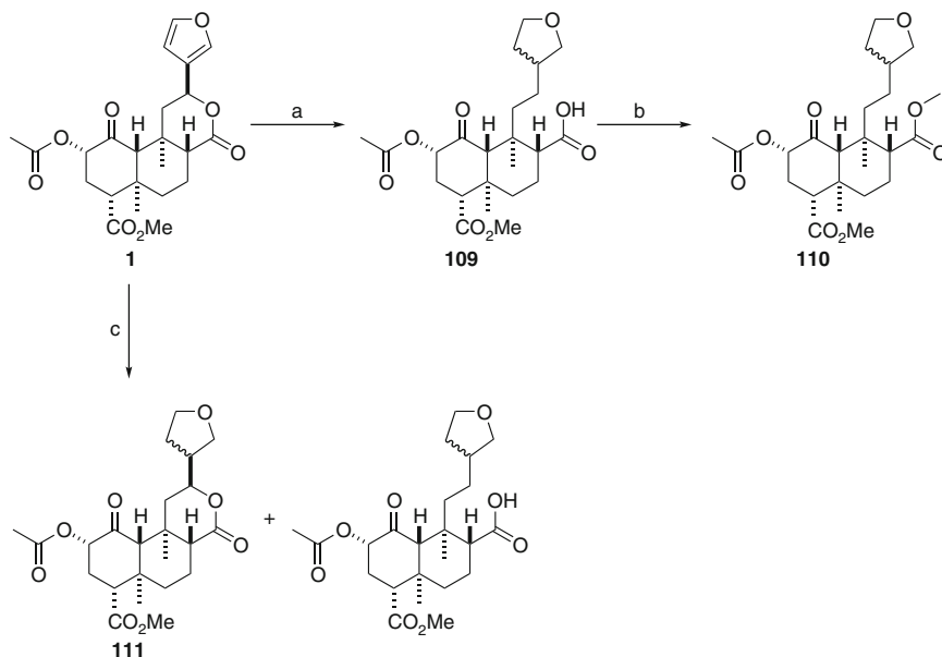
Scheme 17 (a) \text{H}_2 , Pd/C, MeOH; (b) \text{CH}_2\text{N}_2/\text{MeOH} , 0 °C; (c) \text{H}_2 , Rh/C, \text{CH}_2\text{Cl}_2/\text{MeOH}
