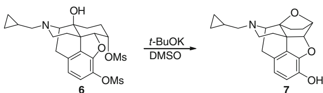
Scheme 2 Intramolecular S_N2 reaction between the 14-OH group and the 6 \alpha -mesylate of naltrexone derivative 6
