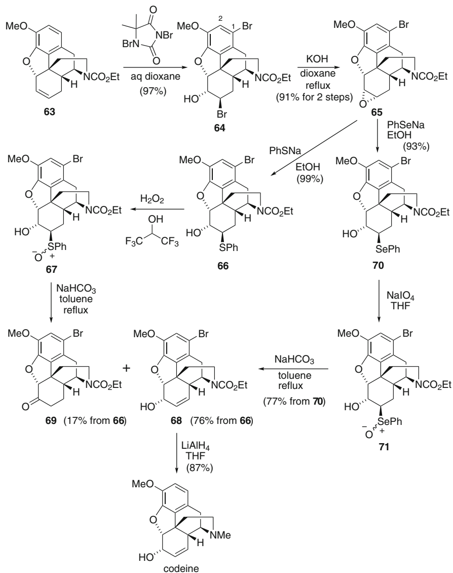
Scheme 14 Synthesis of codeine by Magnus
