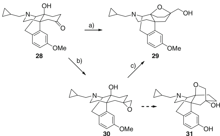
Scheme 9 Reaction of morphinan 28 with stable sulfur ylide to produce oxabicyclo[2.2.1]heptane derivative 29 . Reagents and conditions: (a) trimethylsulfoxonium iodide, NaH, THF, 55 °C, 80%; (b) trimethylsulfoxonium iodide, NaH, THF, rt; (c) NaH, DMF 80 °C, 61%
