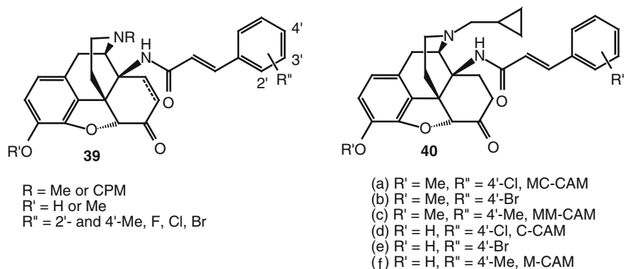
Fig. 3 14-Cinnamoylamino analogues
