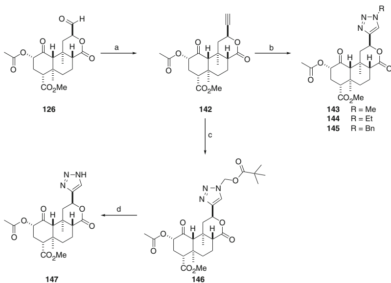
Scheme 23 (a) Ohira-Bestmann reagent; (b) \text{RN}_3\text{CuSO}_4 (cat.), sodium asorbate, t -BuOH/ \text{H}_2\text{O} ; (c) azidomethyl pivalate, \text{CuSO}_4 (cat.), sodium asorbate, t -BuOH/ \text{H}_2\text{O} ; (d): (1) 1M NaOH (2.2 eq.), MeOH/ \text{H}_2\text{O} , (2) 1M HCl (2.2 eq.), (3) \text{Ac}_2\text{O} , pyridine
