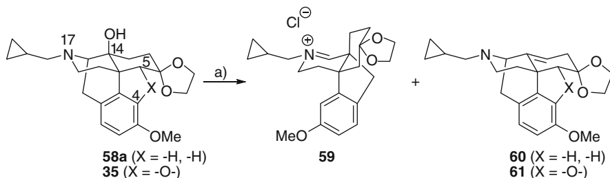
Scheme 25 Dehydration of morphinan 58a and 4,5-epoxymorphinan 35 . Reagents and conditions: (a) \text{SOCl}_2 , py
