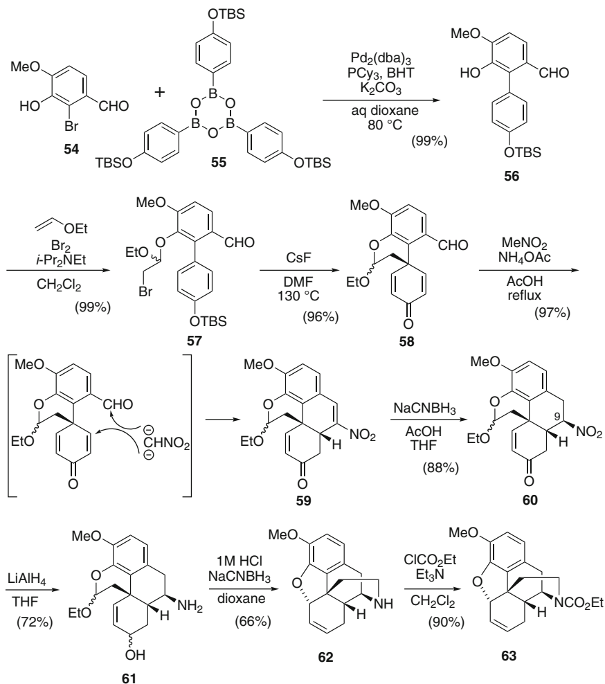
Scheme 13 Synthesis of a tetracyclic core of morphine by the intramolecular \text{S}_{\text{N}}2 reaction
