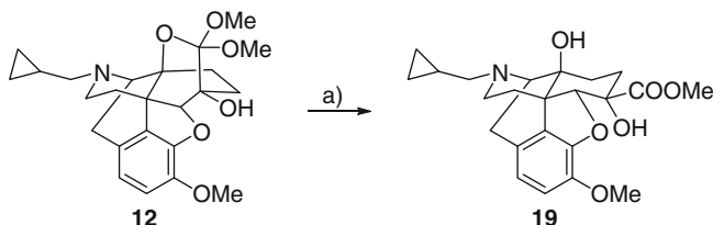
Scheme 5 Hydrolysis reaction of ortho ester 12 . Reagents and conditions: (a) AcOH, 80\text{ }^{\circ}\text{C} , 67%
