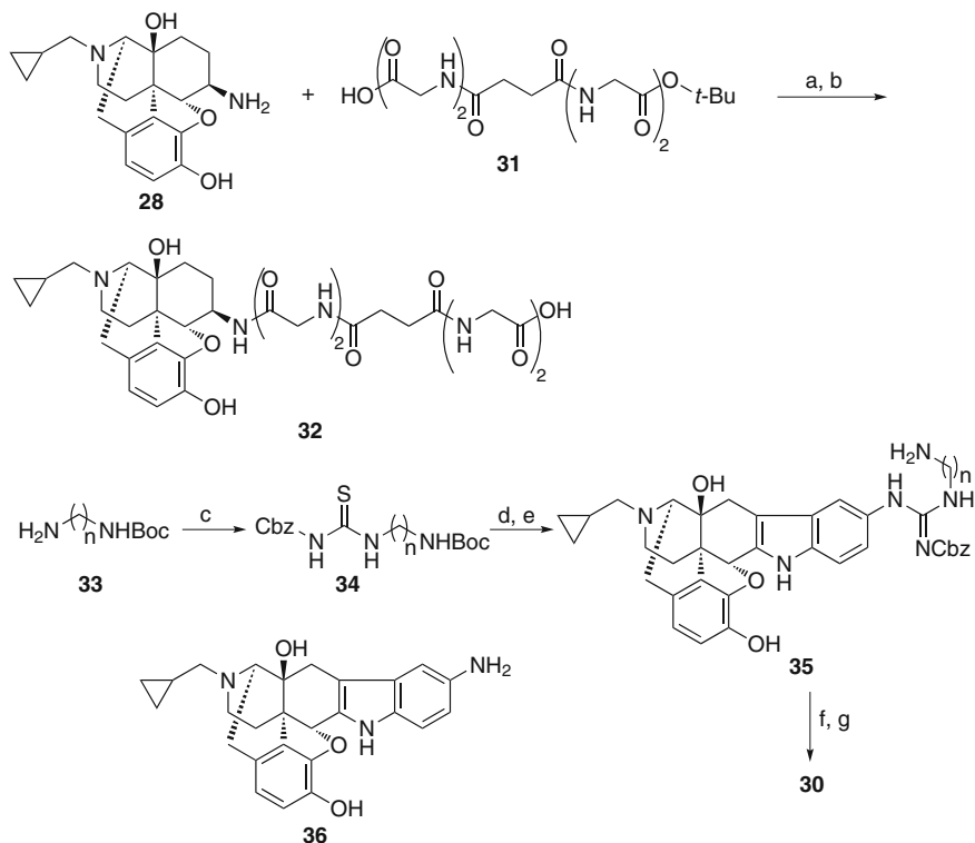
Scheme 3 Synthesis of compounds 30. Reagents and conditions: (a) DCC, HOBT, DMF; (b) TFA, CH 2 Cl 2 ; (c) Cbz-Cl, KSCN; (d) 36, HgCl 2 , Et 3 N; (e) HCl/Et 2 O; (f) 32, DCC, HOBT, DMF; (g) cyclohexadiene, Pd/C
