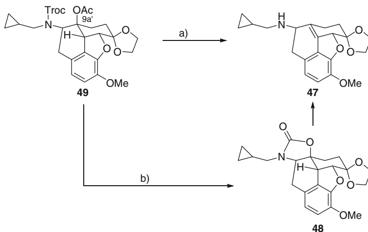
Scheme 20 Elimination reaction of compound 49 . Reagents and conditions: (a) \text{K}_2\text{CO}_3 , MeOH/ \text{H}_2\text{O} , 80^\circ\text{C} , 80%; (b) \text{K}_2\text{CO}_3 , MeOH/ \text{H}_2\text{O} , rt, 94%
