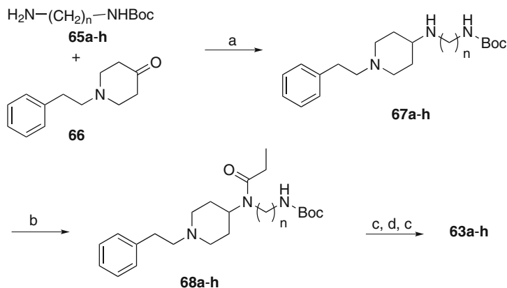
Scheme 6 Synthesis of twin drugs 63 . Reagents and conditions: (a) NaBH 3 CN, MS 3A, MeOH, rt, 50–82%; (b) (EtCO) 2 O, DMAP, py, CH 2 Cl 2 , rt, 53–86%; (c) TFA, CH 2 Cl 2 , 60–99%; (d) BocNH(C=S)NHBoc, HgCl 2 , Et 3 N, CH 2 Cl 2 , rt, 50–95%
