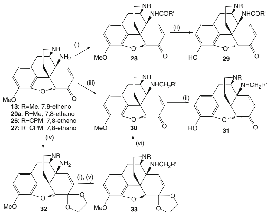
Scheme 5 (i) R'COCl or R'COOCOR' , NEt_3 , 40–90%; (ii) BBr_3 , CH_2Cl_2 , 50–80%; (iii) R'CH_2X (X = halide), NaHCO_3 , 35–80%; (iv) ethylene glycol, HCl , CH_2Cl_2 ; (v) LiAlH_4 , THF, 60%
