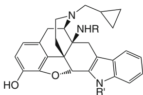
Fig. 13 17-Cyclopropylmethylmorphindole derivatives
