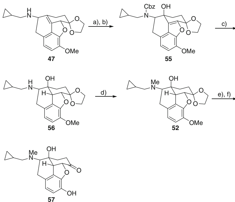
Scheme 24 Synthesis of 15–16 nornaltrexone derivative 57 . Reagents and conditions: (a) Cbz-Cl, proton-sponge, CH 2 Cl 2 , rt; (b) m CPBA, CH 2 Cl 2 , 0 °C, 68% from 47 ; (c) H 2 , 10% Pd/C, MeOH, rt, 69%; (d) (CH 2 O) n , NaBH 3 CN, AcOH, rt, 88%; (e) 2 M HCl, MeOH, reflux, quant.; (f) BBr 3 , CH 2 Cl 2 , rt, 19%
