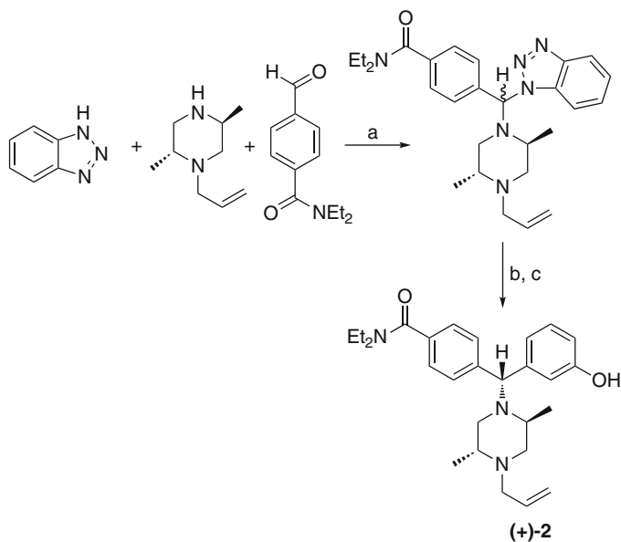
Scheme 1 Reagents. (a) Toluene, 110°C, (-H 2 O); (b) 3-(3- tert -Butylmethylsilyloxy)phenylmagnesium bromide, THF, 25 °C; (c) 3 N HCl [56]
