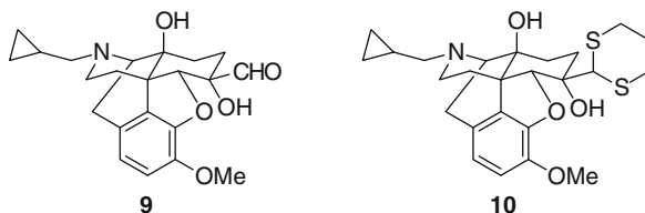
Fig. 4 The structures of \alpha -hydroxyaldehyde 9 and thioacetal 10
