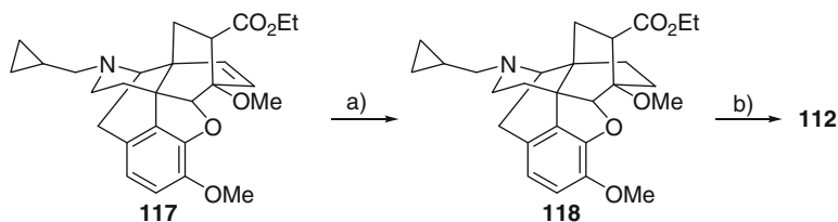
Scheme 38 Preparation of primary alcohol 112 from ester 117 . Reagents and conditions: (a) H 2 (0.4 MPa), Pd/C, EtOH, 50 °C, 93%; (b) LiAlH 4 , THF, 0 °C to rt, 95%
