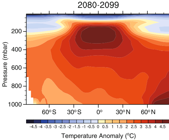
Fig. 2.17 Mean of 21 AOGCM models which were used for the projection of climate change for the Fourth Assessment Report of the Intergovernmental Panel on Climate Change, IPCC (2007) . The zonal average temperature change in the atmosphere over the last 20 years of the twenty-first century for the emission scenario A1B is shown. The troposphere shows a warming, amplified between 7 and 12 km in the tropics, as well as on the surface north of 60°N. The stratosphere shows a cooling. Figure from IPCC (2007) , Chap. 10 (Fig. 10.7, p. 765).
