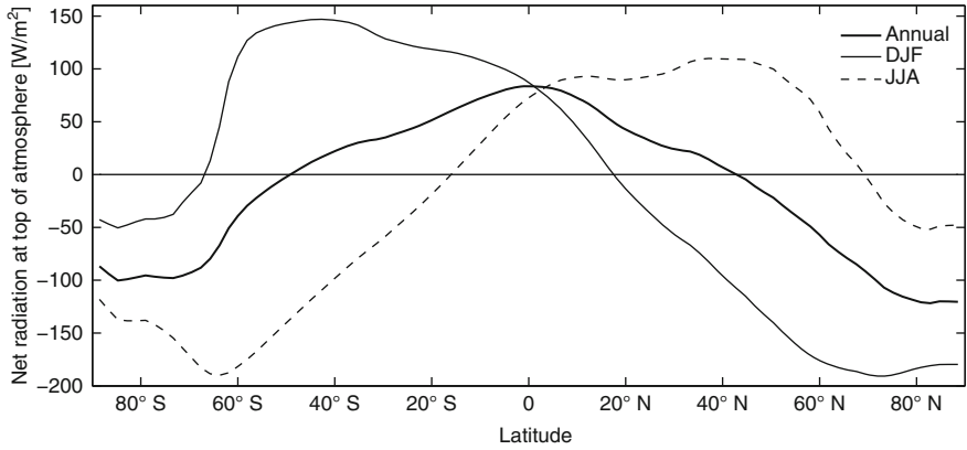
Fig. 4.1 Radiation balance as a function of latitude. Shown are the annual mean as well as the two seasonal means DJF (December-January-February) and JJA (June-July-August). Data from NCEP reanalysis (Saha et al. 2006). Figure constructed by F. Lehner.
