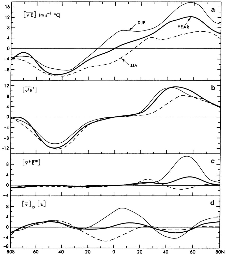
Fig. 4.4 Profile of the zonally and vertically averaged meridional transports of the total energy in (4.1) in ^{\circ}\text{C m s}^{-1} . (a) total; (b) transient eddies; (c) stationary eddies; (d) mean meridional flow, for the annual mean ( bold ), winter ( thin line ) and summer ( dashed ) months. In order to obtain units of PW, the factor (2 \pi R \cos \phi) c_p (p_0/g) has to be multiplied. Figure from Peixoto and Oort (1992).
