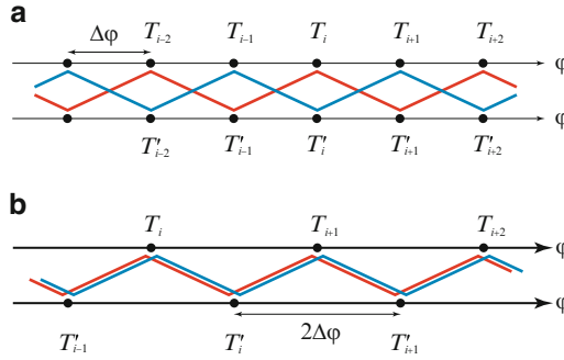
Fig. 6.7 (a) A-grid for the one-dimensional energy balance model. The scheme (6.27) for the solution of (6.26) results in two independent sub-grids ( colored lines ). (b) C-grid for the one-dimensional energy balance model.
