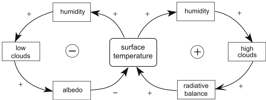
Fig. 2.14 Cloud feedback loops. The sign depends on the location and the quality of clouds. Low clouds affect short-wave radiation via albedo as opposed to high clouds affecting long-wave irradiance.
