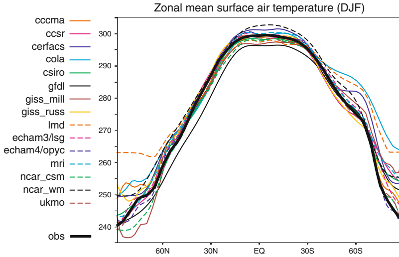
Fig. 2.4 December–February temperatures in Kelvin, zonally averaged for 15 global AOGCMs and comparison with the observed climatology ( black line ). Figure from IPCC (2001) , Chap. 8 (Fig. 8.2, p. 480).
