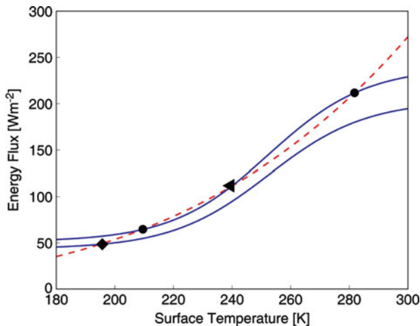
Fig. 9.5 Right-hand ( dashed ) and left-hand sides of (9.6) for S_0 ( upper curve ) and 0.85 S_0 . The temperature dependence of the albedo produces several equilibrium solutions: stable states ( filled circles and diamond ) and an unstable equilibrium state ( triangle ).
