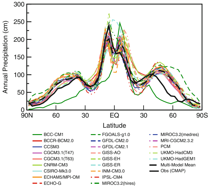
Fig. 2.5 Annual-mean, zonally-averaged precipitation amount simulated by 23 comprehensive coupled climate models used in IPCC (2007) . Observed estimates are shown by the black bold line and they are compared with the multi-model mean ( black dashed ). Figure from IPCC (2007) , Chap. 8, Supplementary Materials (Fig. S8.10, p. SM.8-49).
