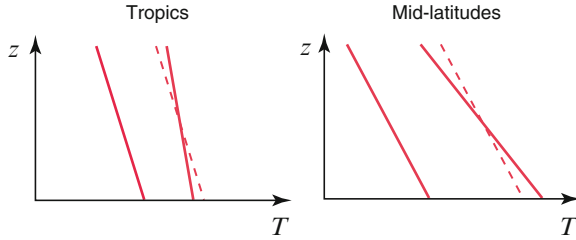
Fig. 2.15 Schematic illustration of changes in the vertical temperature structure in the tropics and in the mid-latitudes. Due to increased convection, the lapse rate decreases in the tropics. In the mid-latitudes the horizontal flow limits the warming to the surface and the lower atmosphere which causes the lapse rate to increase. Compared to the mean warming, a reduced warming of the surface occurs in the tropics (therefore a negative feedback), while it is enhanced in the mid-latitudes (positive feedback).
