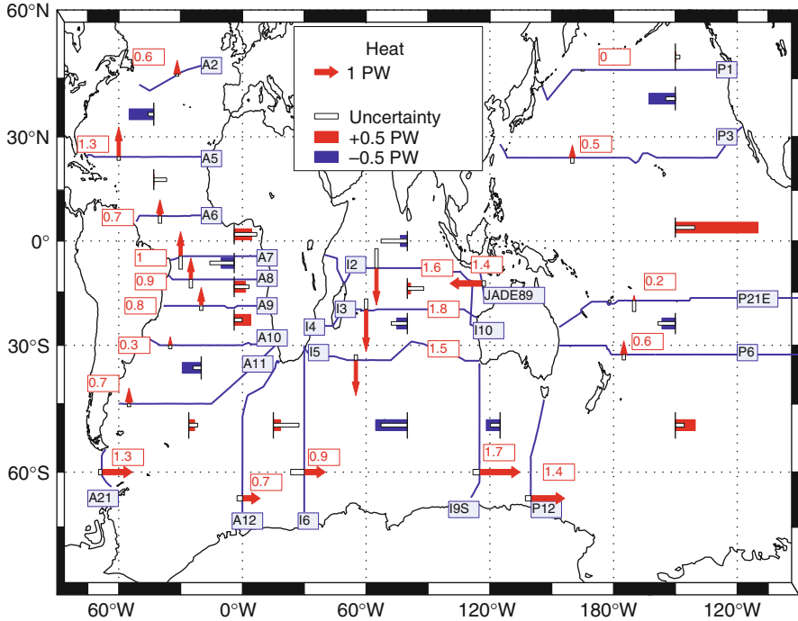
Fig. 4.6 Meridional and vertical heat transports in the different regions of the world ocean. Numbers in boxes denote the meridional transport in PW. Horizontal bars represent the vertical transport (to the left = downwards). Figure from Ganachaud and Wunsch (2000).
