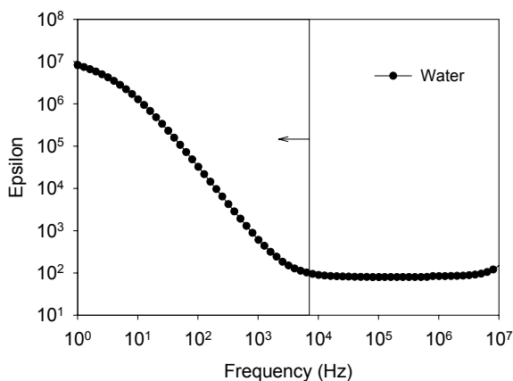
Fig. 4.18. Water calibration. Pure, deionized water (18.0 MΩ/cm) tends to a relative permittivity of \epsilon = \kappa \sim 80 at high frequency in accordance with values well established in the literature. The sharp rise in the lower frequencies (shown by the arrow) illustrates the polarization effect
