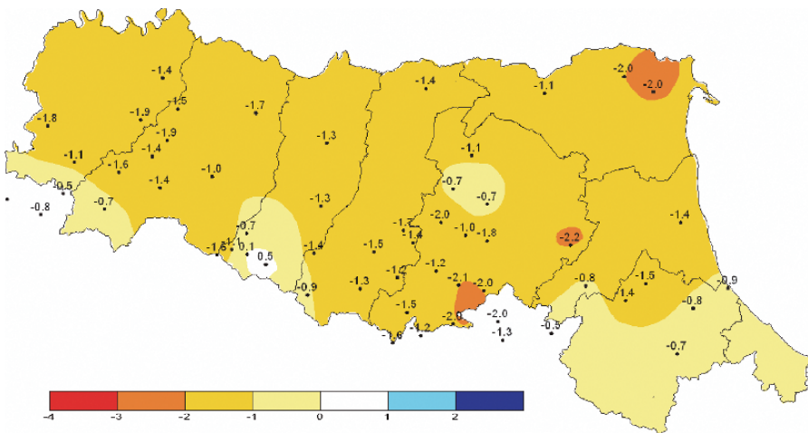
Figure 5. SPI 3-month index for the month of July 2006 calculated using as forecast the 50th percentile of the rainfall distribution function of the month of July
