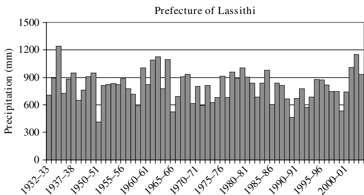
Figure 7. Annual precipitation for Lassithi prefecture (1932–2004)
