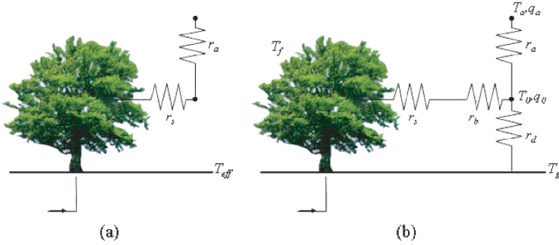
Figure 1. Schematic representation of the main elements of (a) a single-component and (b) a two-component canopy model (modified from Garratt, 1992)
