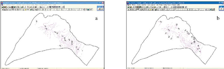
Figure 11. Potentiometric surface from October 1995(a) to March 1996(b)
