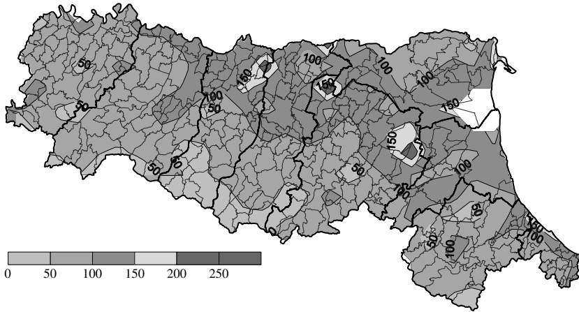
Figure 12. DT180 values (mm) for grassland (Emilia-Romagna; July 20, 2005)
