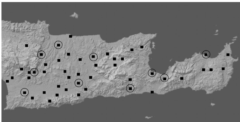
Figure 5. Meteorological stations of the study area (dots indicate availability of precipitation data, circles indicate availability of temperature data)
