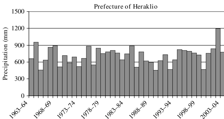
Figure 6. Annual precipitation for Heraklio prefecture (1963–2004)
