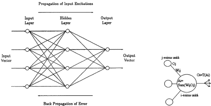
Figure 2. Structure of a Back Propagation Artificial Neural Network
