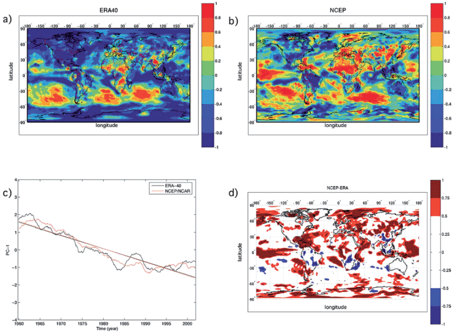
Figure 2. (a) First loading pattern of the SPI-24 for the globe obtained using the ERA-40 data set, contour interval is 0.2; (b) as in (a) but for NCEP/NCAR data set; (c) first PC scores for ERA-40 (black line) and NCEP/NCAR (red line), straight lines denote the fitted linear trends; (d) differences between the first loading of NCEP/NCAR and that of ERA-40, absolute values less than 0.5 are denoted by white colour
