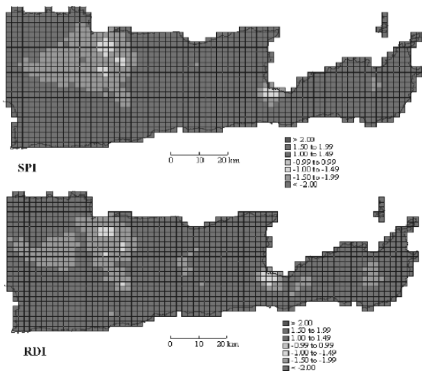
Figure 18. SPI and RDI st for a dry year (1989–90)
