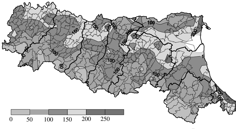
Figure 11. DT180 values (mm) for grassland (Emilia-Romagna; July 20, 2003)
