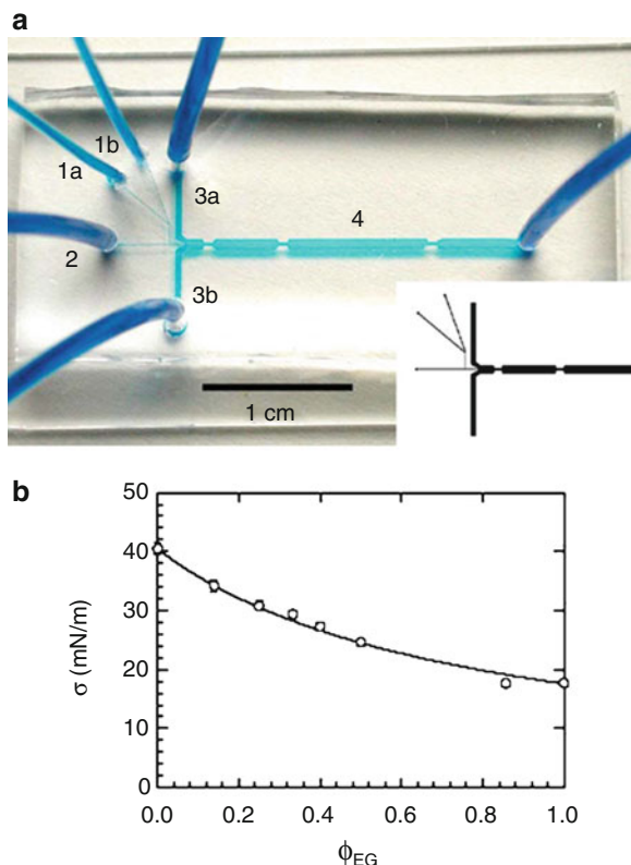
Fig. 23 a Image of a microfluidic chip used for IFT measurements filled with liquid dye to illuminate channels. To perform the measurement, drops (fluid 1a and b) are injected into an immiscible stream (2). Additional immiscible matrix is added (3a and 3b) conveying the drops into channel 4 for analysis and measurement. Constrictions in channel 4 accelerate/stretch the drops. Multiple constrictions enable measurement at different interface age. The channel geometry is shown schematically in the inset (from [108]). b Interfacial tension ( \sigma ) of water/ethylene glycol mixtures (binary drops) in PDMS oil, as a function of composition ( \phi ). (Reproduced with permission from [109])
