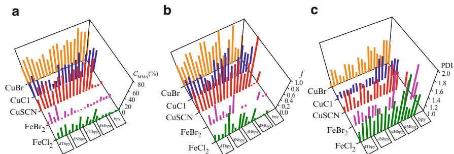
Fig. 2 Effects of metal salts, ligands, and initiators on C_{MMA} (a), f (b), PDIs (c) of the polymers in the atom transfer radical polymerization (ATRP) of methyl methacrylate (MMA) in p -xylene at 90 °C. [MMA]_0:[initiator]_0:[metal\ salt]_0:[ligand]_0 = 150:1:1:2 , MMA/p\text{-xylene} = 1:2\text{ v/v} . EBIB, MBP, BEB, and TsCl were used as initiator from right to left in each ligand column, respectively (Reprinted with permission from [34]. Copyright (2004) John Wiley & Sons, Inc.)
