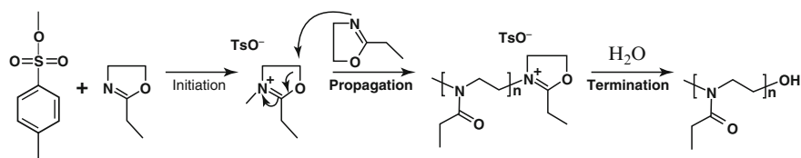
Scheme 6 Schematic representation of the CROP of 2-ethyl-2-oxazoline (EtOx) initiated by the methyl tosylate
