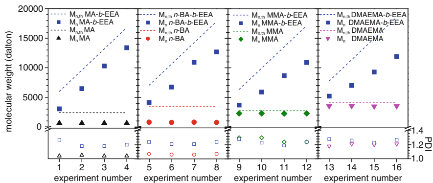
Fig. 15 Number average molar masses ( M_{n,GPC} ) and PDI values obtained for the first blocks and for the final copolymers of PMA, PnBA, PMMA, or PDMAEMA (25 units) with PEEA (25, 50, 75, and 100 units for 100% conversion). All M_{n,GPC} values are calculated against PMMA standards. SEC eluent \text{CHCl}_3:\text{NET}_3:i\text{-PrOH} . (Reprinted with permission from [87]. Copyright (2005) American Chemical Society)
