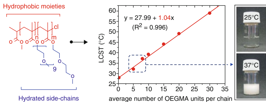
Fig. 11 Plots of the measured lower critical solution temperature (LCST) as a function of the theoretical average number of OEGMA 475 units per chain for a series of P(MeO 2 MA- co -OEGMA 475 ) copolymers of various composition. Hydrophobic and hydrophilic molecular regions on the copolymer are indicated in red and blue , respectively. (Reprinted with permission from [76]. Copyright (2008) John Wiley & Sons, Inc.)
