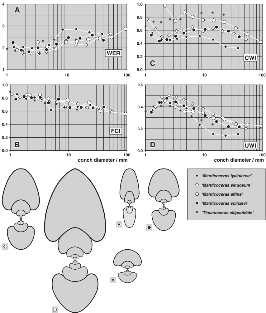
Fig. 3.12. Bivariate diagrams showing the ontogenetic development of the whorl expansion rate (WER; in A), flank convergence index (FCI; in B), conch width index (CWI = w/dm ; in C), and umbilical width index (UWI = uw/dm ; in D) of sectioned specimens of mantiloceratid ammonoids from the Timan, the South Urals, and the Altay Mountains. Cross sections after Bogoslovsky (1969), \times 0.75 .
