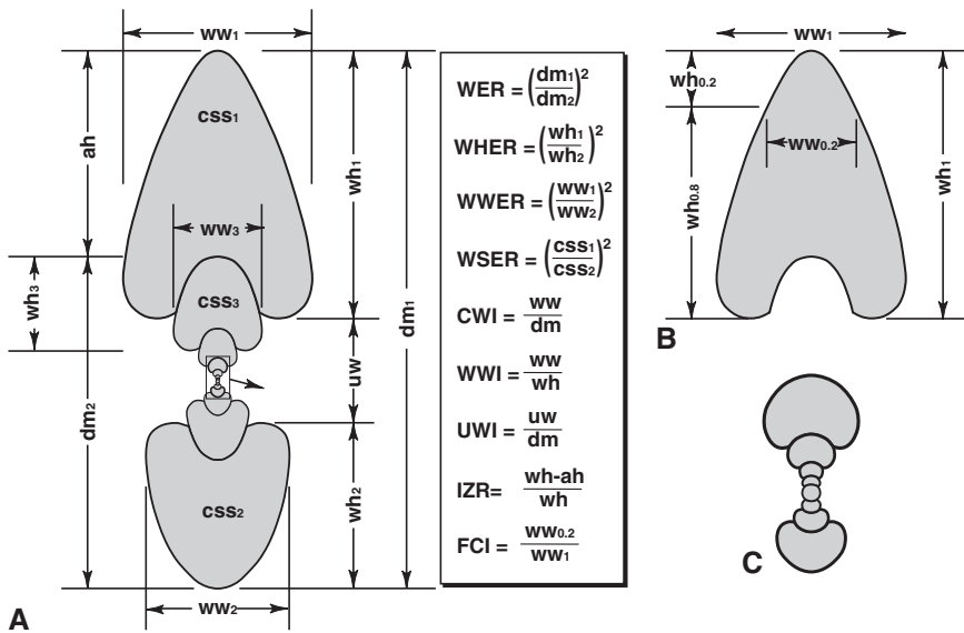
Fig. 3.5 The conch parameters and ratios used in the text. A – conch parameters in a cross section of a Manticoceras specimen ; B – parameters for calculating the flank convergence index (FCI); C – enlarged inner whorls showing the large protoconch (x 3) ( dm = conch diameter; ww = whorl width; wh = whorl height; uw = umbilical width; ah = apertural height; css = cross-section surface; WER = whorl expansion rate; WHER = whorl height expansion rate; WWER = whorl width expansion rate; WSER = whorl surface expansion rate; CWI = conch width index; WWI = whorl width index; UWI = umbilical width index; IZR = imprint zone rate; FCI = flank convergence index).
