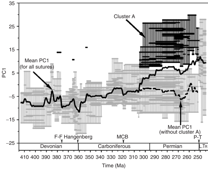
Fig. 8.3 Detailed view of the change in suture morphology through time, using PC1 scores as a proxy. Data are binned into 168 1-my time intervals. Points correspond to the score for each genus and are connected vertically to emphasize total range of values per interval. Black points highlight a statistically distinct cluster of morphologies (A) generated mainly during the Upper Carboniferous–Permian radiation. Comprising taxa belong almost exclusively to three subclasses ( Goniatitina , Prolecanitida , Ceratitida ), with the middle Devonian anarcestid Beloceras [4] being the only notable exception. The solid black line tracks the mean evolutionary trajectory for all sampled taxa. Note how the average runs through unoccupied space during the Permian due to the effect of the outlying Cluster A taxa. The dotted black line tracks the trend after removal of those taxa, emphasizing the morphological stasis that persisted until the P-T extinction.
