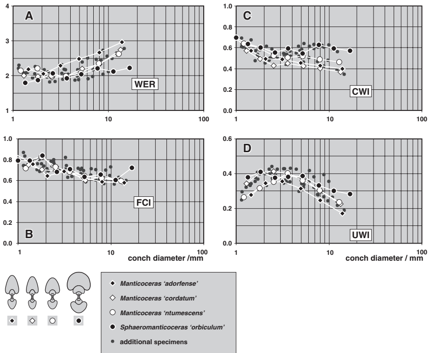
Fig. 3.11 Bivariate diagrams showing the ontogenetic development of the whorl expansion rate (WER; in A), flank convergence index (FCI; in B), conch width index (CWI = w/dm ; in C), and umbilical width index (UWI = uw/dm ; in D) of sectioned specimens of Manticoceras from Büdesheim (Eifel). Cross sections after Clausen (1969), \times 0.75 .
