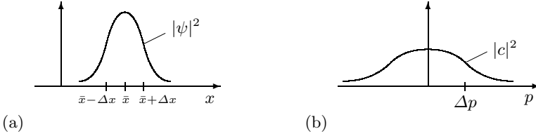
Fig. 12.3. Gaussian distribution
