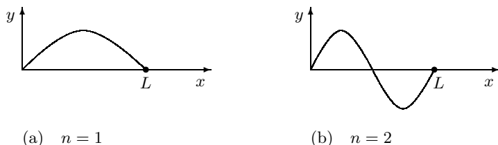
Fig. 2.3. Standing waves
