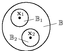
Fig. 5.21. Singularities
