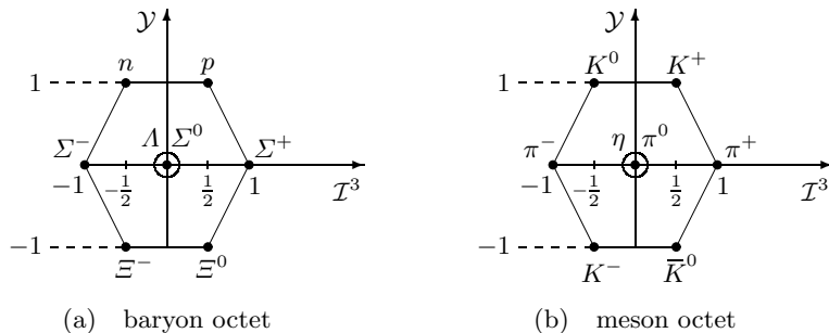
Fig. 2.20. Composed particles
