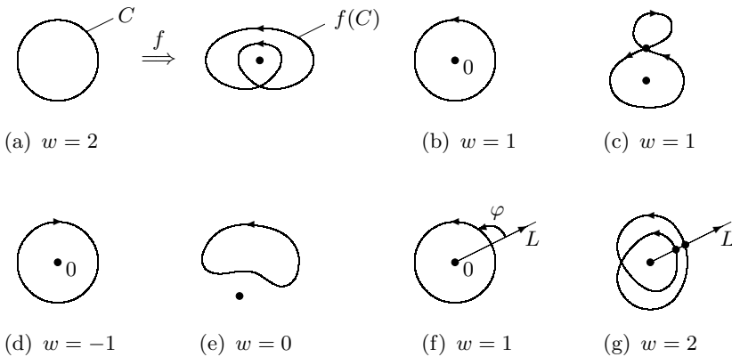
Fig. 5.6. Winding number
