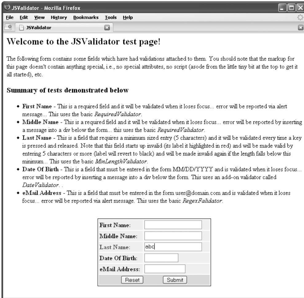
Figure 8-3. Showing a validation error via field highlighting
