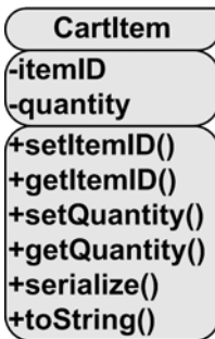
Figure 10-10. UML diagram of the CartItem class
