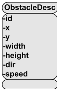
Figure 11-13. UML diagram of the ObstacleDesc class
