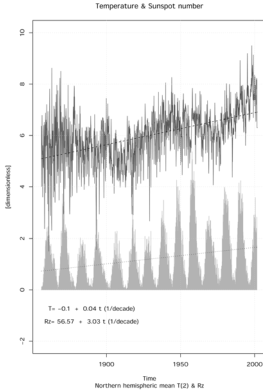
Figure 8.5. Estimated linear trend (black) in the northern hemisphere mean temperature anomalies from Jones (dark grey) suggests a mean warming of 0.04^\circ\text{C}/\text{decade} over the period 1856–2001. A similar analysis carried out for the sunspot number (grey bars) gives a trend of 3.03 numbers/decade. The data shown have been standardised. Data from: ftp://ftp.ngdc.noaa.gov/STP/SOLAR_DATA and CRU.
