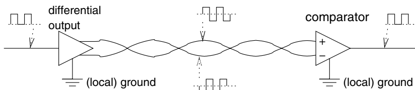
Figure 3.8. Differential signaling
