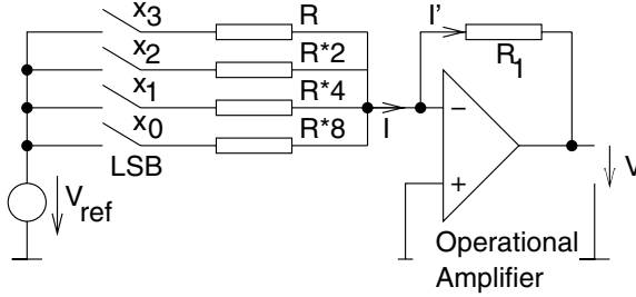
Figure 3.31. D/A-converter
