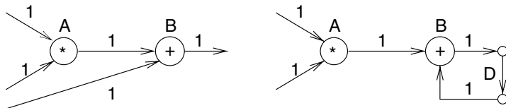
Figure 2.47. Graphical representations of synchronous data flow
