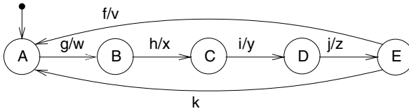
Figure 2.15. FSM described in SDL
