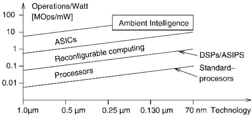
Figure 3.9. Hardware efficiency
