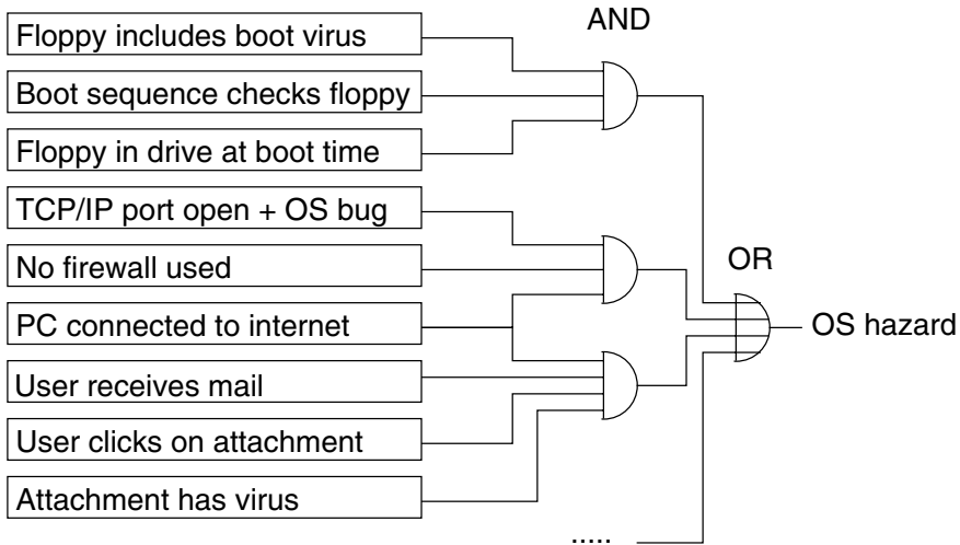
Figure 6.5. Fault tree
