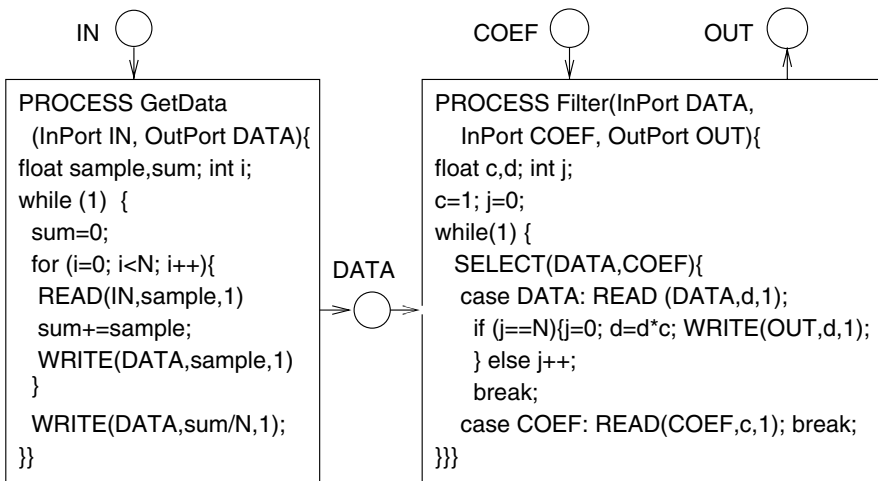
Figure 5.5. System specification
