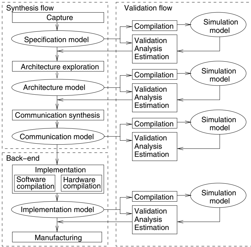
Figure 5.25. Codesign methodology possible with SpecC
