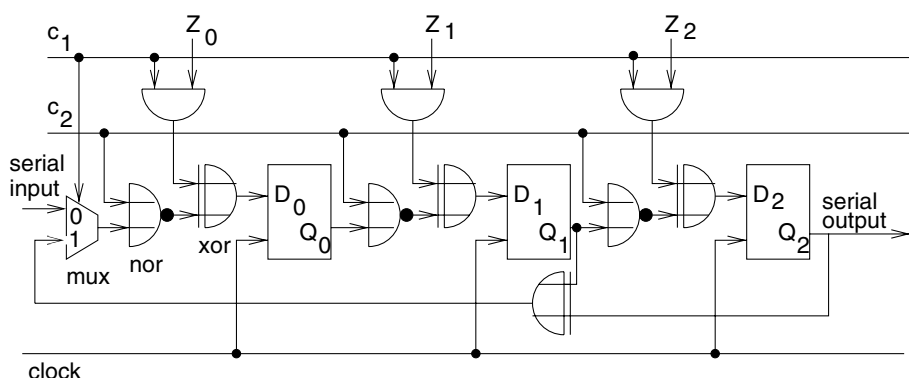
Figure 6.3. BILBO
