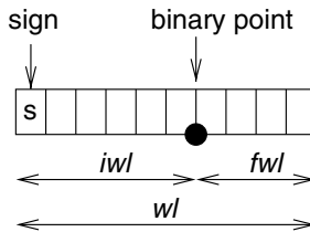
Figure 3.17. Parameters of a fixed-point number system
