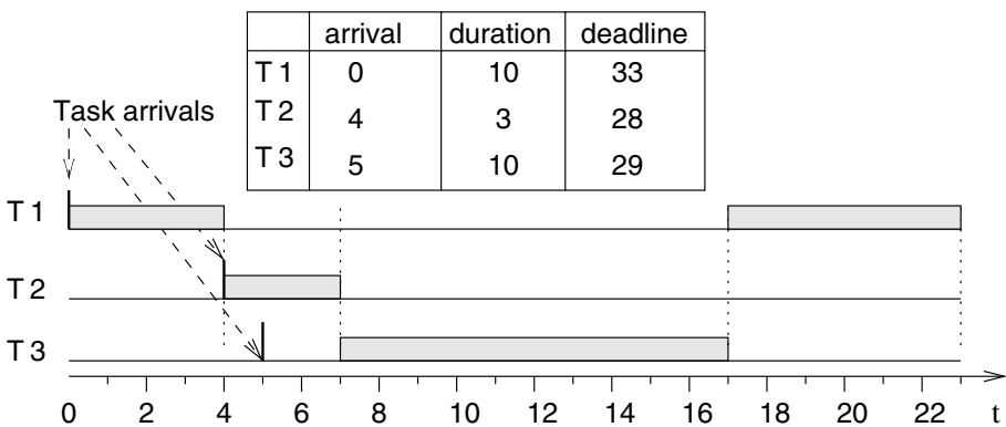
Figure 4.5. EDF schedule
