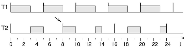
Figure 4.12. RM schedule does not meet deadline at time 8
