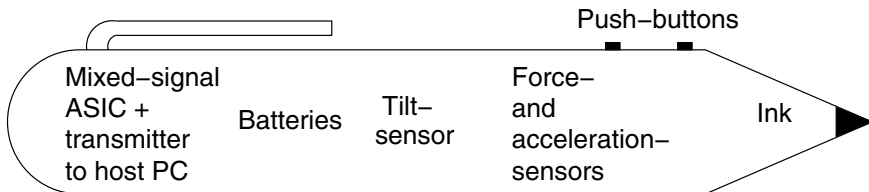
Figure 1.2. SMARTpen
