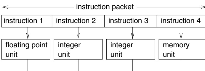
Figure 3.19. VLIW architecture (example)
