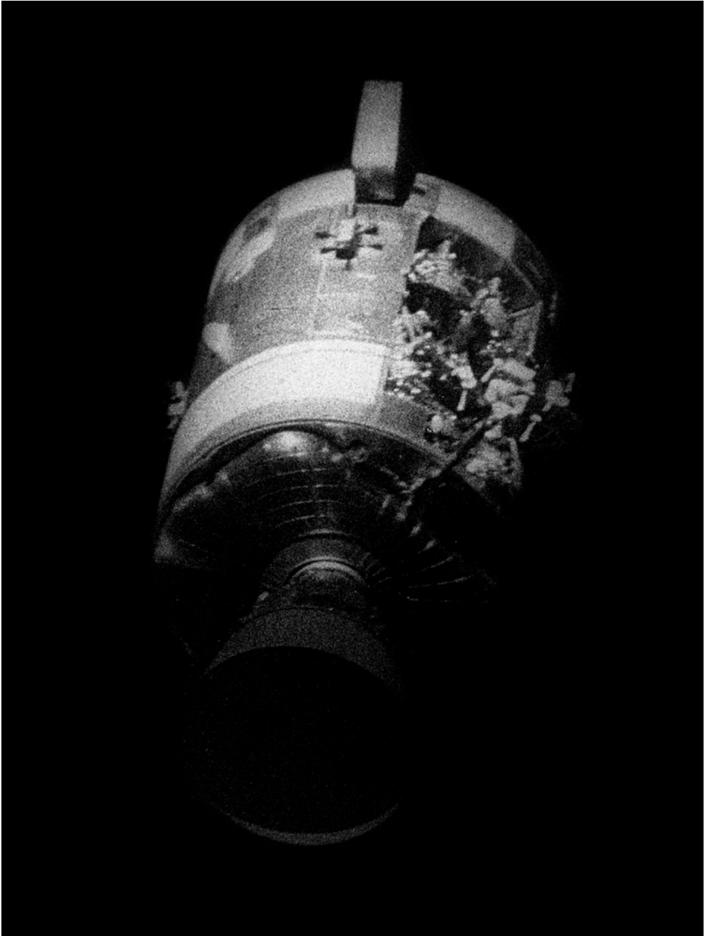
When the SM was jettisoned, the full extent of the damage became evident.
