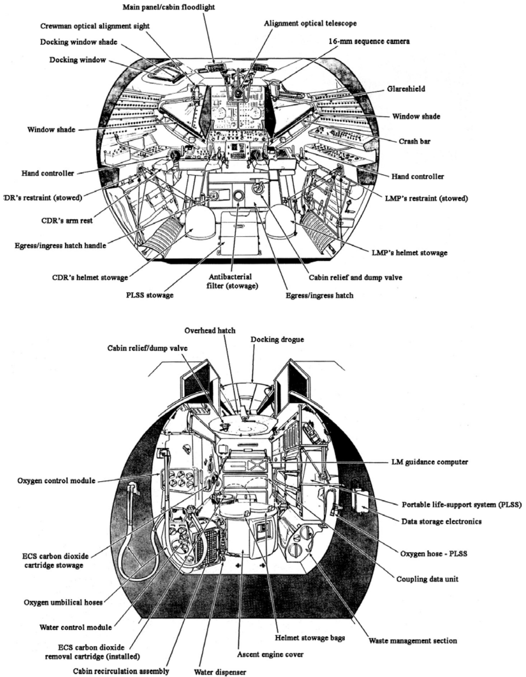
The interior layout of the LM.
