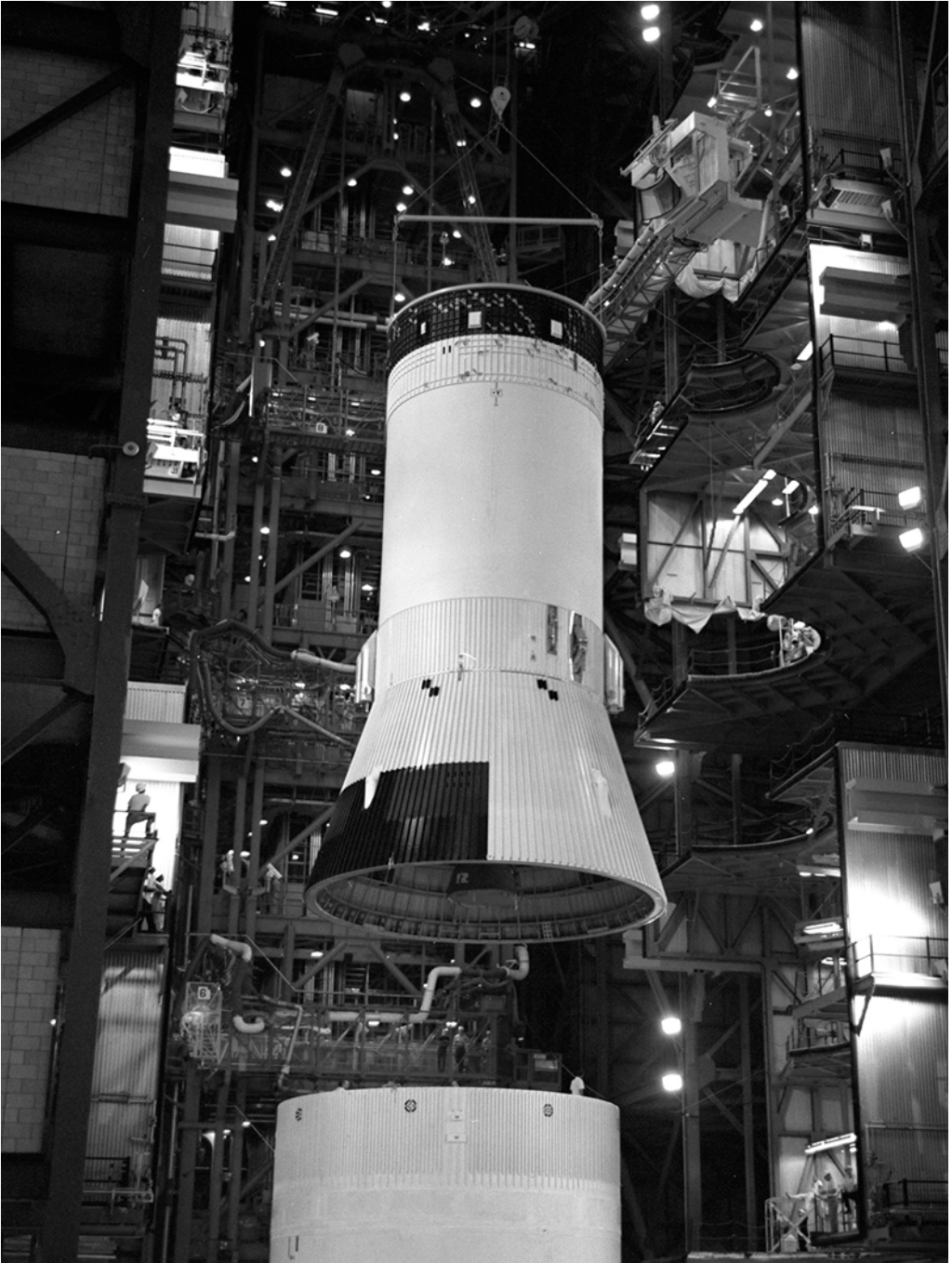
The S-IVB for AS-501 is added to the S-IC/S-II stack in a high bay of the VAB.
