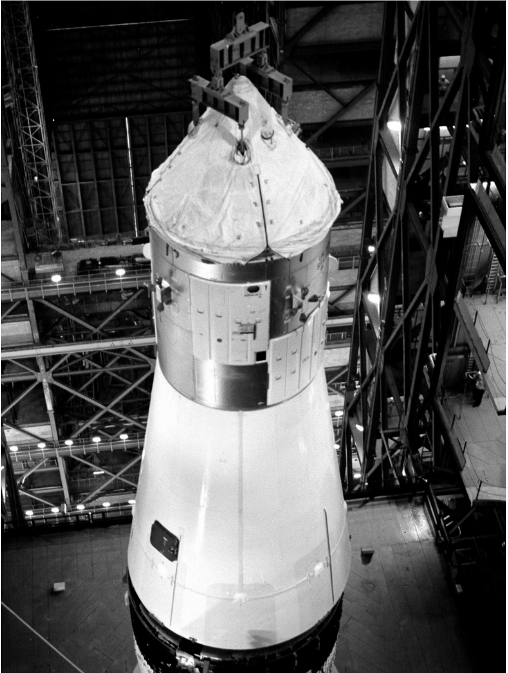
CSM-017 and LTA-10R (inside the adapter) are added.
