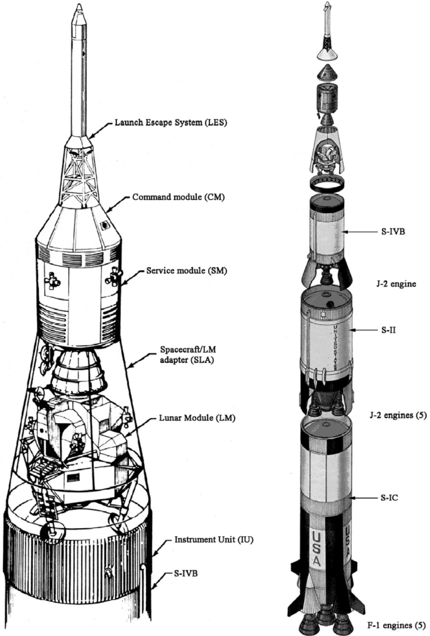
The major structural components of the Apollo-Saturn V space vehicle.
