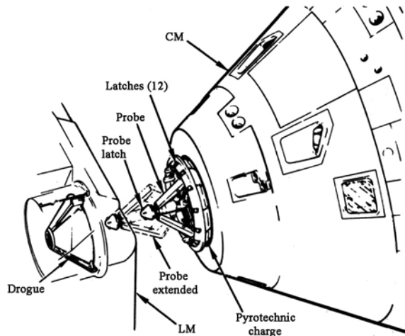
For Apollo a ‘probe and drogue’ docking assembly was selected.
