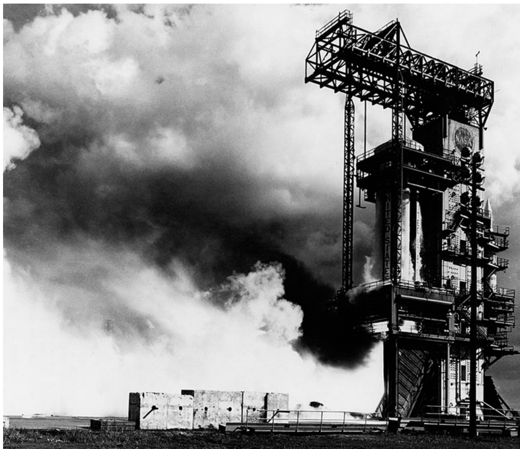
Testing the first stage for SA-1 at Huntsville.
