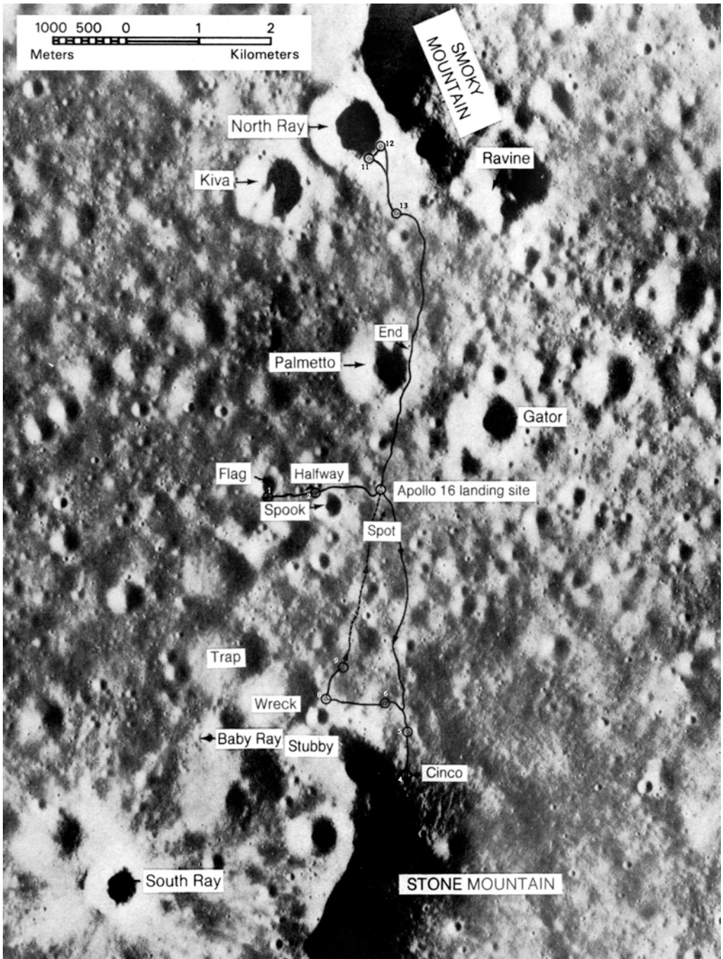
The Apollo 16 traverses. (Courtesy USGS.)
