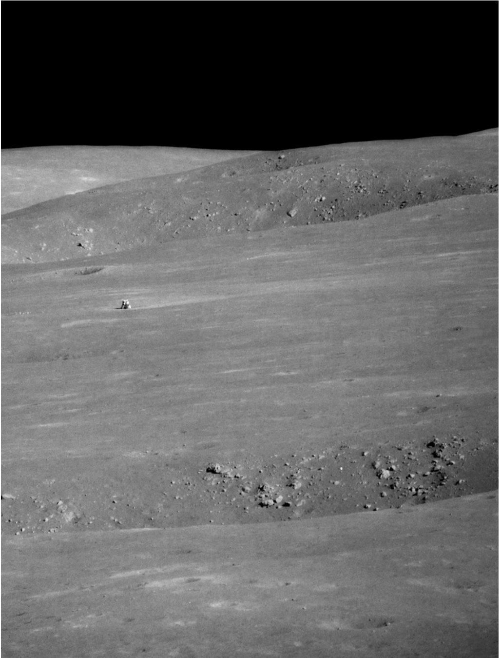
A view from the flank of Mount Hadley Delta with the LM on the plain and the North Complex beyond.
