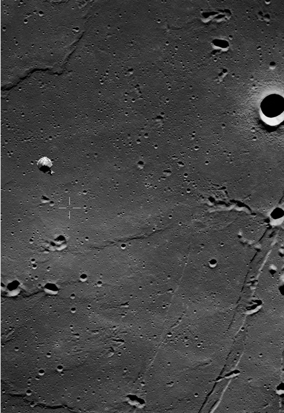
A vertical view of ALS-2 taken from the LM soon after separation (the CSM is also in the frame).
