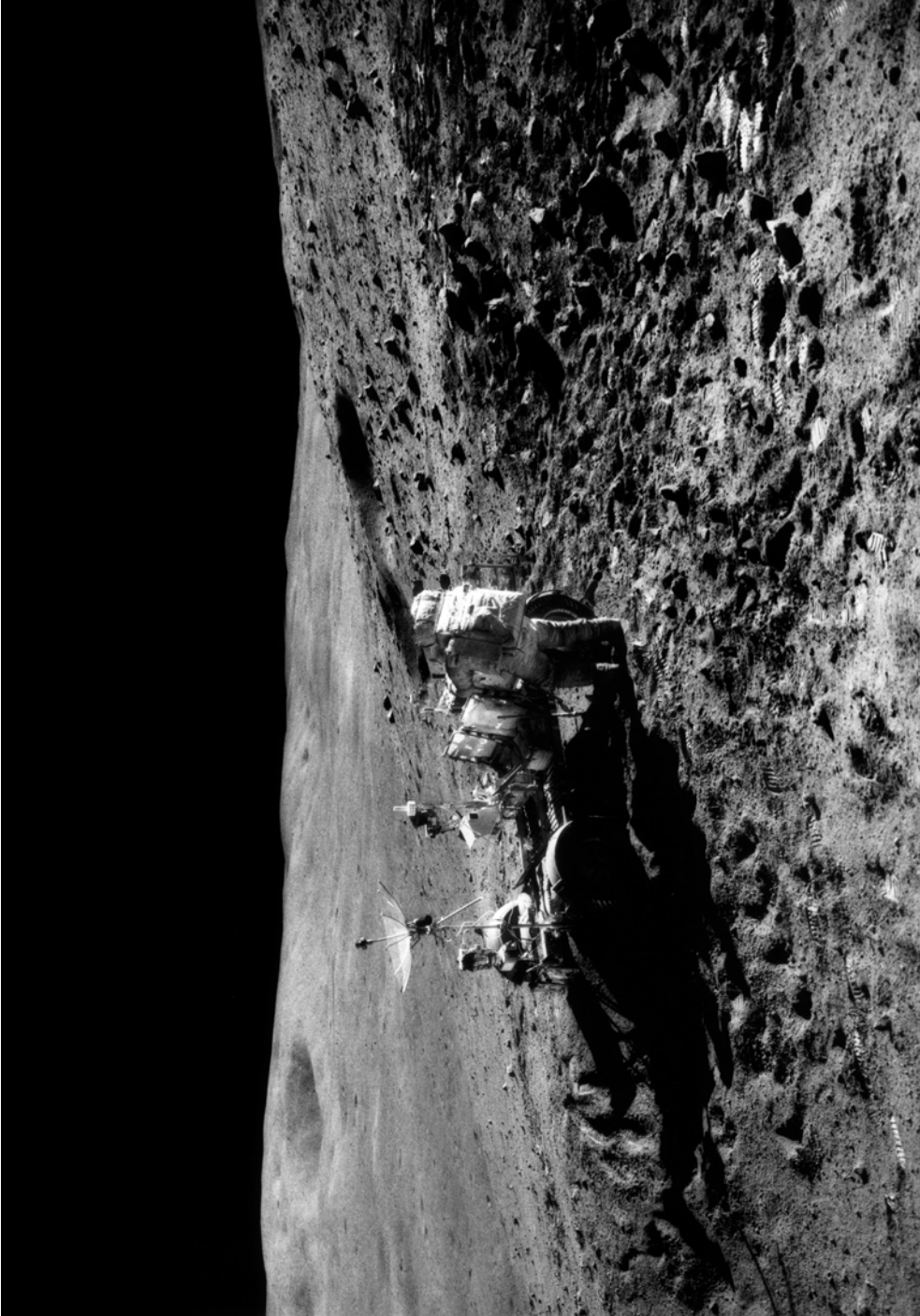
A view from station 4 on the flank of Stone mountain across the plain to Smoky mountain.
