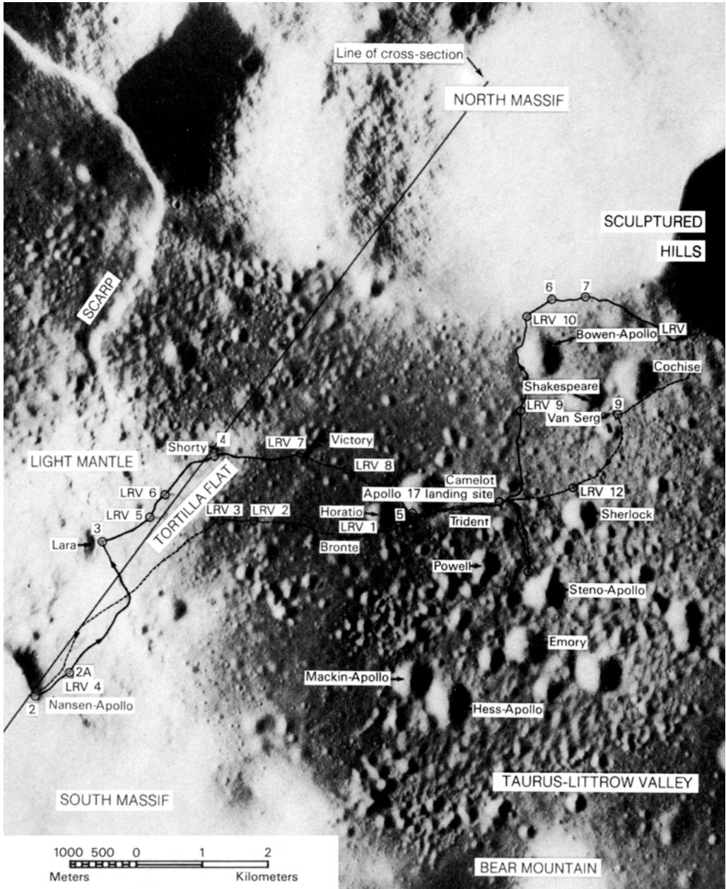
The Apollo 17 traverses. The diagonal line shows the inferred cross-section (see below). Note that although the crater near station 6 is listed as 'Bowen-Apollo', the crew actually referred to it as 'Henry the Navigator'. (Courtesy USGS.)
