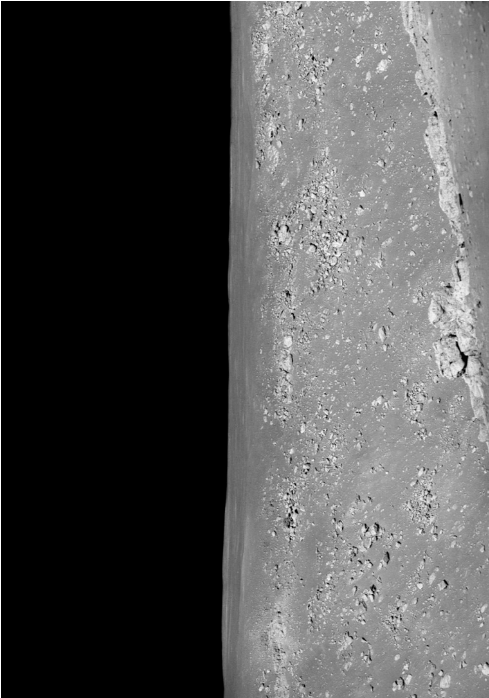
The far wall of Hadley Rille viewed from station 9A, with blocks on the near rim in the foreground.
