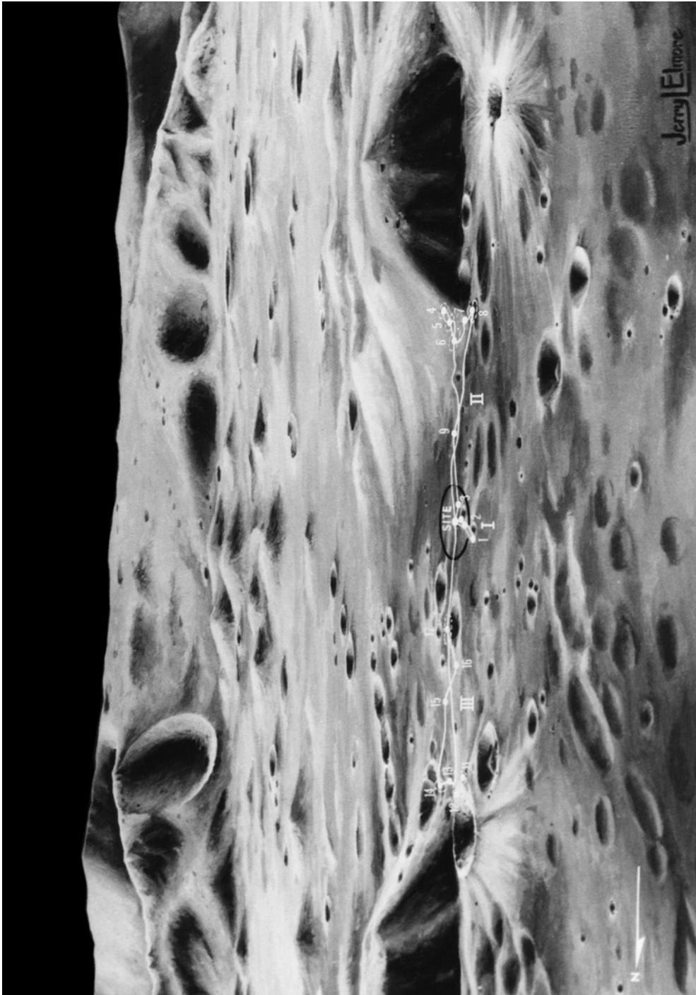
An artist's depiction of the three LRV traverses planned for Apollo 16. (Courtesy NASA.)
