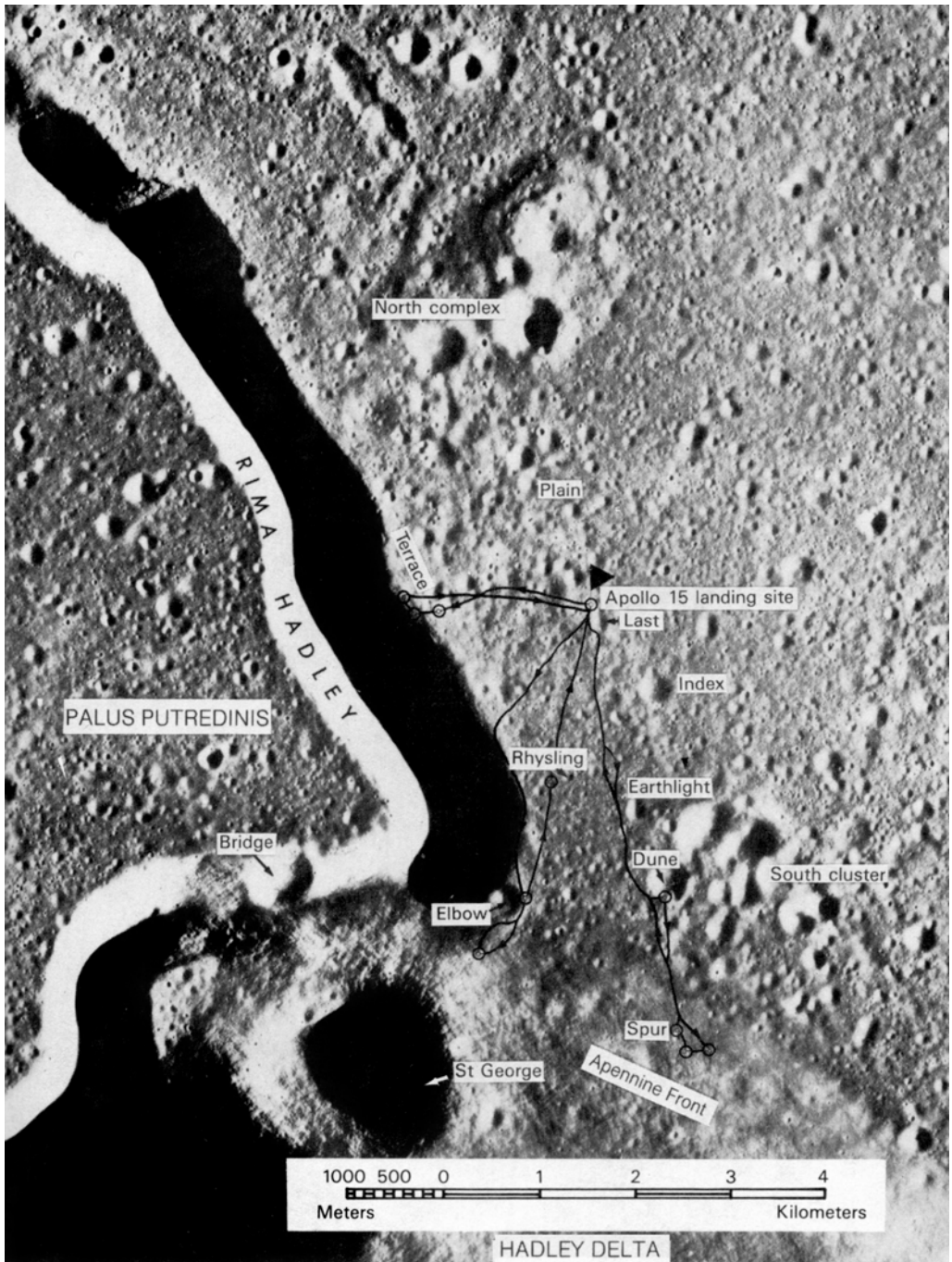
The Apollo 15 traverses. (Courtesy USGS.)
