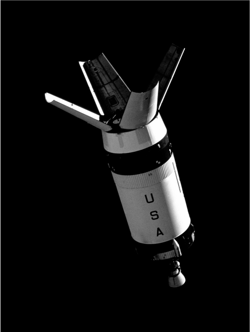
Apollo 7's spent S-IVB stage in space, with its SLA panels fully deployed.
