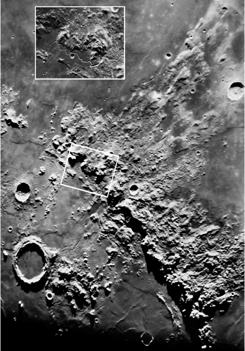
The Apollo 15 objective was Hadley Rille at the foot of the Apennine mountains.
