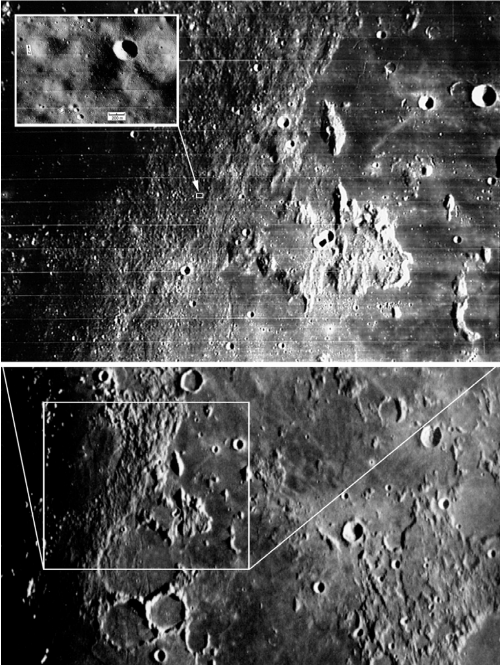
The objective was west of a small crater in the hummocky Fra Mauro Formation.
