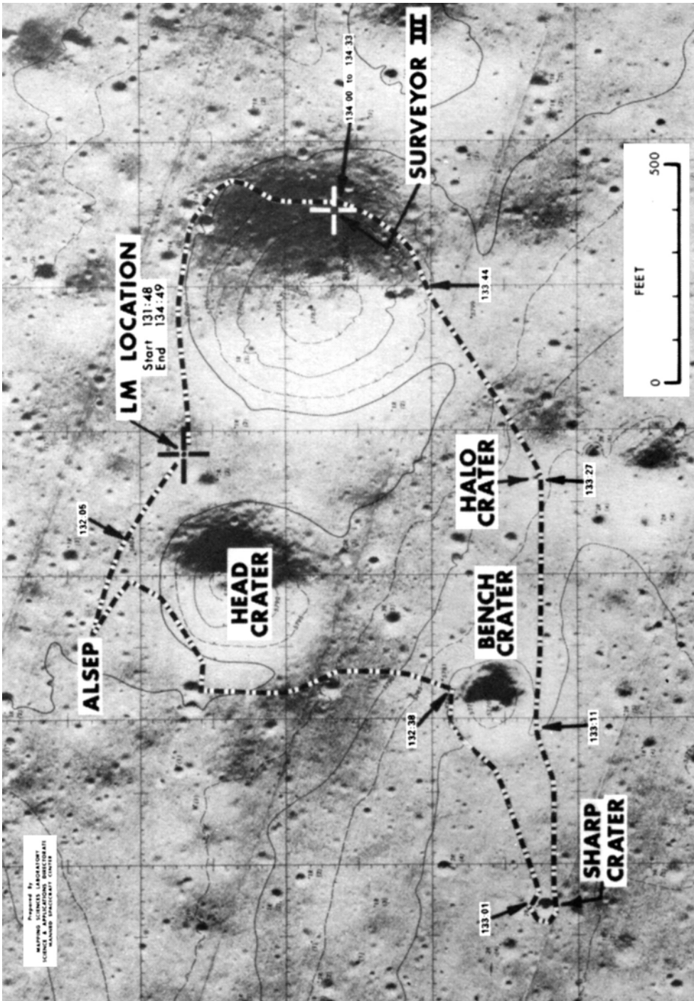
The route of Conrad and Bean's long traverse. (Courtesy USGS.)
