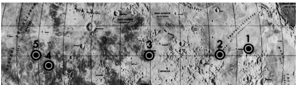
The Surveyor sites, the 'Apollo box', and the five candidate Apollo landing sites, ALS-2 being the best.
