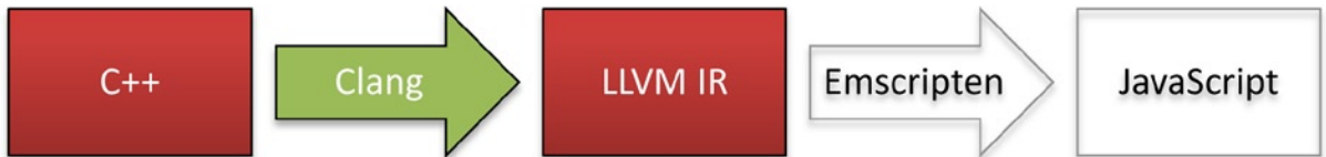
Figure 18-2. The Clang stage
