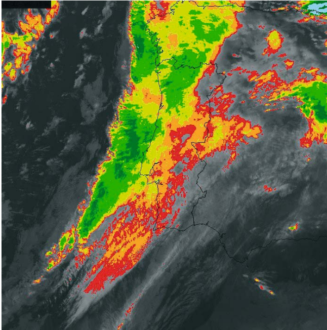
Fig. 4.5. NOAA image showing an active frontal surface crossing Mainland Portugal on 26th December, 2002
