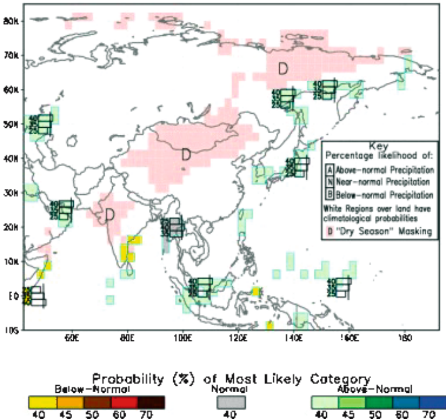
Fig. 7.10. Skill at predictions of seasonal weather has increased, especially utilizing ensemble modeling approaches and incorporating ocean data, as this prediction from Columbia University exemplifies (Source: International Research Institute – IRI)
