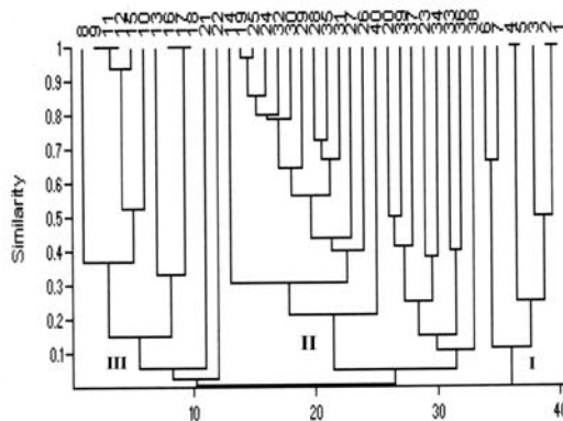
Fig. 4. Cluster analysis based on the Jaccard coefficient of similarity (the paired group average method), applied to 40 ostracod species and morphs from the study area
