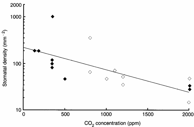
Fig. 3. Diagram showing the density of stomata in relation to the concentration of carbon dioxide in the atmosphere. Extant plants are open symbols and fossil taxa are filled symbols (after Beerling and Woodward, 1996)
