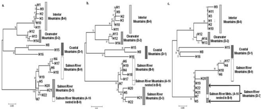
Fig. 3. Three phylogenetic gene trees produced from the intersected data set for (a) cytochrome b and ISR combined, (b) cytochrome b as a partition, and (c) ISR as a partition. The intersected data reduced to 22 haplotypes, seen at the terminal nodes of each branch (H1--H22). Bootstrap values are located at the nodes of each branch, bars to the right of each tree identify regionally based monophyletic clades, and the alpha-numeric labels, in parentheses, refer to clades from the ISR marker. A sub-clade within the Salmon River Mountains (A-16) is incongruent, whereas the Interior, Clearwater, and Coastal Mountain groups are congruent. Note that the haplotype labels in these trees apply only to this figure, because the data were reduced to include the intersected sequence partitions
