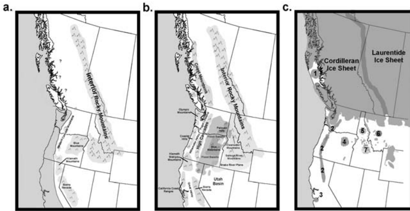
Fig. 6. The Cordilleran Ice sheet (dark grey shading) forced populations into seven isolated refugia during the Pleistocene; these are identified by the stippled regions and associated numbers
