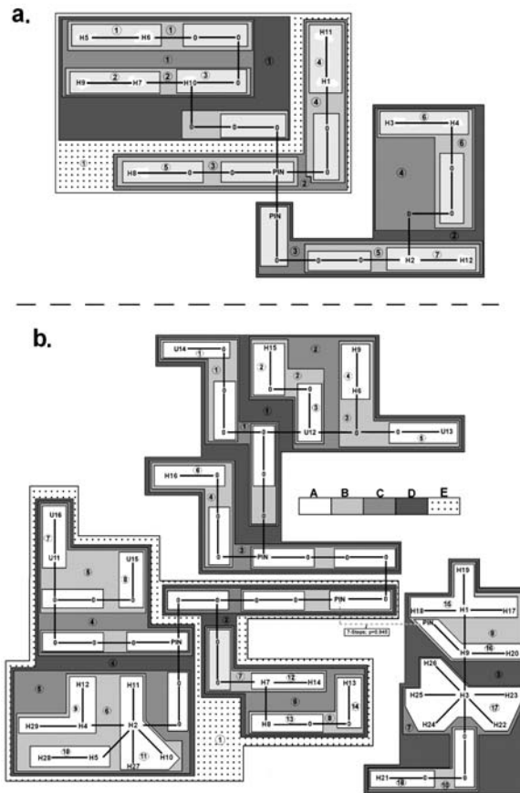
Fig. 5. In (a), the cytochrome b genealogy is resolved as a single TCS network, and the nested design contains 12 haplotypes (H1--H12). In (b), the ISR marker genealogy is statistically resolved, and the relationship among 29 haplotypes (H1--H29) is summarized into two TCS networks with a nested design. The ISR network (b) contains six haplotypes starting with a U, which refer to published GenBank sequences (McKnight and Shaffer 1997). A dashed line connecting two PINs (b) identifies the closest connection in the unresolved relationship between the two ISR networks. A shaded key discerns nesting levels A to E, and numbers in circles reference each nested category. Clades are referenced by the nesting level followed by the nested address (e.g., A-16 contains haplotypes H9 and H20, and one PIN)
