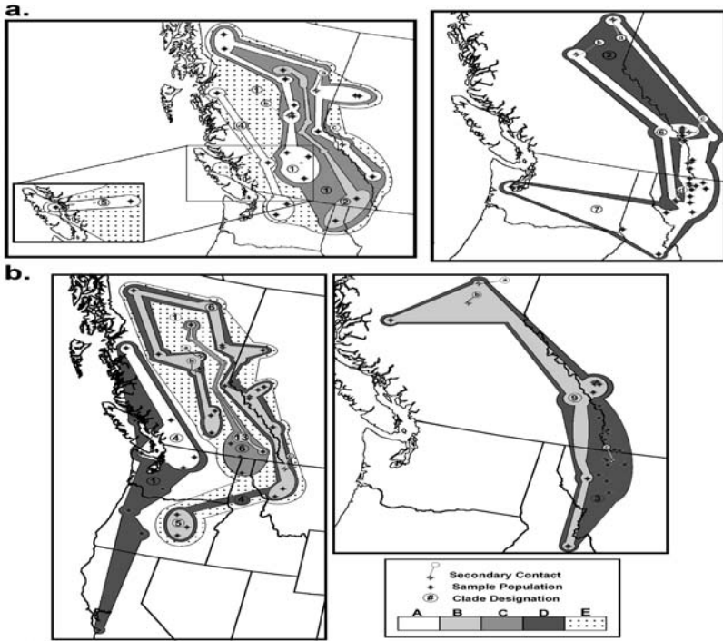
Fig. 7. Nested clade designs from Fig. 5 are spatially overlain onto a map for (a) the cytochrome b genealogy and (b) the ISR genealogy. Numbers in small circles and nesting levels correspond to those in the network design (Fig. 5). An inset of Vancouver Island, in (a), isolates clade A-5 from others for visual clarity. For reasons of simplicity, only the nesting categories that have significant range differences are indicated, and private haplotypes (haplotypes that occur in only one population, sensu Hartl and Clark 1989) are also exempt in this regard. Several populations are labeled in the post-glacial regions of Alberta and British Columbia (circles containing letters a--c), which contain a mixture of disparate clades
