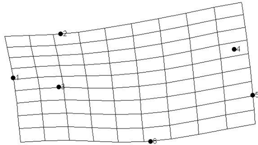
Fig. 5. The non affine deformation for the comparison between MTA and MTB
