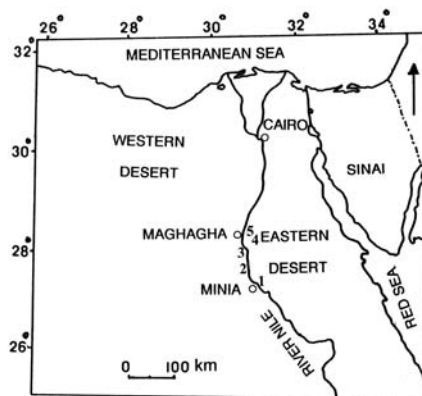
Fig. 1. Location map of the studied sections. Numbers 1 to 5 stand for the studied sections
