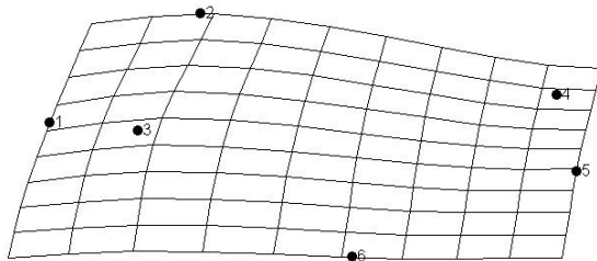
Fig. 7. The non affine deformation for the comparison between MTB and MTC
