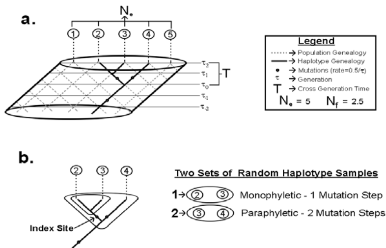
Fig. 4. A graphical illustration of a genealogy evolving within a localized portion of a population tree (a). The illustrated population has an effective breeding number ( N_e ) of 5 individuals. Five sexual generations ( \tau ) are shown with a haplotype genealogy superimposed. A single line of descent, leading to individuals 2 to 4, is isolated in (b), and these individuals share a haplotype from a single mutation between \tau_0 and \tau_1 in (a). If individuals 2 and 3 are sampled at random, then a monophyletic clade unites these haplotypes by a single index mutation, the parsimonious state, but if individuals 3 and 4 (or 2 and 4) (b) are sampled, then a non-parsimonious paraphyletic union is constructed and requires two mutational steps, a non-parsimonious state
