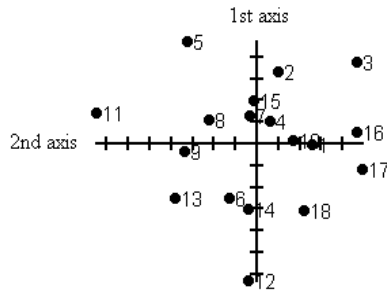
Fig. 3. Ordination by the non-affine shape components for the three studied forms. 1-10: Paracosta mokattamensis , 11-16: P. humboldti , 17-18: P. humboldti ducassae
