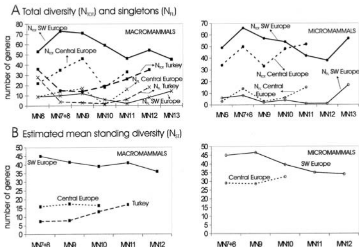
Fig. 10. Diversity calculated for selected squares: SW Europe (squares 12 + 13), Central Europe (squares 24 + 25) and Turkey (squares 8 + 9) (see text for details). A) Total diversity ( N_{TOT} ) and singletons ( N_{FL} ); B) Estimated mean standing diversity ( N_{ST} ). Plots display results for macromammals and micromammals. For results of correlation test between N_{ST} and r_i see Table 2
