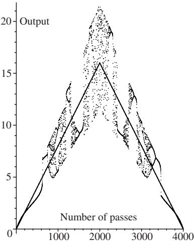
Figure 14.13: Bifurcation diagram when B = 0.15 using the second iterative method showing a plot of triangular input and output intensities against number of ring passes for the SFR resonator.
