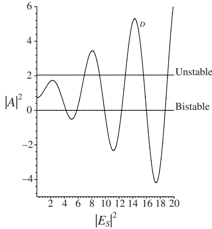
Figure 14.12: Stability diagram for the SFR resonator when B = 0.15 ( \kappa = 0.0225 ). The system is stable as long as 0 < D < 2(1 + B^2) .
