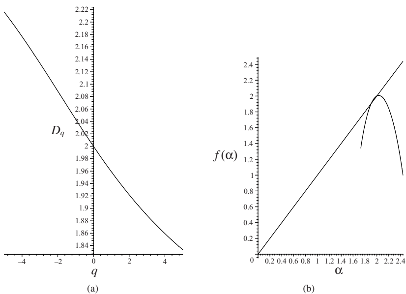
Figure 15.18: Plots for Example 5: (a) the D_q spectrum when -5 \leq q \leq 5 and (b) the f(\alpha) spectrum.
