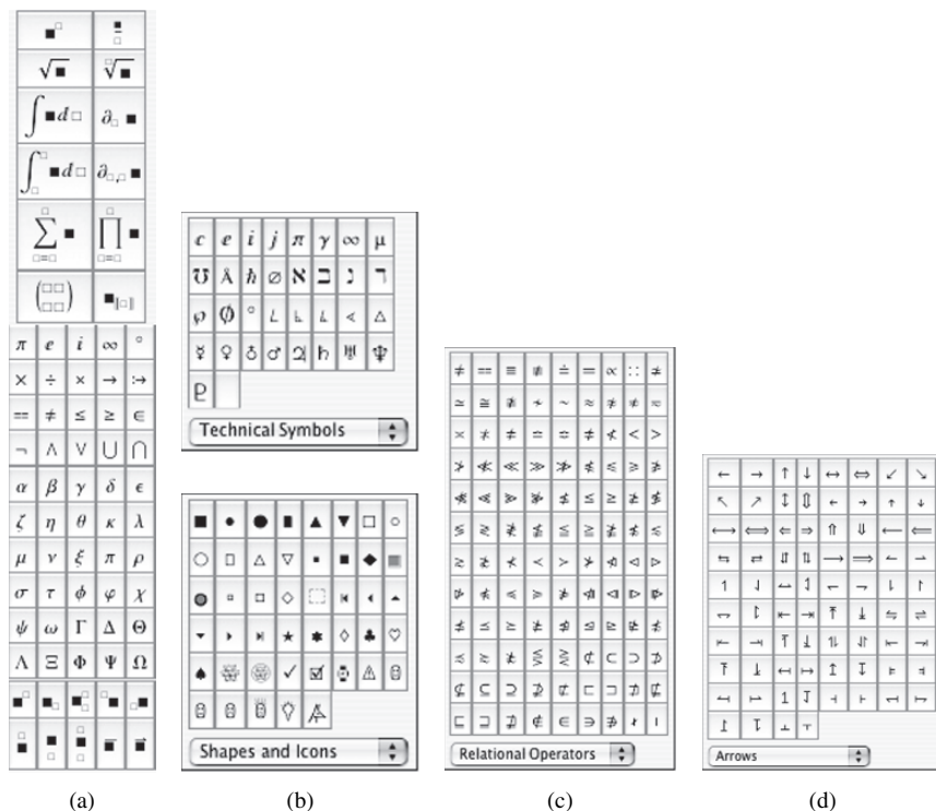
Figure 0.1: Some Mathematica palettes: (a) Basic input palette. (b) Technical symbols, shapes, and icons. (c) Relational operators. (d) Relational arrows.
