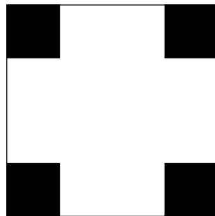
Figure 8.15: The mappings \mathbf{H} and \mathbf{H}^{-1} .
