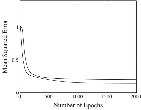
Figure 17.8: Number of epochs versus mean squared error for the Boston housing data. The upper curve is the error with one hidden neurons (settles to approximately 0.2); the lower curve is the error with two hidden neurons (stabilizes to approximately 0.14). The learning rate used in this case was \eta = 0.05 .
