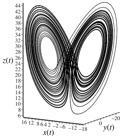
Figure 7.11: [Notebook] A strange attractor for the Lorenz system when \sigma = 10 , b = \frac{8}{3} , and r = 28 .
