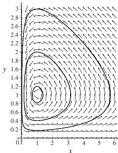
Figure 3.2: A phase portrait for the Lotka–Volterra model.
