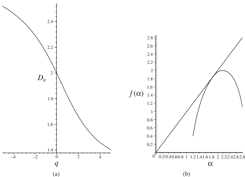
Figure 15.19: Plots for Example 6: (a) the D_q spectrum when -5 \leq q \leq 5 and (b) the f(\alpha) spectrum.
