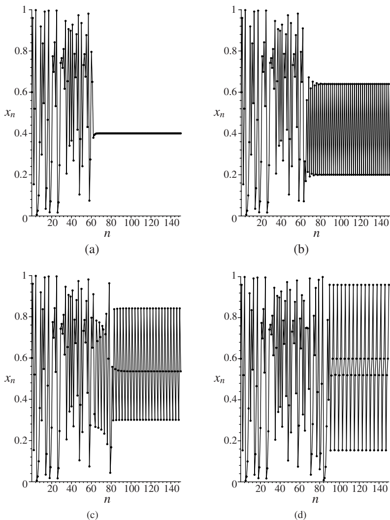
Figure 16.3: [Notebook] Stabilization of points of periods one, two, three, and four for the logistic map when \mu = 4 ; (a) x_S = 0.4 , k = 0.417 ; (b) x_S = 0.2 , k = 0.217 ; (c) x_S = 0.3 , k = 0.302 ; and (d) x_S = 0.6 , k = 0.601 . In each case k is computed to three decimal places.
