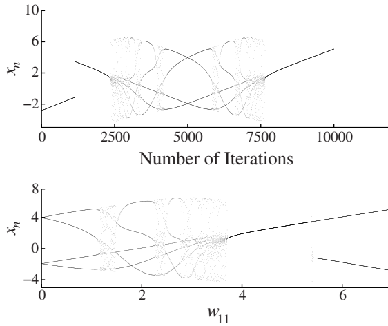
Figure 17.16: Bifurcation diagrams for system (17.7) under conditions (17.10) and (17.11) as w_{11} varies. The initial conditions chosen at w_{11} = 7 were x_0 = -3 and y_0 = -2 .
