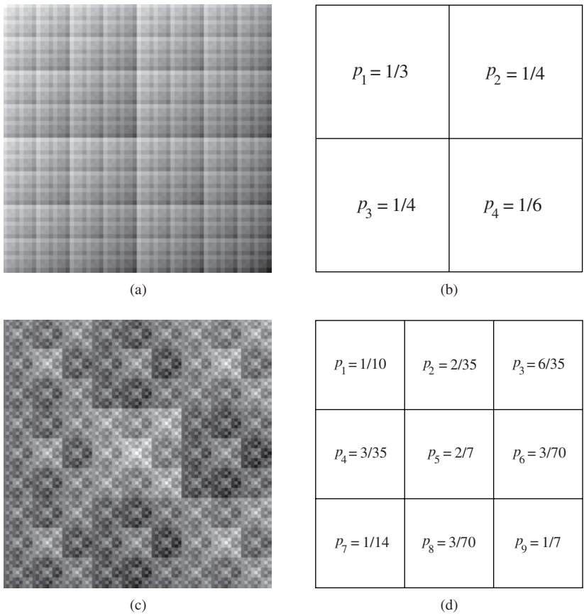
Figure 15.17: Multifractal images and the weight distribution motifs. The weights are related to the grey scale; for example, p_1 = 1 would be white and p_1 = 0 would be black on this scale.
