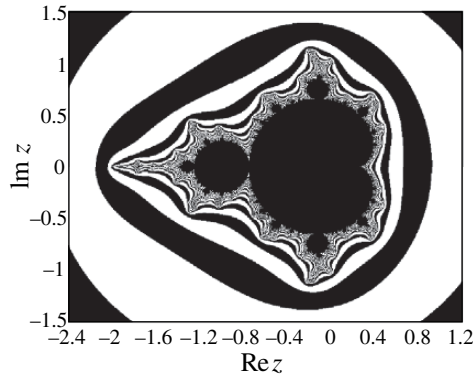
Figure 13.2: [Notebook] The Mandelbrot set (central black figure) produced using a personal computer.
