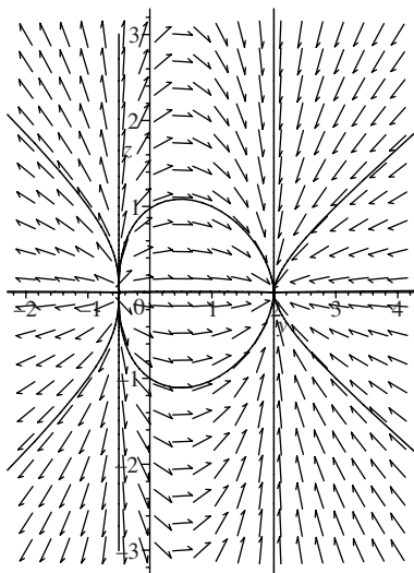
Figure 10.6: Some trajectories in the yz plane ( X = 1 ) that define the flow at infinity.
