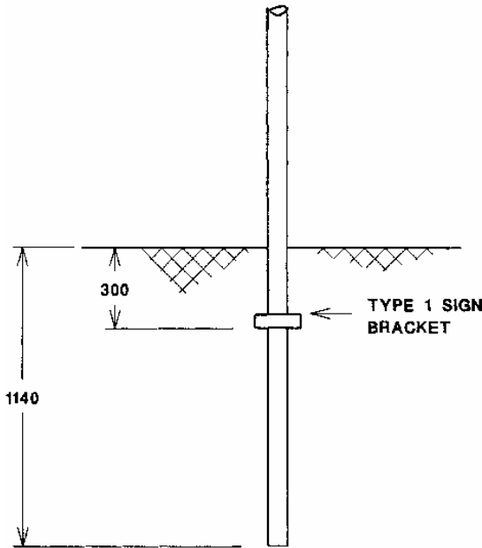
FIGURE 7.23 Aluminum tube sign installation. Dimensions shown as mm. Conversions: 300 mm = 12 in, 1140 mm = 45 in.
