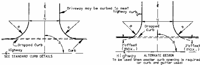
FIGURE 2.56 Designs for commercial drives. (From Location and Design Manual, Vol. 1, Roadway Design, Ohio Department of Transportation, with permission)
