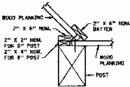
TRAFFIC SIDE WALL TYPE NO. 3 ① ②
