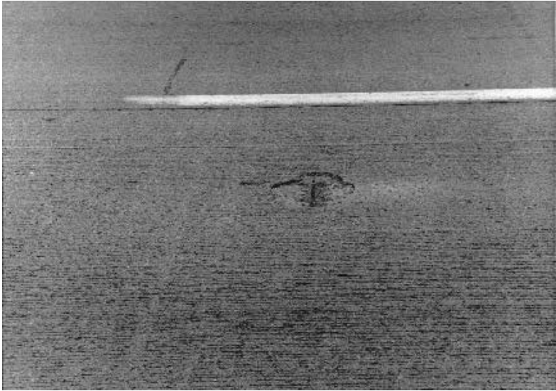
FIGURE 3.23 Example of popout in jointed rigid pavement.
