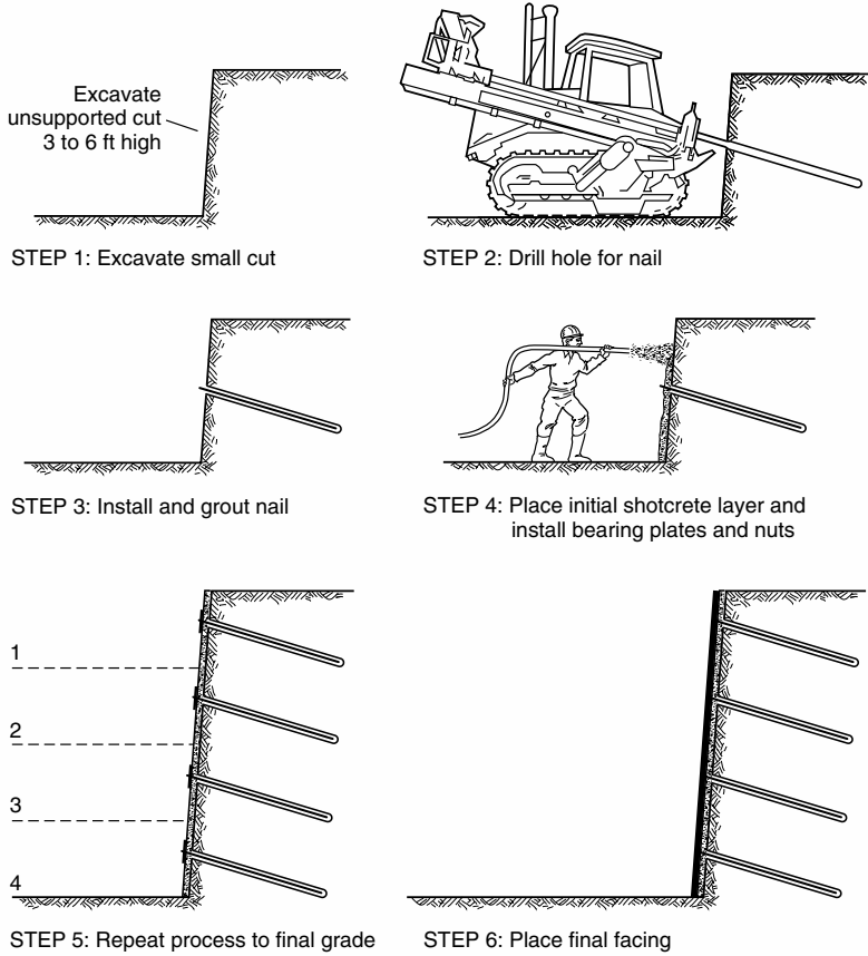
FIGURE 8.56 Typical construction sequence for soil nailed wall.
