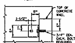
ELEVATION 90° JOINT
