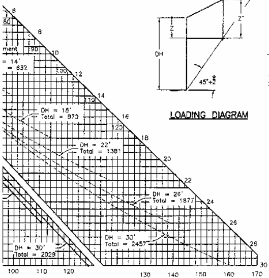
PATTERN C REINFORCEMENT PATTERNS (See note 2)
