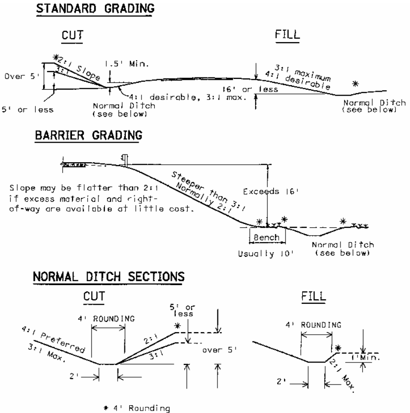
FIGURE 2.19 Examples of standard grading and normal ditches. (From Location and Design Manual, Vol. 1, Roadway Design, Ohio Department of Transportation, with permission)
