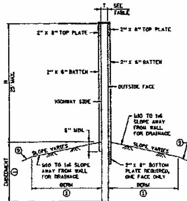
SECTION A-A WITHOUT EARTH FILL
