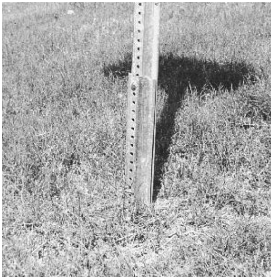
FIGURE 7.12 Improper splice of U-channel post system.
