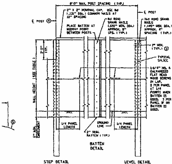
FRONT ELEVATION POST BATTERS NOT SHOWN
