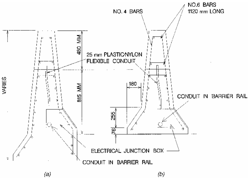
FIGURE 7.94 Details for luminaire foundation installed in concrete median barrier. (a) With super-elevation. (b) Without super-elevation. Dimensions shown as mm. Conversions: 76 mm = 3 in, 180 mm = 7 in, 255 mm = 10 in, 480 mm = 19 in, 815 mm = 32 in, 1120 mm = 44 in.
