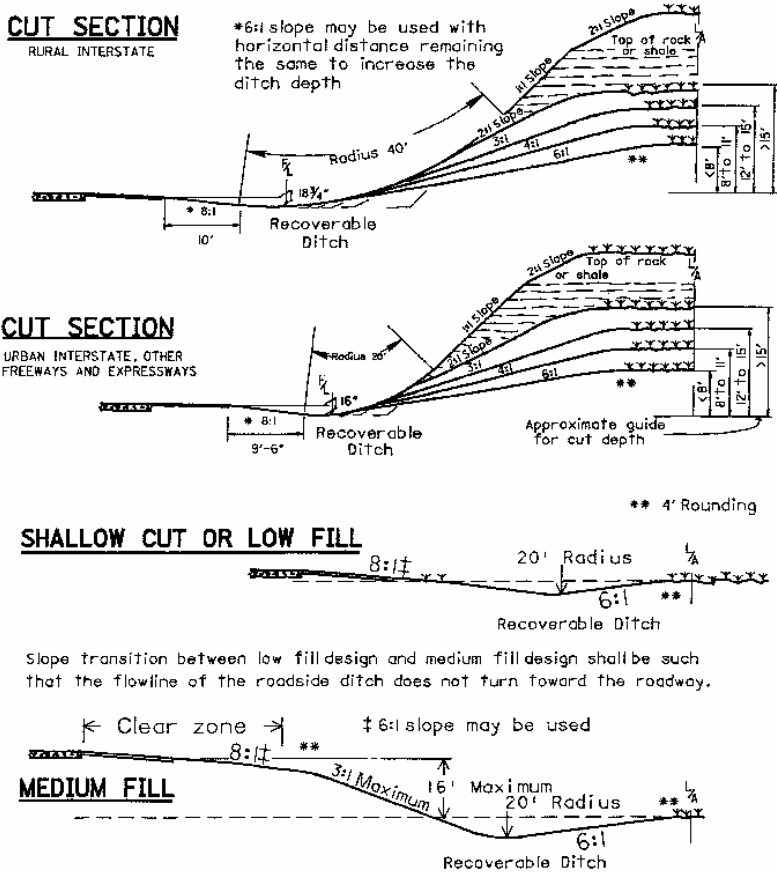
FIGURE 2.16 Cross sections showing safety grading for four different conditions. (From Location and Design Manual, Vol. 1, Roadway Design, Ohio Department of Transportation, with permission)
