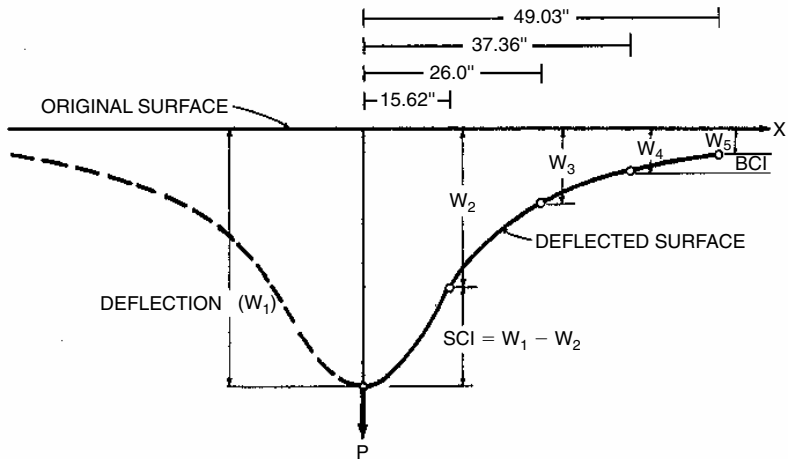
FIGURE 3.48 Typical Dynaflect deflection bowl deflection basin parameters. W_{\text{MAX}} = deflection ( W_1 ); SCI = surface curvature index (numerical difference between sensors 1 and 2); BCI = base curvature index (numerical difference between sensors 4 and 5); SPR% = spreadability ( \sum W/W_1 \times 100 ). (From K. Majidzadeh and V. Kumar, Manual of Operation and Use of Dynaflect for Pavement Evaluation, Resource International, Inc., Columbus, Ohio, Report No. FHWA/OH-83/004, October 1983, with permission)
