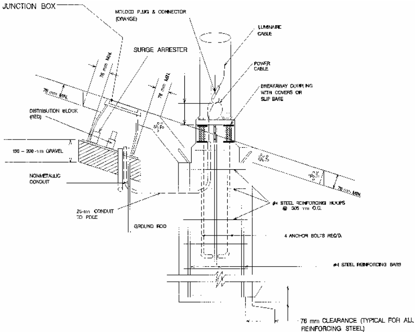
FIGURE 7.87 Flush-mounted electrical junction box. Conversions: 25 mm = 1 in, 76 mm = 3 in, 150 mm = 6 in, 200 mm = 8 in, 305 mm = 12 in.
