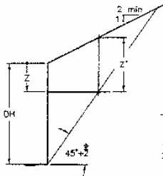
LOADING DIAGRAM
