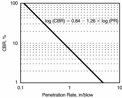
FIGURE 3.47 Correlation of California Bearing Ratio (CBR) and penetration rate. (From Pavement Technology Advisory 97-7 , Dynamic Cone Penetrometer, Illinois Department of Transportation, Bureau of Materials and Physical Research, 1997, with permission)
