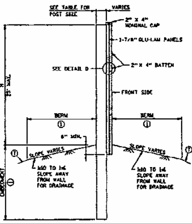
SECTION AT POST WITHOUT EARTH FILL
