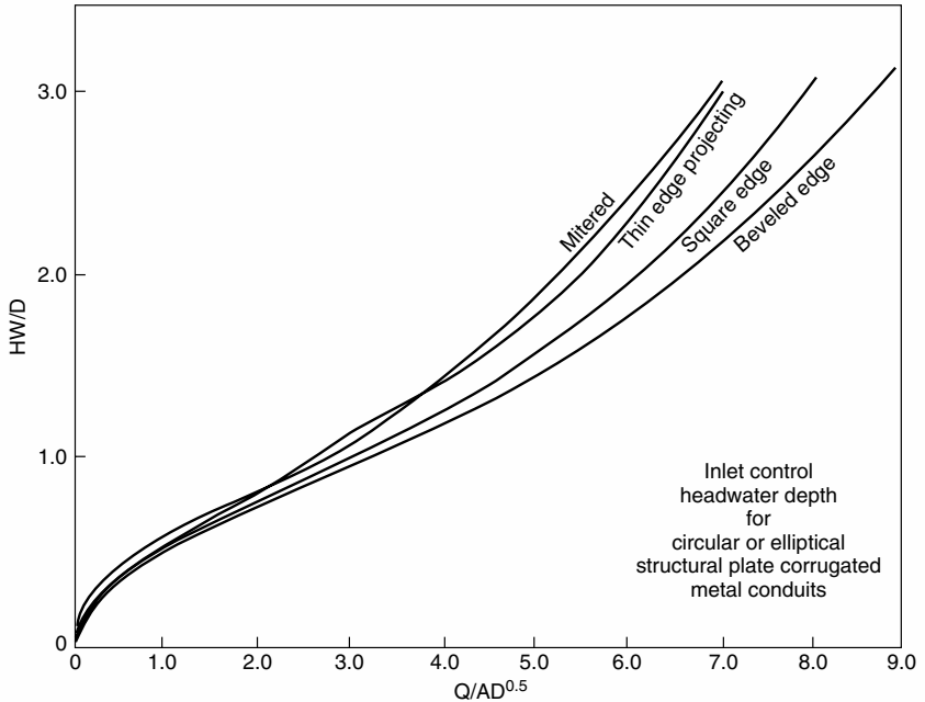
FIGURE 5.17 Performance charts for circular or elliptical structural-plate conduits under inlet flow control. (From "Hydraulic Design of Highway Culverts," Hydraulic Design Series No. 5, FHWA, with permission)
