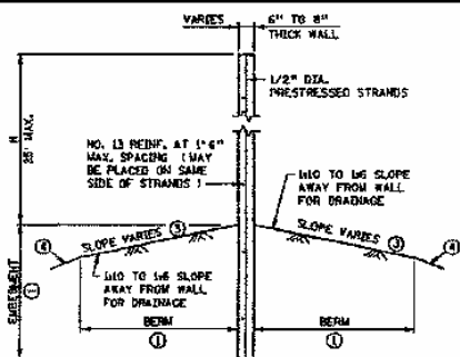
SECTION THRU WALL WITHOUT EARTH FILL
