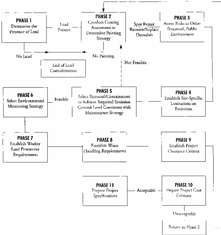
FIGURE 1.2 Decision chart for management of lead paint removal. (From K. A. Trimblor, Industrial Lead Paint Removal Handbook, 2d ed., Steel Structures Painting Council/KTA-Tator, Inc., Pittsburgh, 1993, with permission. )
