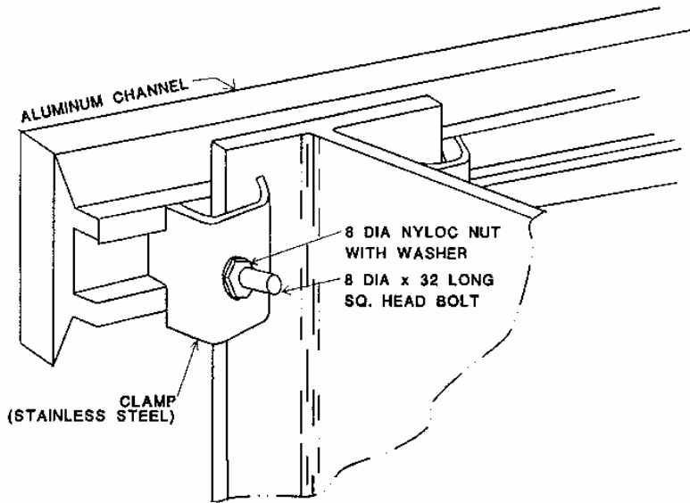
FIGURE 7.60 Extruded aluminum channel for attaching sign panels to beam post. Dimensions shown as mm. Conversions: 8 mm = \frac{5}{16} in, 32 mm = 1 \frac{1}{8} in.
