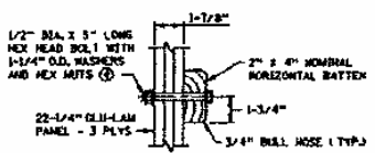
DETAIL D
