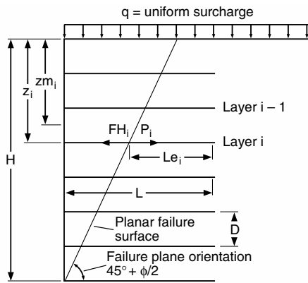
FIGURE 8.31 Parameters for tied-back wedge analysis.
