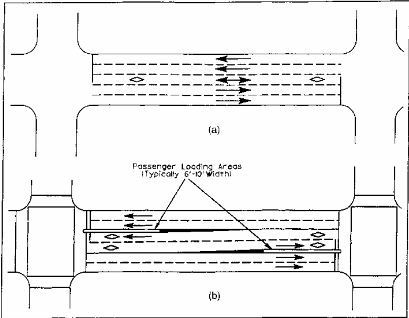
FIGURE 2.70 Examples of median HOV lanes for buses. (a) Reversible lanes for express buses. (b) Two-way lanes for local buses. (From Guide for the Design of High Occupancy Vehicle Facilities , American Association of State Highway and Transportation Officials, Washington, D.C., 1992, with permission)
