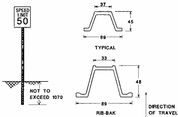
FIGURE 7.9 Installation and cross section of typical steel U-channel and RIB-BAK 3-lb/ft (4.5-kg/m) posts. Dimensions shown as mm. Conversions: 33 mm = 1 \frac{1}{8} in, 37 mm = 1 \frac{1}{2} in, 45 mm = 1 \frac{3}{4} in, 89 mm = 3 \frac{1}{2} in, 1070 mm = 42 in.
