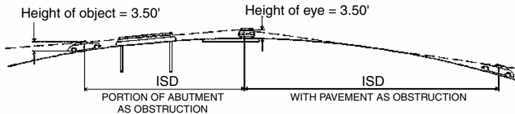
FIGURE 2.7 Intersection sight triangles. (a) Sight triangles. (b) Vertical components. a_1 = the distance, along the minor road, from the decision point to \frac{1}{2} the lane width of the approaching vehicle on the major road. a_2 = the distance, along the minor road, from the decision point to 1\frac{1}{2} the lane width of the approaching vehicle on the major road. b = intersection sight distance (ISD). d = the distance from the edge of the traveled way of the major road to the decision point; the distance should be a minimum of 14.4 ft and 17.8 ft preferred. (From Location and Design Manual, Vol. 1, Roadway Design, Ohio Department of Transportation, with permission)
