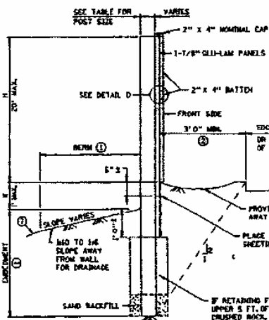
SECTION AT POST WITH EARTH FILL
