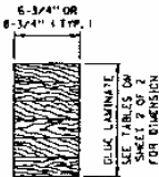
OPTIONAL GLUE LAMINATE POST DETAIL
