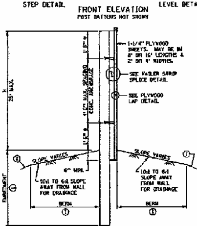
SECTION AT POST WITHOUT EARTH FILL
