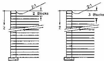
PATTERN C REINFORCEMENT PATTERNS (See note 2)
