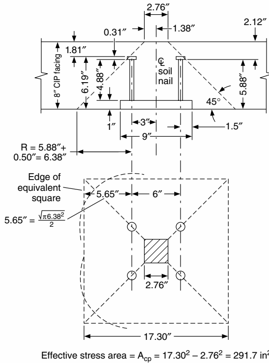
FIGURE 8.62 Bearing plate for soil nailed wall showing effective stress area for embedment design capacity. (From J. W. Keeley, Soil Nail Wall Facing: Sample Design Calculations , Federal Highway Administration, 1993, with permission)
