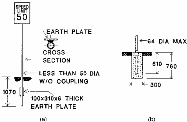
FIGURE 7.20 Standard steel-pipe sign supports. (a) Direct burial. (b) Breakaway collar assembly. Dimensions shown as mm. Conversions: 6 mm = \frac{1}{4} in, 64 mm = 2.5 in, 50 mm = 2 in, 100 mm = 4 in, 300 mm = 12 in, 310 mm = 12 in, 610 mm = 24 in, 760 mm = 30 in, 1070 mm = 42 in.
