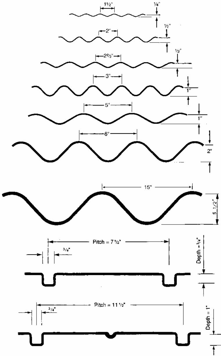
FIGURE 5.24 Profiles for corrugated steel pipe and spiral-rib pipe. (From Handbook of Steel Drainage and Highway Construction Products, American Iron and Steel Institute, 1994, with permission)
