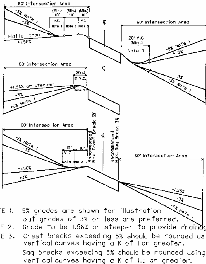
FIGURE 2.32 Crossroad profiles for stop condition where through road is superelevated. (From Location and Design Manual, Vol. 1, Roadway Design, Ohio Department of Transportation, with permission)
