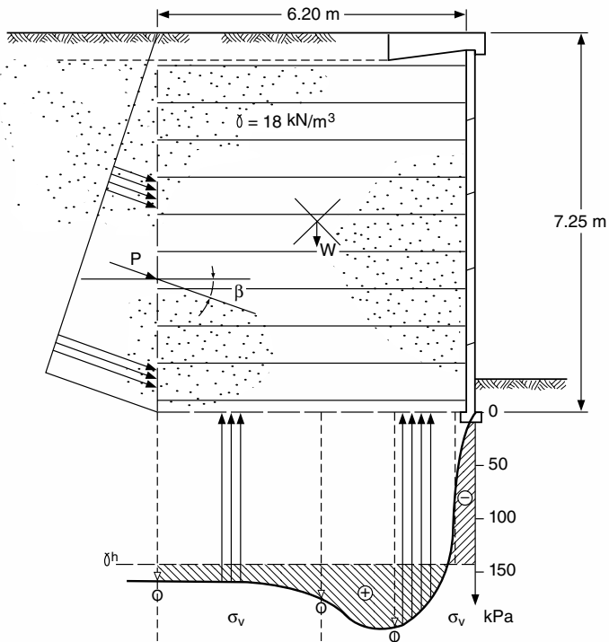
FIGURE 8.34 Freimersdorf MSE wall with foundation pressures from pressure cell readings. (From the Reinforced Earth Co., with permission)
