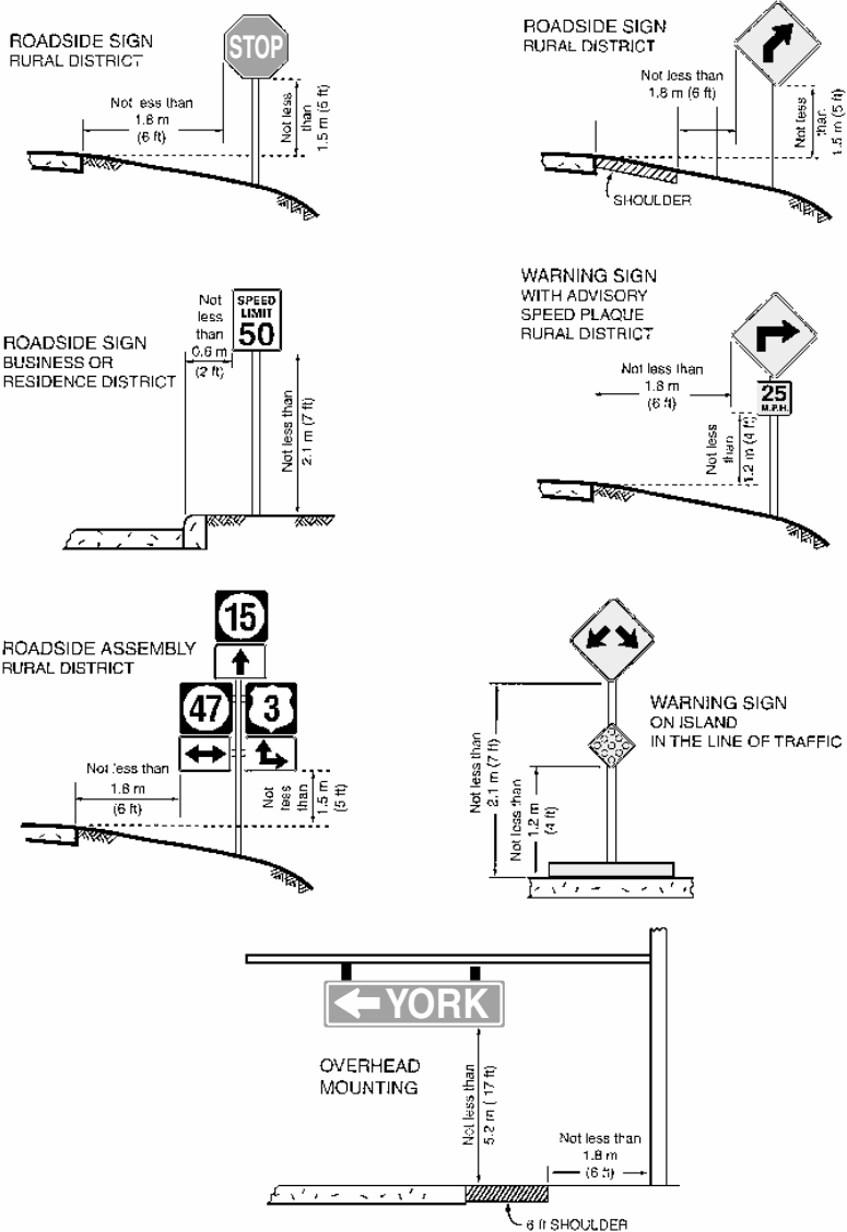
FIGURE 7.2 Height and lateral placement of signs. (Adapted from Manual on Uniform Traffic Control Devices, FHWA, 2001)
