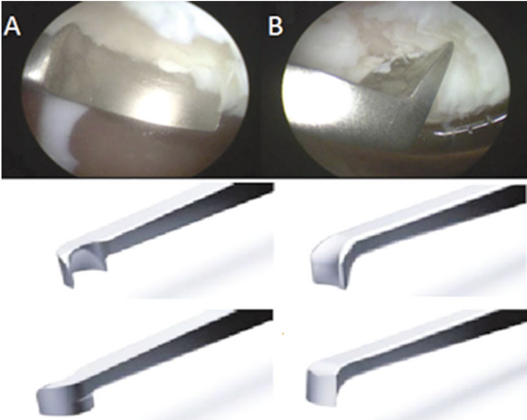
Fig. 3 Chondrectomes: instruments designed for arthroscopic removal of damaged cartilage and for creation of vertical ring surrounding the defected cartilage
