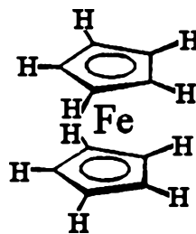
Ferrocene (and derivatives) — Figure
