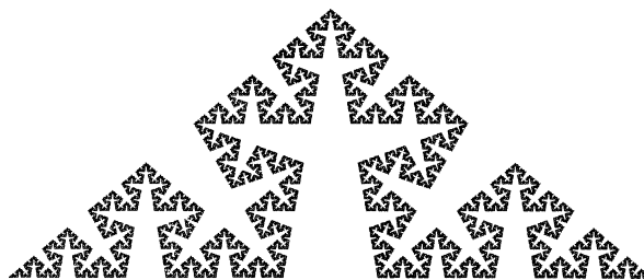
Fractals in electrochemistry — Figure. A von Koch curve of D_f = 1.5 . Note that no characteristic length of the structures can be identified – this is associated with the fact that the size-distribution of the features of the curves is a power-law function
