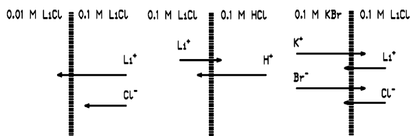
Liquid junction potential — Figure
