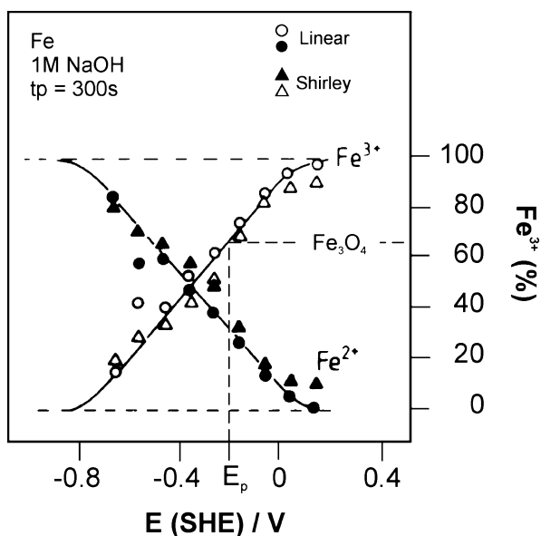
Passivation potential — Figure 3. Evaluation of XPS data of Fig. 2 with an average composition of the oxide layer with composition \text{Fe}_3\text{O}_4 at E_p = E_{\text{Fe}2} [i, iii]
