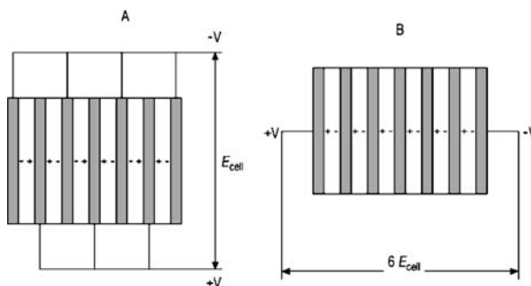
Parallel plate and frame cell — Figure
