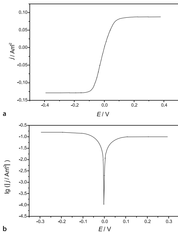
Reversibility — Figure 3. Reversible system. a Current–potential curve and b \lg |j| – E plot. Characteristic parameters are: E_e = 0.0 V, j_0 = 50 A m ^{-2} , n = 1 , D_R = 5 \times 10^{-10} m ^2 s ^{-1} , D_O = 10^{-9} m ^2 s ^{-1} , c_R^* = c_O^* = 10^{-4} mol dm ^{-3} , \omega_r = 50 s ^{-1} , v = 10^{-6} m ^2 s ^{-1} , \alpha_a = \alpha_c = 0.5 , T = 298.15 K
