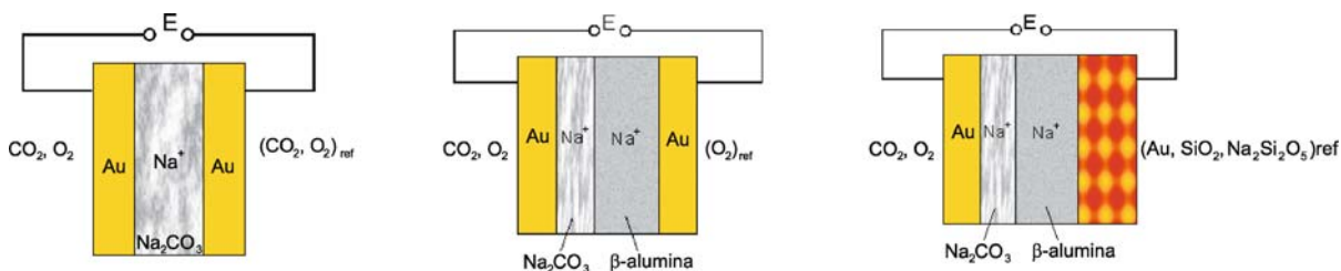
Gas sensors — (b) Gas sensors with solid electrolytes — Figure 6. Basic principle of CO 2 sensors
