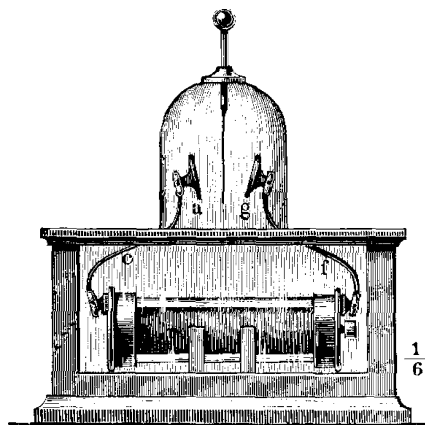
Fechner electroscope (electrometer) — Figure
