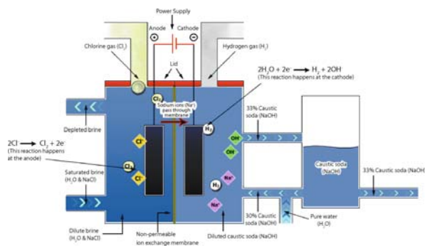
Alkali chloride electrolysis — Figure 3
