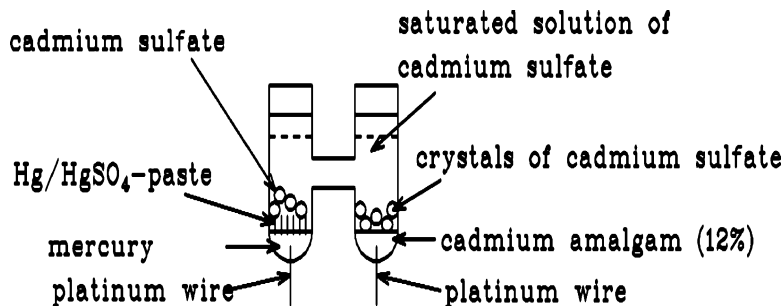
Weston normal element (cell) — Figure
