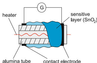
Gas sensors — (c) Metal oxide gas sensors — Figure 7. Gas sensor based on SnO 2 thick-film
