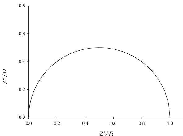
Complex plane plot — Figure. Theoretical \rightarrow impedance of a parallel connection of a resistance and a capacitance
