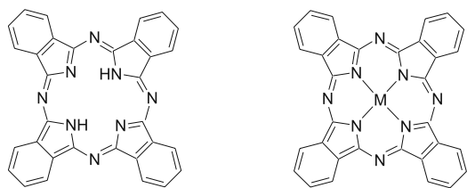
29H, 31H-phthalocyanine
