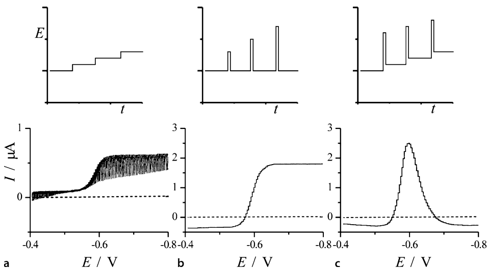
Polarogram — Figure. Potential program and the respective (a) direct current (DC) (staircase ramp), (b) normal pulse (NP) and (c), differential pulse (DP) polarograms of 0.1 \text{ mM Cd}(\text{NO}_3)_2 . All measurements were in water with 0.1 \text{ M KCl} , E is versus a SCE, scan rate = 2 \text{ mVs}^{-1} and drop time = 2 \text{ s} . Differential pulse height = 10 \text{ mV}
