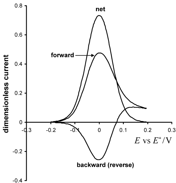
Reversible square-wave voltammogram — Figure . Theoretical dimensionless square-wave voltammogram of a reversible electrode reaction (see → reversible redox reaction ) of a dissolved redox couple at a planar electrode assuming a semi-infinite diffusion model simulated with nE_{sw} = 50 mV and a scan increment of the staircase ramp of 5 mV (see → square-wave voltammetry )
