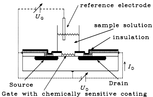
CHEMFET — Figure
