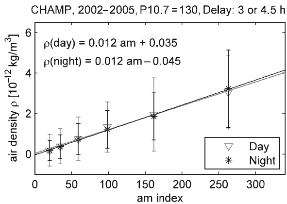
Fig. 22.3 Dependence of the low-latitude ( \pm 30^\circ lat.) mass density on magnetic activity, as represented by the index a_m . A linear fit to the medians of each bin was applied ( solid lines ). The error bars indicate the standard deviation of the values within a bin (adopted from Müller et al., 2009)
