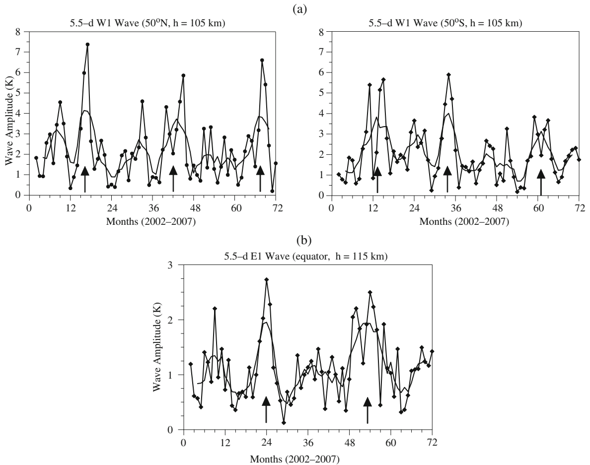
Fig. 2.14 (a) Monthly mean amplitudes of the \sim 5 -day Rossby wave at altitude of 105 km and at 50^\circ\text{N} (left plot) and 50^\circ\text{S} (right plot) drawn by thin line, while the 5-month running mean amplitudes are shown by thick line; (b) The same as (a), but for the
