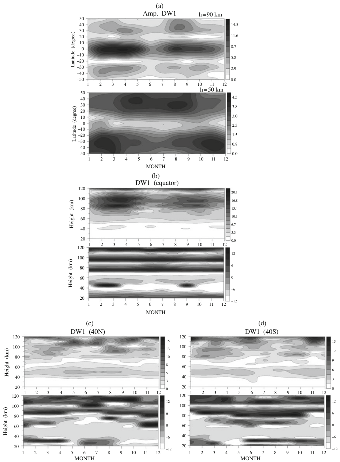
Fig. 2.1 (a) Latitude-time cross sections of DWI tidal amplitudes (in Kelvin) at altitudes of 50 km ( bottom ) and 90 km ( upper ), (b) Altitude-time cross sections of DWI amplitude ( upper ) and phase (in local time, LT) ( bottom ) at the equator, (c) The same as (b), but for 40°N, and (d) The same as (b), but for 40°S
