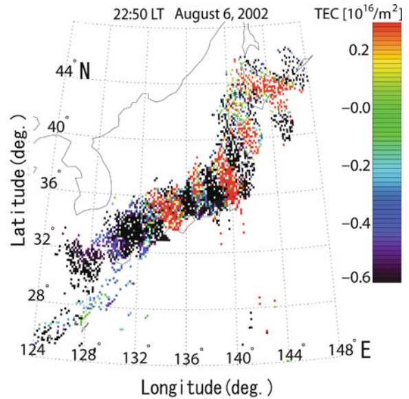
Fig. 21.1 Two-dimensional map of TEC perturbations observed with GPS network in Japan at 2250 LT on August 6, 2002
