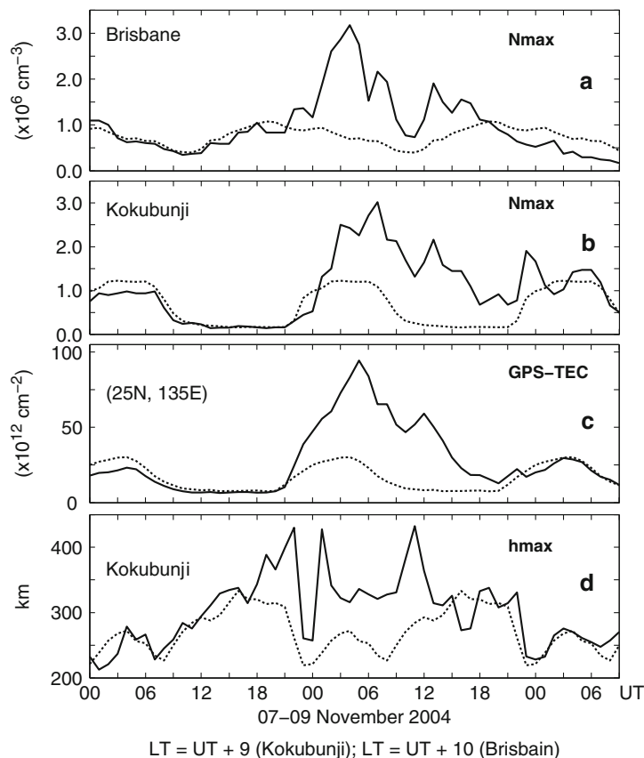
Fig. 36.6 N_{max} variations at Brisbane (153.17°E, 27.5°S; 36.7°S magnetic; LT = UT + 10, panel a ) and Kokubunji (139.5°E, 35.7°N; 26.8°N magnetic; LT = UT + 9, panel b ), and GPS-TEC close to Kokubunji ( panel c ) from 00 UT on 07 November to 09 UT on 09 November 2004 ( solid curves ); dashed curves show the seven quiet day averages prior to the storm. Panel d shows the corresponding h_{max} at Kokubunji
