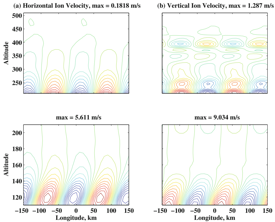
Fig. 10.11 (a) Horizontal or Zonal ( u_{ix} ) and (b) Vertical ( u_{iy} ) components of ion velocity for AGW corresponding to Case 4a at t = 50 min. In the lower (upper) panels, 110–210 km (210–510 km) altitude region are plotted
