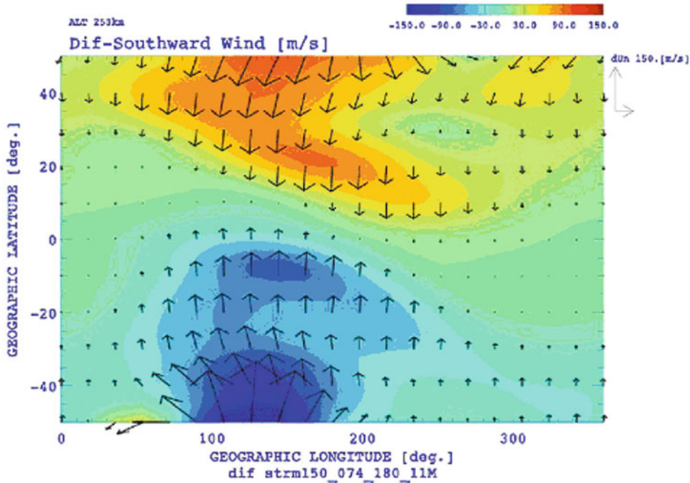
Fig. 32.4 Simulation of the response of the neutral winds at mid and low latitudes at 250 km altitude, shortly after a sudden increase in high-latitude Joule heating. The region within 50^\circ of the geographic equator is shown at 15 UT, 3 h after the increase in high latitude magnetospheric forcing, equivalent to a K_p \sim 7 .
