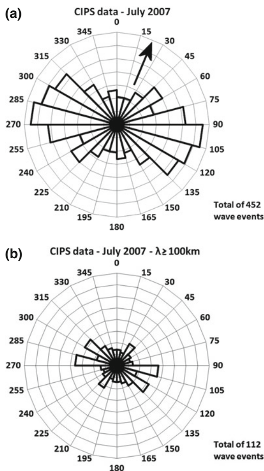
Fig. 7.8 Azimuthal distributions showing the normal direction to each wave event summed into 15° wide bins. There is a 180° ambiguity in the direction of motion of the wave events (as evident in the symmetry of these plots). All 452 wave events are shown in (a) while (b) shows directionality of the 112 wave events ( \lambda \geq 100 km). Both plots indicate marked anisotropy suggesting a strong preference for zonal wave propagation. The arrow indicates the dominant direction of motion for NLC type II bands (Pautet et al., 2010)
