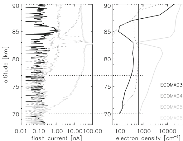
Fig. 4.6 Comparison of altitude profiles of flash currents measured during the ECOMA sounding rocket flights in summer (left panel) and corresponding electron densities from the wave propagation experiment. Dotted horizontal lines indicate altitudes with electron densities of 600 \text{ cm}^{-3} (vertical black line) for flights ECOMA04 and ECOMA06. Grey shading indicates the altitude range with ice particles. Updated from Rapp et al. (2010), copyright by the AGU
