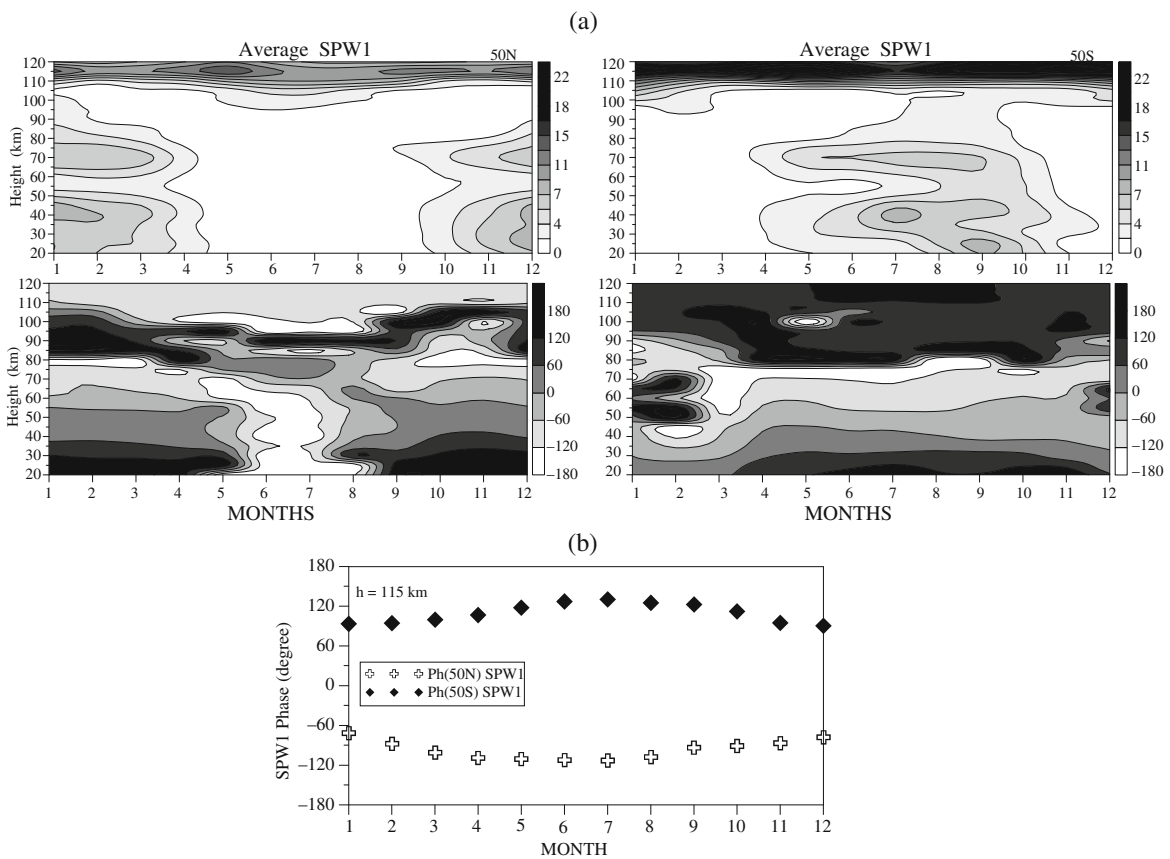
Fig. 2.10 (a) Average (2002–2007) altitude-time cross sections of SPWI at 50°N (left column) and 50°S (right column); (b) Hemispheric comparison of SPWI average phases at altitude of 115 km
