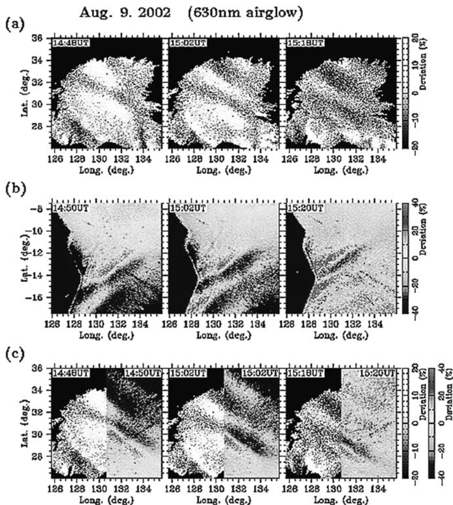
Fig. 20.1 Two-dimensional maps of 630-nm airglow intensity observed at Sata and Darwin that are geomagnetic conjugate locations [After Otsuka et al. (2004)]. (a) Sata. (b) Darwin. (c) Sata (left) and conjugate of Darwin (right)
