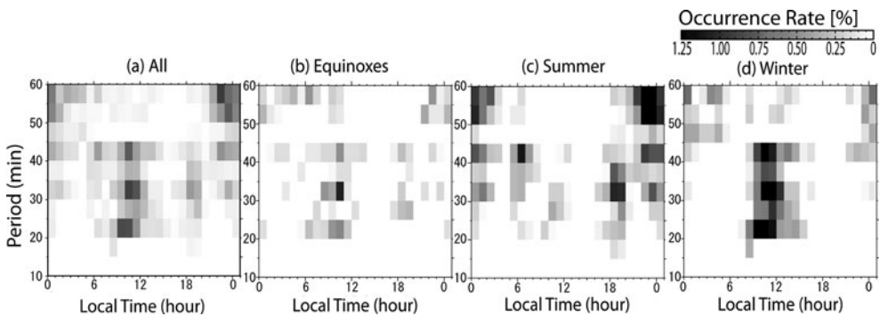
Fig. 21.5 Local time variation of period of MSTIDs observed in Japan for (a) all seasons, (b) equinoxes, (c) summer, and (d) winter
