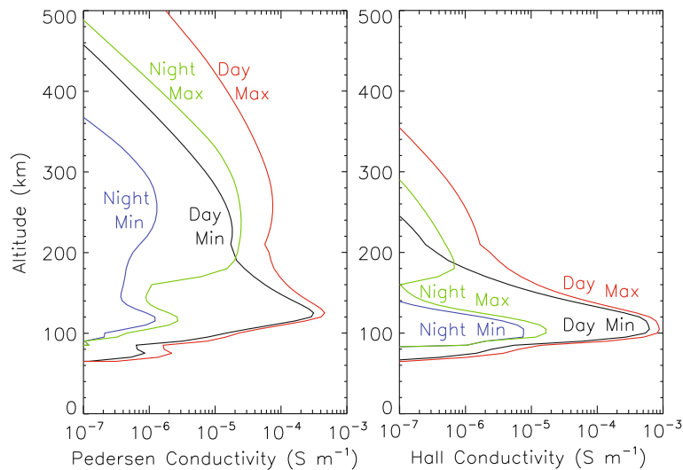
Fig. 13.1 Pedersen and Hall conductivities calculated for the location of the Arecibo radar (18.3° N, 66.75° W) for magnetically quiet equinox conditions ( A_p = 4 ), local midnight (Night) and noon (Day), for low solar activity (Min, F_{10.7} =
