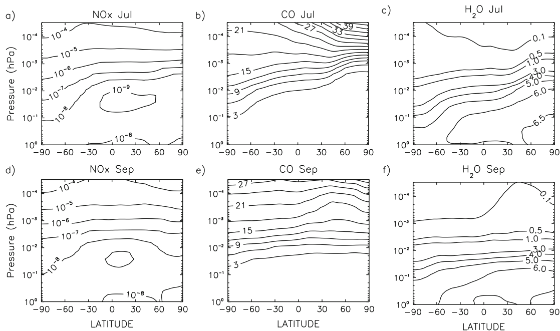
Fig. 1.5 Zonal-mean, July 2005 monthly-mean volume mixing ratios of (a) NO, (b) CO (ppm), and (c) H 2 O (ppm). (d-f) as (a-c) for September 2005
