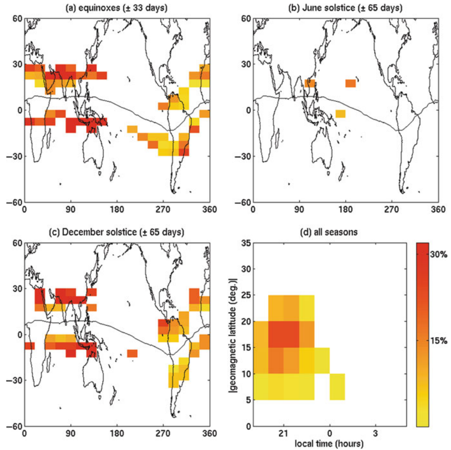
Fig. 22.12 Global distribution of NDD-to-EPB ratio separately for the different seasons (a, b, c). Panel (d) shows the NDD-to-EPB ratio as a function of geomagnetic latitude and local time (all seasons) (after Park et al., 2010)
