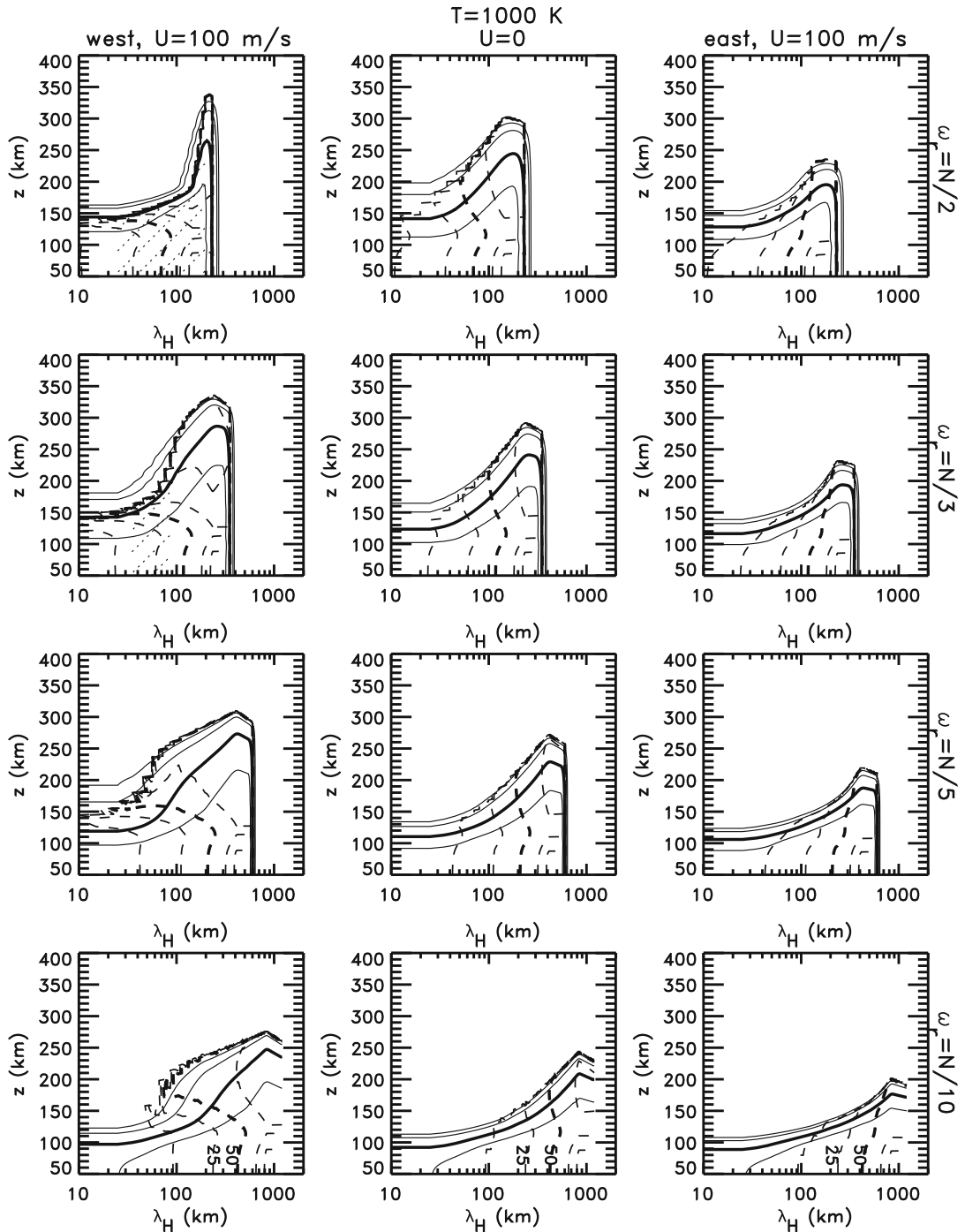
Fig. 8.2 Top panels show gravity wave penetration altitudes for horizontal wavelengths varying from 10 to \sim 1000 km for initial GW frequencies of N/2 , N/3 , N/5 , and N/10 (top to bottom, with N=0.02 \text{ s}^{-1} ) and for GW propagation against, across, and along (left to right) an eastward thermospheric wind of 100 \text{ m s}^{-1} . Bottom panels show horizontal and vertical wavelengths achieving altitudes of 150, 200, 250, and 300 km (top to bottom) for GW
