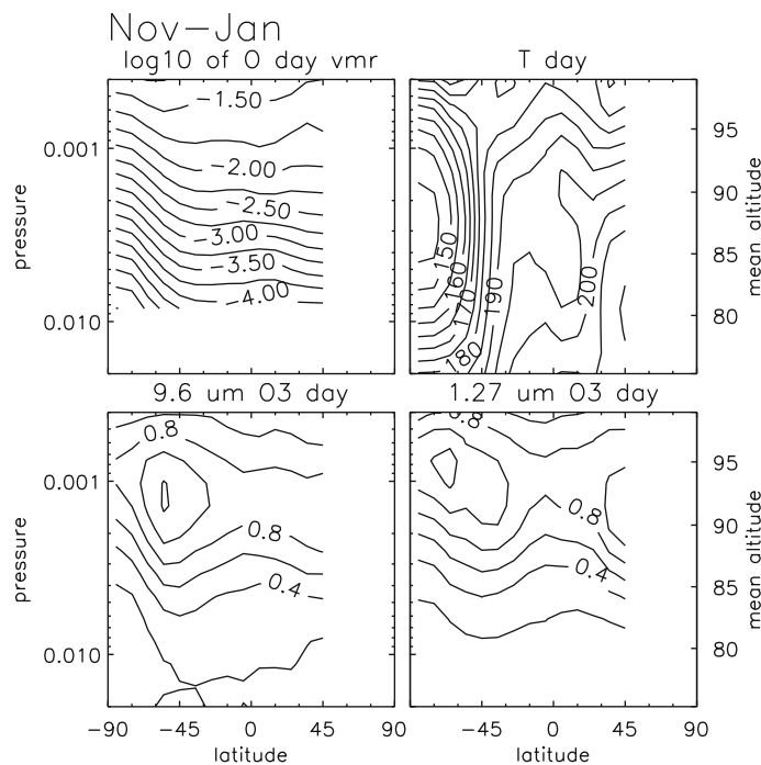
Fig. 5.1 Latitude-pressure cross-sections of the mean daytime O (log 10 of mixing ratio), T (K), and O_3 (mixing ratio in ppm) from two independent retrievals averaged over 8 years for the period mid-November to mid-January
