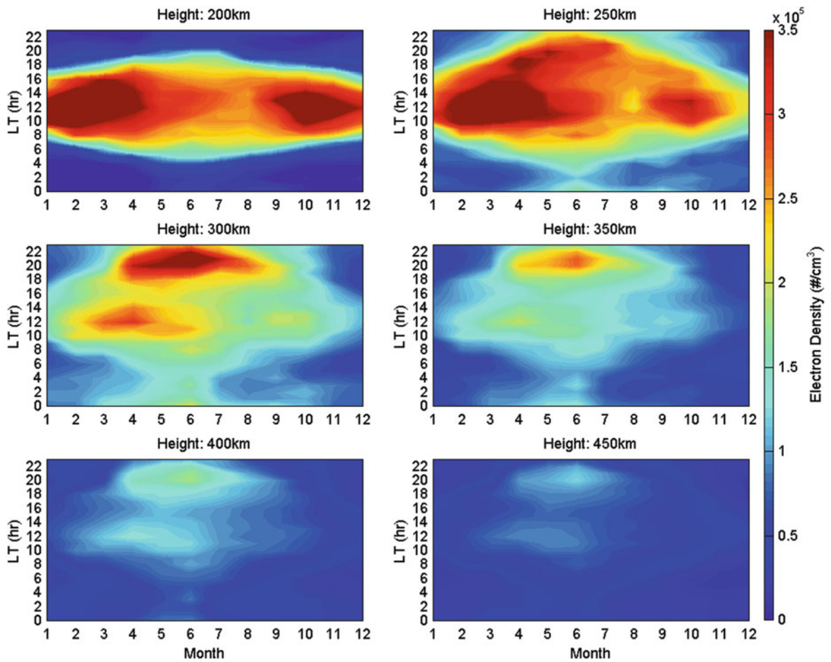
Fig. 27.7 Local time variations of the electron density at (52^{\circ}\text{N}, 104^{\circ}\text{E}) in geographic coordinate) at various altitudes in each month of 2007. This figure indicates that the northern MSNA occurs from April to September
