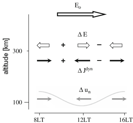
Fig. 26.9 Schematic diagram for the generation of the perturbation electric field by zonal winds (Jin et al., 2008)
