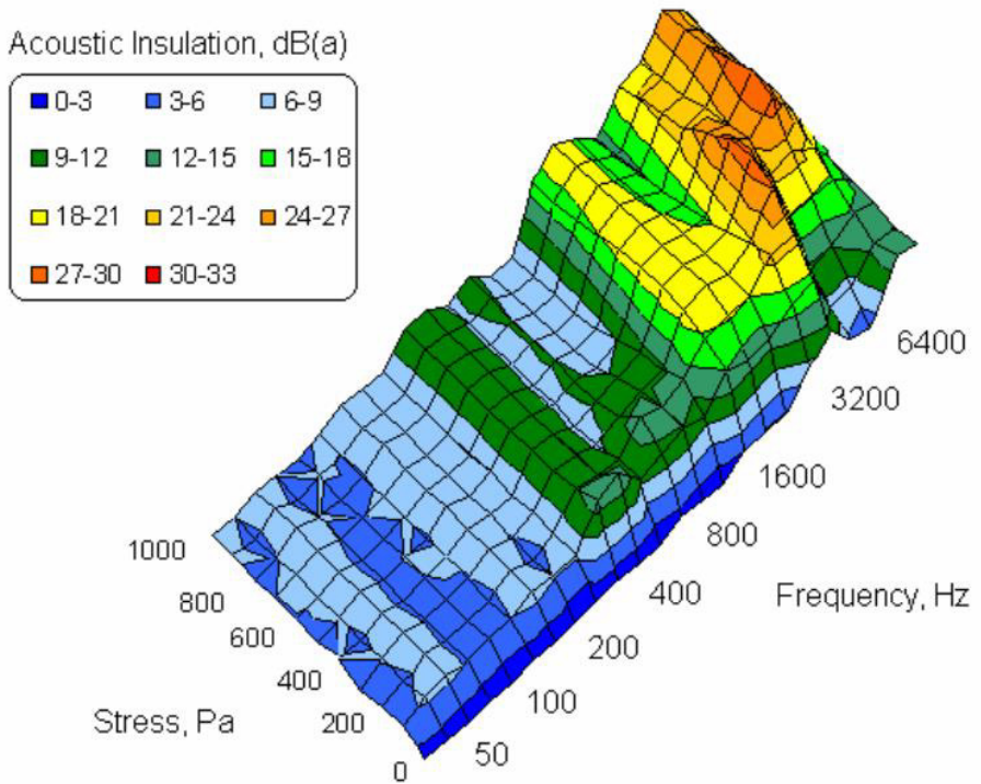
Fig. 7. Sound reduction index of foamed polyurethane under low-pressure.
