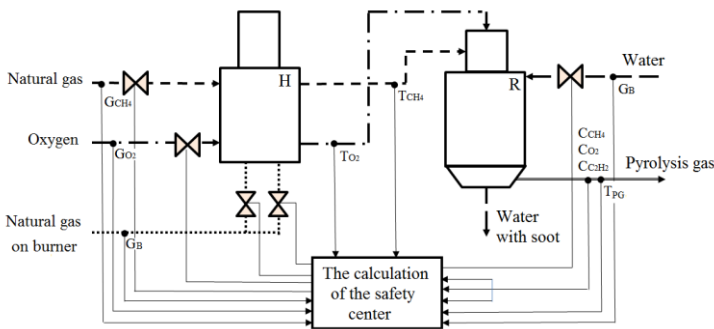
Fig. 2. The control system of acetylene receiving process
