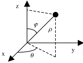
Figure 2-2. The spherical coordinate system
