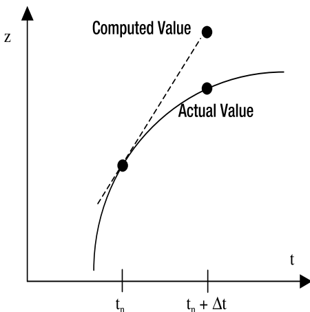
Figure 4-4. Euler's method is inaccurate if the curve is not linear.
