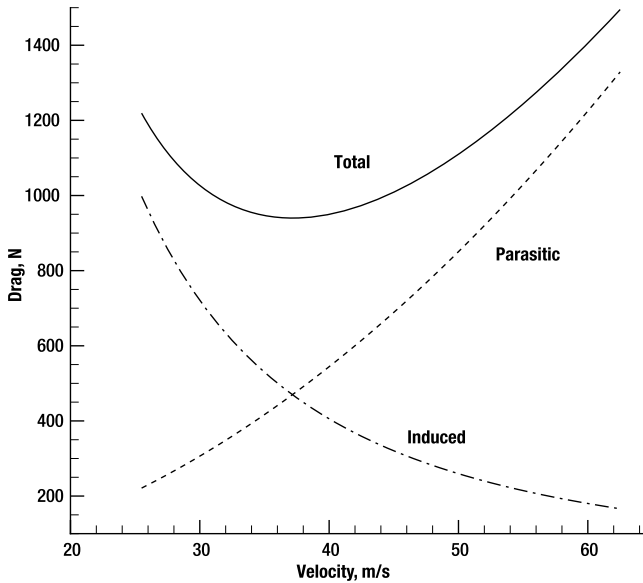
Figure 10-19. Straight-and-level drag profiles for the Cessna 172 Skyhawk
