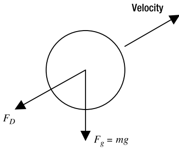
Figure 5-7. The force diagram with gravity and drag effects
