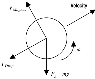
Figure 5-15. The projectile force diagram including gravity, drag, and Magnus force
