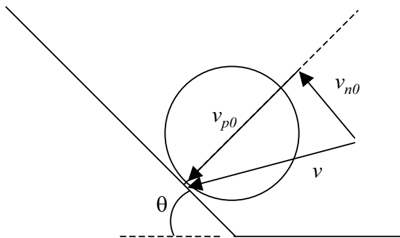
Figure 6-14. A general, two-dimensional oblique collision
