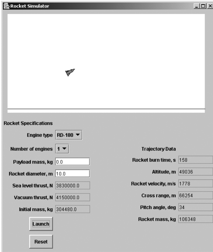
Figure 11-7. A typical Rocket Simulator screen shot
