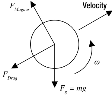
Figure 7-6. Force diagram for a golf ball in flight
