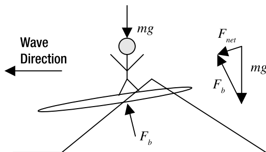
Figure 9-15. When a surfer catches a wave, a net force pushes the surfboard forward.
