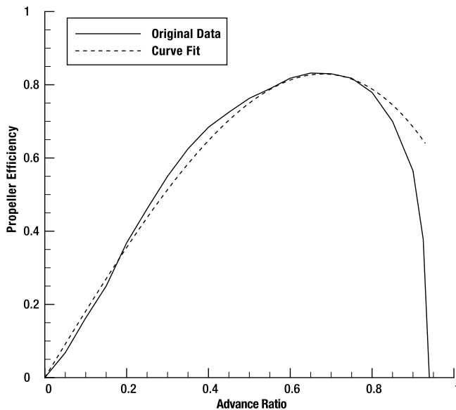
Figure 10-14. Original and curve fit values of propeller efficiency
