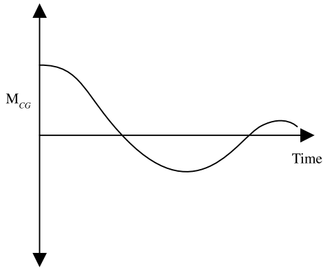
Figure 10-32. A plane is dynamically stable if deviations from the equilibrium orientation die out over time.
