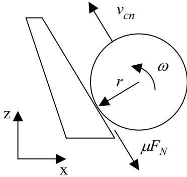
Figure 7-5. Friction between the ball and club face causes the ball to spin.
