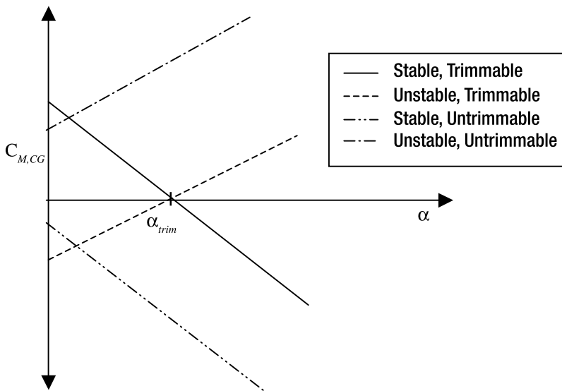
Figure 10-31. The four stability trim possibilities
