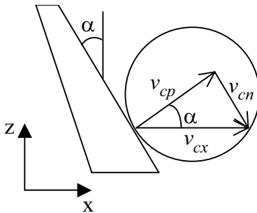
Figure 7-4. Schematic of a club head—golf ball collision
