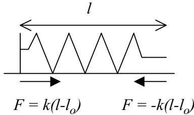
Figure 3-7. A spring exerts an equal and opposite restoring force when deflected.
