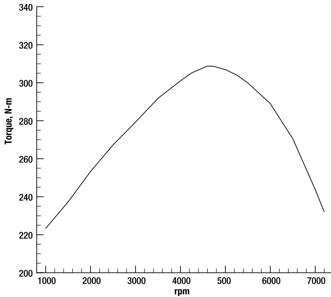
Figure 8-2. A typical torque curve
