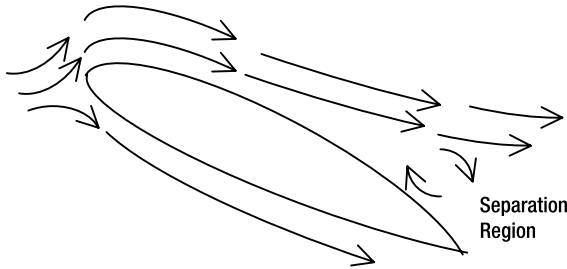
Figure 10-9. Flow separation reduces the lift generated by an airfoil.
