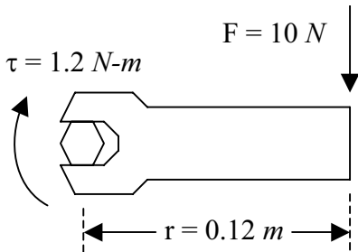
Figure 4-8. Force applied at a distance from an axis of rotation generates a torque.
