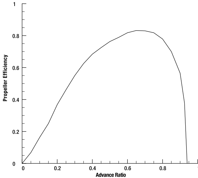
Figure 10-13. Propeller efficiency coefficient, McCauley 7557 propeller
