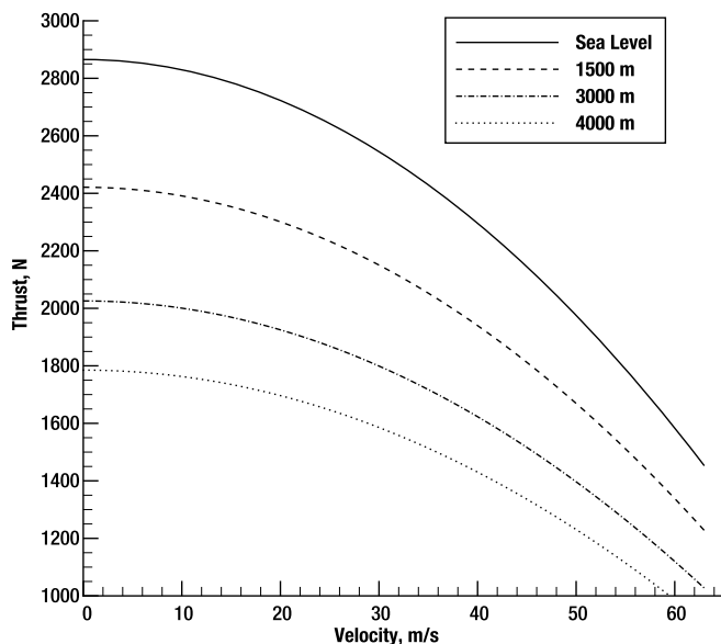
Figure 10-16. Computed thrust profiles for the Cessna 172 Skyhawk
