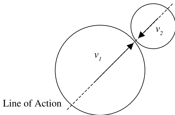
Figure 6-12. Velocity and line of action are in the same direction for direct impact collisions.
