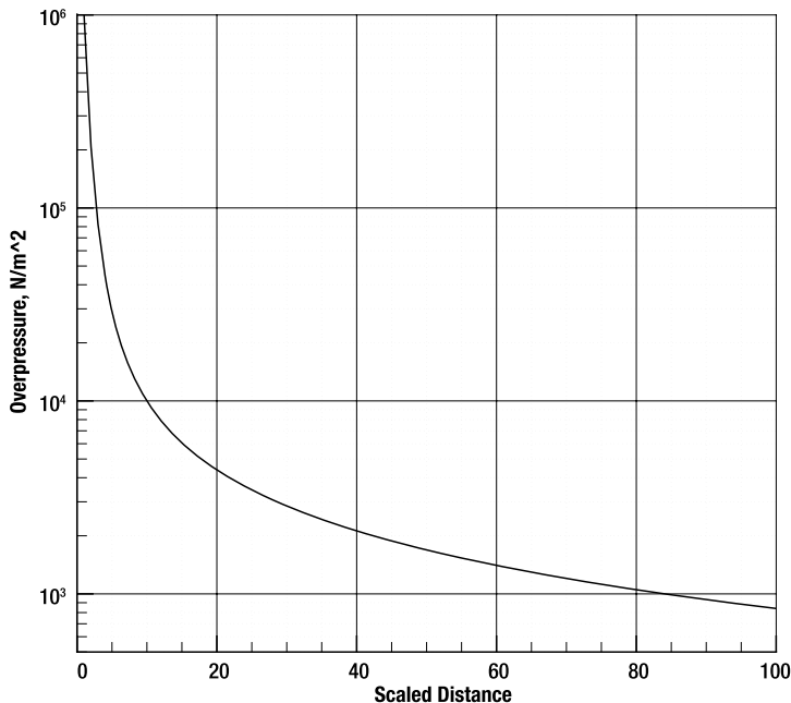
Figure 13-2. Overpressure as a function of scaled distance, TNT explosion
