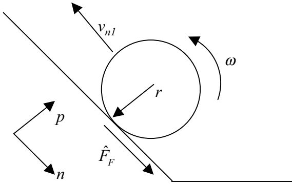
Figure 6-15. A frictional impulse causes a rotation.
