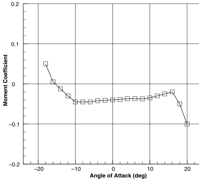
Figure 10-26. Moment coefficient data for the NACA 2412 airfoil
