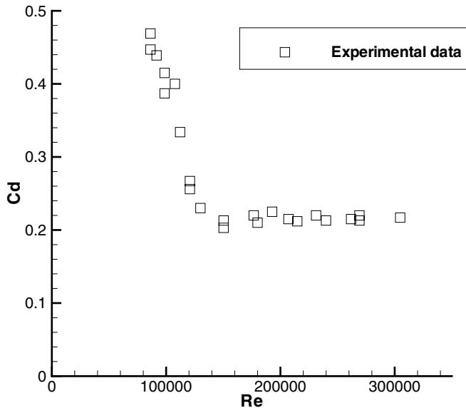
Figure 7-13. Drag coefficient of a nonspinning soccer ball
