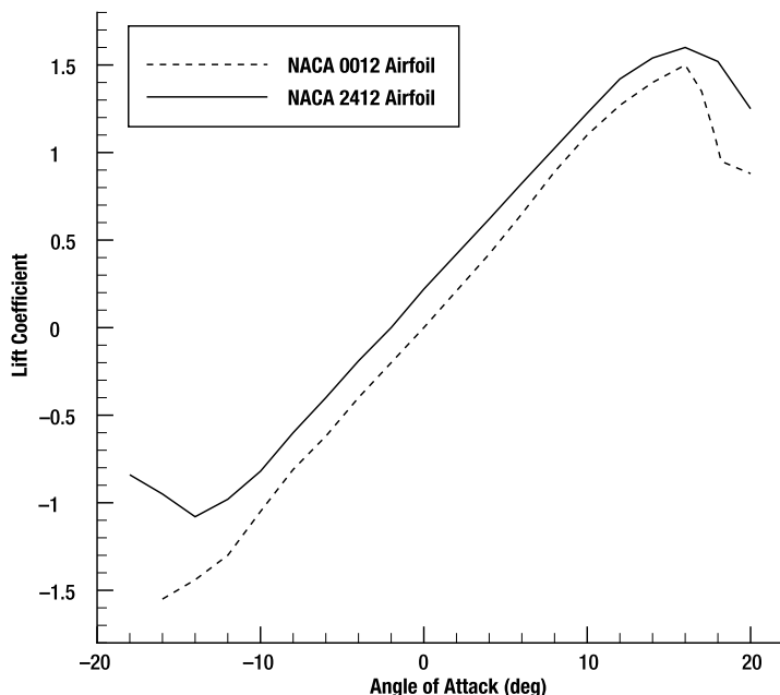
Figure 10-8. Lift coefficient data for the NACA 0012 and 2412 airfoils
