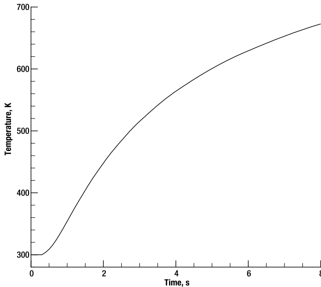
Figure 12-5. Time-varying temperature profiles at the inner wall of an aluminum gas tank. Tank thickness = 0.025\text{ m} . Outer wall temperature = 1000\text{ K} .
