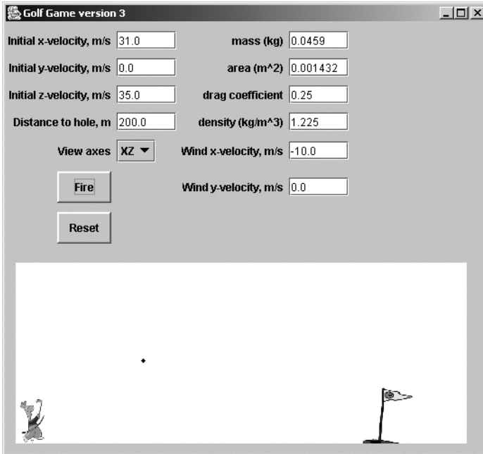
Figure 5-11. A typical Golf Game version 3 screen shot
