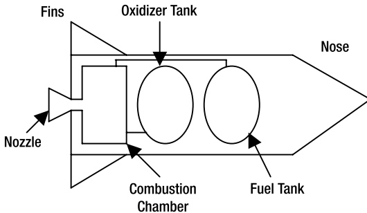
Figure 11-2. A cross section of a liquid-propellant rocket
