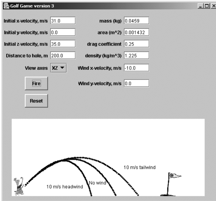
Figure 5-12. The effects of headwind or tailwind on a golf ball trajectory
