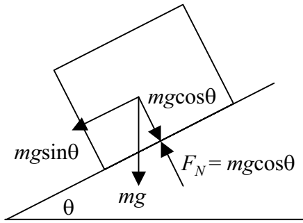
Figure 3-3. Normal force on a box resting on an inclined ramp
