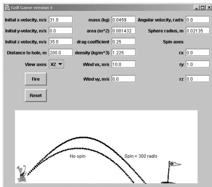
Figure 5-17. The effect of spin on golf ball flight
