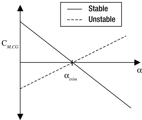
Figure 10-30. Stability depends on the slope of the moment-angle of attack curve.
