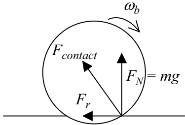
Figure 7-11. The contact force on a rolling object acts slightly forward of the center of gravity.
