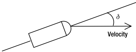
Figure 5-19. Bullets usually have a yaw angle during flight.
