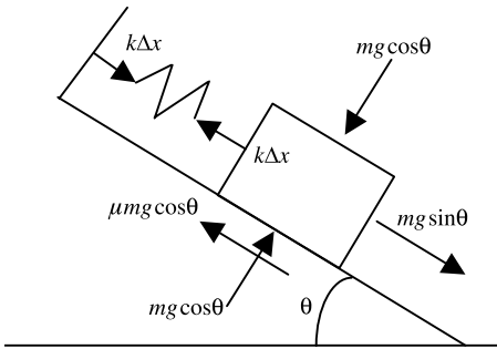
Figure 3-10. The force diagram for the box on a ramp
