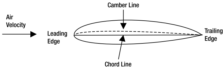
Figure 10-4. An airfoil schematic
