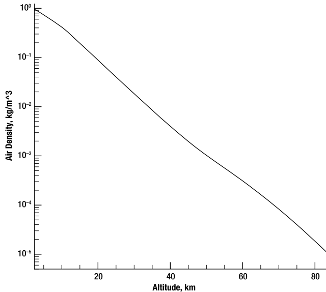
Figure 11-5. Variation of atmospheric density with altitude
