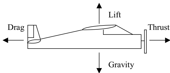
Figure 10-3. Basic force diagram for an airplane
