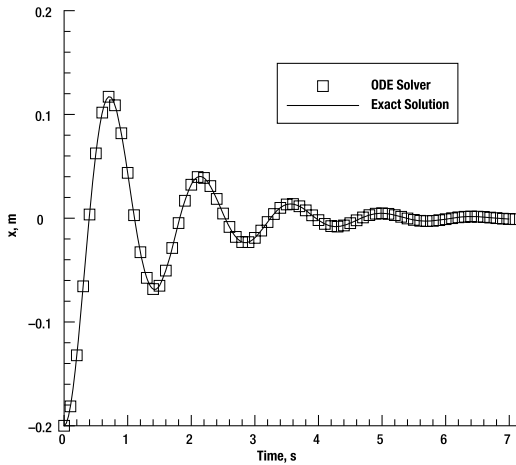
Figure 4-5. Spring location as a function of time
