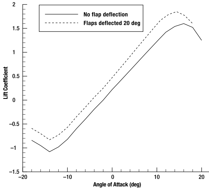
Figure 10-11. The effect of flap deflection on lift coefficient
