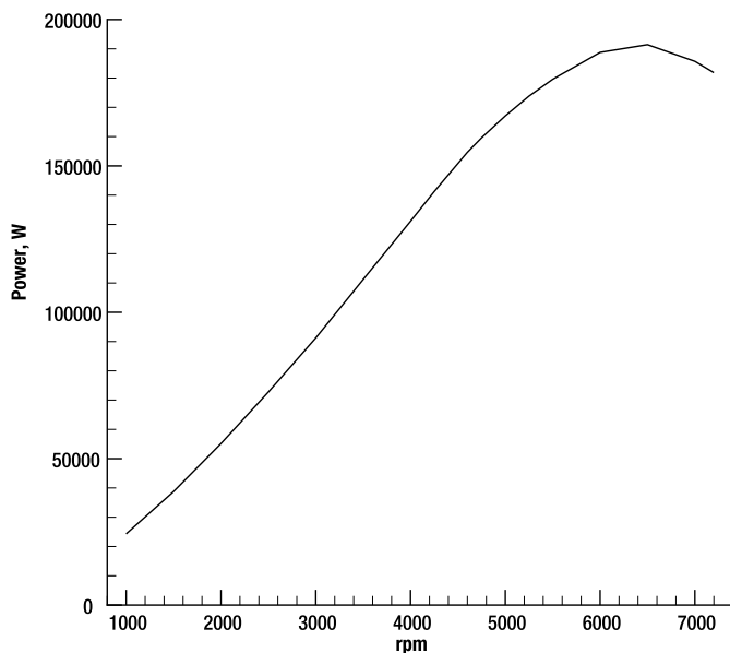
Figure 8-4. The power curve for the 2004 Boxster S
