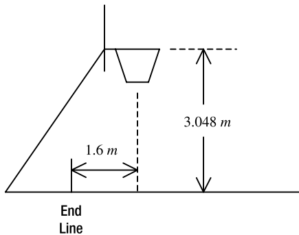
Figure 7-19. Basket and backboard schematics
