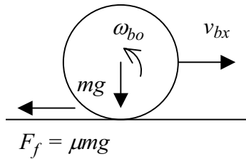
Figure 7-10. The forces and velocities at the beginning of the skid phase
