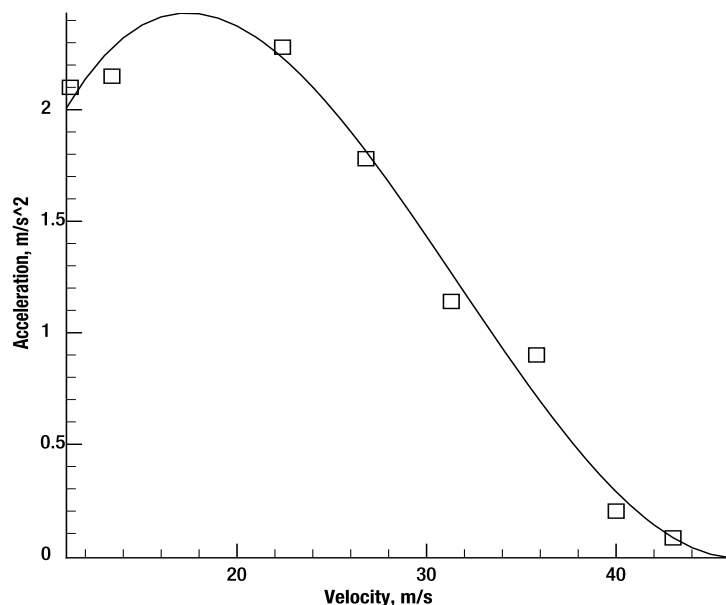
Figure 9-8. Acceleration profile for the Fountain Lightning
