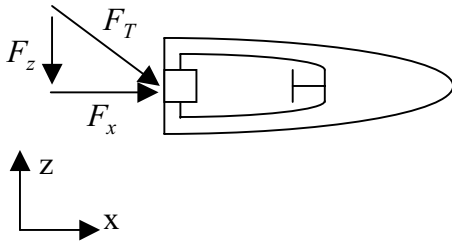
Figure 9-10. Rotating the thrust force vector creates a torque that turns the boat.
