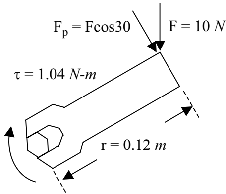
Figure 4-9. If force is applied at an angle to the moment arm, torque is reduced.
