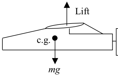
Figure 10-27. Lift from the wing generates a moment about the c.g. of the airplane.
