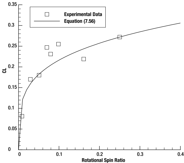
Figure 7-15. Experimental and computed soccer ball lift coefficients
