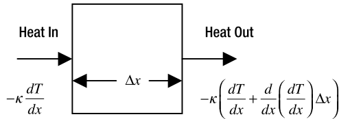
Figure 12-2. A heat conduction energy balance
