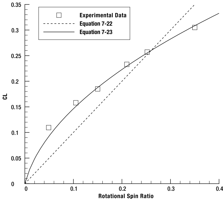
Figure 7-7. Experimental and computed lift coefficients for a standard golf ball
