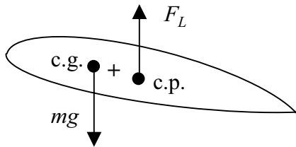
Figure 10-25. Gravitational and lift forces can generate a moment.
