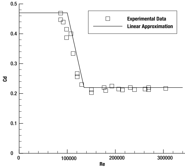
Figure 7-14. A linear approximation to soccer drag coefficient data
