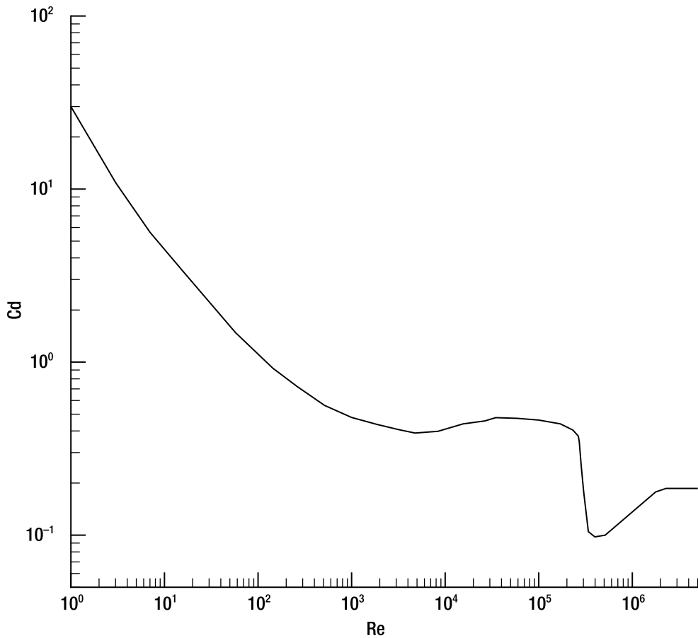
Figure 5-6. The drag coefficient of a sphere as a function of Reynolds number
