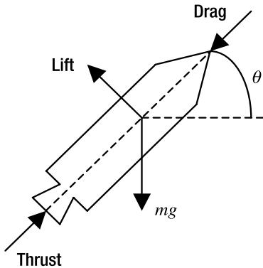
Figure 11-3. A rocket during ascent experiences thrust, drag, lift, and gravity forces.
