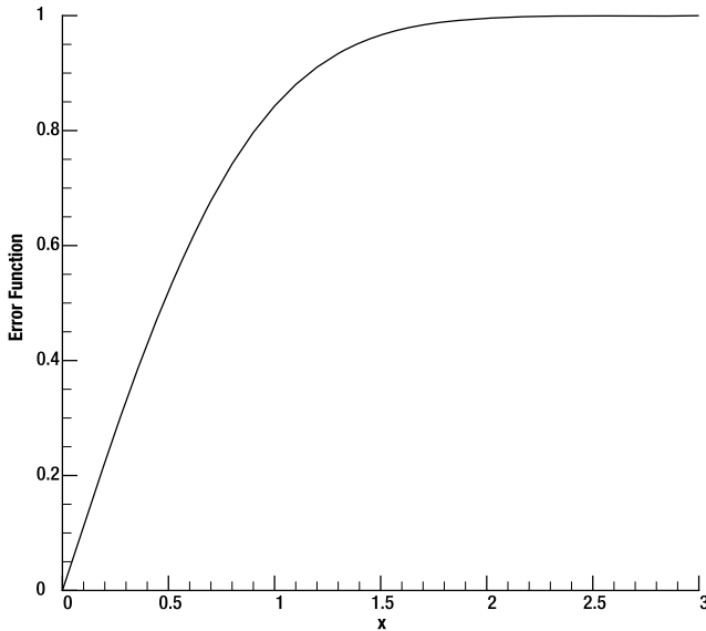
Figure 12-3. The error function profile
