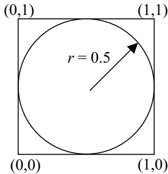
Figure 15-8. To compute the value of \pi , start with a circle inside a box.
