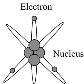
Figure 14-1. A schematic of a typical atom
