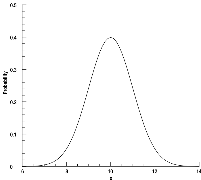
Figure 15-1. A typical probability function
