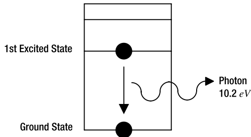
Figure 14-4. When an electron transitions to a lower energy state, it emits a photon.
