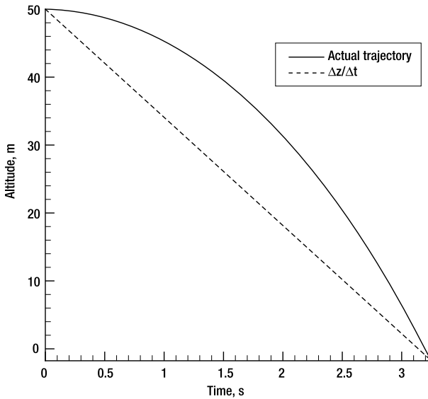
Figure 2-7. \Delta z/\Delta t does not accurately predict the rate of fall at a given time.
