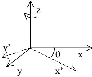
Figure 2-4. A coordinate axes rotation about the z-axis
