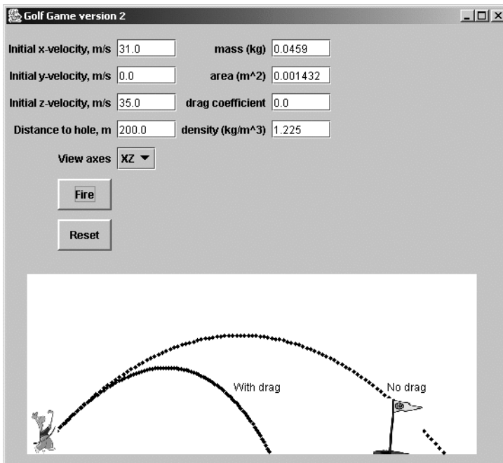
Figure 5-9. The effect of drag on the flight of a golf ball
