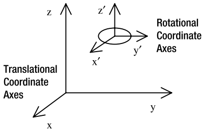
Figure 4-12. The six coordinate axes for analyzing rigid body motion
