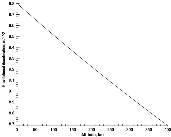
Figure 11-4. Gravitational acceleration as a function of altitude
