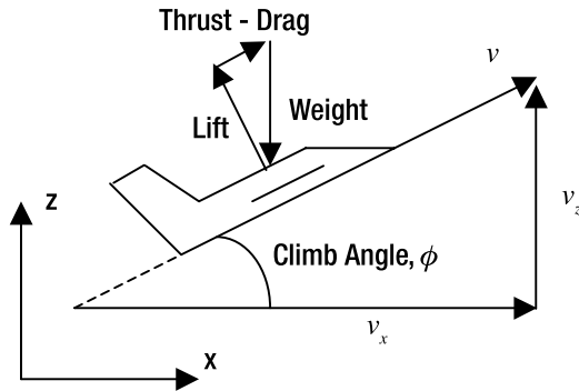
Figure 10-20. Force diagram for an airplane that is climbing
