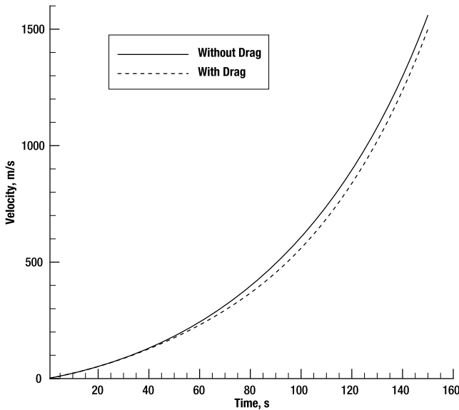
Figure 11-6. Saturn 1B velocity profiles with and without drag
