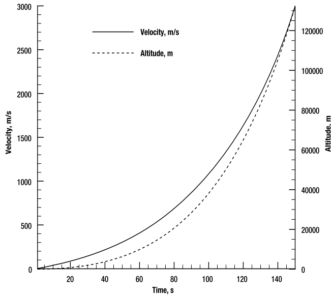
Figure 11-8. Velocity profile for vertical ascent simulation
