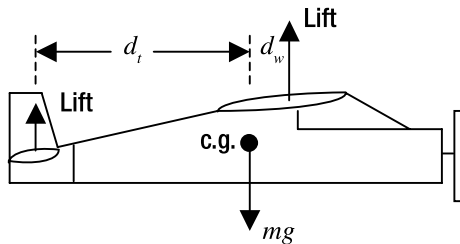
Figure 10-28. A counterbalancing moment is generated by the horizontal stabilizer.
