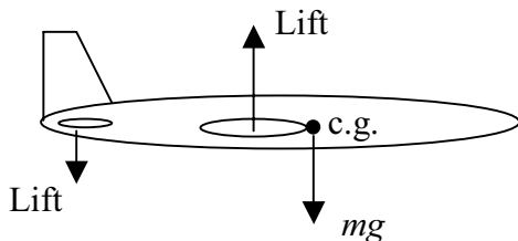
Figure 10-29. To create the proper counterbalancing moment, sometimes the horizontal stabilizer lift must be negative.
