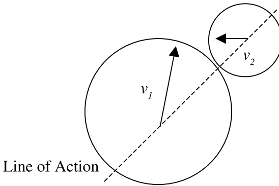
Figure 6-13. Velocity doesn't line up with line of action for oblique impacts.
