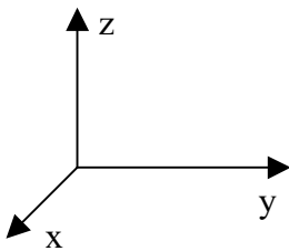
Figure 2-1. The Cartesian coordinate system
