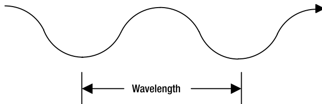
Figure 14-5. Every photon will have a wavelength.
