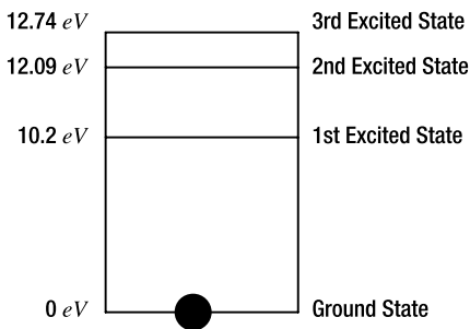
Figure 14-2. Energy levels for hydrogen atom electrons
