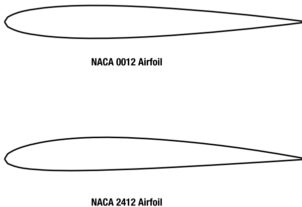
Figure 10-7. The shapes of the NACA 0012 and 2412 airfoils
