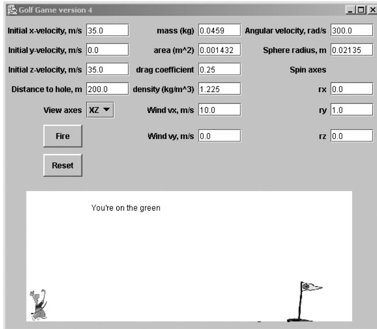
Figure 5-16. A typical Golf Game version 4 screen shot
