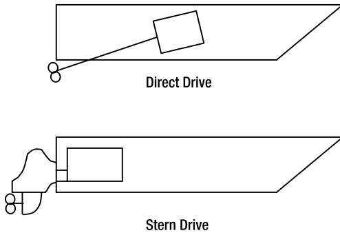
Figure 9-5. Drive system types
