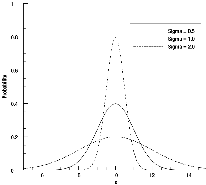
Figure 15-4. The effect of standard deviation on the Gaussian distribution curve
