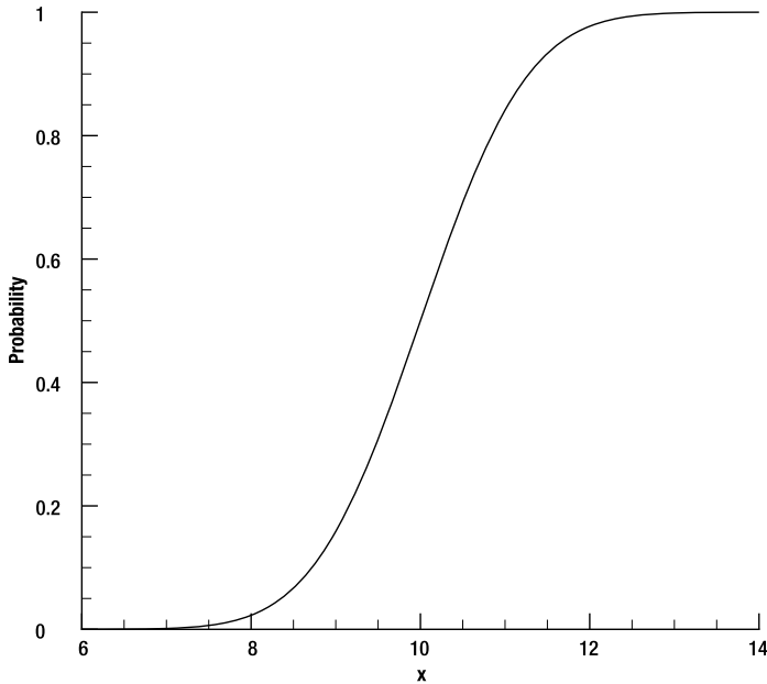
Figure 15-2. A typical cumulative distribution function
