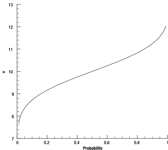
Figure 15-3. An inverse cumulative distribution function
