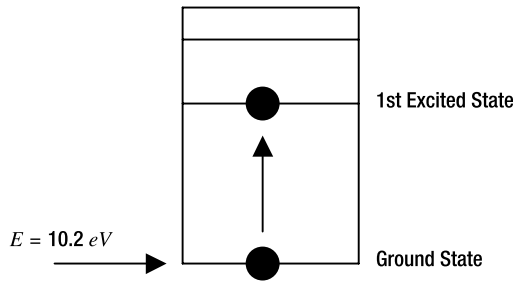
Figure 14-3. When an atom absorbs energy, one of its electrons can move to a higher energy state.
