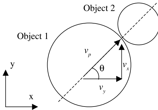
Figure 6-6. A general two-dimensional collision
