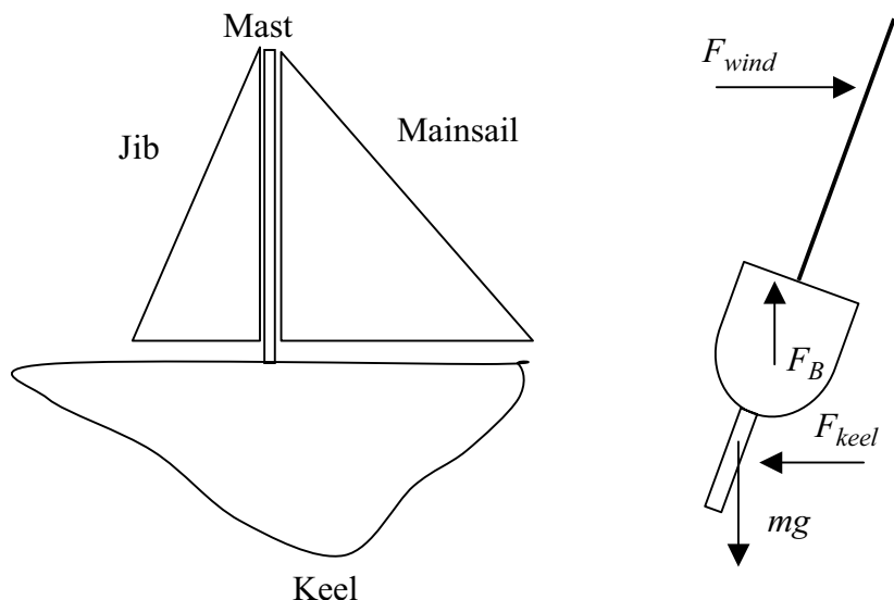
Figure 9-12. A schematic of a typical sailboat
