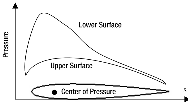
Figure 10-12. A typical surface pressure distribution
