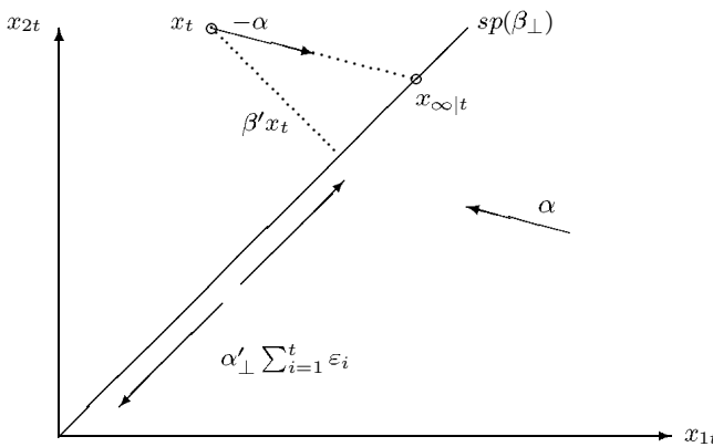
Fig. 1 In the model \Delta x_t = \alpha\beta'x_{t-1} + \varepsilon_t , the point x_t = (x_{1t}, x_{2t}) is moved towards the long-run value x_{\infty|t} on the attractor set \{x|\beta'x = 0\} = sp\{\beta_{\perp}\} by the forces -\alpha or +\alpha , and pushed along the attractor set by the common trends \alpha'_{\perp} \sum_{i=1}^t \varepsilon_i .
