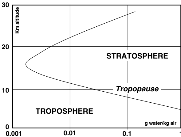
Figure 4.24. Average water vapour in the atmosphere as a function of altitude (Junge, 1963)
