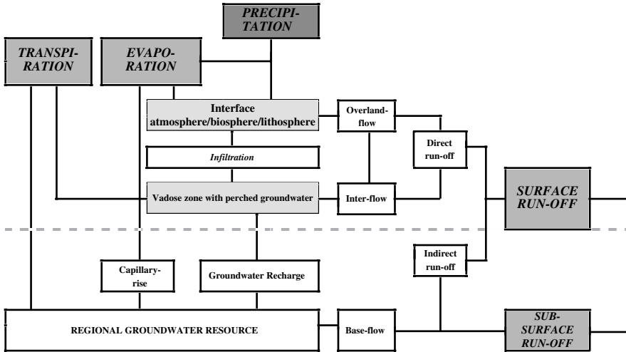
Figure 3.1. Transformations of the input (dark grey) to the output (medium grey) in the continental water cycle. Transformation paths above the broken line are dominant in arid and cold climates. Light grey: main transformation compartments
