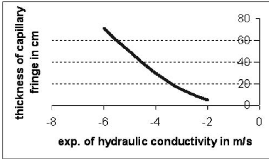
Figure 4.6. Thickness of the capillary fringe as a function of the hydraulic conductivity of unconsolidated rocks
