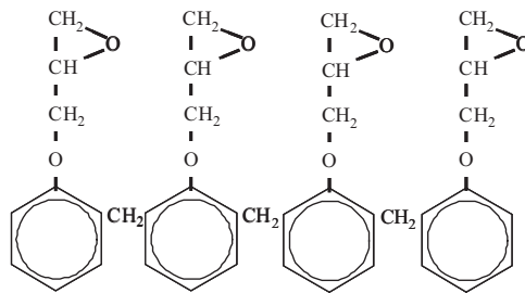
Figure 2.21. Representative structure of epoxy novolac resin.
