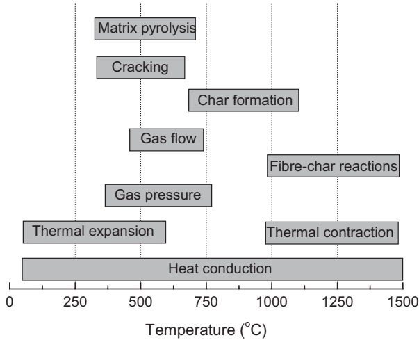
Figure 5.1. Effect of temperature on the various responses of a fibreglass composite. (The temperatures are approximate, and will vary with the composition of the material and fire conditions).
