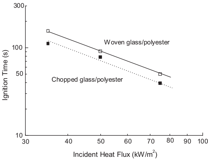
Figure 3.5. Effect of heat flux on the ignition times of polyester laminates reinforced with woven glass or chopped glass fibres. Data from Brown and Mathys [15].
