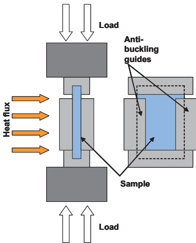
Figure 6.16. Restrained compression test. (a) Schematic of picture frame restraint jig and (b) propane burner test on a polymer laminate under compression.
