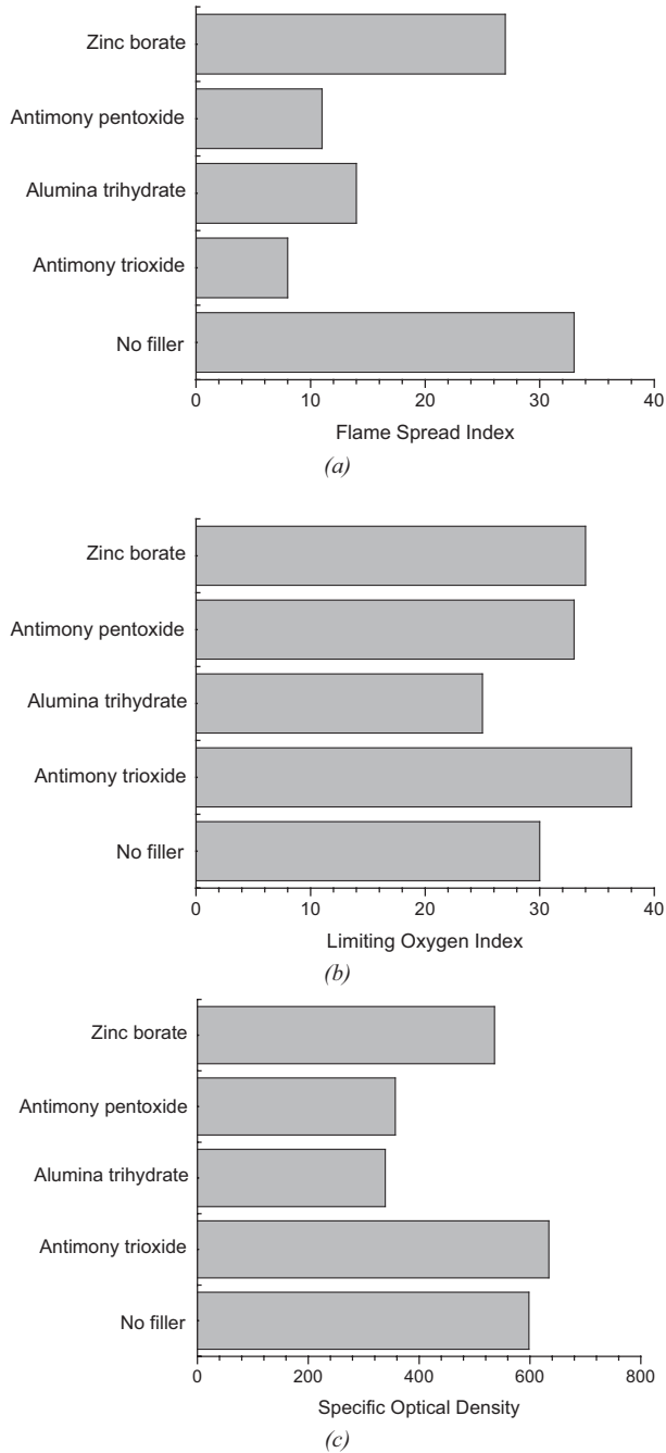
Figure 8.16. Effect of flame retardant fillers on the (a) flame spread index, (b) limiting oxygen index and (c) specific optical density of a brominated vinyl ester. Data from Morchat and Hiltz [33].
