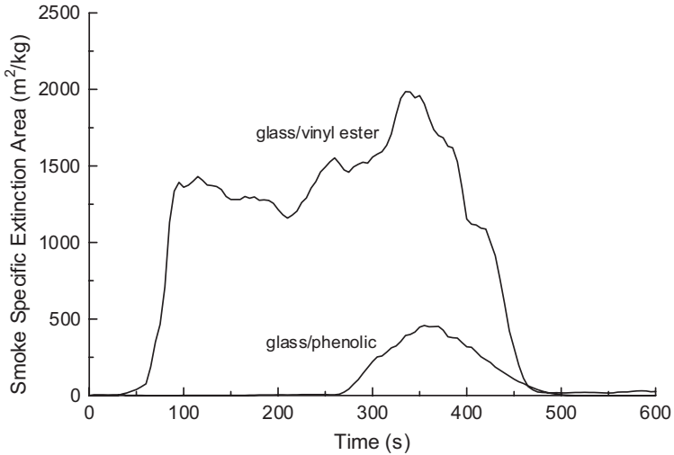
Figure 3.23. Smoke generation (specific extinction area) versus time for glass/vinyl ester and glass/phenolic composites tested at the heat flux of 50 \text{ kW/m}^2 .
