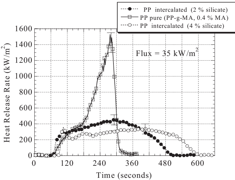
Figure 9.5. Comparison of the heat release rate (HRR) plots for pure PP-g-MA and two PP-g-MA-layered-silicate nanocomposites, at 35\text{ kW/m}^2 heat flux, showing a 70-80% reduction in peak HRR for the nanocomposites with a mass fraction of only 2% or 4% layered silicate, respectively. (Reprinted with permission from Chem. Mater. 12, 2000, 1866-1873 copyright 2000 American Chemical Society).
