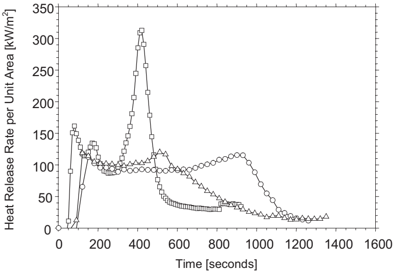
Figure 4.10. Heat release rate per unit area from plywood ( \square ), E-Glass FR vinyl ester (O), and E-Glass FR vinyl ester sandwich composite with a balsa core ( \Delta ) using the cone calorimeter with a heater incident heat flux of 50 \text{ kW/m}^2 . Data from Lattimer and Sorathia [24].
