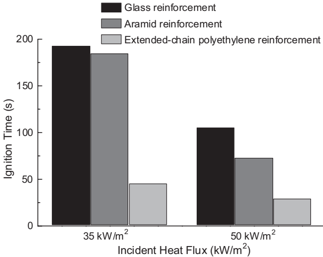
Figure 3.6. Effect of heat flux on the ignition times of vinyl ester-based laminates containing glass, aramid or extended chain polyethylene fibres. Data for the glass laminate from Brown and Mathys [15] and for the aramid and polyethylene reinforced composites from Brown et al. [9].
