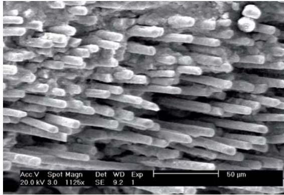
Figure 7.6. Microstructure of the char in a thermoset laminate following a fire.
