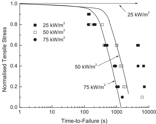
Figure 6.23. Comparison of the calculated and measured times for a woven glass/vinyl ester laminate under tensile loading and one-sided heat flux. The curves were calculated using the two-layer model.
