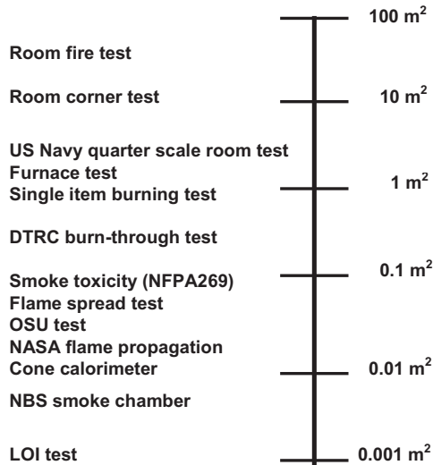
Figure 11.1. Range of specimen sizes of various fire test methods used to measure the fire reaction and fire resistive properties of materials.
