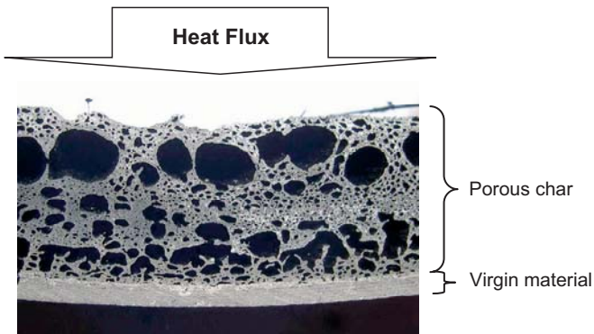
Figure 2.33. Section of a fire-damaged carbon/epoxy laminate showing a porous char structure.
