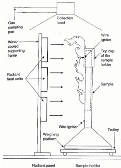
Figure 11.5. Schematic of the intermediate-scale cone calorimeter. Reproduced with permission from Babrauskas [23].
