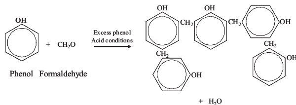
Figure 2.24. Phenolic Novolac-type resin preparation, showing an indicative structure.
