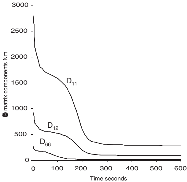
Figure 6.25. Laminate model for a glass/vinyl ester laminate: predicted variation of the components of the laminate A , B and D matrices with time for a heat flux of 75 \text{ kW/m}^2 . (a) A , (b) B and (c) D matrix components.
