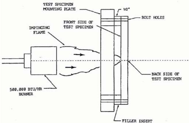
Figure 11.11. Schematic of the DTRC Burn-Through test. Reproduced with permission from Greene [25].
