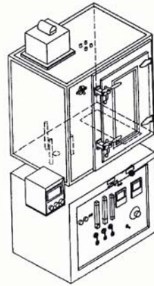
Figure 11.9. General view and schematic diagram of the N.B.S. smoke chamber. The photograph and diagram is reproduced with permission from Fire Testing Technology Ltd. and Greene [25], respectively.
