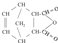
Figure 2.11. Nadic anhydride.
