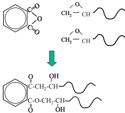
Figure 2.20. Epoxy resins: anhydride cure- simplified reaction.
