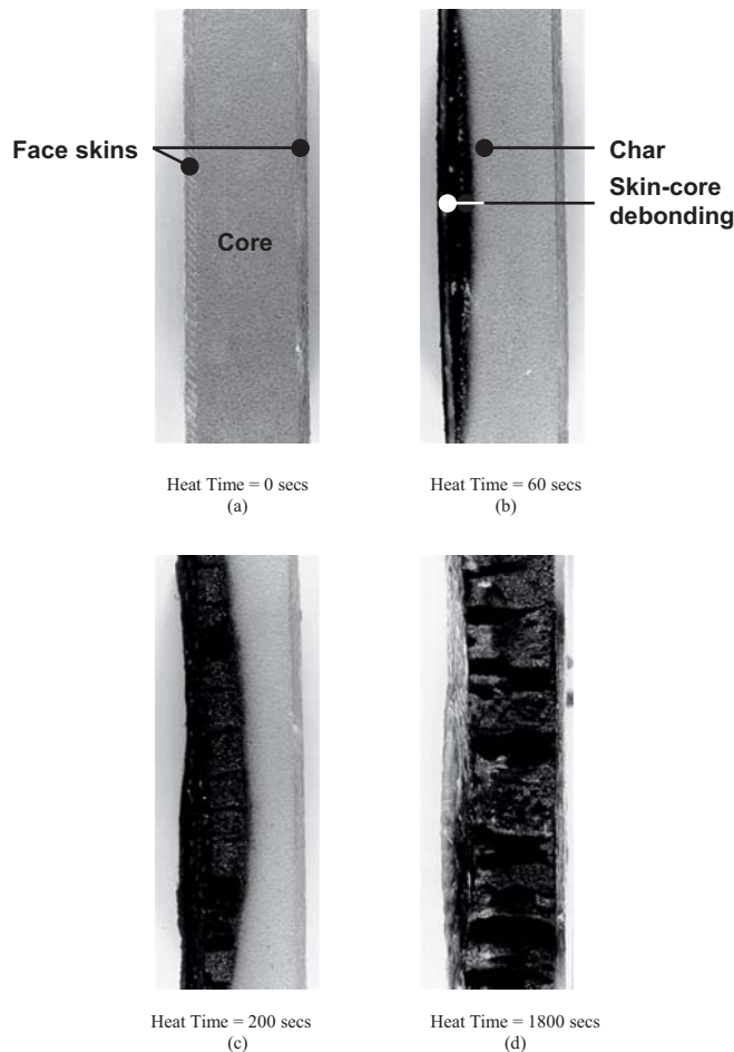
Figure 2.31. Section of a fire-damaged sandwich composite showing the different damage zones. The composite was exposed to a heat flux of 50 \text{ kW/m}^2 for different times.
