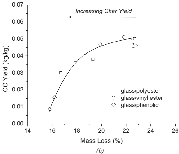
Figure 12.2. Relationship between mass loss and CO yield for several (a) thermoset polymers and (b) woven glass/thermoset polymer composites. Data from Brown et al. [33].
