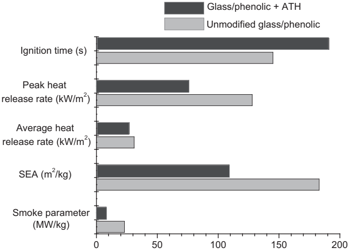
Figure 8.5. Effect of ATH filler on the fire reaction properties of a glass/phenolic composite tested at an incident heat flux of 50 kW/m 2 . Data from Scudamore [12].
