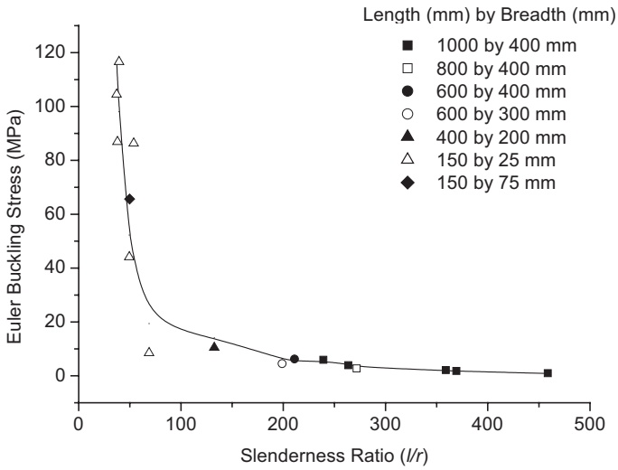
Figure 7.15. Euler buckling strength as a function of slenderness ratio for various size glass/polyester plates and beams following exposure to a fuel fire. The solid line is the model calculation. Data from Gardiner et al. [18].
