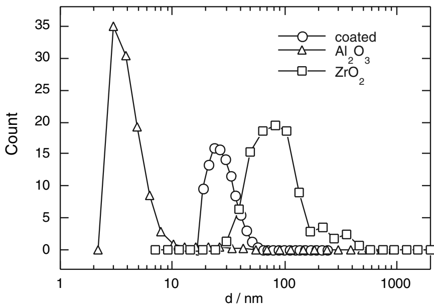
FIGURE 3 Size distribution of dispersions of the pure oxides \text{ZrO}_2 and \text{Al}_2\text{O}_3 in water. Note the improvement of the size distribution of \text{ZrO}_2 coated with a thin layer of \text{Al}_2\text{O}_3 . The alumina nanoparticles can be dispersed to the size of the dry as prepared powder. SOURCE: Möller, 2000.
