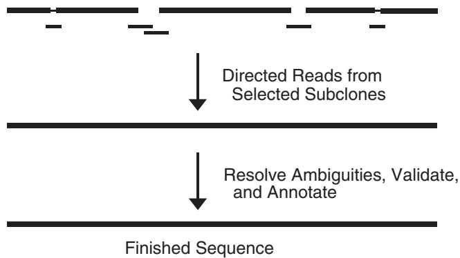
FIGURE 3 Shotgun DNA sequencing. The dominant genomic sequencing strategy being used in the Human Genome Project is shotgun sequencing, which consists of two major phases. In the first random shotgun phase a genomic clone (e.g., BAC) is subcloned into approximately 2 kb fragments. Sequence reads are then obtained from one or both ends of a large number of randomly selected subclones. Sufficient sequence data are generated such that each base of the starting clone is read, on average, about 6 to 10 times. These redundant sequence data are then analyzed with various computational tools, allowing the assembly of sequence contigs. Typically, only a handful of gaps between sequence contigs and other problems (e.g., low-quality regions) remain at this stage. In the second directed finishing phase, additional data are generated to complete the sequence, most often by obtaining directed reads from strategically selected subclones. This usually allows the merger of the remaining sequence contigs and the refinement of any low-quality regions to yield a final contiguous, high-accuracy (i.e., finished) sequence. SOURCE: Reprinted with permission from The McGraw-Hill Companies (Green, 2001).
