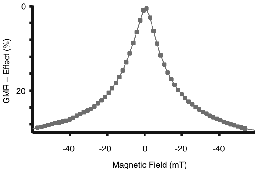
FIGURE 1 Change of the normalized electrical resistance (GMR effect) as a function of the magnetic field for a granular thin film of silver/cobalt prepared by molecular beam epitaxy. SOURCE: Aloff, 2000.
