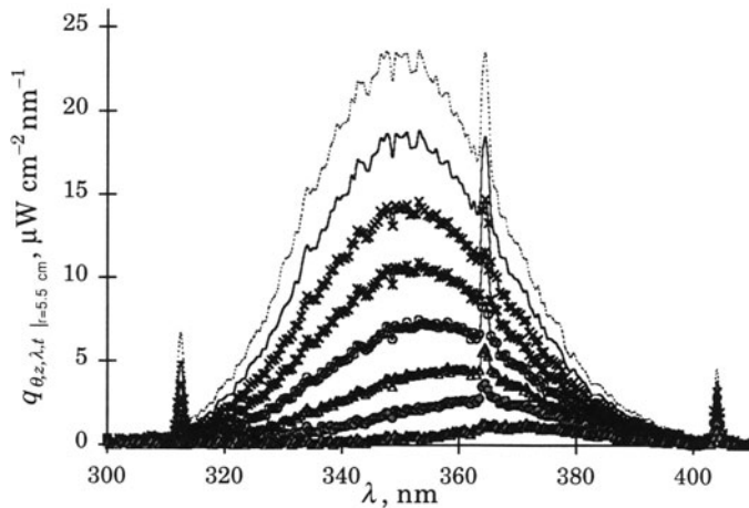
FIGURE 4.32. Transmission spectrum 5.5 cm from the lamp surface for several Hombikat UV-100 concentrations in g L^{-1} . (---) 0.0, (—) 0.017, (×) 0.033, (*) 0.05, (o) 0.075, ( \Delta ) 0.108, (●) 0.150, and (black \Delta ) 0.258 (Reprinted with permission from Ind. Eng. Chem. Res. , 40 (23), M. Salaices, B. Serrano and H.I. de Lasa, Photocatalytic conversion of organic pollutants: Extinction coefficients and quantum efficiencies, 5455–5464, Copyright 2001 American Chemical Society).
