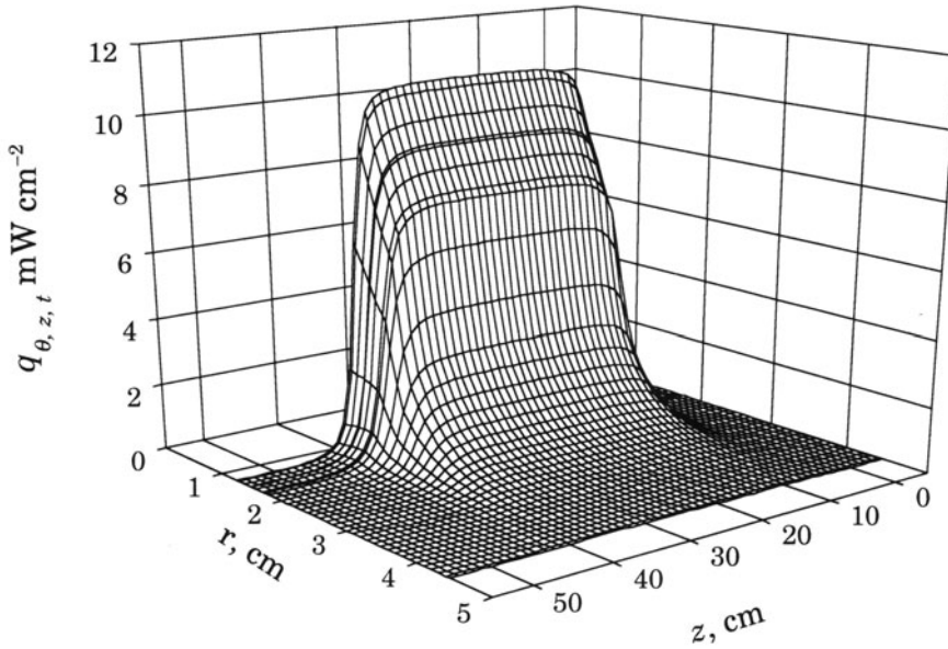
FIGURE 4.15. Radiative flux distribution in a Degussa P25 loaded annular reactor allowing for 0.2% light transmission (Reprinted from Chem. Eng. J. , 90 , M. Salaiques, B. Serrano and H.I. de Lasa, Experimental evaluation of photon absorption in an aqueous TiO 2 slurry reactor, 219–229, Copyright 2002, with permission from Elsevier).
