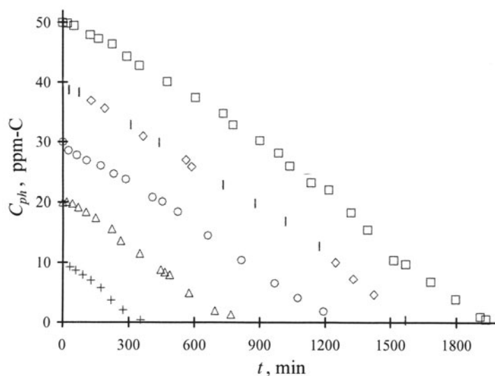
FIGURE 1.6. TOC profiles for the photodegradation of several initial concentration of phenol. (□) 50 ppm, (◇) 40 ppm, (○) 30 ppm, (Δ) 20 ppm, (+) 10 ppm. (Reprinted with permission from Ind. Eng. Chem. Res. , 40 (23), M. Salaices, B. Serrano and H.I. de Lasa, Photocatalytic conversion of organic pollutants: Extinction coefficients and quantum efficiencies, 5455–5464. Copyright 2001 American Chemical Society).
