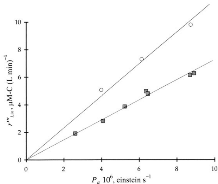
FIGURE 1.2. Initial phenol photoconversion rate ( r'''_{1,in} ) versus incident radiation intensity. (■) Removable 3.2-cm diameter glass inner tube, (○) Removable 5.6-cm diameter glass inner tube. (Reprinted with permission from Ind. Eng. Chem. Res. , 40 (23), M. Salaiques, B. Serrano and H.I. de Lasa, Photocatalytic conversion of organic pollutants: Extinction coefficients and quantum efficiencies, 5455–5464. Copyright 2001 American Chemical Society).
