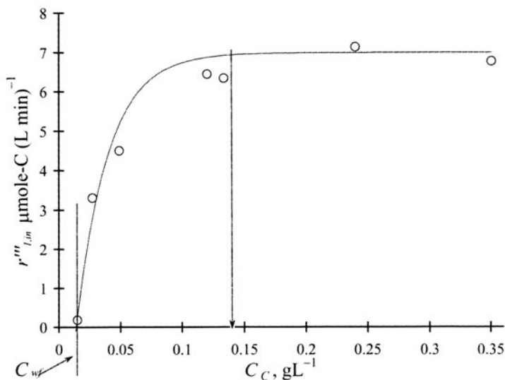
FIGURE 1.3. Initial reaction rate as a function of the catalyst loading. Catalyst: Degussa P25 (Reprinted with permission from Ind. Eng. Chem. Res. , 40 (23), M. Salaiques, B. Serrano and H.I. de Lasa, Photocatalytic conversion of organic pollutants: Extinction coefficients and quantum efficiencies, 5455–5464. Copyright 2001 American Chemical Society).
