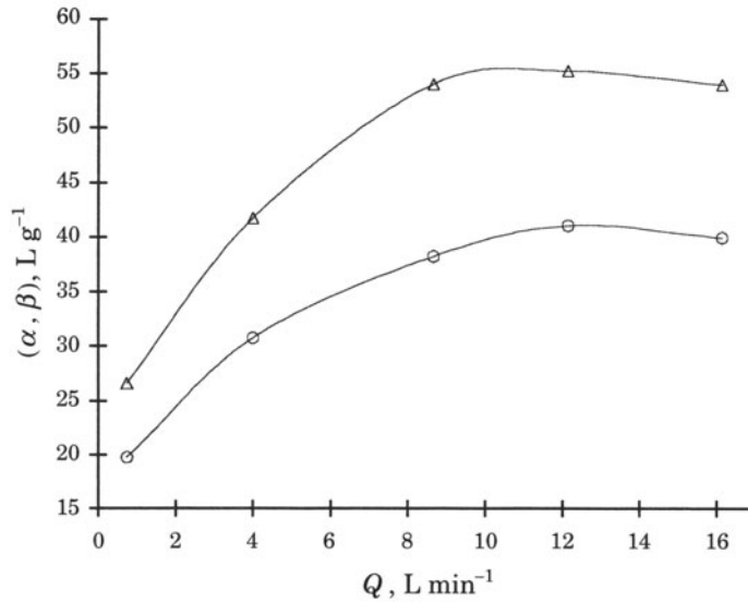
FIGURE 4.20. Effective extinction coefficients versus flow rate for Degussa P25. Keys: ( \Delta ) \beta extinction coefficient, ( \circ ) \alpha effective extinction coefficient, (Reprinted from Chem. Eng. J. , 90 , M. Salaices, B. Serrano and H.I. de Lasa, Experimental evaluation of photon absorption in an aqueous TiO 2 slurry reactor, 219–229, Copyright 2002, with permission from Elsevier).
