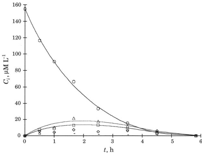
FIGURE 5.5. Concentration profiles of the photodegradation of 155 \mu\text{M L}^{-1} of phenol over Degussa P25 at an initial pH of 4: (o) phenol, ( \Delta ) p -DHB, ( \square ) o -DHB, ( \diamond ) 1,2,4-THB, (-) 1,4-BQ. Full lines represent best-fit model curves. (Reprinted from Chem. Eng. Sci. , 59 , M. Salaces, B. Serrano and H.I. de Lasa, Photocatalytic conversion of phenolic compounds in slurry reactors, 3-15, Copyright 2004, with permission from Elsevier).
