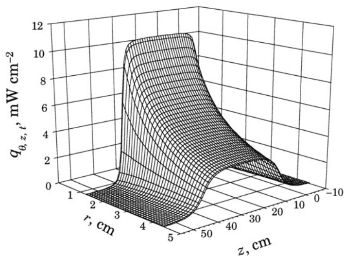
FIGURE 4.3. Radiative flux distribution in an empty annular reactor (Reprinted from Chem. Eng. Journ. , 90 , M. Salaces, B. Serrano and H.I. de Lasa, Experimental evaluation of photon absorption in an aqueous TiO 2 slurry reactor, 219-229, Copyright 2002, with permission from Elsevier).
