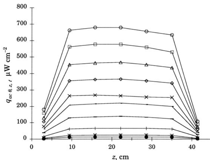
FIGURE 4.10. Axial radiation distribution for several Degussa P25 concentrations using the UV-reflecting collimator 1. Concentrations in \text{mg L}^{-1} . (o) 0; ( \square ) 3; ( \Delta ) 5; ( \diamond ) 10; ( \times ) 15; (-) 20; (-) 30; (+) 50; (*) 80; ( \bullet ) 100 (Reprinted from Chem. Eng. J. , 90 , M. Salices, B. Serrano and H.I. de Lasa, Experimental evaluation of photon absorption in an aqueous \text{TiO}_2 slurry reactor, 219-229, Copyright 2002, with permission from Elsevier).
