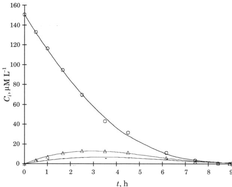
FIGURE 5.8. Concentration profiles of the photodegradation of 158 \mu\text{mole L}^{-1} of phenol over Hombikat UV-100 at an initial pH of 7: (o) phenol, ( \Delta ) p -DHB, (—) 1,4-BQ. Full lines represent best-fit model curves. (Reprinted from Chem. Eng. Sci. , 59 , M. Salaiques, B. Serrano and H.I. de Lasa, Photocatalytic conversion of phenolic compounds in slurry reactors, 3-15, Copyright 2004, with permission from Elsevier).
