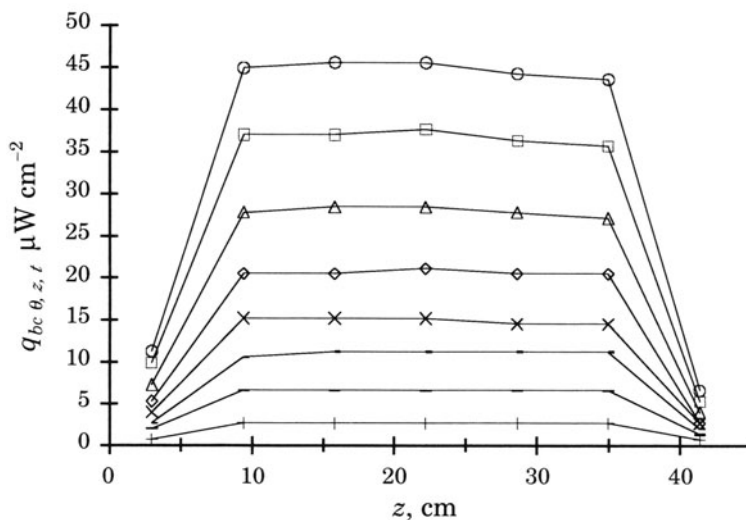
FIGURE 4.11. Axial distribution of the radiation transmission for several Degussa P25 catalyst concentrations using the UV-opaque collimator 3. Concentrations are in \text{mg L}^{-1} . (o) 0; ( \square ) 3; ( \Delta ) 5; ( \diamond ) 10; ( \times ) 15; (-) 20; (-) 30; (+) 50.
