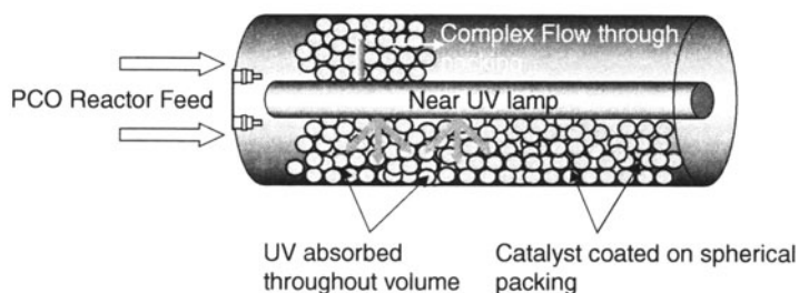
FIGURE 2.6. Annular packed-bed reactor ( AIChE Jour. , 43(3), G.B. Raupp, J.A. Nico and S. Annangi, Two-flux radiation-field model for an annular packed photocatalytic oxidation reactor, 792–801. Reproduced with permission. Copyright © 1997 AIChE)
