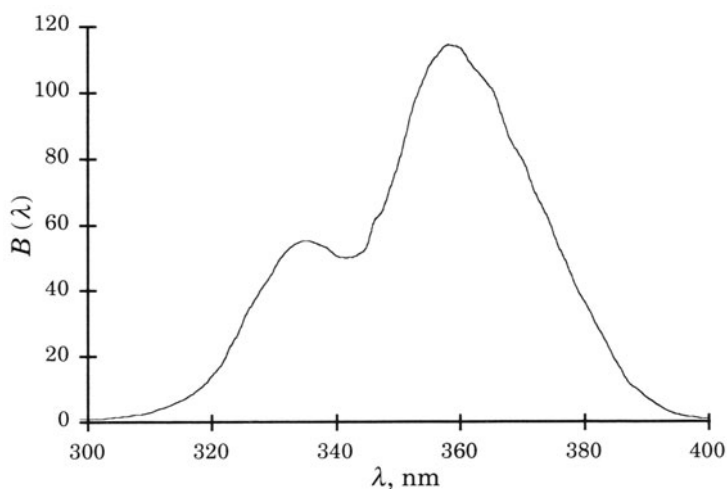
FIGURE 3.1. Spectral Response of the UVX-36 Sensor Cell. (Reprinted with permission of M. Salaces, PhD Dissertation, University of Western Ontario © 2002).
