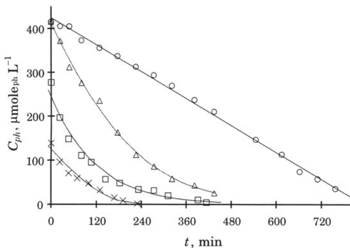
FIGURE 1.5. Phenol photodegradation at several initial concentrations. (○) TOC 412.5 \mu\text{-mole L}^{-1} (30 ppm), Phenol concentrations: (Δ) 412.5 \mu\text{-mole L}^{-1} (30 ppm), (□) 242.0 \mu\text{-mole L}^{-1} (20 ppm), (x) 124.8 \mu\text{-mole L}^{-1} (10 ppm). (Reprinted with permission from Ind. Eng. Chem. Res. , 40 (23), M. Salaices, B. Serrano and H.I. de Lasa, Photocatalytic conversion of organic pollutants: Extinction coefficients and quantum efficiencies, 5455–5464. Copyright 2001 American Chemical Society).
