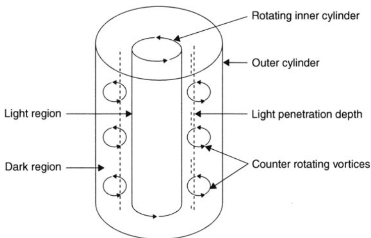
FIGURE 2.2. Taylor vortex reactor in operation (Reprinted from Chem. Eng. Sci. , 50 (20), J.G. Szechowski, C.A. Koval and R.D. Noble, A Taylor vortex reactor for heterogeneous photocatalysis, pp. 3163–3173, Copyright 1995, with permission from Elsevier)
