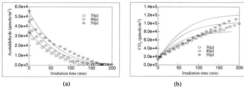
FIGURE 8.5. Changes of acetaldehyde (a) and \text{CO}_2 (b) concentrations with reaction time using Degussa P25. Full line: model predictions. Circles: experimental data (AIChE Journal Copyright 2004, Vol. 50, Issue. 5, Wiley InterScience, p. 1017–1027).
