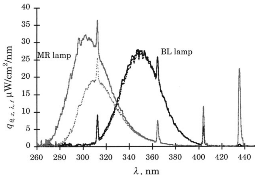
FIGURE 4.9. MR and BL lamp radiation spectra variation through the 0.23-cm-thickness \times 3.2-cm-diameter inner tube (Reprinted with permission from Ind. Eng. Chem. Res. , 40 (23), M. Salaiques, B. Serrano and H.I. de Lasa, Photocatalytic conversion of organic pollutants: Extinction coefficients and quantum efficiencies, 5455–5464. Copyright © 2001 American Chemical Society).
