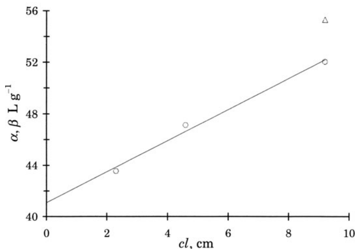
FIGURE 4.14. Exponential factors versus the collimator length for the determination of the effective extinction coefficient (○) \alpha and (Δ) \beta .
