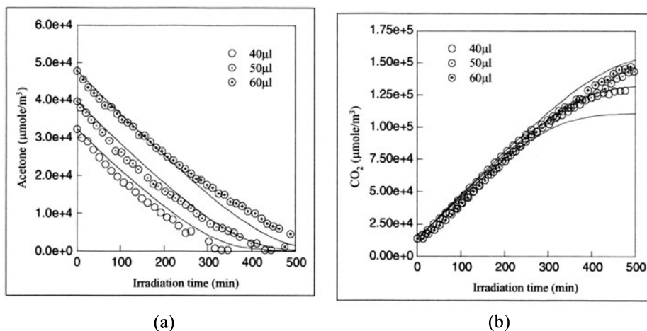
FIGURE 8.2. Changes of acetone concentrations (a) and CO 2 (b) with reaction time using Hombikat UV-100. Full line: model predictions, circles: experimental data. (AIChE Journal Copyright 2004, Vol. 50, Issue. 5, Wiley InterScience, p. 1017–1027).
