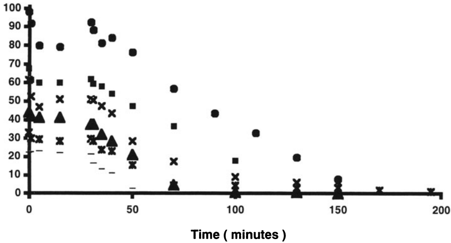
FIGURE 9.1. Photo reduction of silver at different initial concentrations (●) 100 ppm, t_{util} = 101.37 h, (■) 68 ppm, t_{util} = 93.3 h, (×) 63 ppm, t_{util} = 91.3 h, (▲) 45 ppm, t_{util} = 97.7 h, (*) 35 ppm, t_{util} = 96.05 h and (□) 25 ppm, t_{util} = 99.37 h.
