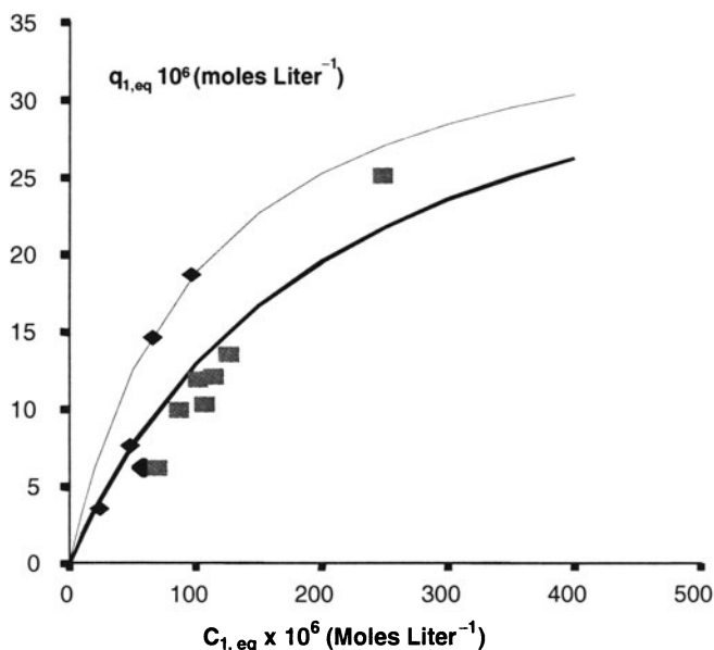
FIGURE 7.5. Equilibrium adsorption isotherms: (◆) 2-4 dichlorophenol, (■) chlorophenol (Reprinted from Chem. Eng. Sci. , 54, B. Serrano and H.I. de Lasa, Photocatalytic degradation of water organic pollutant reactivity and kinetic modeling, 3063–3069, Copyright 1999, with permission from Elsevier).
