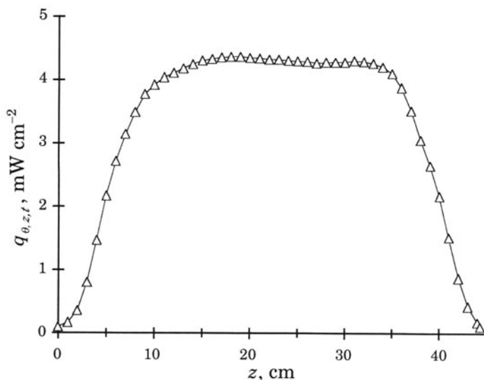
FIGURE 3.2. Typical BL lamp radiative flux axial distribution at 3.1 cm from the reactor axis. (Reprinted with permission from Ind. Eng. Chem. Res. , 40 (23), M. Salaiques, B. Serrano and H.I. de Lasa, Photocatalytic conversion of organic pollutants: Extinction coefficients and quantum efficiencies, 5455–5464. Copyright 2001 American Chemical Society).
