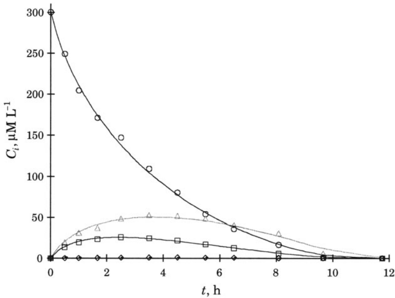
FIGURE 5.4. Concentration profiles of the photodegradation of 300 \mu\text{M L}^{-1} of phenol over Degussa P25 at pH 4: (o) phenol, ( \Delta ) p -DHB, ( \square ) o -DHB, ( \diamond ) 1,2,4-THB, (-) 1,4-BQ. Full lines represent best-fit model curves. (Reprinted from Chem. Eng. Sci. , 59 , M. Salaces, B. Serrano and H.I. de Lasa, Photocatalytic conversion of phenolic compounds in slurry reactors, 3-15, Copyright 2004, with permission from Elsevier).
