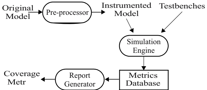
Figure 2-12. Code coverage process
