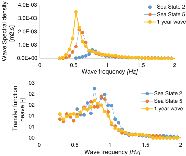
Fig. 8 Illustration of the wave spectrum and in heave obtained in different irregular waves
