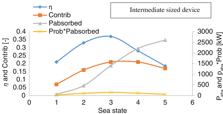
Fig. 15 Illustration of the possible effects of the scaling ratio, with as reference the lab model, on the performance of the device. In this figure, the curves for the intermediate size of the WEC are presented
