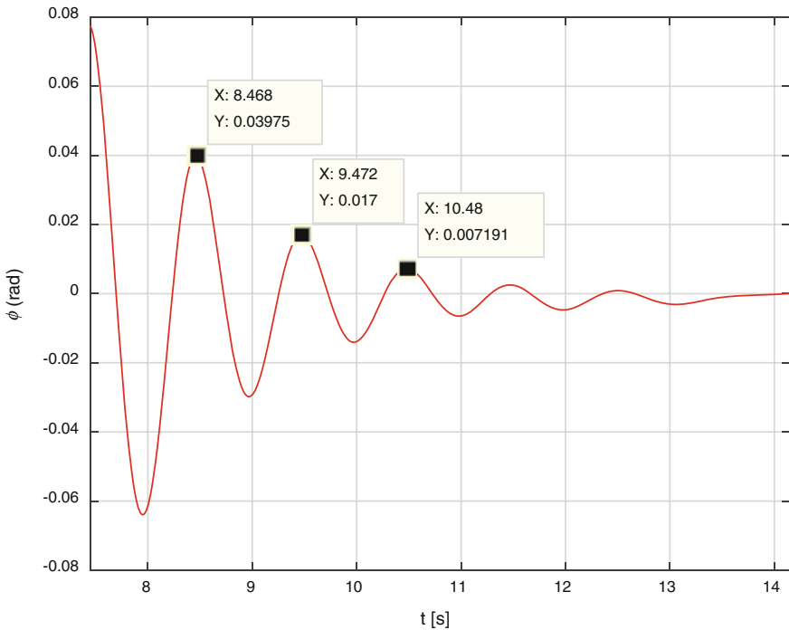
Fig. 6 Results of a decay test for one of the degrees of freedom of the system
