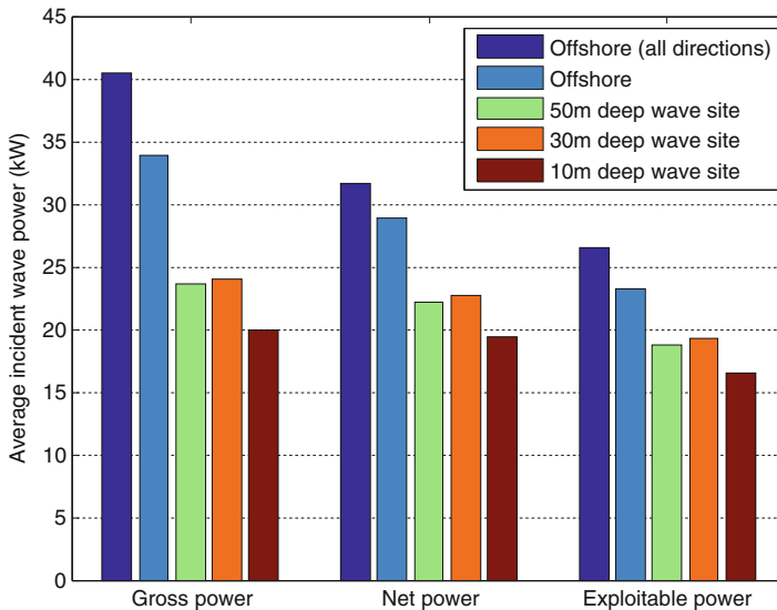
Fig. 16 Average incident wave power at the European Marine Energy Centre, Orkney, Scotland [17]
