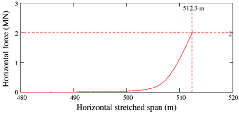
Fig. 14 The horizontal force as function of the horizontal, stretched span
