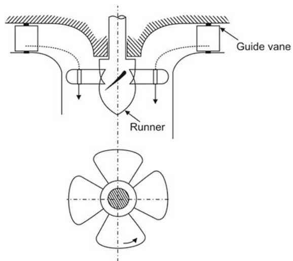
Fig. 12 Schematic of a cross-section view of a Kaplan turbine ( top ) and bottom view of the runner ( bottom ) (taken from [41])
