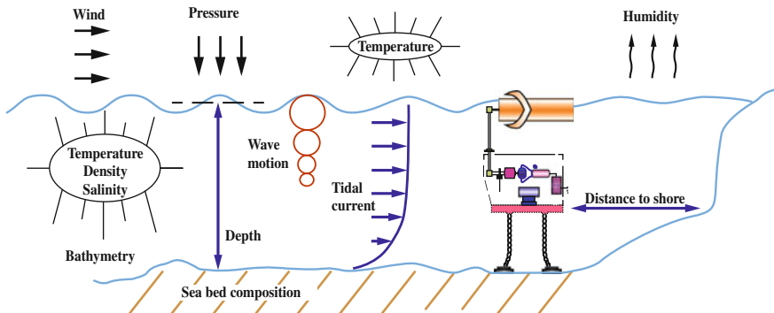
Fig. 2 Metocean parameters applicable to marine energy converts, and their primary sub-systems. Adapted from [4]
