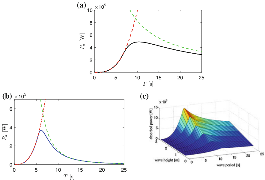
Fig. 12 Upper bounds for a heaving semi-submerged sphere (a), and for a surging semisubmerged sphere (b), both of radius 5 m, and with an incident wave amplitude of 1.0 m. Fully drawn lines shows the absorbed power curves for an optimally controlled buoy. Budal diagram for the heaving sphere extended to also include variation in the wave height H (c). All the diagrams are based on a stroke limit of \pm 3 m
