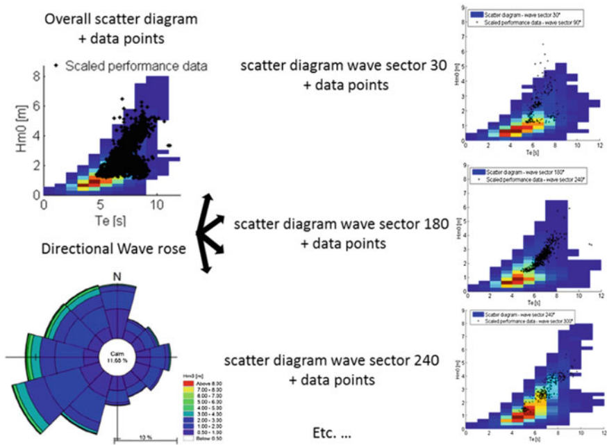
Fig. 20 The overall bi-variate scatter diagram with data points and corresponding directional wave rose ( left ) or the directional scatter diagrams with corresponding data points
