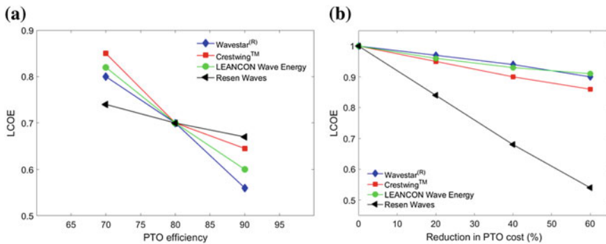
Fig. 2 Influence of a the PTO efficiency and b the relative reduction (in %) in the cost of the PTO system on the relative LCOE for different wave energy converters
