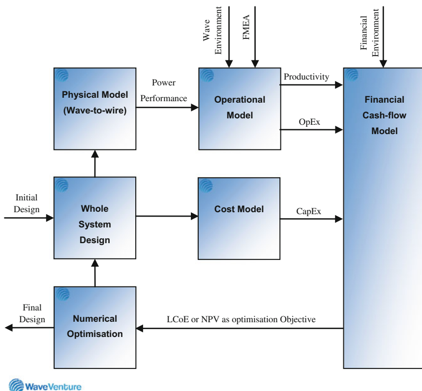
Fig. 2 Schematic of the information flow in an integrated techno-economic optimisation. A techno-economic assessment follows the same structure but without the numerical optimisation step which closes the loop. FMEA is Failure Modes Effects Analysis. Courtesy of Wave Venture Ltd
