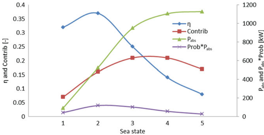
Fig. 10 Example of the representation of \eta_{SS} (blue line), Contrib_{SS} (red line), P_{abs} and Prob * P_{abs} for the different sea states, based on the values given in Table 2
