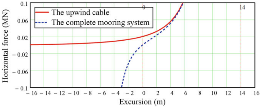
Fig. 16 Horizontal force as a function of the excursion of the buoy. Different range of vertical axis compared to Fig. 15
