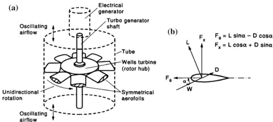
Fig. 6 Illustration of a self-rectifying Wells turbine (taken from [37])
