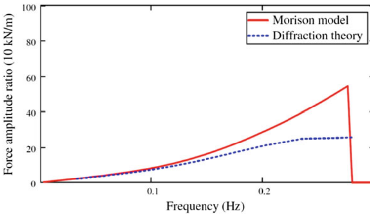
Fig. 12 Force amplitude ratio according to the Morison approach and diffraction theory
