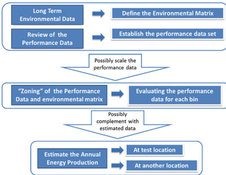
Fig. 19 Overview of the power performance assessment procedure
