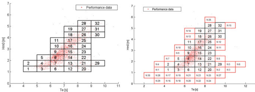
Fig. 23 The original ( left ) and extended ( right ) bins zoning the power performance data ( little dots ) obtained through sea trials and estimations
