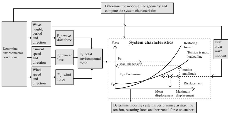
Fig. 18 Quasi-static analysis. Adapted from [26]
