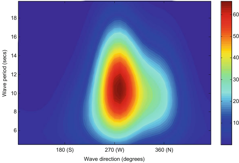
Fig. 8 Average directional spectral variance density ( \text{m}^2/\text{Hz}/\text{rad} ) at the European Marine Energy Centre, Orkney, Scotland
