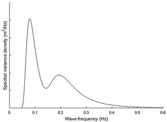
Fig. 12 Example spectrum of a bimodal sea-state
