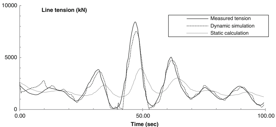
Fig. 19 Course of cable tension around the time for maximum tension in a model test of GVA 5000P (Troll C). [29]
