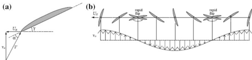
Fig. 9 a Schematic of an aerofoil and b illustration of the aerofoil pitching sequence in oscillating flow for a Denniss-Auld turbine (taken from [39])
