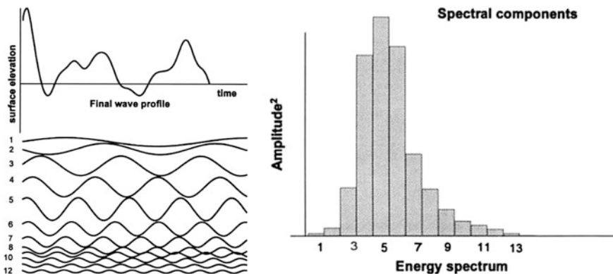
Fig. 11 Super-positioning of waves (corresponding to spectral components) to create water surface elevation (left) and the resulting spectrum (right) [11]
