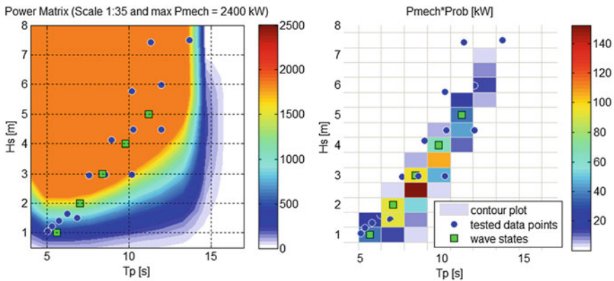
Fig. 11 Power matrix and P_{mech} * Prob plot with scaled tested wave conditions ( blue dots ) and corresponding sea states ( green squares ) (Illustration of the WEPTOS WEC in Danish North Sea wave conditions at a scaling ratio of 1:35 and with a maximum full-scale P_{mech} of 2400 kW)
