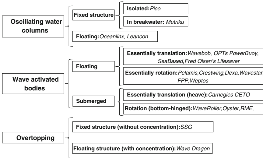
Fig. 5 Categorization of wave energy technologies following IEA – Ocean Energy Systems [16]. Technologies mentioned in the various categories are the ones illustrated in the following figures
