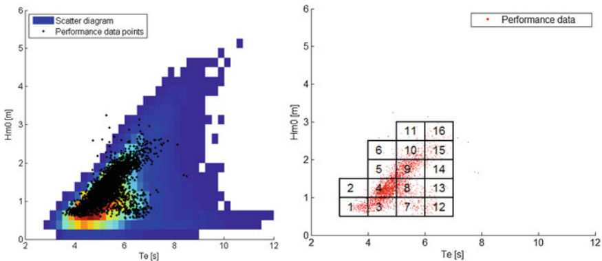
Fig. 21 Scatter diagram with performance data (left) and zoning of the performance data (right)
