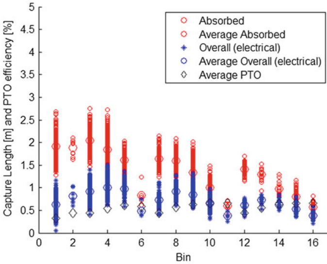
Fig. 22 Representation of the performance data for all bins
