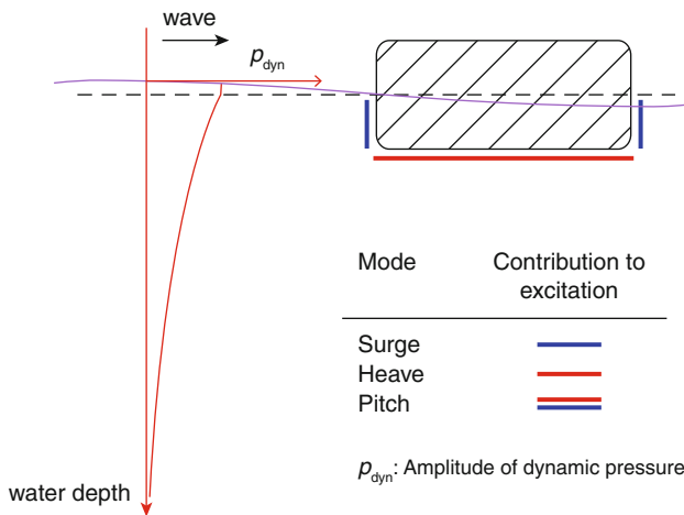
Fig. 8 Parts of the body surface area that contributes to surge ( vertical ), heave ( horizontal ) and pitch (both) excitation. The curve to the left shows the amplitude of hydrodynamic pressure versus distance to mean surface level
