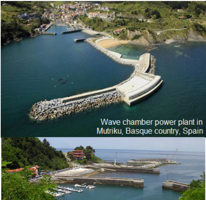
Fig. 6 Mutriku Oscillating Water Column breakwater, equipped with 16 WaveGen Wells turbines, total capacity of 300 kW [24]
