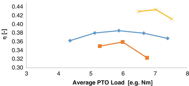
Fig. 12 Illustration of the effect of the PTO loading on the non-dimensional performance ( \eta ), given for three different configurations of the same WEC model
