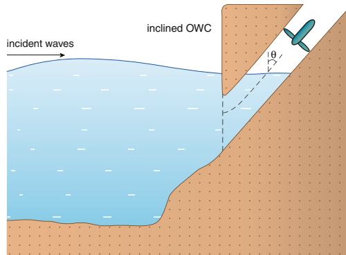
Fig. 6 Oscillating water column inclined at an angle \theta
