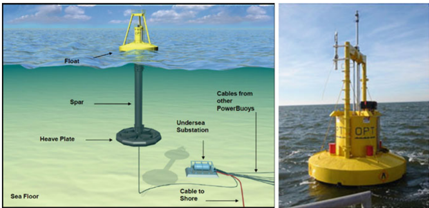
Fig. 12 OPTs PowerBuoy PB40. A slack moored pointer absorber with heave plate [30]
