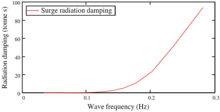
Fig. 10 Surge radiation damping, B_{11} , as a function of wave frequency
