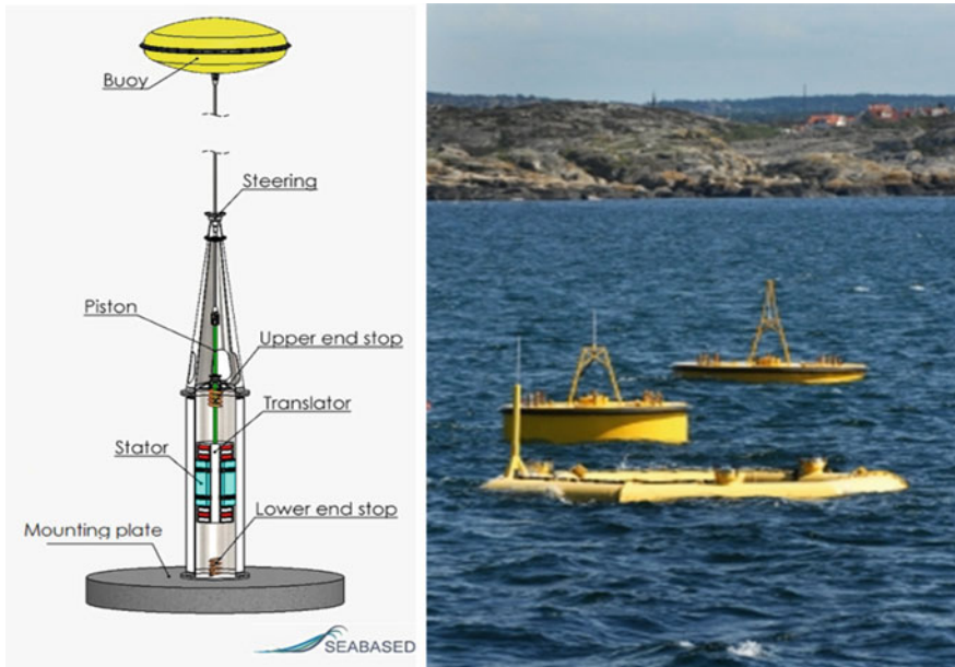
Fig. 14 SeaBased. A point absorber with a directly driven linear generator placed at the sea bottom [32]
