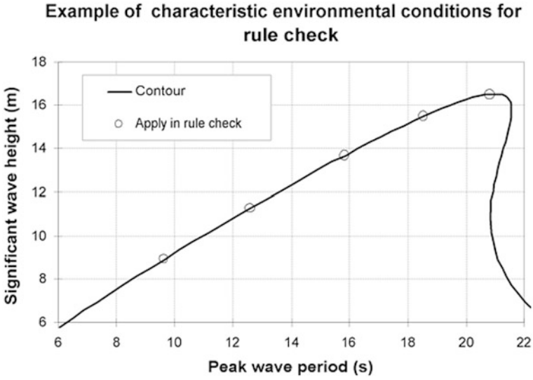
Fig. 2 Selections of sea states along a 100-year contour line. (DNV-OS-E301 [5])
