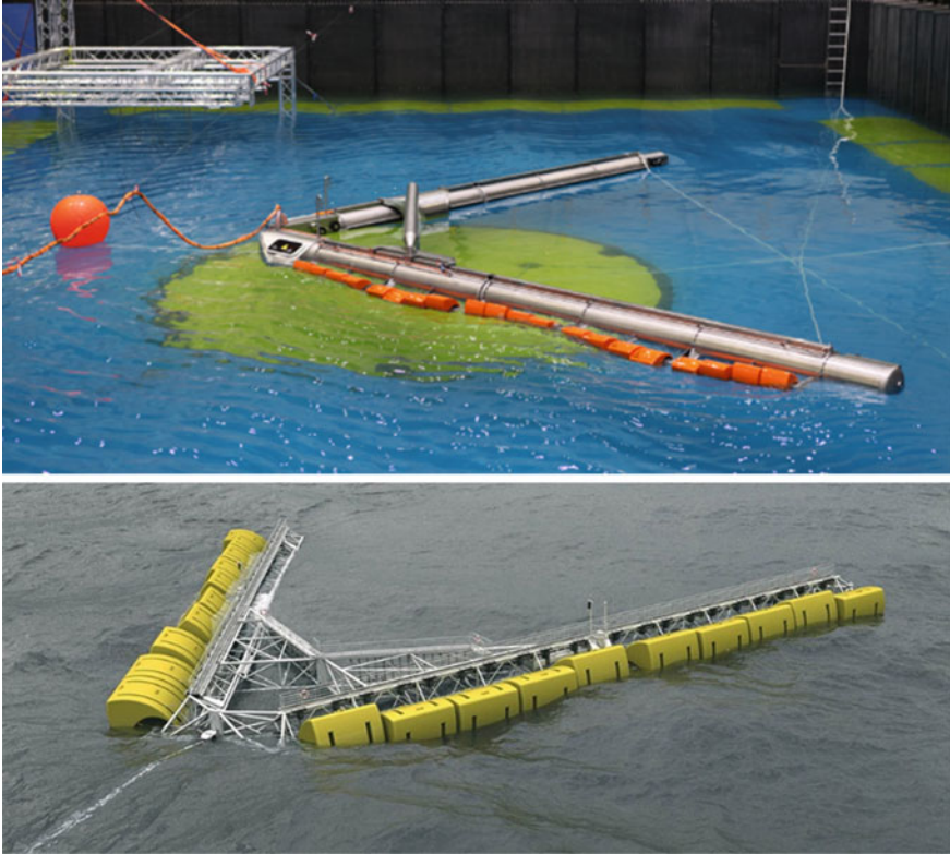
Fig. 23 A fully functional WEPTOS model undergoing testing at CCOB, IH Cantabria, Spain (Sept. 2011) ( top ) and artist impression of the full scale Weptos WEC ( bottom ). Courtesy of Weptos [39]
