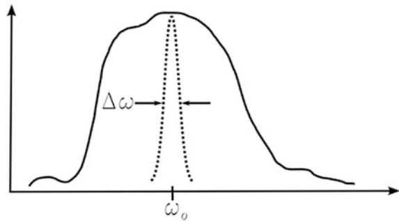
Fig. 15 Representation of the wave spectrum (solid line) compared to the power response of a narrow spectrum wave absorber
