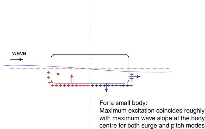
Fig. 9 Illustration of the hydrodynamic pressure along a body
