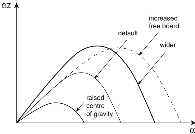
Fig. 4 GZ curve and how it is influenced by changes in geometry. Inspired by [2]
