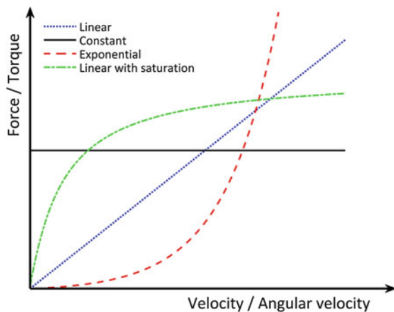
Fig. 16 Various types of linear and non-linear passive loading
