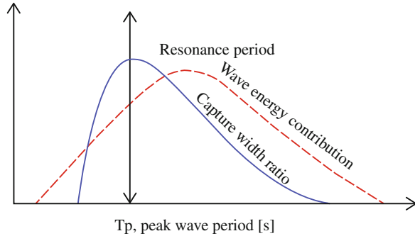
Fig. 13 Illustration of a possible overlap between the resonance period of the wave absorbing body, with the capture width ratio of the WEC and the wave energy contribution given against the peak wave period
