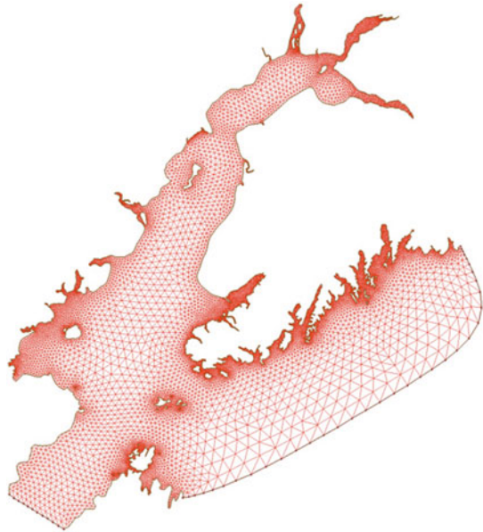
Fig. 22 An example grid for a spectral wave model
