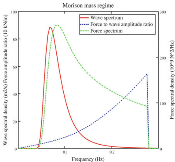
Fig. 8 Wave energy spectrum, S_{PM}(f) , force amplitude ratio, f_w(f) , and force spectrum, S_F(f) . Morison approach
