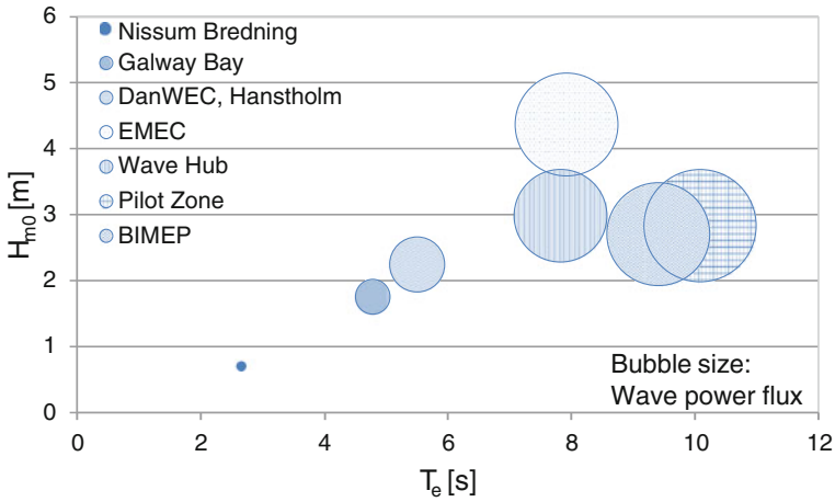
Fig. 28 Characteristic power production wave conditions (significant wave height and energy period) at selected European test sites (Weight averaged with contribution to mean wave power flux)
