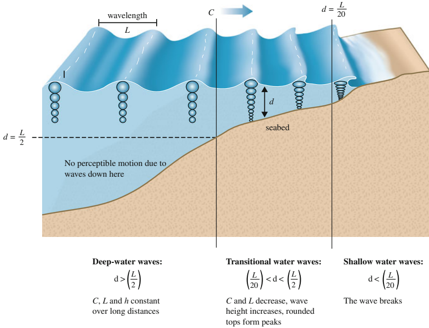
Fig. 6 Motion of water particles in deep and shallow water. Adapted from [2]
