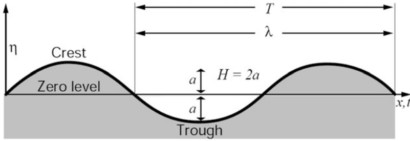
Fig. 4 Definition of wave parameters over a sinusoidal wave [1]
