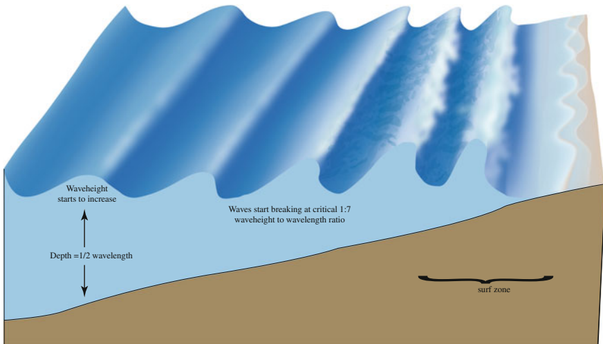
Fig. 13 Change in wave shape due to water depth. Adapted from [7]
