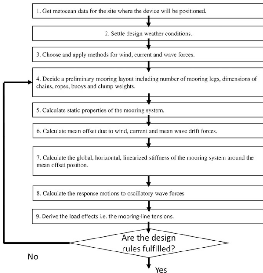
Fig. 1 Flow chart of the quasi-static mooring design loop
