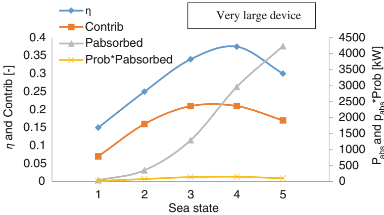
Fig. 16 Illustration of the possible effects of the scaling ratio, with as reference the lab model, on the performance of the device. In this figure, the curves for the largest size of the WEC are presented
