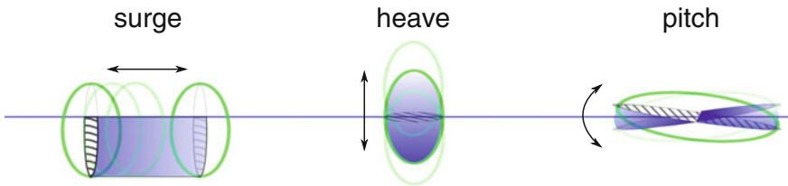
Fig. 11 Illustration of the available volume stroke for the different modes of motion. For heave motion, the volume stroke is the body volume itself if not limited by the stroke of the machinery. For surge and pitch motion, the machinery stroke usually sets the limit for the volume stroke
