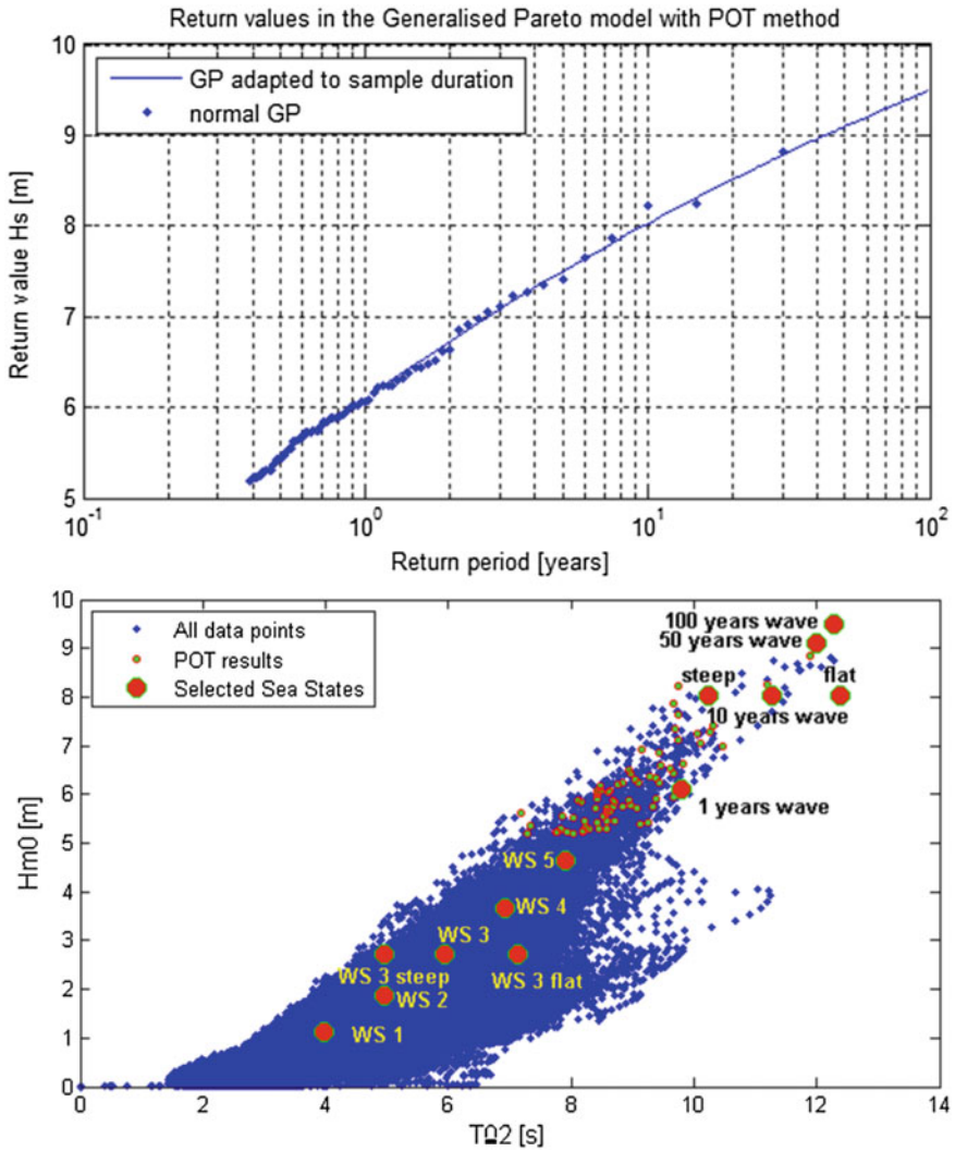
Fig. 5 Estimation of the design wave heights for different return periods ( top ) and representation of the operational and design sea states superposed on the 30 year hindcast scatter diagram of DanWEC Pt 1 ( bottom )
