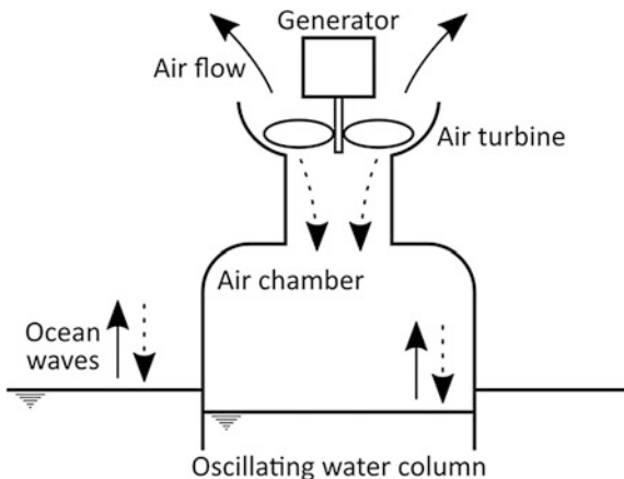
Fig. 5 Schematic of a wave energy converter where an air turbine is employed
