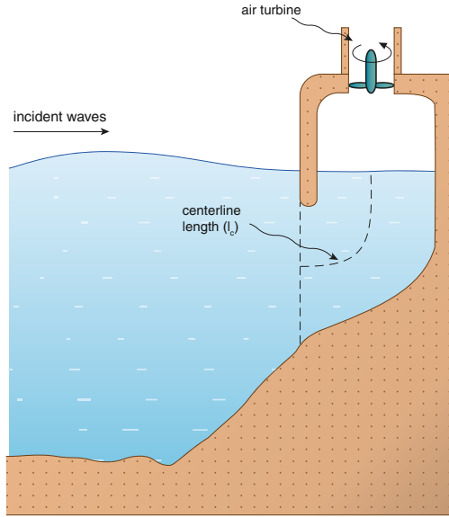
Fig. 5 Oscillating water column where the length l_c is measured along the centreline
