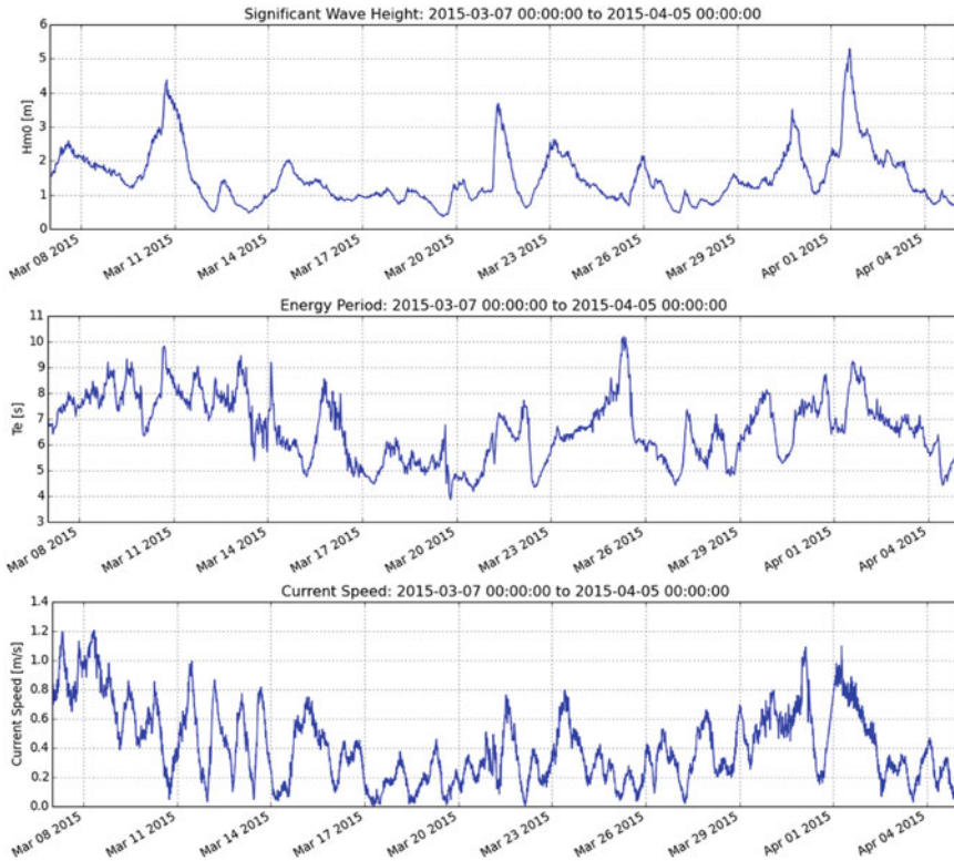
Fig. 7 Example of the variation of the significant wave height, energy wave period and tidal current over one month at DanWEC
