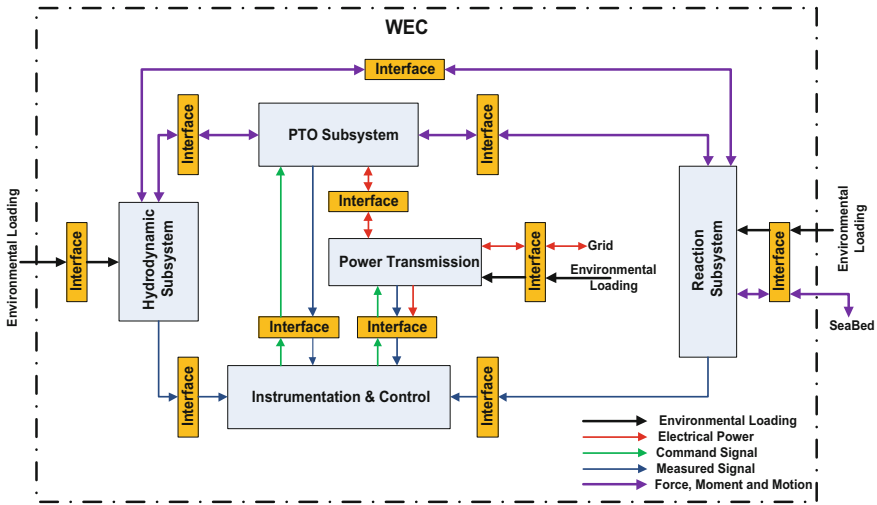
Fig. 5 Generic high level WEC design breakdown [9]
