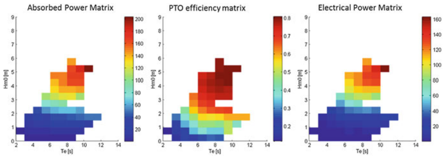
Fig. 24 The absorbed power matrix, the PTO efficiency matrix and the resulting electrical power performance matrix
