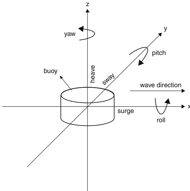
Fig. 2 The motion of a floating body is decomposed in translation: surge (1), sway (2) and heave (3); and rotation: roll (4), pitch (5) and yaw (6). The numbers in parenthesis are often used as index for each of these modes
