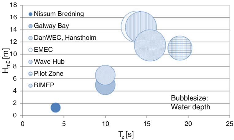
Fig. 29 Extreme wave conditions (significant wave height and average period) at selected European test sites
