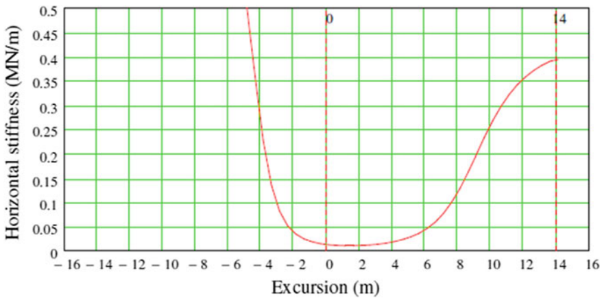
Fig. 17 The horizontal stiffness of the mooring system as a function of the excursion
