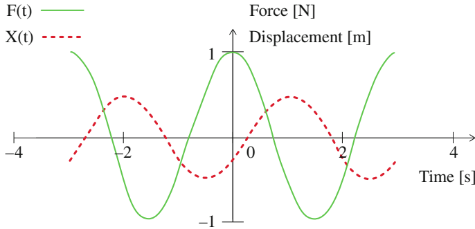
Fig. 22 The exciting harmonic force F(t) and the stationary Response, x(t) , for a linear system
