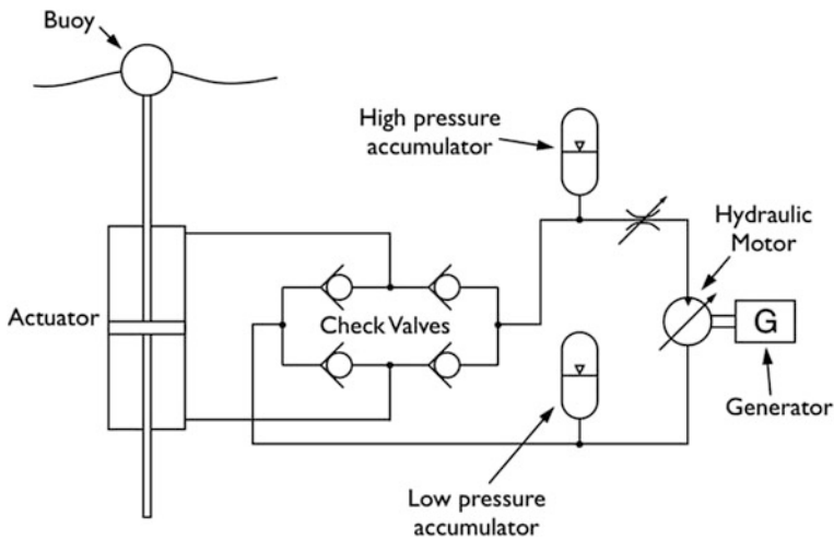
Fig. 10 Example of a hydraulic PTO system for wave energy conversion (taken from [40])
