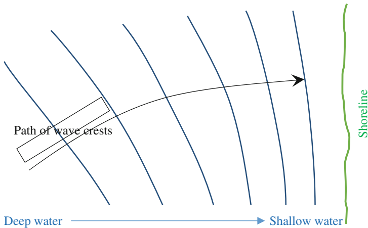
Fig. 14 Wave refraction near the shore due to a change in water depth
