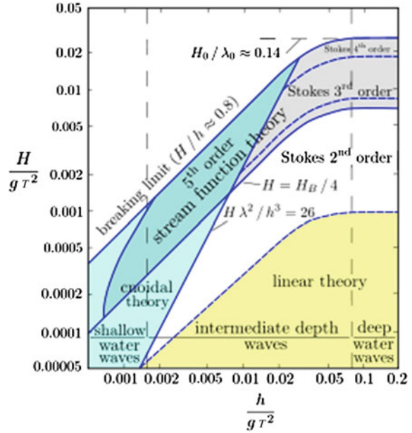
Fig. 5 Chart of wave model suitability [7]
