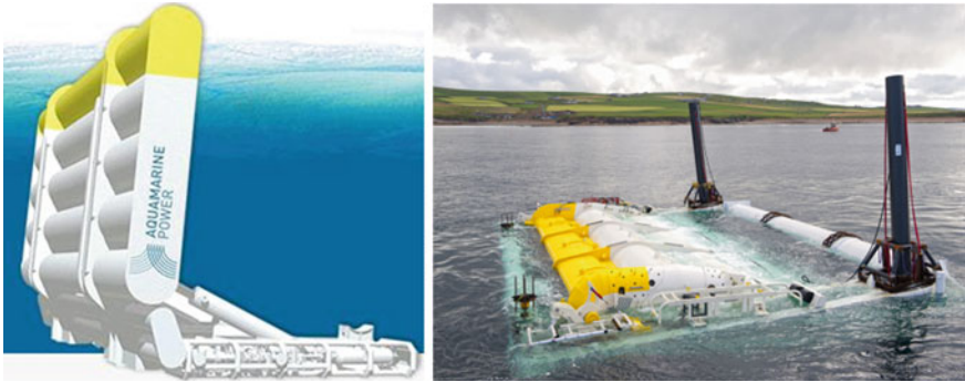
Fig. 17 Installation of the Oyster 800 submerged flap WEC at the European Marine Energy Centre in Orkney, Scotland [34]
