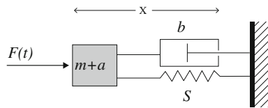
Fig. 20 A mechanical system with one degree of freedom, mass, m , added mass, a , damping coefficient, b , and spring stiffness, S
