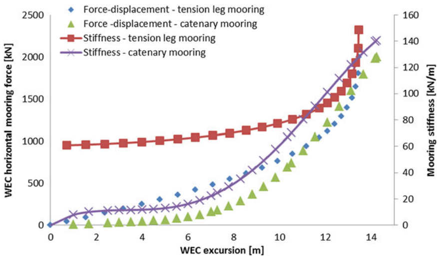
Fig. 17 Example of the force displacement—curves and stiffness relative to displacement curves for a catenary and tension leg mooring system [20]
