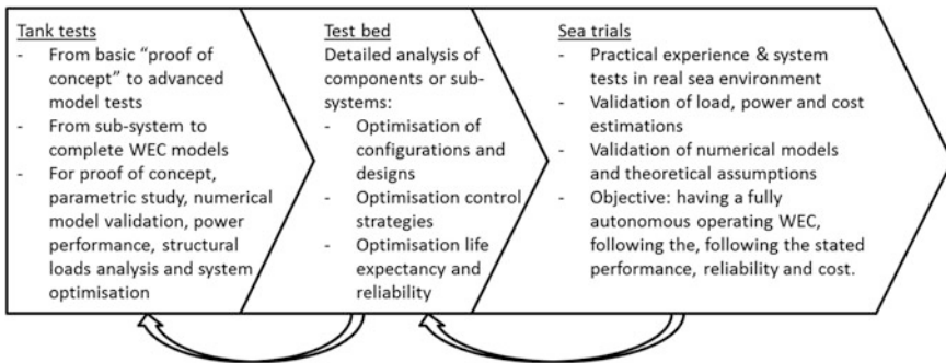
Fig. 1 Flow chart of the experimental testing of WECs
