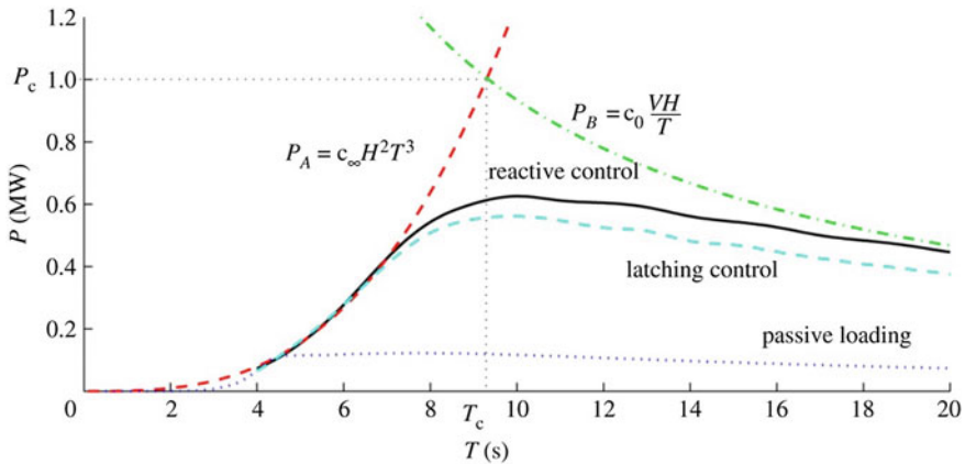
Fig. 18 Comparison of the power that can be absorbed from a given sinusoidal wave by a semi-submerged sphere heaving with optimum condition for three different control strategies (taken from [42])
