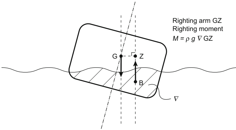
Fig. 3 Righting force \rho g \nabla
