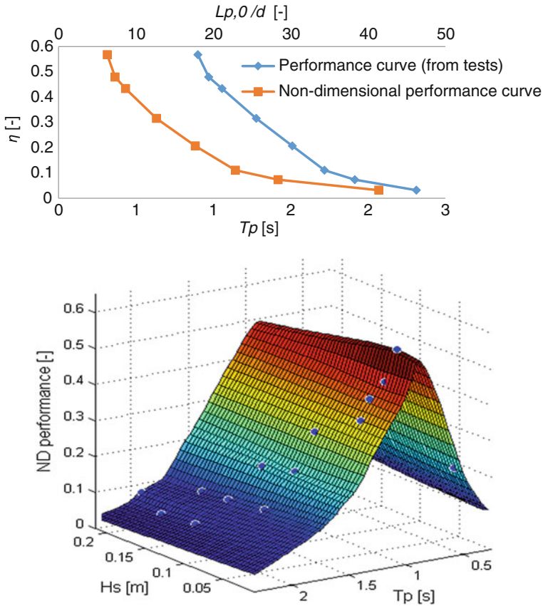
Fig. 9 Illustration of a performance (in terms of CWR = \eta = ND performance) curve and surface that can be obtained through tank testing [18]
