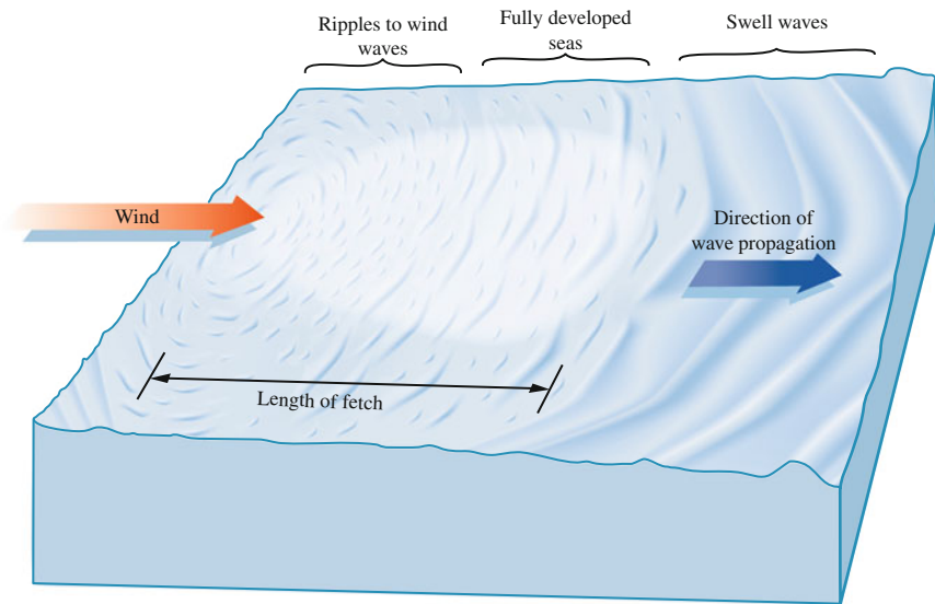
Fig. 2 The generation of ocean waves. Adapted from [2]
