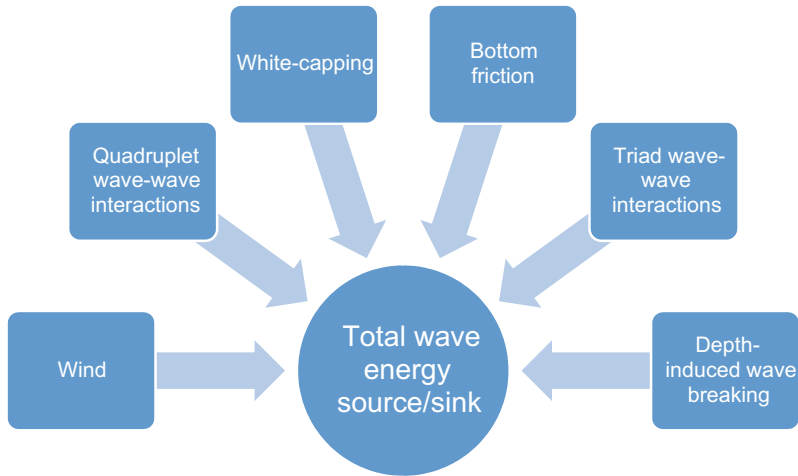
Fig. 21 Source terms used in a third-generation spectral wave model
