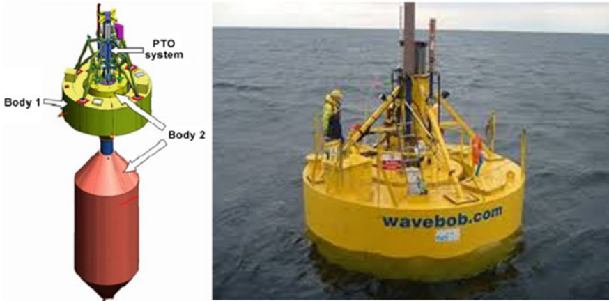
Fig. 13 Wavebob. A slack moored pointer absorber with submerged reference volume [31]
