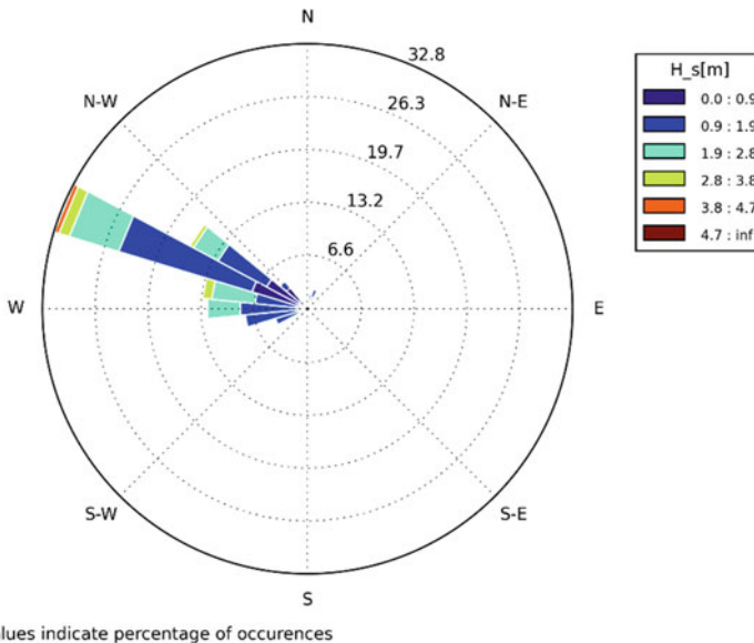
Fig. 10 Example wave rose of significant wave height
