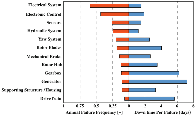
Fig. 5 Failure frequency and downtime of components. Adapted from [23]
