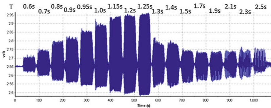
Fig. 7 Illustration of the response motions in 1 DoF of a wave-activated body in regular waves having a same wave height but incrementing wave period (The vertical axis represents the absolute motion of the body)
