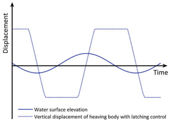
Fig. 17 Illustration of the latching control where a heaving body is kept at a fixed vertical position for a certain time interval in order to achieve phase control
