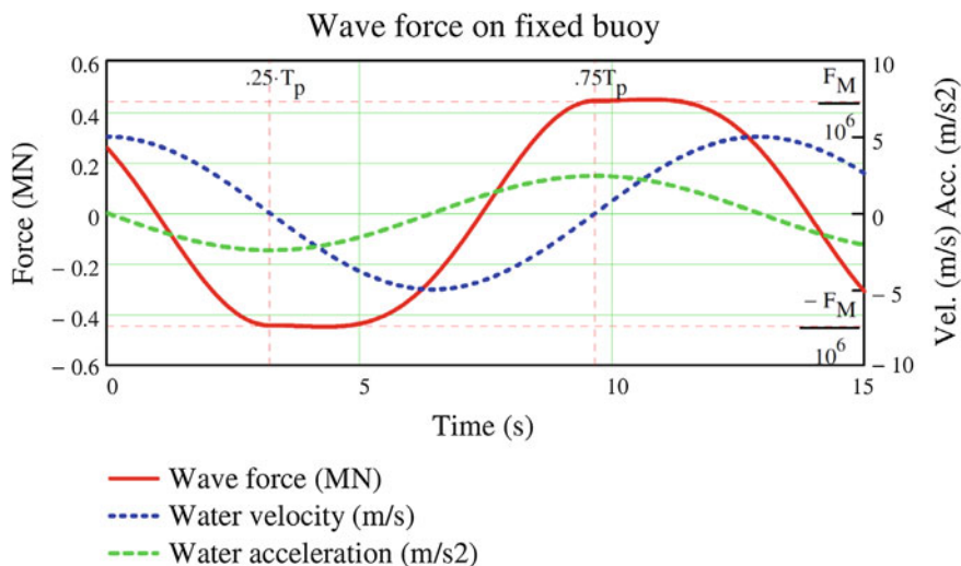
Fig. 7 The Morison force as a function of time for wave amplitude a = H_{max}/2 and period T_p = 12.9 \text{ s} . The water acceleration is drawn for comparison
