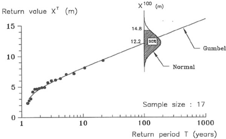
Fig. 4 Illustration of the possible process to define the design wave height for a certain return period, which in this case is 12.2 m for a return period of 100 years without considering sample variability or 14.8 m with sample variability at a 90 % one-sided confidence interval [11]
