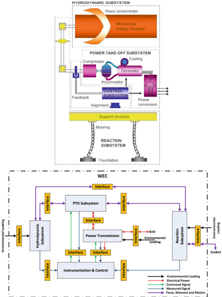
Fig. 3 WEC system design breakdown following Equimar (top) [5] and DNV (bottom) [6]. Courtesy of Equimar and DNV GL
