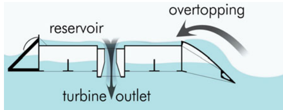
Fig. 11 Illustration of the working principle of a floating overtopping wave energy converter (taken from [14])
