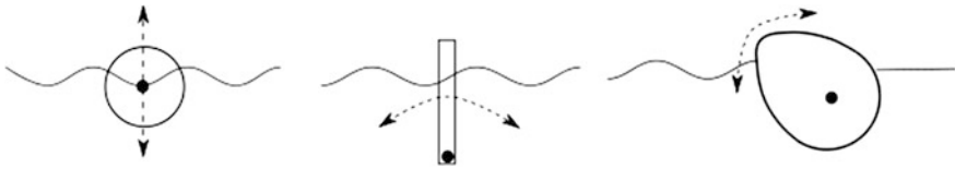
Fig. 4 Illustration of the radiated wave by the motion in one direction by three wave-absorbing bodies, from left to right : heaving point absorber, pitching flap and pitching Salter’s duck
