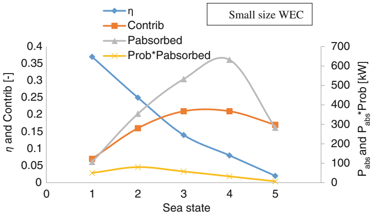
Fig. 14 Illustration of the possible effects of the scaling ratio, with as reference the lab model, on the performance of the device. In this figure, the curves for the smallest size of the WEC are presented
