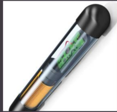
This RFID chip shows the coiled copper antenna it uses to communicate
