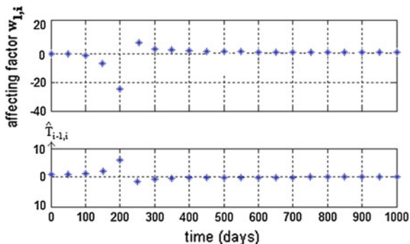
Fig. 7.10 Affecting factor w_{1,i} and effective hydraulic transmissivity \hat{T}_{i-1,i} : T_1 = 0.1 and T_2 = 0.9 \text{ m}^2/\text{day}
