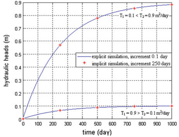
Fig. 7.8 Comparison of the explicit and implicit simulations
