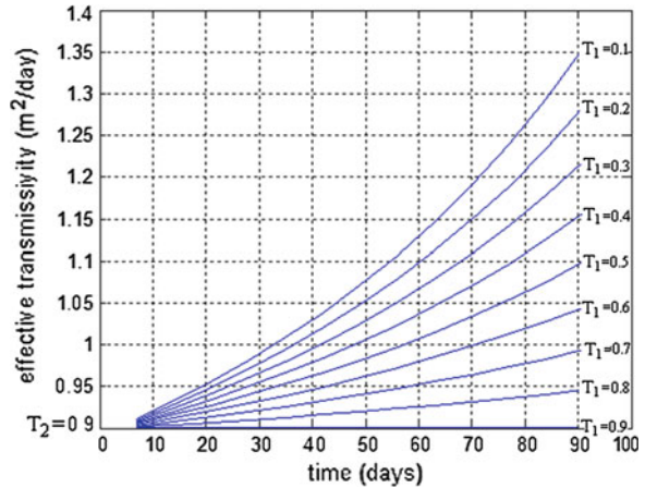
Fig. 9.6 Master curves for effective transmissivities for T_2 > T_1
