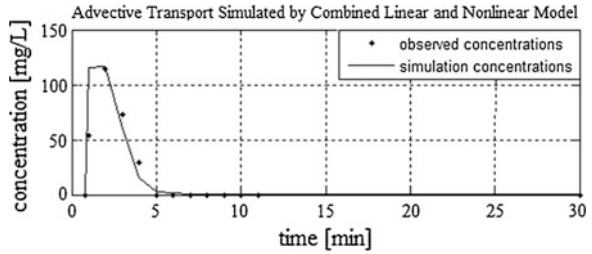
Fig. 10.10 K^+ ion transport: results presented by Paseka et al. (2000) and simulated by Eqs. 10.44 and 10.24 with parameter values \alpha = 1.1 ; A = 0.546/\text{min} ; A_\alpha = 0.1 \text{ mg}^{-0.1} \text{ cm}^{0.3} \text{ min}^{-1}
