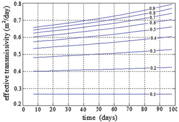
Fig. 9.9 Master curves obtained by the homogeneous interpretation model to the object presented in Fig. 9.8 with the hydraulic transmissivities T_1 = 0.1 , T_2 = 0.2 \text{ m}^2/\text{day} . Values of the transmissivities T_3 are shown on the pertinent plots
