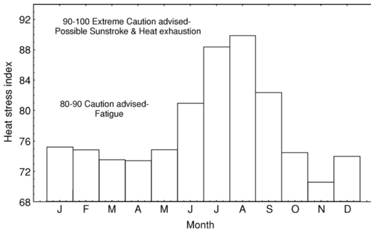
Fig. 9.3. Monthly heat stress index values in Gibraltar for the period 1850 to 1995 (concept from Matzarakis and Mayer 1997).
