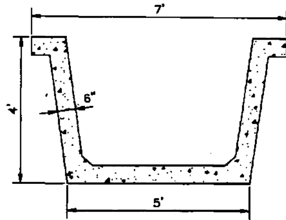
Fig. 12.2.3.1—Precast trapezoidal channel
