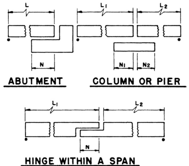
•EXPANSION JOINT OR END OF BRIDGE DECK
