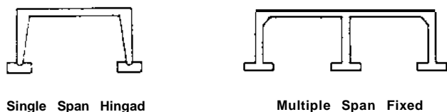
Fig. 2.5.4-Elevations of rigid frame bridges
