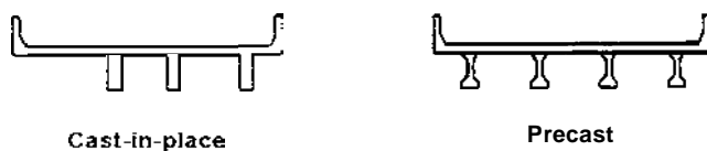
Fig. 2.5.3.2-Cross sections of stringer bridges
