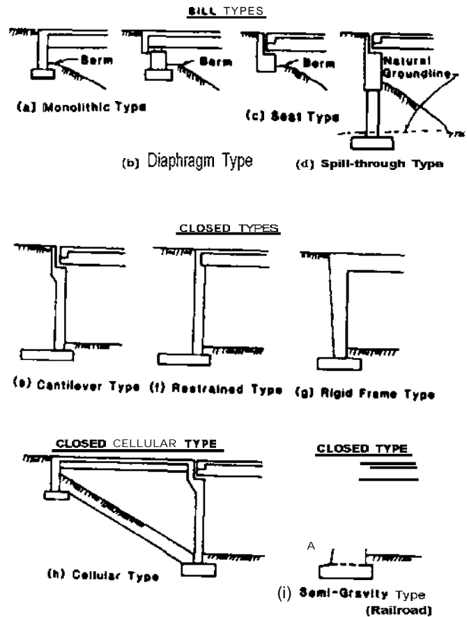
Fig. 11.5.3-Abutment types
