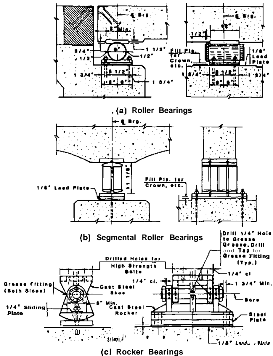
Fig. 11.2.2.4-Steel bearings
