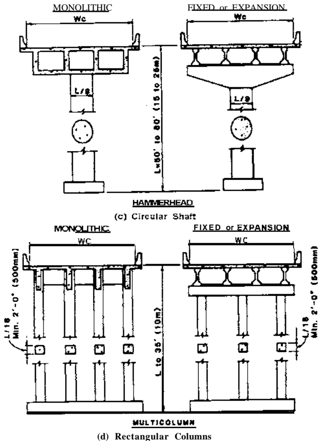
Fig. 11.6.2(c) and (d)-Circular shaft hammerhead and multi-column piers
