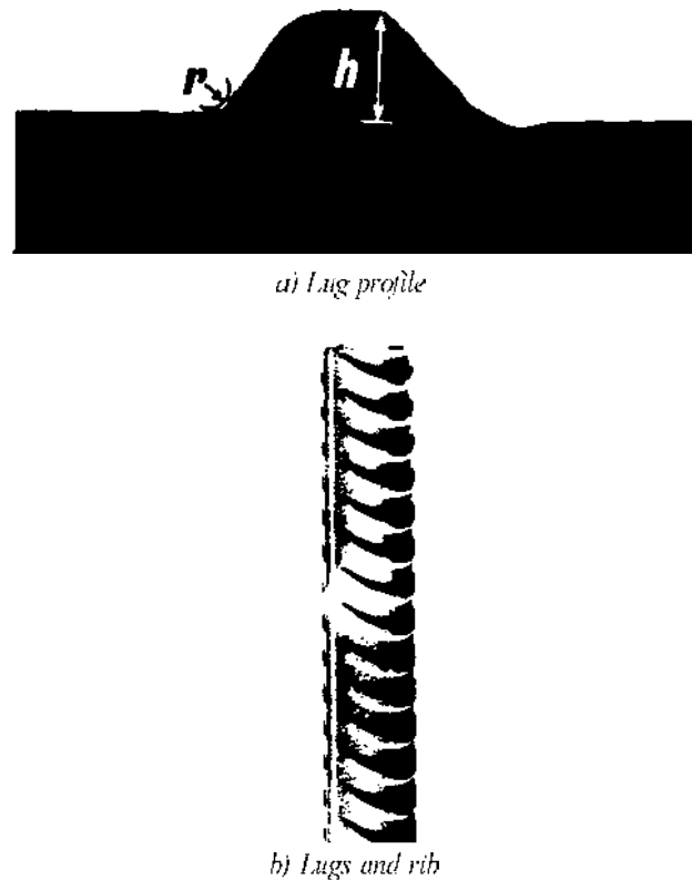
Fig. 8.3-Bar geometry
