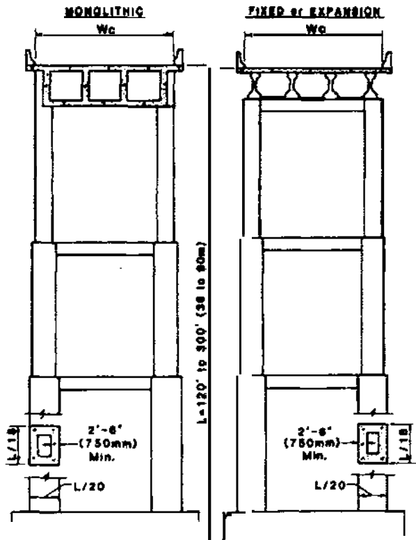
Fig. 11.6.2(h)-Multistory bent piers
