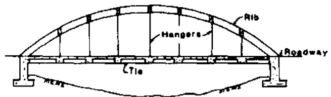
Fig. 2.5.5.3—Tied arch bridge
