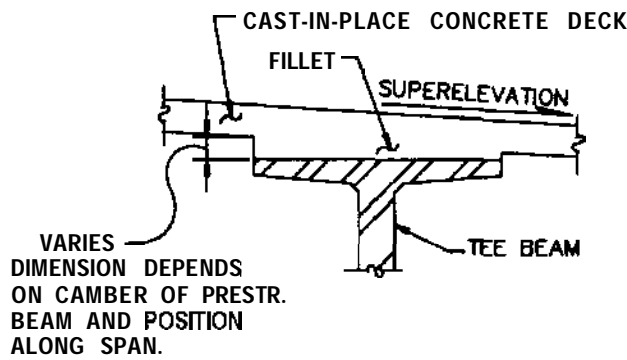
Fig. 12.5.6.1—Wide beam with superelevated CIP deck
