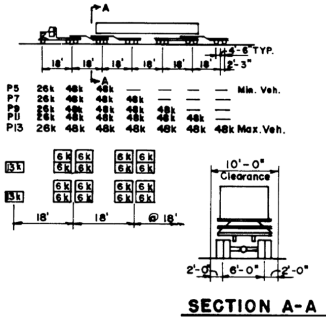
Fig. 5.7.2.3—Permit design live loads.
