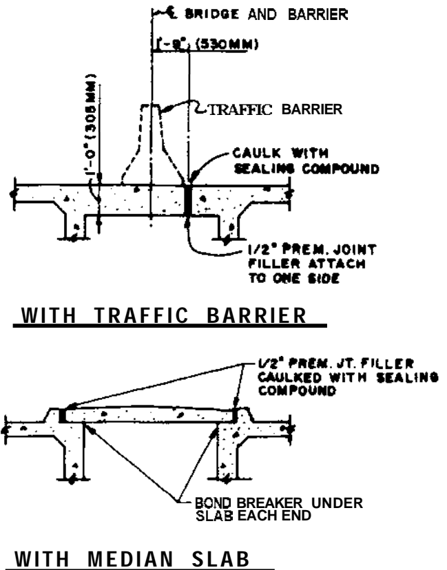
Fig. 4.10.2.3-Examples of longitudinal expansion joints for wide structures
