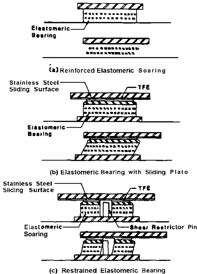
Fig. 11.2.2.1-Elastomeric bearings
