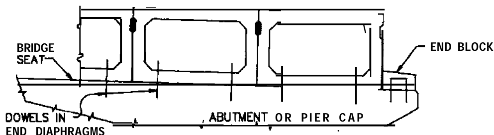
Fig. 12.5.6.2-Superelevated deck with butted box beams
