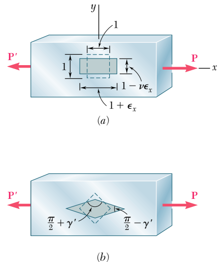
Fig. 2.49 Representations of strain in an axially-loaded bar.
