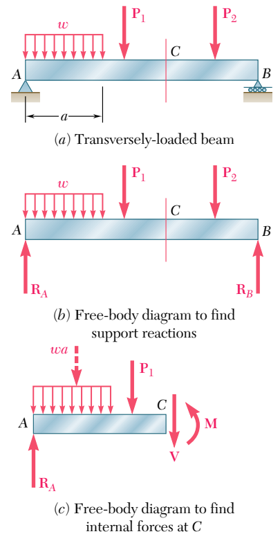
Fig. 5.4 Analysis of a simply supported beam.
