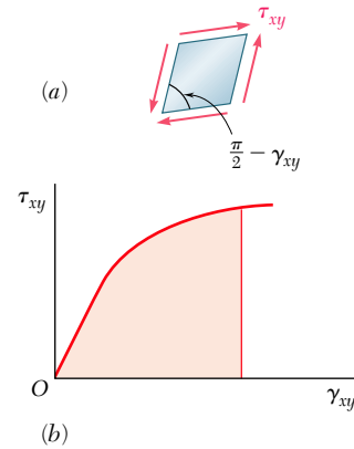
Fig. 11.16 Strain energy due to shear.
