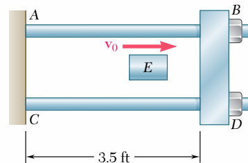
Fig. P11.42 and P11.43
