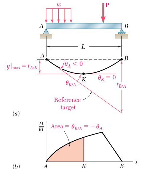
Fig. 9.63 Determination of maximum deflection using moment-area method.
