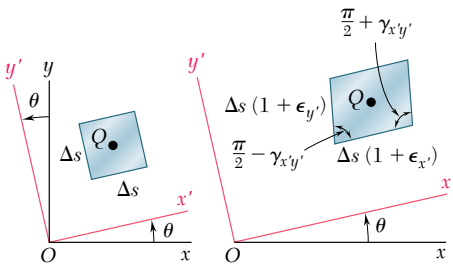
Fig. 7.57 Transformation of plane strain element.
