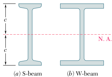
Fig. 4.13 Steel beam cross sections.
