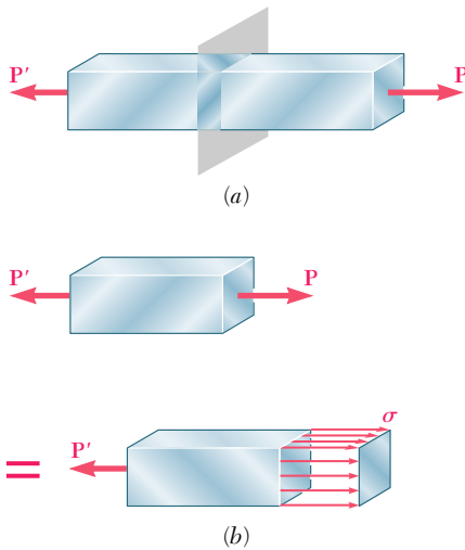
Fig. 1.26 Axial forces.
