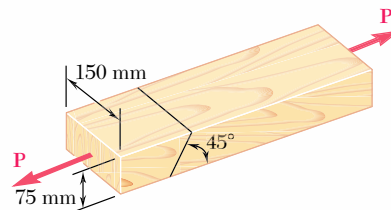
Fig. P1.31 and P1.32
