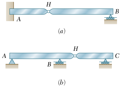
Fig. 5.3 Beams connected by hinges.
