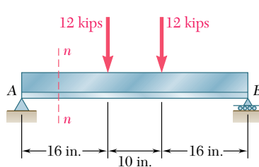
Fig. P6.22 and P6.24
