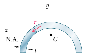
Fig. 6.31 Half pipe beam.
