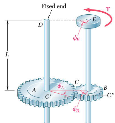
Fig. 3.60 Statically indeterminate shafts
