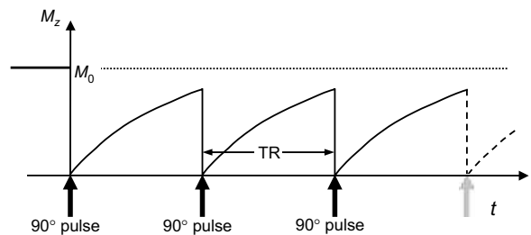
Fig. 1.16. To collect data for an MR image, a series of 90° RF pulses must be applied, with a separation between each pulse of TR. The amount of longitudinal magnetization before each pulse determines how much signal that pulse will generate. Hence, T1 influences the signal intensity in the image as TR is shortened
