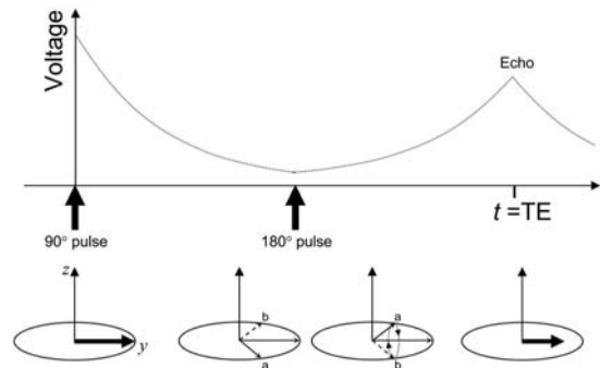
Fig. 1.8. After the initial 90° pulse, dephasing of transverse magnetization occurs, with the magnetization from two locations within the patient, labeled a and b , being shown. A 180° pulse is applied and rotates the magnetization about the y -axis so that the magnetization is flipped over, reversing the phase of a and b . The magnetization continues to precess and comes back into phase at a time TE called the echo time. Deviations from the average motion are shown, so that superimposed on this is a precession at the average Larmor frequency
