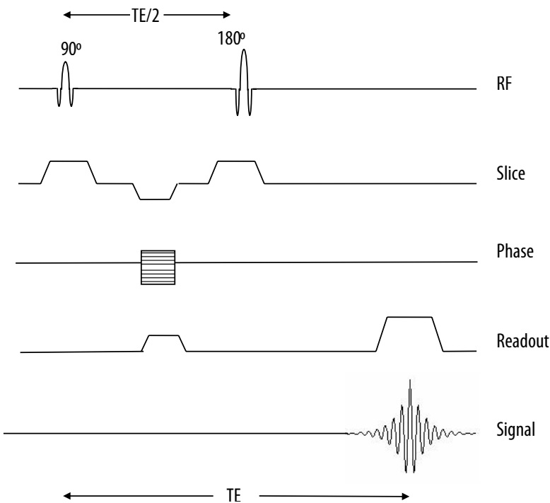
Fig. 3.3. Spin-echo pulse sequence timing diagram where a pair of 90^\circ and 180^\circ radiofrequency ( RF ) pulses are used to create spin echo at echo time ( TE )
