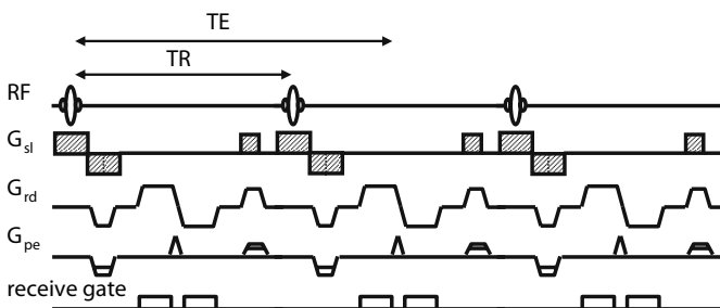
Fig. 8.10. The PRESTO pulse sequence.
