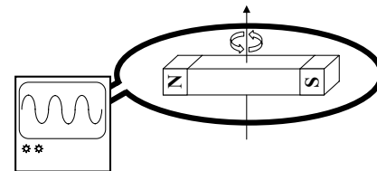
Fig. 1.5. A voltage will be induced across the ends of a coil of wire placed around a rotating magnet. In an MRI scanner, this rotating magnetism originates in the patient after a 90° pulse has been applied. An oscilloscope connected to the coil would show a sinusoidally oscillating voltage, with the frequency of oscillation equal to the Larmor frequency, and the peak-to-peak voltage being proportional to the number of spins within the sensitive region of the coil
