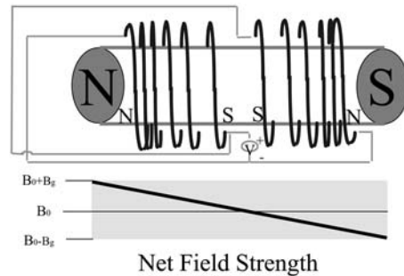
Fig. 2.7. Diagram of a solenoidal gradient coil and the effect on net magnetic field
