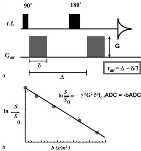
Fig. 6.1a,b. a Typical spin-echo Stejskal Tanner pulse sequence for diffusion weighting with a pair of pulsed field gradients of strength G and length d . Data acquisition is denoted by a free induction decay. b Calculation of the apparent diffusion constant ( ADC ) from a linear fit of the normalized logarithmic signal decay as a function of b -factor. The diffusion time and signal decay are defined for a pair of square field gradients
