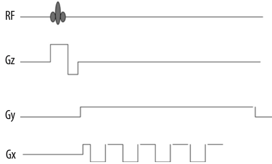
Fig. 4.15. Timing diagram example for echo planar imaging
