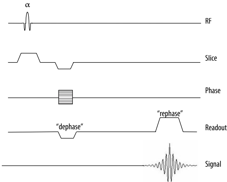
Fig. 3.6. Gradient-echo pulse sequence timing diagram where frequency encoded gradient pulses (i.e., readout) are used to first "dephase" and then "rephase" the spins to create the echo. The flip angle ( \alpha ), repetition time, and echo time help to determine the degree of T1 and T2 weighting of the image
