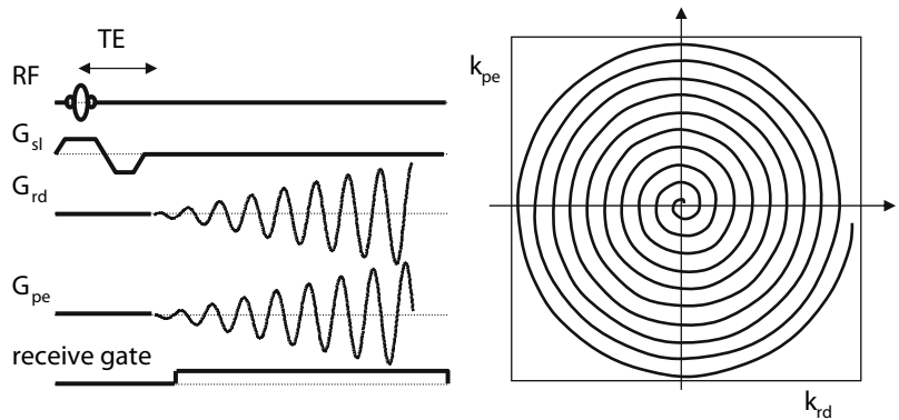
Fig. 8.9. Spiral pulse sequence and k -space trajectory.
