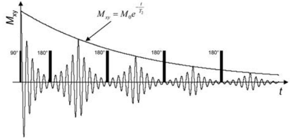
Fig. 1.10. Multiple spin-echoes are formed by applying 180° pulses in succession. The echoes form in the spaces between the pulses, and the amplitude of echoes in the “train” decreases exponentially with a time constant T2
