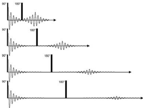
Fig. 1.9. Increasing the time between the 90° and 180° pulses causes the spin-echo to form later. While the effects of magnetic field inhomogeneity are reversed by the 180° pulse, some reduction in the echo amplitude with increasing echo time remains; the time constant for echo amplitude decay is T 2 , the transverse relaxation time
