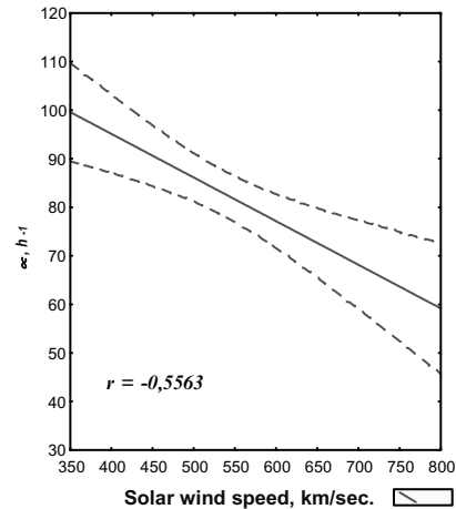
Figure 7. Dependence of growth rate upon the solar wind speed.
