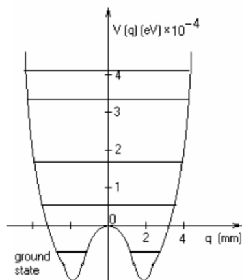
Figure 1a. Organism's ground state (health). Landau-Haken potential. V(q) = kq^2/2 + k_1q^4 ( k < 0 , k_1 > 0 )
