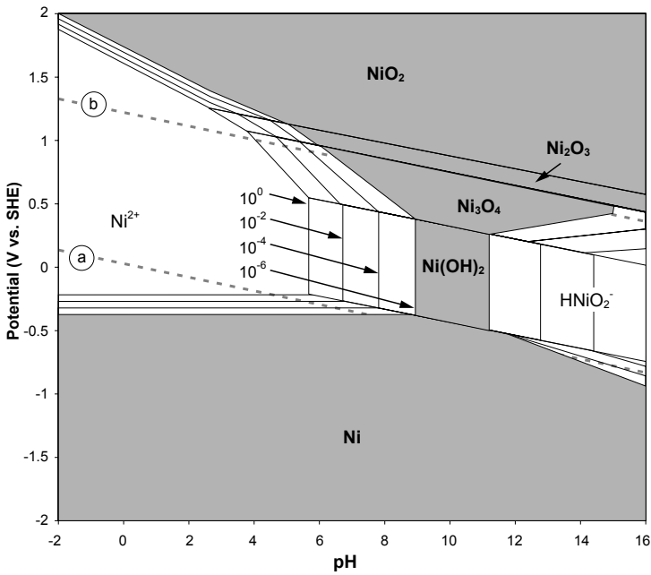
Figure F.16 Potential-pH equilibrium diagram for the nickel-water system at 60°C considering the hydrated oxide forms.
