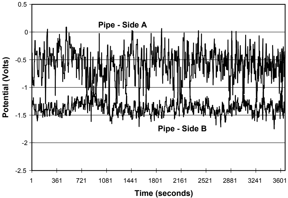
Figure 11.20 Potential fluctuations due to stray current effects on two sides of an insulator in a pipeline. Note the opposite direction of the potential transients on the two sides.
