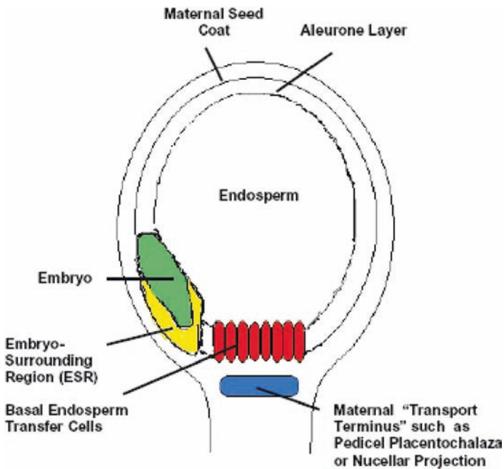
Fig. 6 Schematic of the developing cereal caryopsis and tissues important to transport processes (modified from Olsen, 2004)
