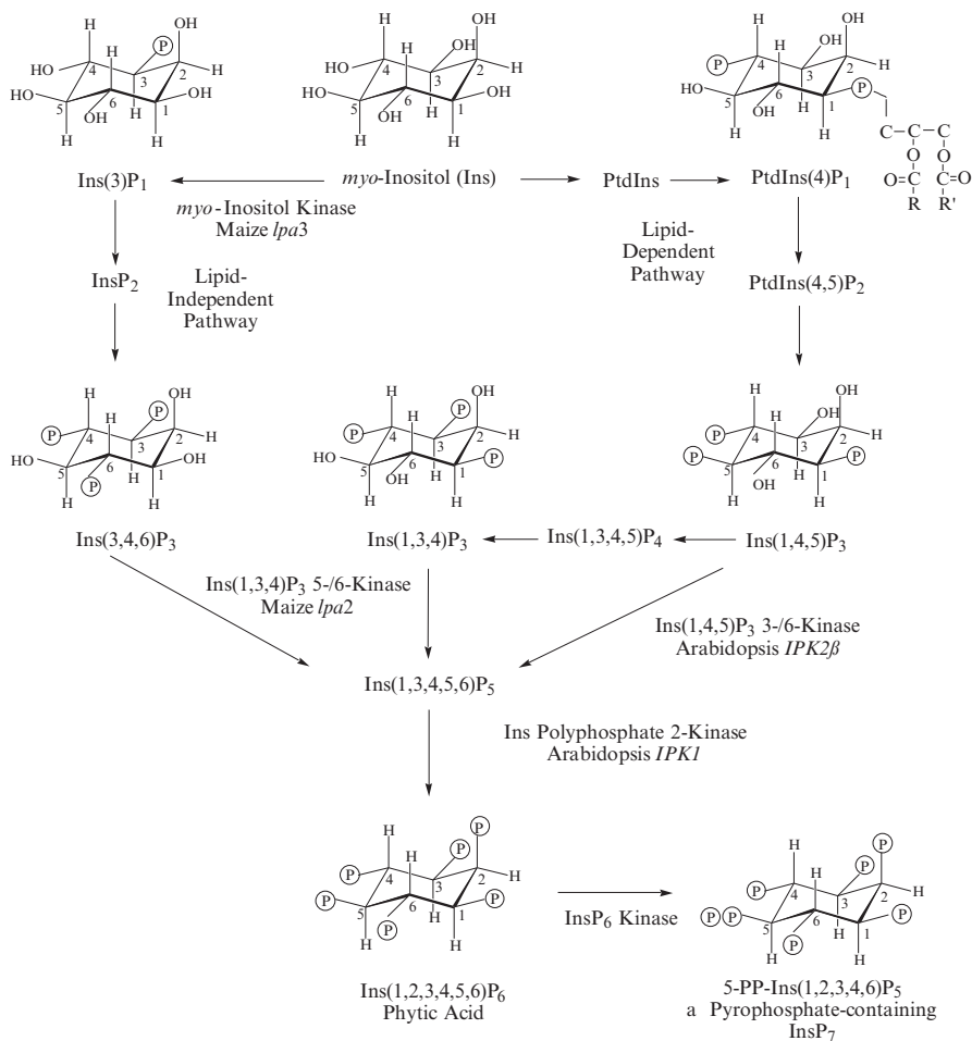
Fig. 4 Biochemical pathways leading from myo -inositol (Ins; top center) to Ins(1,2,3,4,5,6)P 6 or phytic acid (bottom center) in developing seed. On the top left is the pathway which proceeds via “lipid-independent” precursors, while on the top right is the pathway that proceeds via “lipid-dependent” precursors that include phosphatidylinositol (PtdIns) and PtdIns phosphates. P = H 2 PO 4
