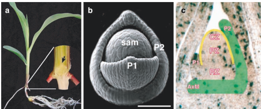
Fig. 1 Location, morphology and histology of the maize seedling SAM. (a) A maize seedling at about 10 days post germination, with four visible leaves. Inside the whorl several additional leaves are tightly wrapped around the SAM. To the right is shown an enlarged median section through the shoot, at a position corresponding to the white lines, with the position of the SAM arrowed. At this stage of development the SAM is at the summit of a small region of unexpanded stem, at about 2–3 mm above the root-shoot junction. (b) Further dissection and careful removal of most of the leaf primordia reveals the SAM and the most recently initiated leaf primordia, P1 and P2, viewed here in the scanning electron microscope. Scale bar = 100 \mu\text{m} (figure adapted from Jackson and Hake, 1999). (c) A longitudinal section through the SAM, showing the cellular organization of the meristem (L1 layer of SAM is shaded yellow, the P2 “phytomer” in green) AxM = axillary meristem of the P2 phytomer. In the figure, the distribution of cell divisions is marked by dark punctate in situ staining of a cyclin mRNA (figure adapted from Jackson and Hake, 1999). The SAM zones are also labeled, central zone (CZ), peripheral zone (PZ) and rib zone (RZ). Note the relatively low rate of cell division in the SAM compared to the leaf primordia, except for the region on the right flank of the SAM, which corresponds to the P0 site of leaf initiation opposite the P1
