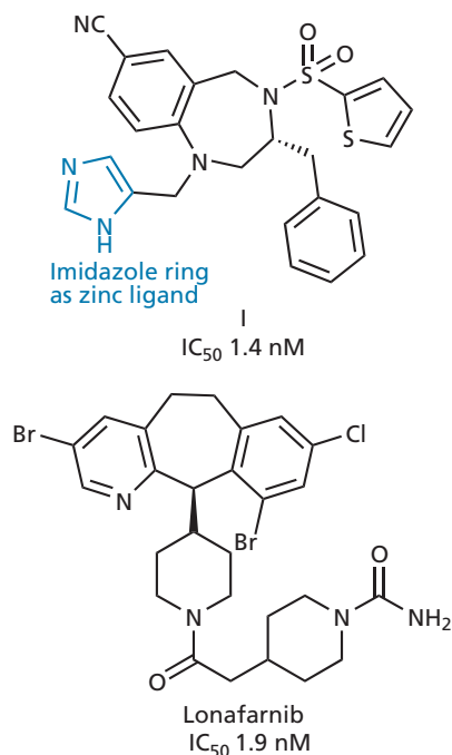
FIGURE 21.45 Non-peptide-like inhibitors of Ftsase undergoing clinical trials.
