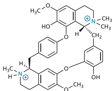
FIGURE 1 Computer-generated model of tubocurarine (Chem3D).
