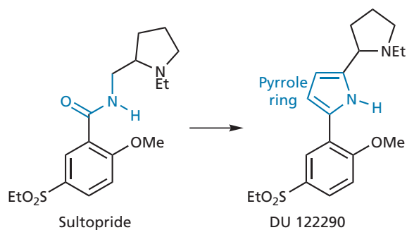
FIGURE 13.47 Introducing a pyrrole ring as a bioisostere for an amide group.
