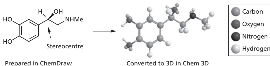
FIGURE 17.2 Conversion of a 2D drawing to a 3D model.
