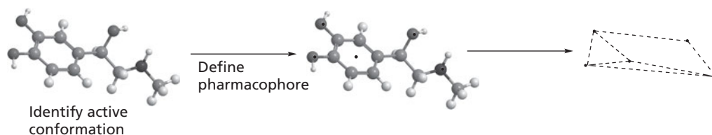
FIGURE 18.20 Identification of the active conformation and pharmacophore.
