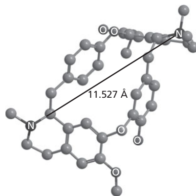
FIGURE 1 Computer-generated model of tubocurarine (Chem3D).
