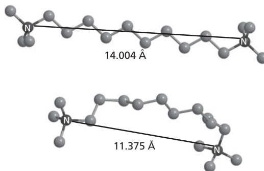
FIGURE 2 Computer-generated conformations of decamethonium (Chem3D).
