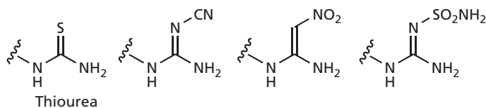
FIGURE 13.46 Non-classical isosteres for a thiourea group.
