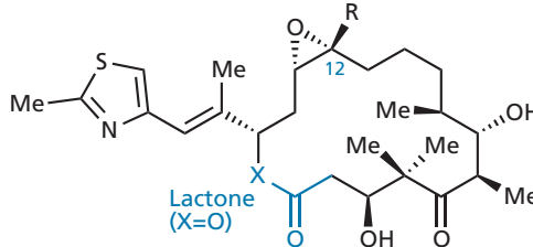
Epothilone A: R=H, X=O Epothilone B: R=Me, X=O BMS 247550: R=Me, X=NH
