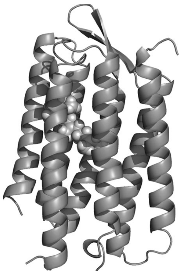
FIGURE 17.44 Bacteriorhodopsin with bound retinal.
