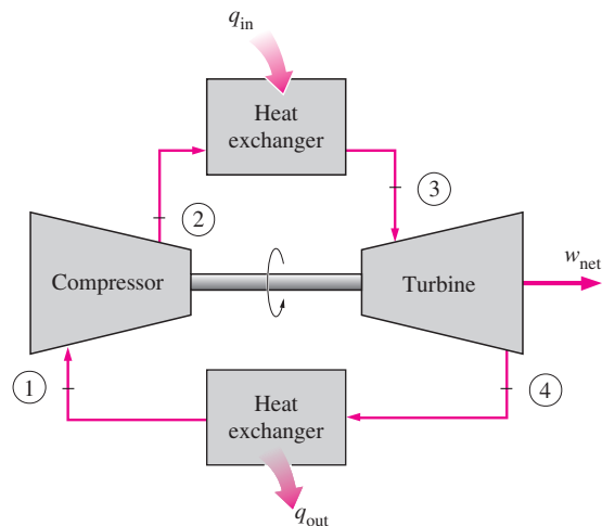
FIGURE 9-30 A closed-cycle gas-turbine engine.
