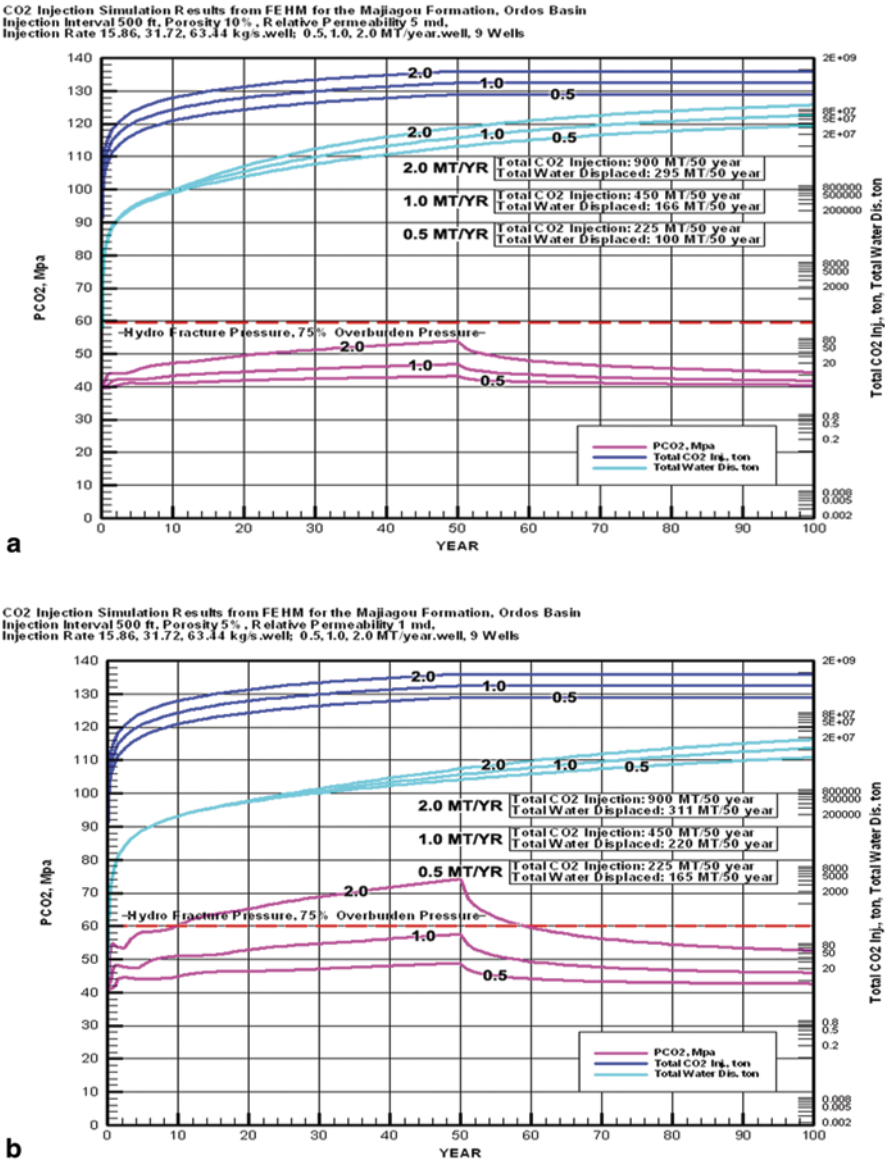
Fig. 13.3 FEHM simulation results for various porosities, permeabilities, and CO 2 injection rates. (From Jiao et al. 2011)
