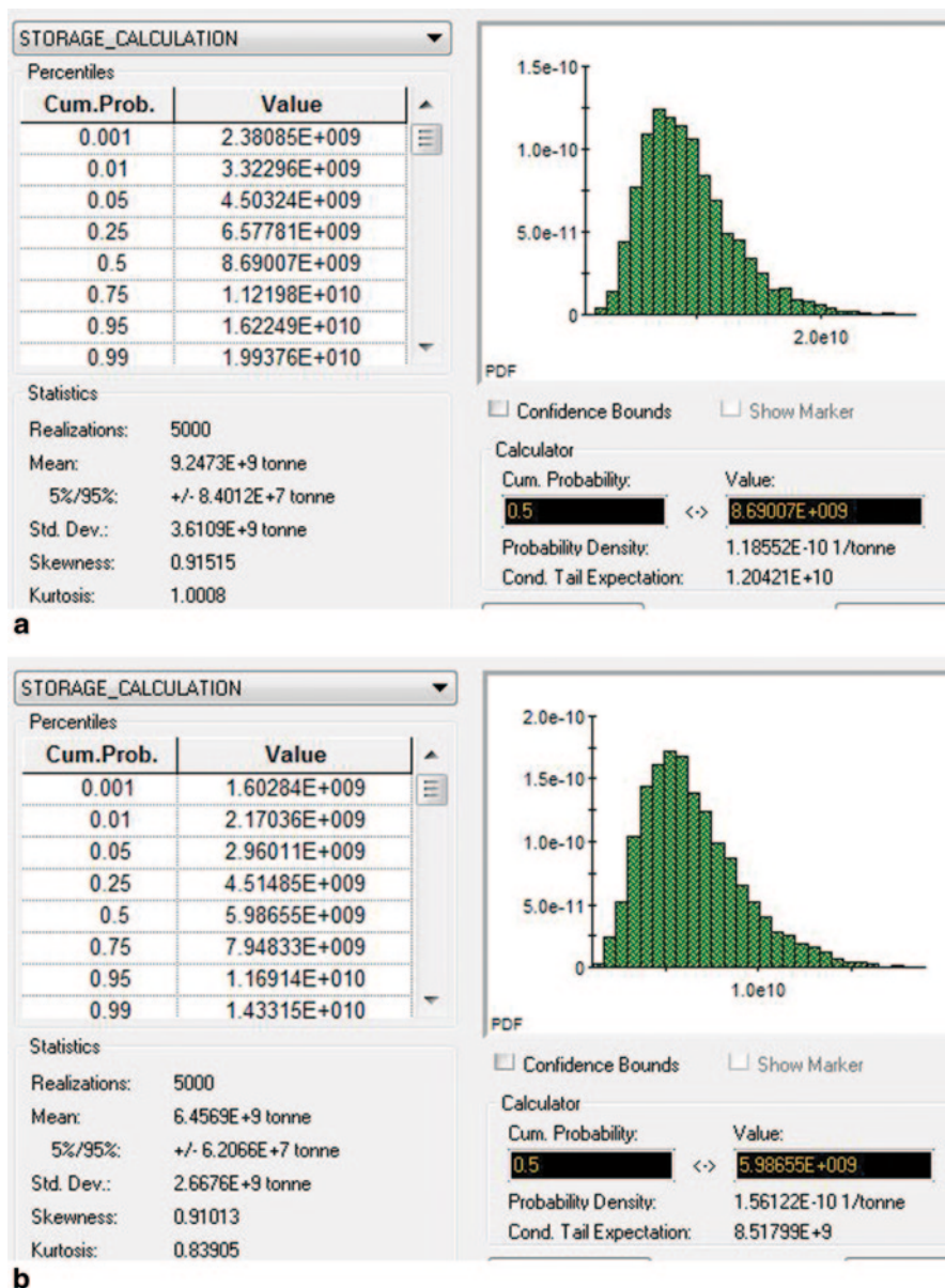
Fig. 10.4 (a) Probability density of the CO 2 storage capacity of the Weber Sandstone in the RSU. A cumulative probability of 25% yields a value of 6.6 Gt. This indicates that for this particular distribution, we have a 25% chance of storing 6.6 Gt of CO 2 or less. Put another way, this indicates that we have a 75% chance of storing at least 6.6 Gt CO 2 in the Weber Sandstone on the RSU. (b) Probability density of the CO 2 storage capacity of the Madison Limestone on the RSU. A cumulative probability of 25% yields a value of 4.5 Gt. This indicates that we have a 75% chance of storing at least 4.5 Gt CO 2 in the Madison Limestone on the RSU
