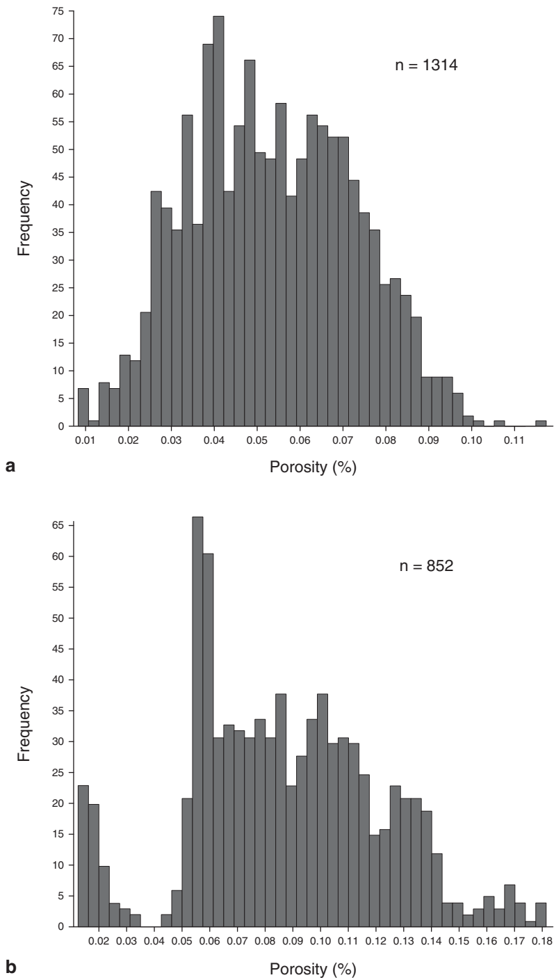
Fig. 10.3 Histograms of the density-neutron porosity of (a) the Weber Sandstone and (b) the Madison Limestone, Rock Springs Uplift
