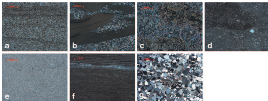
Fig. 6.11 (a) 10,601.9 ft (3231 m) Typical cross-bedded Triassic siltstone. (b) 10,640.1 ft (3243 m) Intraclasts of shale in Triassic siltstone. Intraclasts of mudstone, shale, and carbonates are common. The matrix of the siltstone is predominantly anhydrite. (c) 10,633.8 ft (3241 m) Chicken-wire anhydrite nodules with halite in Triassic siltstone suggest precipitation in hypersaline, evaporative conditions. (d) 12,224 ft (3726 m) Clastic shale with hematitic mudstone intraclast in the Amsden Formation. (e) 12,199 ft (3718 m) Dolostone; sub- to euhedral dolomite crystals with detrital quartz and authigenic pyrite. Amsden carbonates, such as this dolostone, typically lack porosity. (f) 12,225 ft (3726 m) Hematitic, laminated shale at the base of the Amsden formation. Note the dolomitized layer near the top of the slide. (g) 12,215.6 ft (3723 m) Clastic siltstone in the Amsden Formation with carbonate and anhydrite cement. Aside from contact points, detrital grains are mostly free of pressure solution deformation
