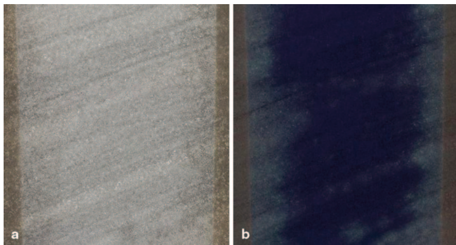
Fig. 6.7 Core samples from the Weber Sandstone at 11,481.4 ft (3500 m) deep. (a) Eolian sandstone showing pinstriped cross-bedding under white light illumination. (b) Ultraviolet image of a, showing fluorescence due to the presence of hydrocarbon (natural or introduced during core extraction). Width of the field is 5 cm
