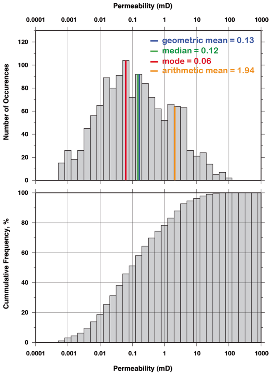
Fig. 9.10 Permeability distribution within the Weber Sandstone unit (11,155–11,825 ft depth interval; 1,341 data samples). Ordinary histogram ( top ); cumulative histogram ( bottom )
