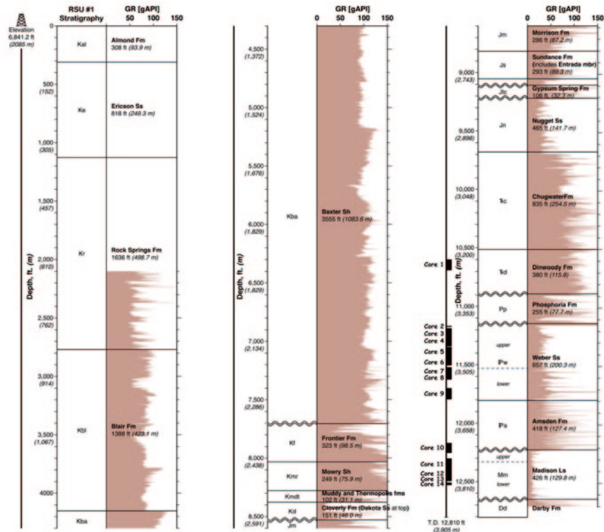
Fig. 5.5 Stratigraphic column for the RSU #1 well including gamma log and cored intervals
