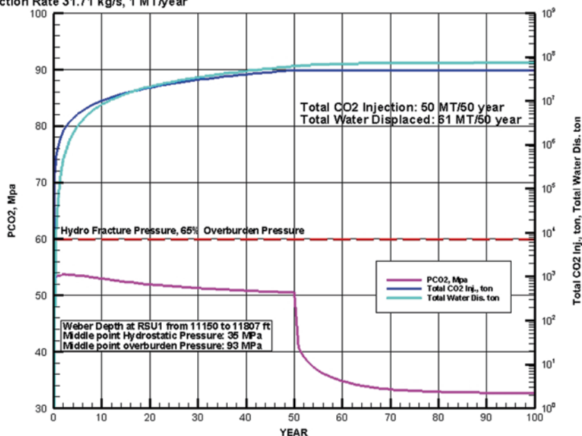
Fig. 10.6 FEHM CO 2 injection simulation results for the Weber Sandston, RSU. The simulation was set up for homogenous reservoir petrophysical conditions with 10% porosity and 1 mD relative permeability. The injection rate of 31.71 kg/s was constant for 50 years; then injection ceased, and the simulation ran for another 50 years without CO 2 injection. The reservoir pressure elevated quickly when injection began but was below the hydro-fracture pressure throughout injection. After injection ceased, the reservoir pressure fell back to near the original reservoir pressure within 10 years
