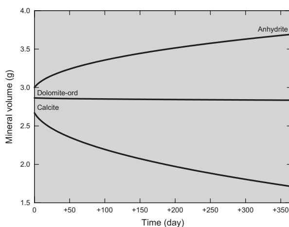
Fig. 8.6 Modeling results in the Madison show calcite dissolution and anhydrite precipitation in response to \text{CO}_2 injection. Dolomite shows only slight dissolution
