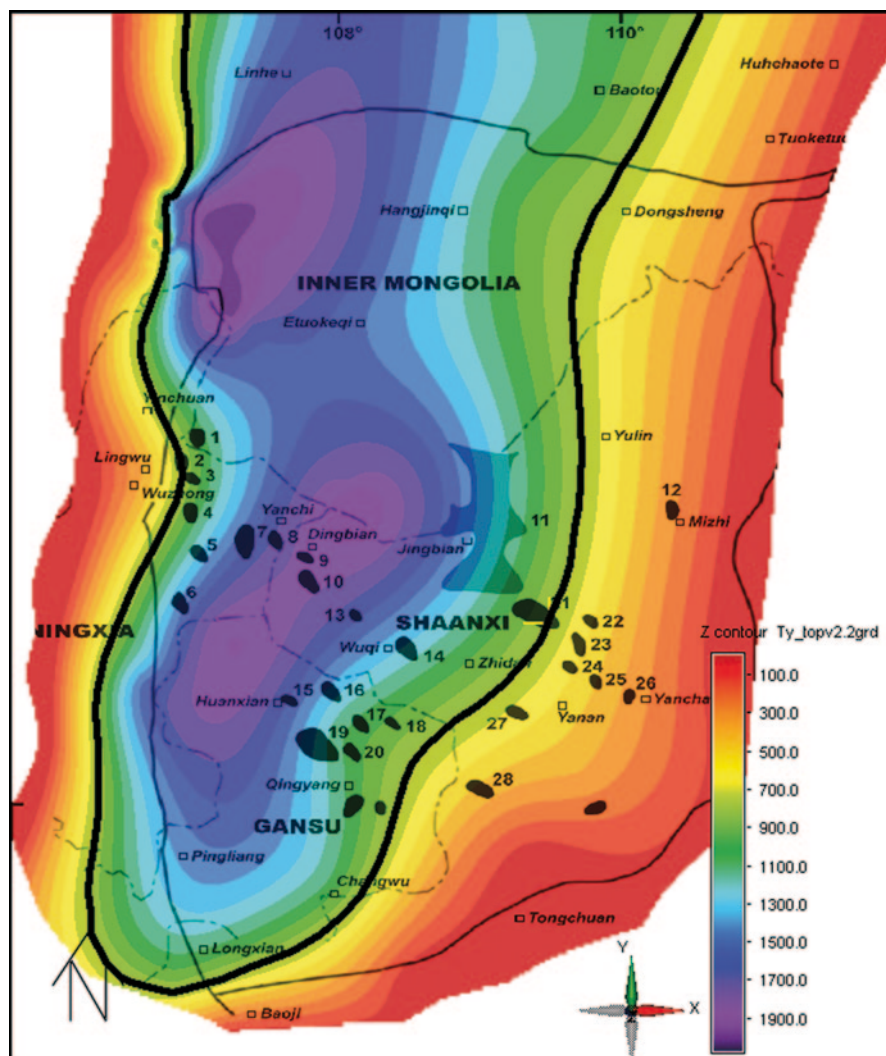
Fig. 13.5 Yanchang Formation oil fields superimposed on a map of the burial depth of the Yanchang Formation top
