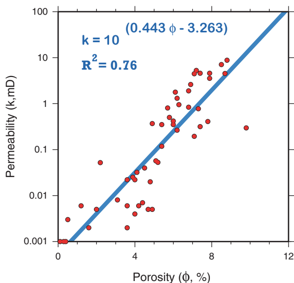
Fig. 9.7 Semilog plot of permeability vs. porosity for the core samples from the Weber Formation, RSU #1 well, Rock Springs Uplift, Wyoming ( red dots ). The corresponding semi-logarithmic regression for permeability k (the line, equation, and coefficient of determination) is shown in blue
