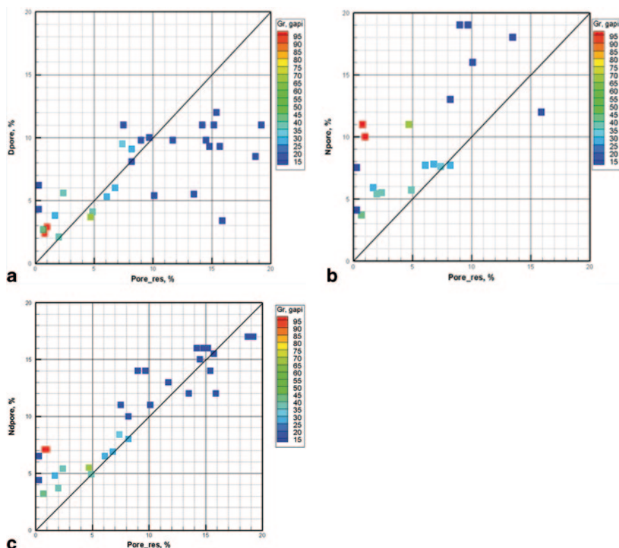
Fig. 10.11 Crossplot of the laboratory measured porosity at reservoir conditions vs. the log-derived (a) bulk density porosity and (b) neutron porosity. (c) Crossplot of the laboratory measured porosity at reservoir conditions vs. the log derived neutron-density porosity
