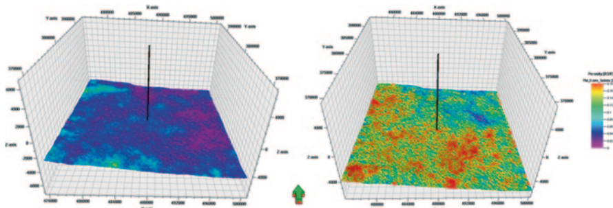
Fig. 10.18 The porosities derived from the seismic interval velocities for the Weber Sandstone ( left ) and the Madison Limestone ( right ) show significant heterogeneous characteristics in the geologic CO 2 storage simulation domain
