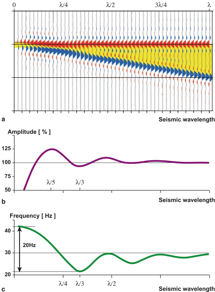
Fig. 7.22 (a) Low-impedance wedge model (yellow) and its seismic response generated using zero-phase Ormsby wavelet with frequency passband 8–48 Hz. (b) Amplitude and (c) mean frequency variations estimated on top of the wedge
