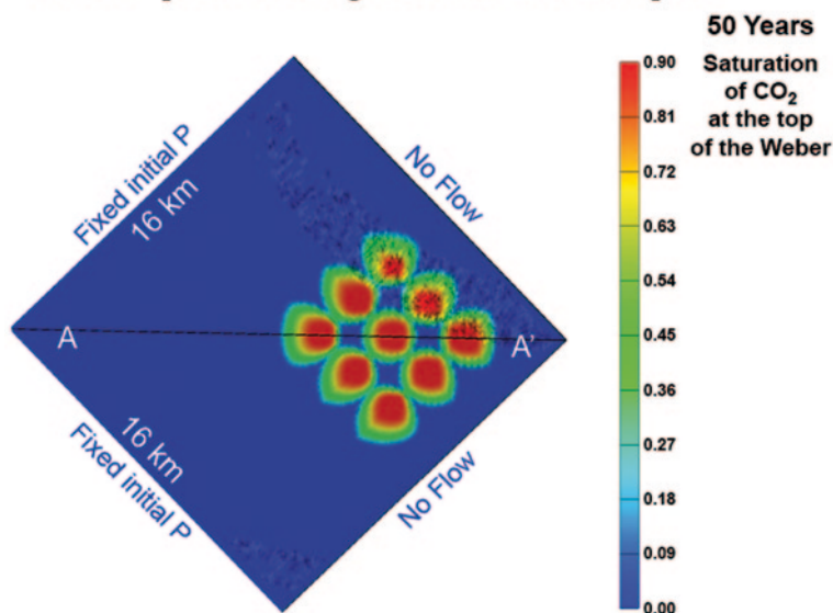
Fig. 11.3 The 750 Mt CO 2 injection over a period of 50 years at the Rock Springs Uplift (see Fig. 11.1 and 11.2) is contained within the Weber Sandstone beneath a 16 × 16-km area. (Modified from Stauffer et al. 2009)
