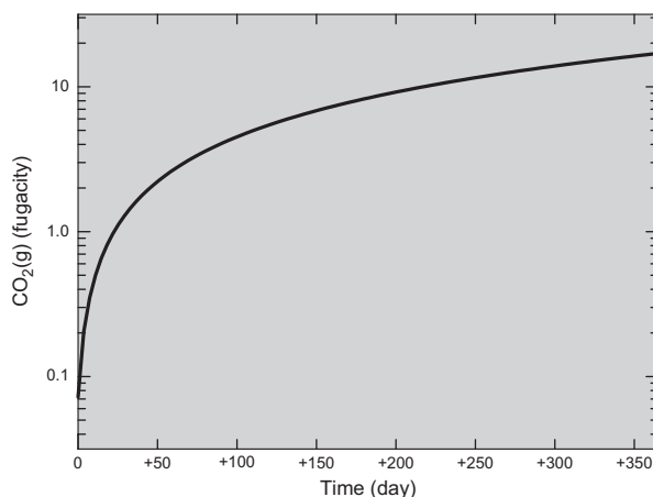
Fig. 8.5 Modeling results for the Madison show increases in P(\text{CO}_2) from \text{CO}_2 injection and calcite dissolution
