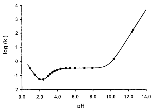
Figure 3.3 Rate of hydrolysis (log k ) of aspirin in aqueous media (ionic strength 0.5M) as a function of pH at 25°C (from studies by Some et al. , 2000 which is similar to data from Edwards, 1950; 1952 performed at 20°C). Reproduced from International Journal of Pharmaceutics , 198 : 39–49. (© 2000 with permission of Elsevier Science.)
