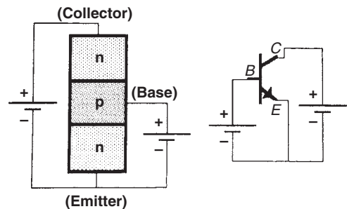
Figure 1-11. An npn junction bipolar transistor showing the potential applied between the emitter, E, and base, B, that controls the flow of current between the emitter and the collector, C. The figure on the right shows the circuit, using the conventional symbol for the transistor (From Misulis, K. E. 1989. Basic electronics for clinical neurophysiology. Journal of Clinical Neurophysiology 6:41–74. By permission of the American Clinical Neurophysiology Society.)
