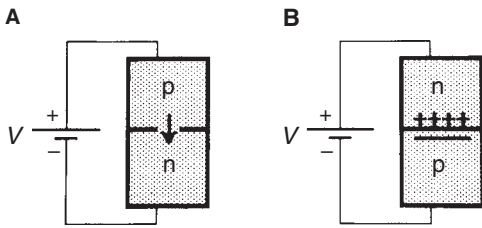
Figure 1-10. A, A forward-biased pn semiconductor junction permits current flow. B, A reverse-biased junction prevents current flow. V, Potential across the semiconductor junction. (From Misulis, K. E. 1989. Basic electronics for clinical neurophysiology. Journal of Clinical Neurophysiology 6:41–74. By permission of the American Clinical Neurophysiology Society.)
