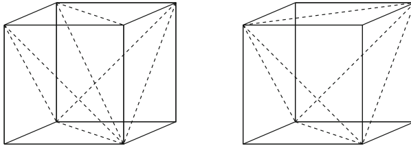
Fig. 3.2 Two (very different) triangulations of the 3-cube.
