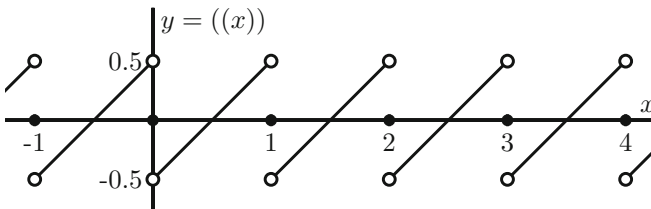
Fig. 7.1 The sawtooth function y = ((x)) .
