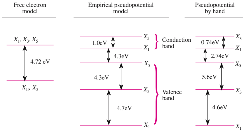
Fig. 2.28. The lowest energy bands at the X point of GaAs computed by the nearly free electron model, the EPM, and the perturbation approach of Problem 2.8. The X_1 – X_3 notation corresponds to v_j^a > 0 , i. e., to placing the cation at (a/4)(111) and the anion at the origin.
