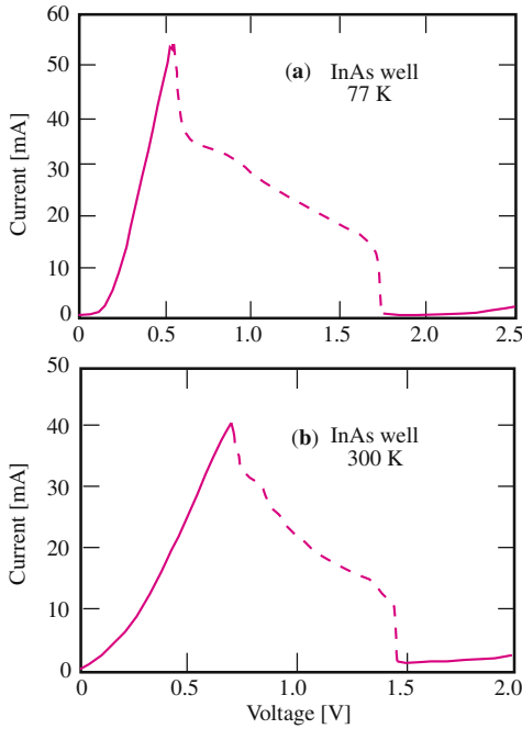
Fig. 9.37. The I-V characteristics of the 30 \times 30 \text{ } (\mu\text{m})^2 pseudo-morphic InGaAs/AlAs/InAs resonant tunneling diode shown in Fig. 9.36, measured at (a) 77 K and (b) 300 K. Notice the very large peak-to-valley current ratio in this device found even at room temperature. From [9.71]
