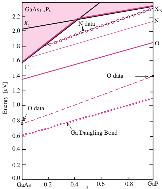
Fig. 4.8. The energy of an A_1 -symmetry deep level for N substituting an anion (labeled “N data”) in GaAs_{1-x}P_x alloy as a function of the alloy composition x . The open circles are experimentally measured energies of an exciton bound to an isolated N center while the line labeled “N” represents the theoretical values. The point X_N represents an exciton bound to a neutral nitrogen. The lines labeled “O data” and “Ga dangling bond” are not relevant to this chapter. (From [4.29]). \Gamma_c and X_c denote, respectively, conduction band minima at the \Gamma and X points of the Brillouin zone
