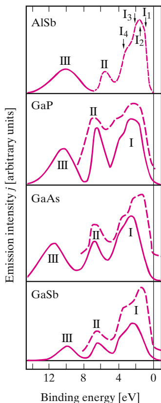
Fig. 8.14. XPS spectra of GaP, GaAs, GaSb, and AlSb ( solid lines ) and UPS angle-integrated spectra ( \hbar\omega_L = 21.2 eV, dashed lines ). The notation I_i denotes structures corresponding to critical points [Ref. 8.2, p. 57]
