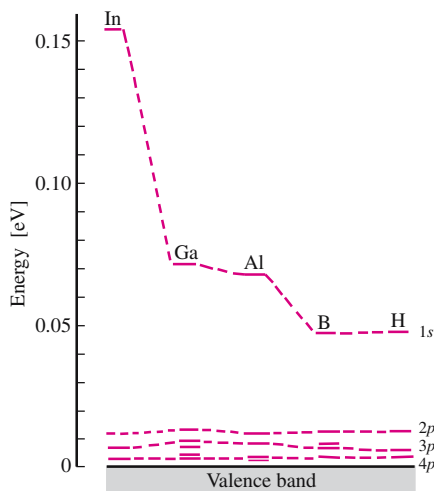
Fig. 3. Suggested term scheme for group III acceptors in Si showing the levels whose energies are derived from the low temperature absorption spectra [6]
