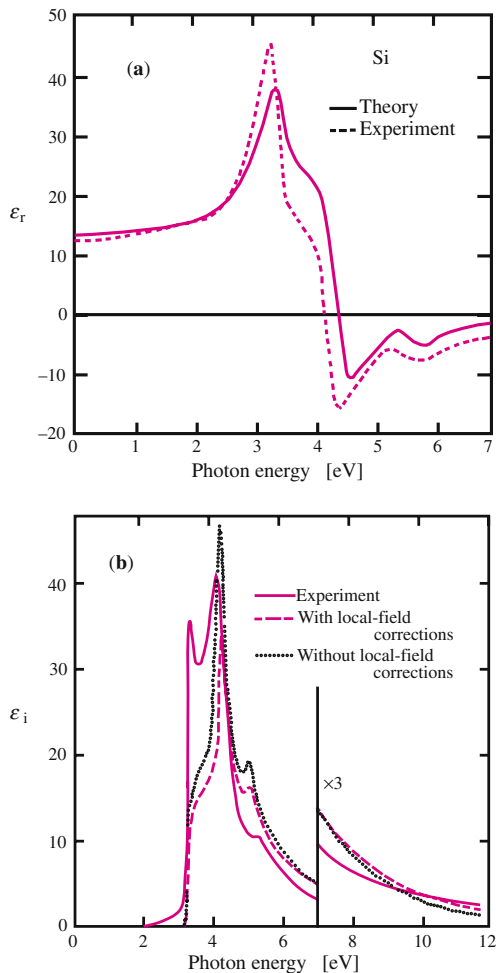
Fig. 6.10a,b. A comparison between the experimental and calculated dielectric function of Si: (a) real part and (b) imaginary part. In (b) the results of two theoretical calculations, one including and the other excluding local-field corrections, are presented [6.21]. For more recent theoretical results see [6.22, 23]. The local field corrections are due to changes in the higher Fourier components of the crystal (pseudo)-potential induced by the electromagnetic field. Note that, according to (b), their effect is small; they do not improve agreement with experimental data. The sharp peak observed at 3.3 eV has been attributed to excitonic effects (see Sect. 6.3.3 and [6.24])
