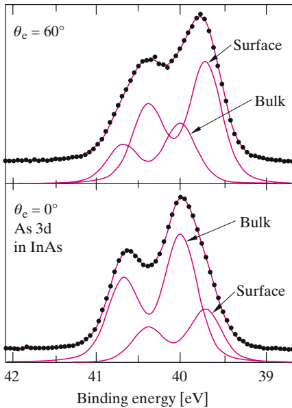
Fig. 8.22. Spectra of the 3d core levels of As measured on an InAs(110) surface with synchrotron radiation (105 eV excitation) using two different azimuthal angles, \theta_e = 0 and 60 . Note the decomposition of the j = (5/2, 3/2) doublet into a surface and a bulk component: the former is stronger for the larger \theta_e [8.46]
