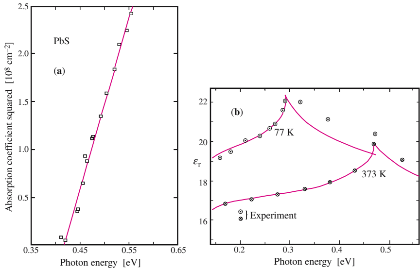
Fig. 6.14. (a) Plot of the square of the absorption coefficient of PbS as a function of photon energy showing the linear behavior discussed in the text. The intercept with the x-axis defines the direct energy gap. Reproduced from [6.30]. (b) Fits ( curves ) to the experimental values of the real part of the dielectric function of PbS ( data points ) measured at 77 and 373 K with the expression in (6.59). Reproduced from [6.144].
