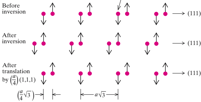
Fig. 2.7. Schematic diagrams of the transformation of (a) the acoustic phonon and (b) the zone-center optical phonon in diamond under inversion plus translation by (a/4)(1,1,1) where a is the size of the unit cube of diamond
