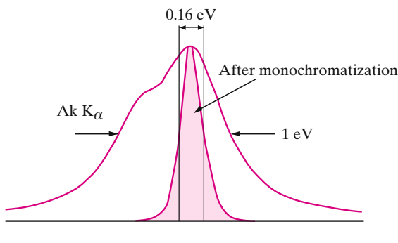
Fig. 8.10. Profile of the Al K_\alpha line used in XPS as produced by the X-ray tube (width 1 eV) and after monochromatization (width 0.16 eV) [8.24]
