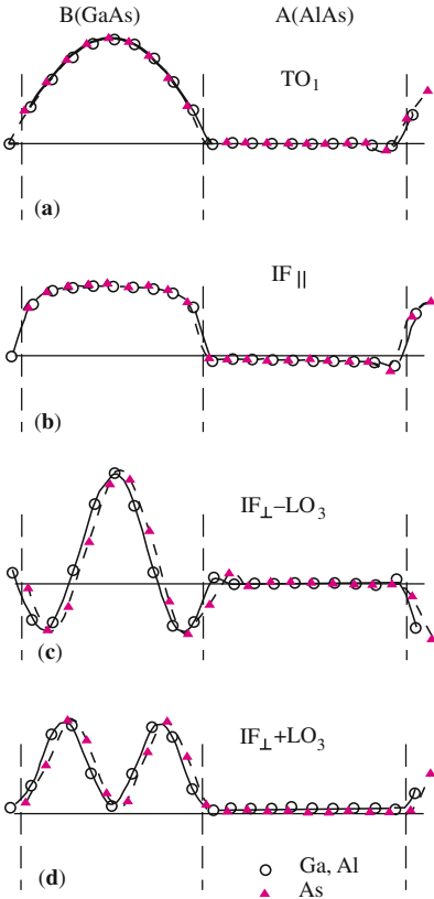
Fig. 9.22. (a) Envelope function for the TO 1 confined modes (i. e., \Theta = 0 ) of a (GaAs) 9 (AlAs) 10 superlattice grown along [111]. (b) The equivalent modes for \Theta = \pi/2 showing the typical flat-top pattern of these so-called interface modes. [Note that, in spite of their name, these modes are not confined to the neighborhood of the interfaces since q_x is infinitesimally small. However, the “interface” label may still be justified since they come closer to the interfaces than the confined mode shown in (a).] (c, d) The envelope function for the \Theta = \pi/2 LO-like, IF and m = 3 modes, showing that they can be decomposed into a mixture of a flat-top mode of the (b) type and an m = 3 confined mode. From [9.44]
