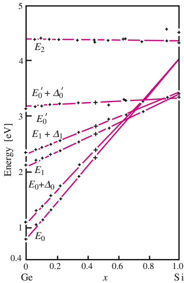
Fig. 6.51. Variation with composition of the energies of the E_0 , E_0 + \Delta_0 , E_1 , E_1 + \Delta_1 , E'_0 , and E_2 electroreflectance peaks observed in the Ge-Si alloy system at room temperature by the electrolyte method [6.125]
