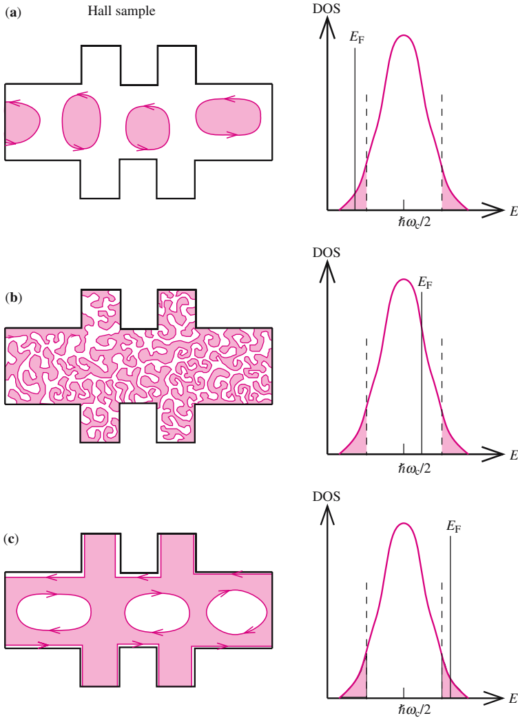
Fig. 9.41a–c. Schematic picture of the quantum Hall droplet (shaded areas), orbit of the edge electrons (curve with arrows) and density of states (DOS) for three positions of the Fermi energy E_F relative to the mobility edge. (a) E_F below the mobility edge in the localized region (shaded region in the DOS plots); (b) E_F in the delocalized regime and (c) E_F in the localized region again but now above the delocalized states. The DOS are representative of a finite size sample at T > 0
