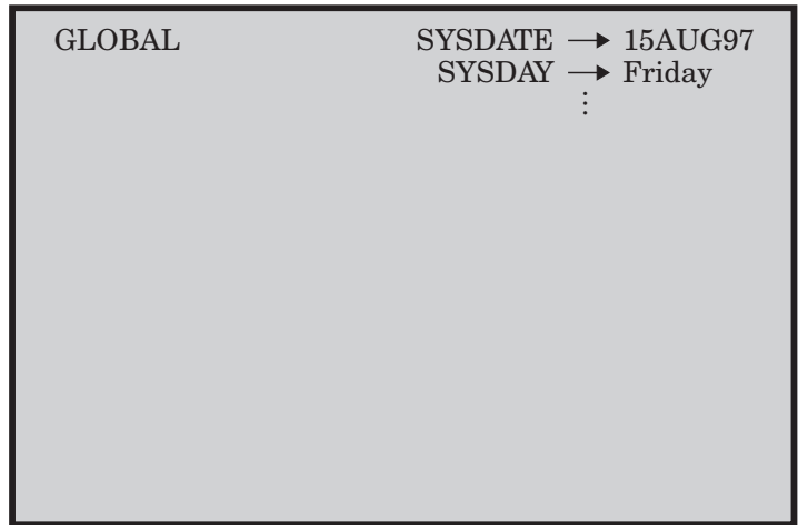
Figure 5.9 The Symbol Tables with the CALL SYMPUT Routine Generating a Complete DATA Step
