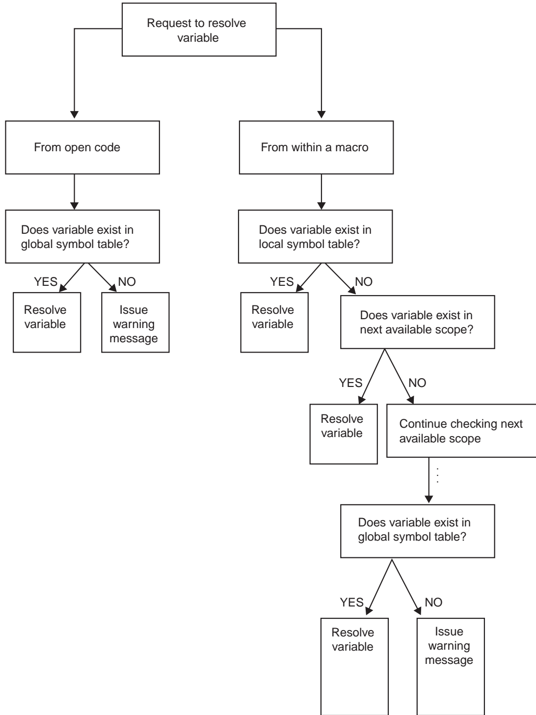
Figure 5.4 Search Order When Resolving Macro Variable References
