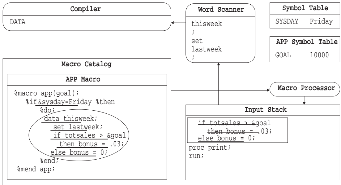
Figure 4.9 Generated Text on Top of Input Stack
