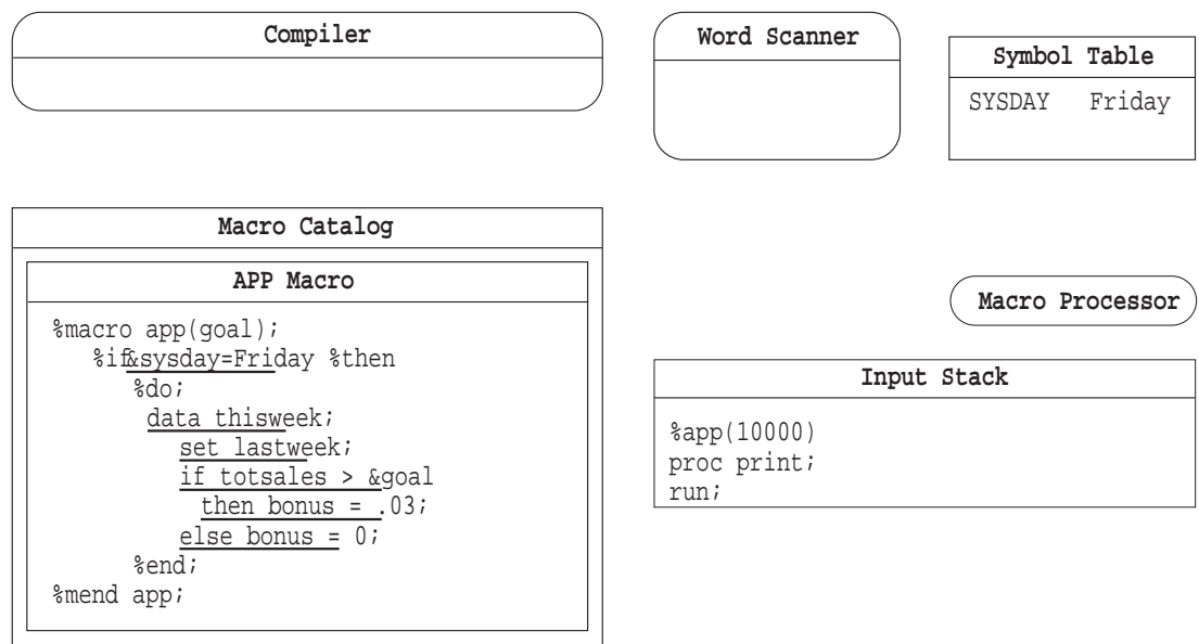
Figure 4.3 The Compiled Macro APP
