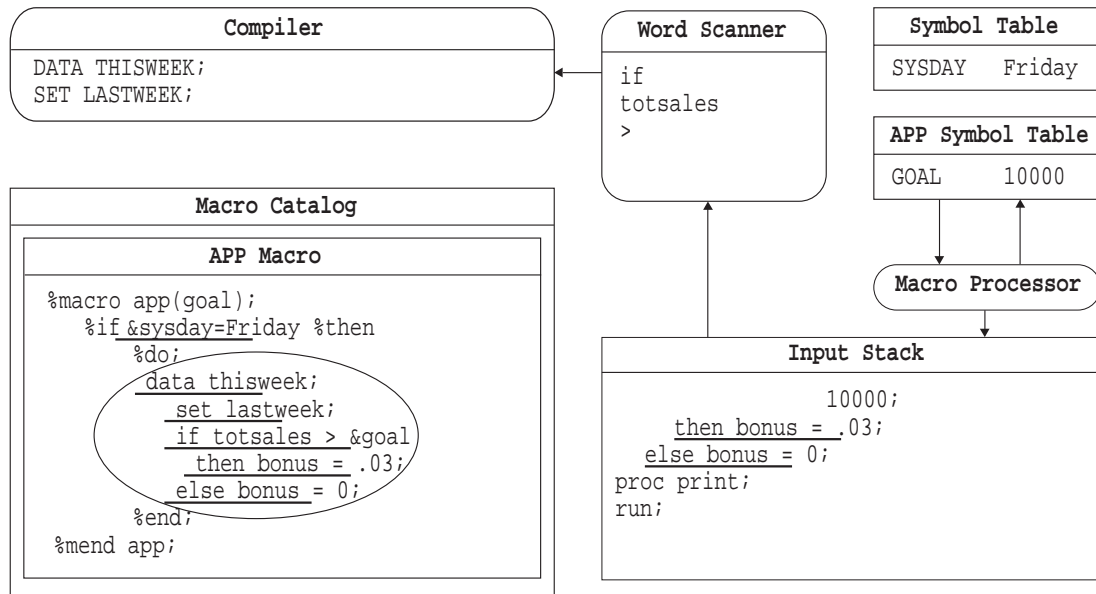
Figure 4.10 The Word Scanner Reads Generated Text
