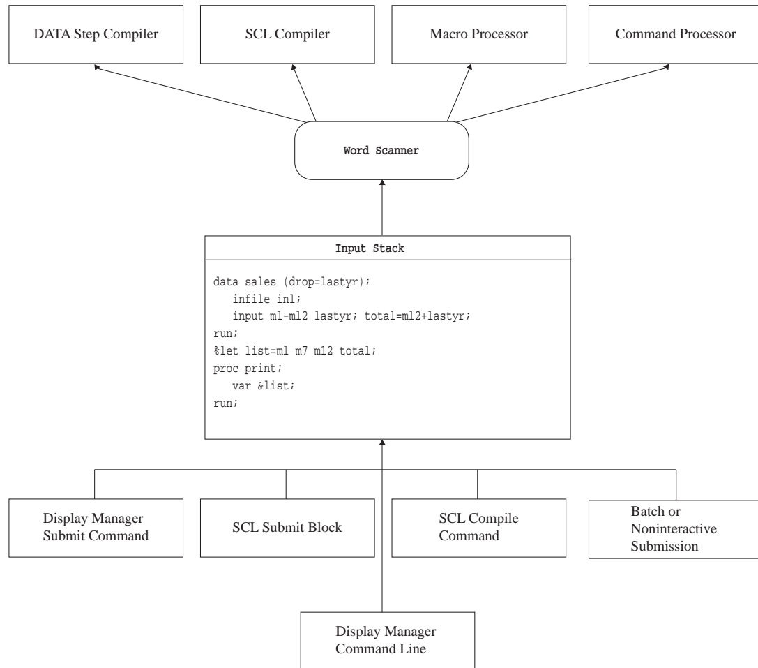
Figure 2.1 Submitted Programs are Sent to the Input Stack
