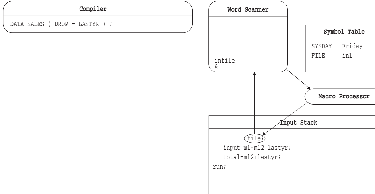
Figure 2.9 The Macro Processor Examines &FILE
